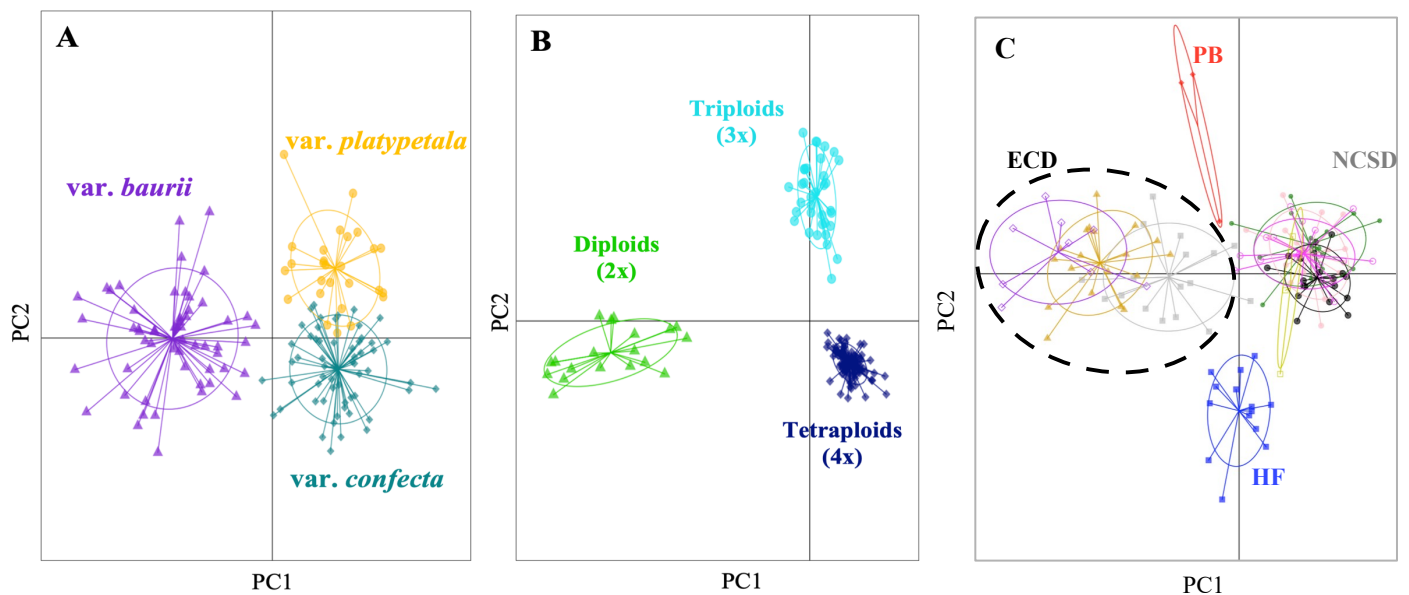
Figure 19. DAPC based on Bruvo genetic distance matrix grouped by A) taxonomic varieties with R. baurii var. baurii (purple triangles), R. baurii var. platypetala (yellow circles) and R. baurii var. confecta (blue diamonds), B) grouped by ploidy levels with diploids (2 \times , green triangles), triploids (3 \times , light blue circles) and tetraploids (4 \times ) shown in navy diamonds and C) grouped by populations with each colour representing a different population, showing the Eastern Cape Drakensberg (ECD) populations grouping together on the left of PC1 (encircled by a black dashed ellipse), and the Northern, Central and Southern Drakensberg (NCSD) populations grouping together on the right of PC1 (encircled by a grey dotted ellipse). Two populations present as outliers, Platberg (PB) in red and Hebron Farm (HF) in blue. Points represent individuals and ellipses show groups identified by DAPC.
