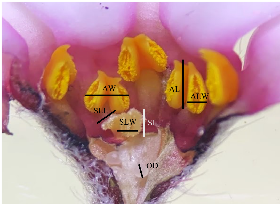
Figure 5. Reproductive morphology measurements in R. baurii varieties: (AL) Anther Length, (AW) Anther Width, (ALW) Anther Lobe Width, (SLL) Stigma Lobe Length, (SLW) Stigma Lobe Width, (OD) Ovule Diameter, (SL) Stigma Length.
