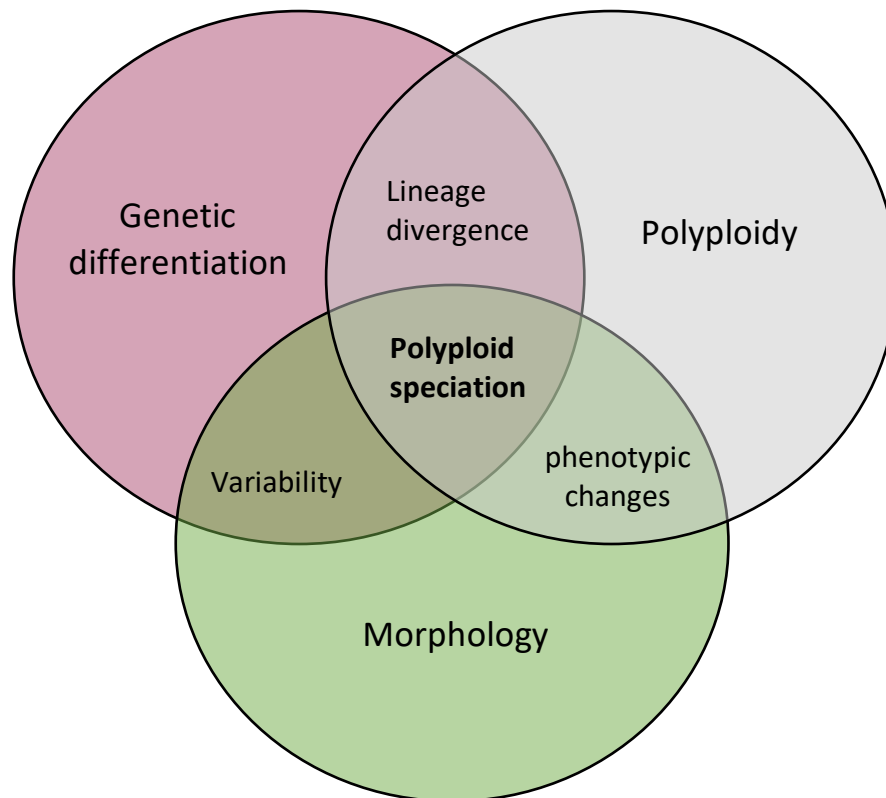
Figure 1. Genetic differentiation, morphological change and changes in polyploidy, when exhibited together, could lead to polyploid speciation events through an increase in variability (both genetic and morphological), phenotypic changes (such as the gigas effect) and lineage divergence.
