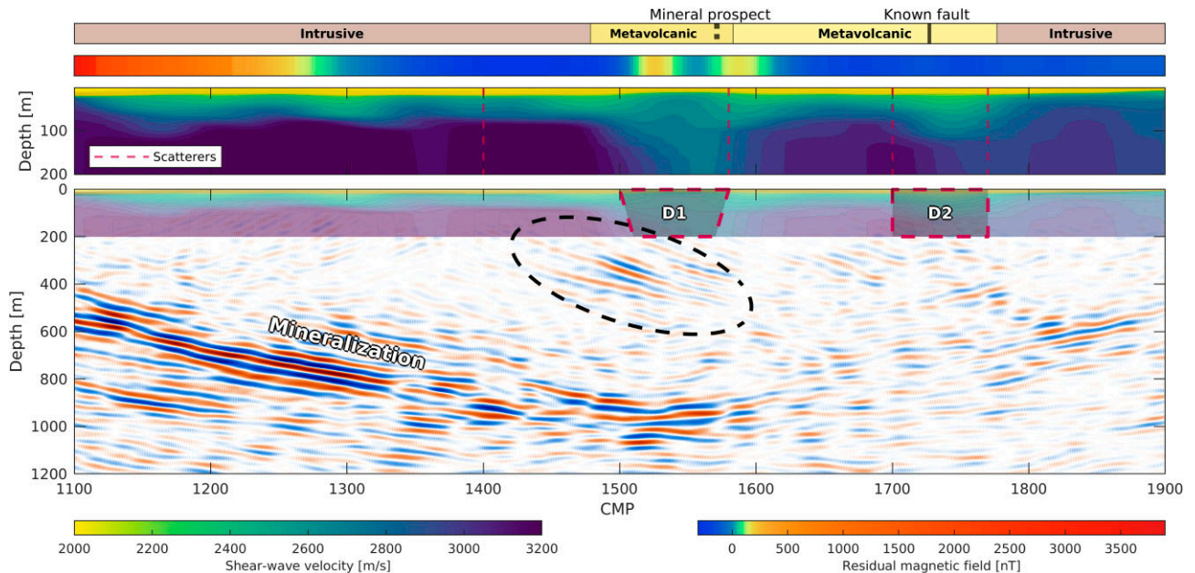
Figure 18. Interpretation of the results using the following panels (top to bottom): surface geology data (SGU 1988), airborne residual magnetic field measurements, shear-velocity section from Fig. 16 with marked scatterers and the same section overlaid (with transparency) on the migrated stacked reflection seismic section (modified after Pertuz et al. 2021). The black ellipse indicates the shallow reflections concordant with the high-shear-velocity anomaly. D1 and D2 mark interpreted deformation zones. The deeper event is the main iron-oxide mineralization (Pertuz et al. 2021).
