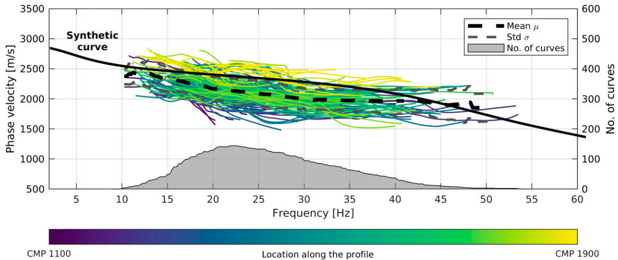
Figure 11. Active source dispersion curves extracted along the profile with the synthetic fundamental mode dispersion curve obtained with a velocity model in Table 1 and calculated mean and standard deviation. The right y-axis corresponds to the number of dispersion curves with a particular frequency (grey polygon). The colour scale corresponds to the position along the line. Note a longer frequency axis than in Fig. 7.
