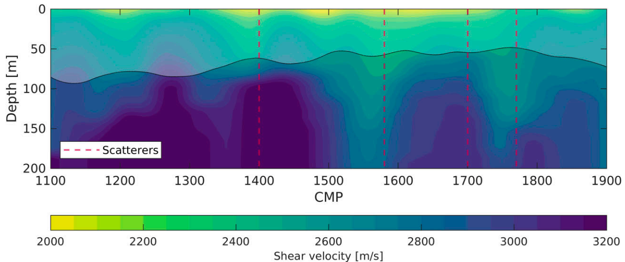
Figure 9. A smoothed passive data 2-D shear-wave velocity section constructed from 1-D models for every fifth CMP. The vertical dashed lines present the position of the scatterers observed in the active data (Fig. 3). The white-shaded area presents the minimum resolution limit according to the \lambda/3 criterion. Colour scale limits were clipped for a better comparison with other data sets.
