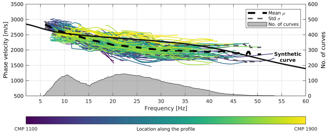
Figure 14. Merged (passive and active) dispersion curves along the profile with the synthetic fundamental mode dispersion curve obtained with a velocity model in Table 1 and a calculated mean and standard deviation. The right y-axis corresponds to the number of dispersion curves with a particular frequency (grey area). The colour scale corresponds to the position along the line. Note a longer frequency axis than in Fig. 7.
