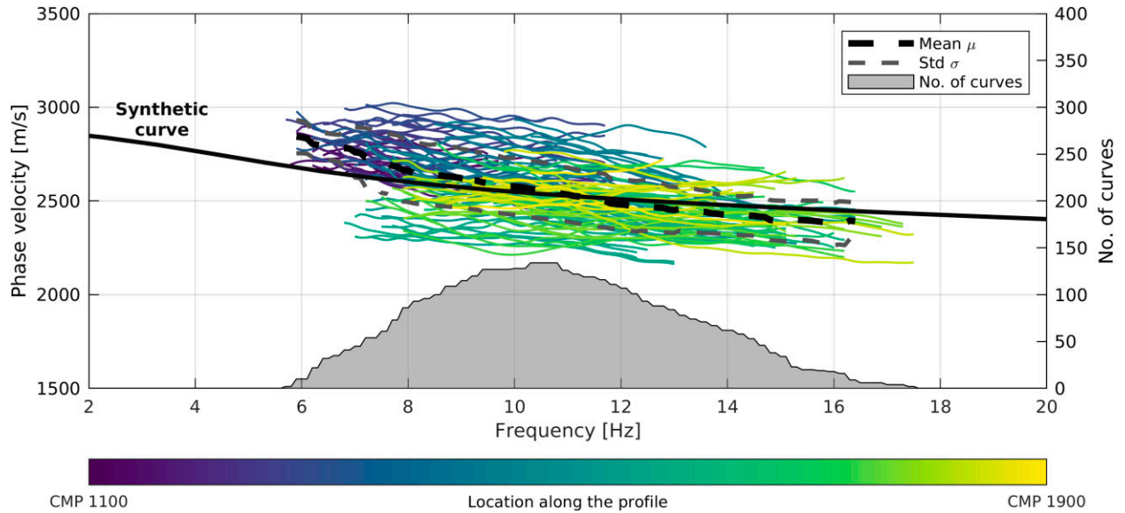
Figure 7. Ambient noise dispersion curves extracted along the profile with the synthetic fundamental mode dispersion curve obtained with a velocity model in Table 1 and calculated mean and standard deviation. The right Y-axis corresponds to the number of dispersion curves with a particular frequency (grey area). The colour scale corresponds to the position along the line.
