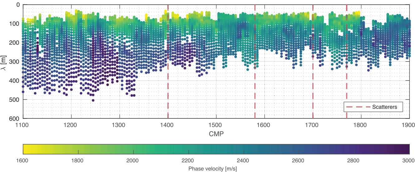
Figure 15. A pseudo-section of merged (passive and active) fundamental mode dispersion curves along the profile with phase velocity colour scaling. The vertical dashed lines present the position of the scatterers observed in the active data (Fig. 3).
