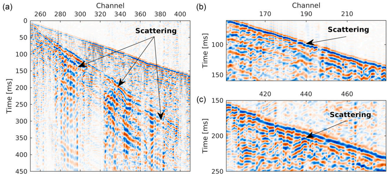
Figure 3. Close-ups of the scattering features observed in active source data. (a) Shot gather 250, channels 290, 340, 380 (CMPs 1580, 1700 and 1770). (b) Shot gather 100, channel 187 (CMP 1400). (c) Shot gather 250, channel 440 (CMP 1900).
