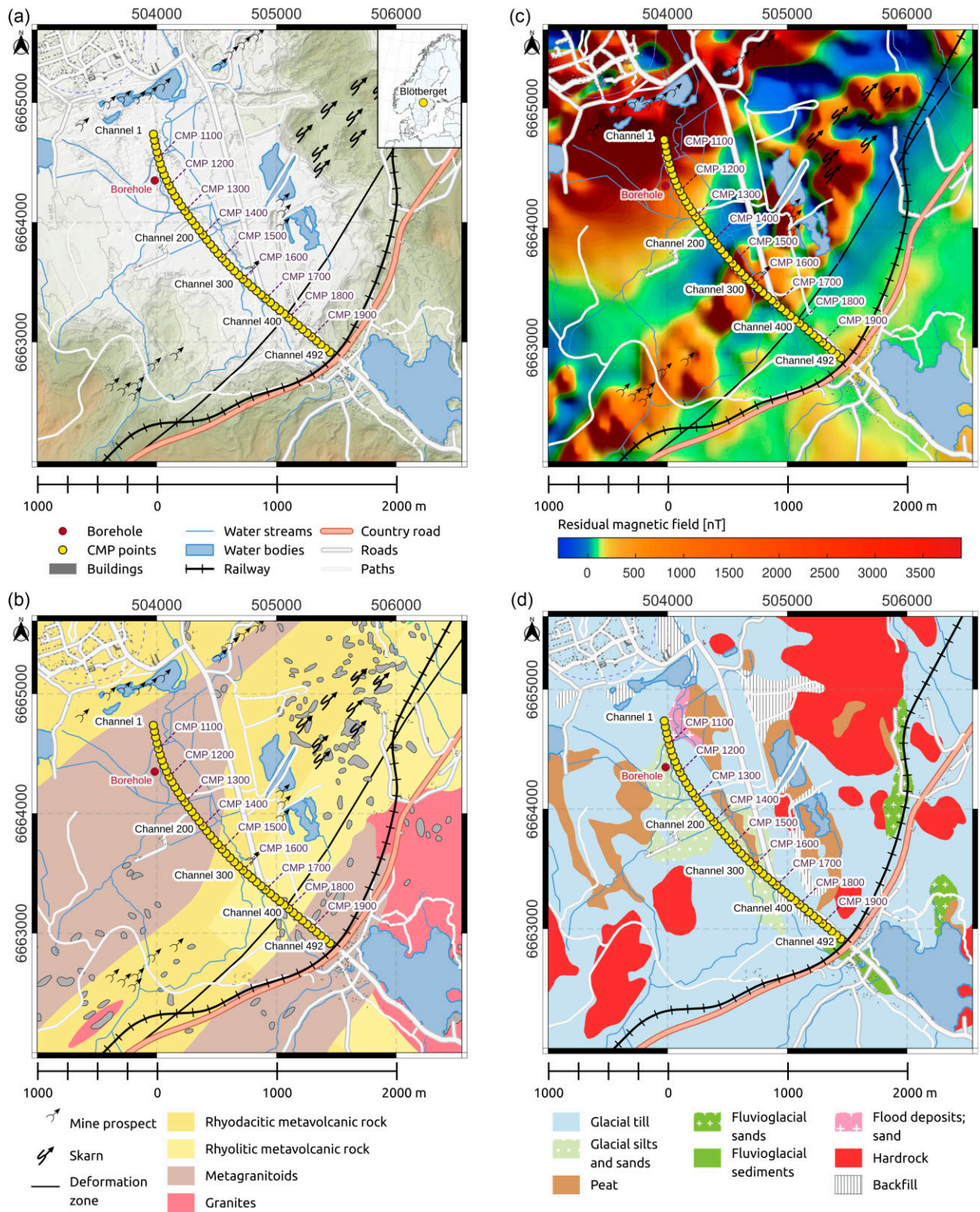
Figure 1. Maps presenting profile channels and common midpoints (CMP) with available geodata. (a) Topography map with elevation profile. (b) Bedrock geology map, modified from Geological Survey of Sweden (SGU, 1988, 2018a). (c) Airborne residual magnetic anomaly map with mineral prospects locations. (d) Soil type map, modified from SGU (2018b).
