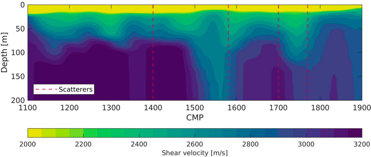
Figure 16. A smoothed merged data (passive and active) 2-D shear-wave velocity section constructed from 1-D models for every fifth CMP. The vertical dashed lines present the position of the scatterers observed in the active data (Fig. 3). Colour scale limits were clipped for a better comparison with other data sets.
