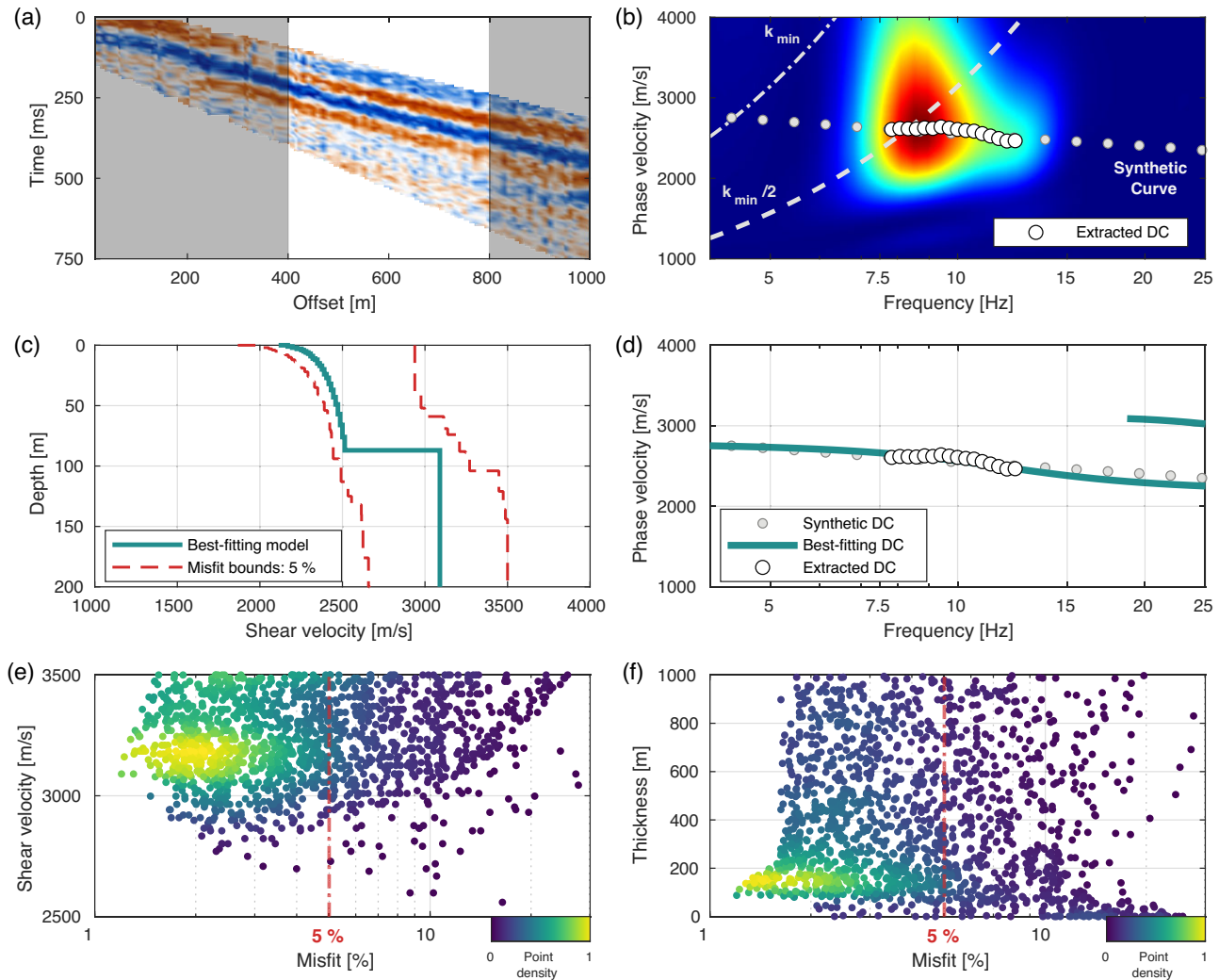
Figure 6. Presentation of the components of the surface-wave analysis (passive data) for virtual CMP 1340. (a) Noise-retrieved CMP gather with top and bottom mutes around the surface-wave arrival. Grey and white polygons present the used array length and source-array offset. (b) Frequency-phase velocity matrix (semblance) with wavenumber resolution limits k_{\min} and k_{\min}/2 and the synthetic fundamental mode dispersion curve from a velocity model in Table 1. The X-axis in logarithmic scale. (c) 1-D shear-wave velocity model from the dispersion curve inversion. The best-fitting model has the lowest obtained misfit. (d) Comparison of the extracted DC with dispersion curves corresponding (fundamental and first higher mode) to the best-fitting model and a synthetic curve from the model in Table 1. (e) Parameter space for the shear-wave velocity of the halfspace (bedrock). (f) Parameter space for the thickness of the first layer (weathered bedrock).
