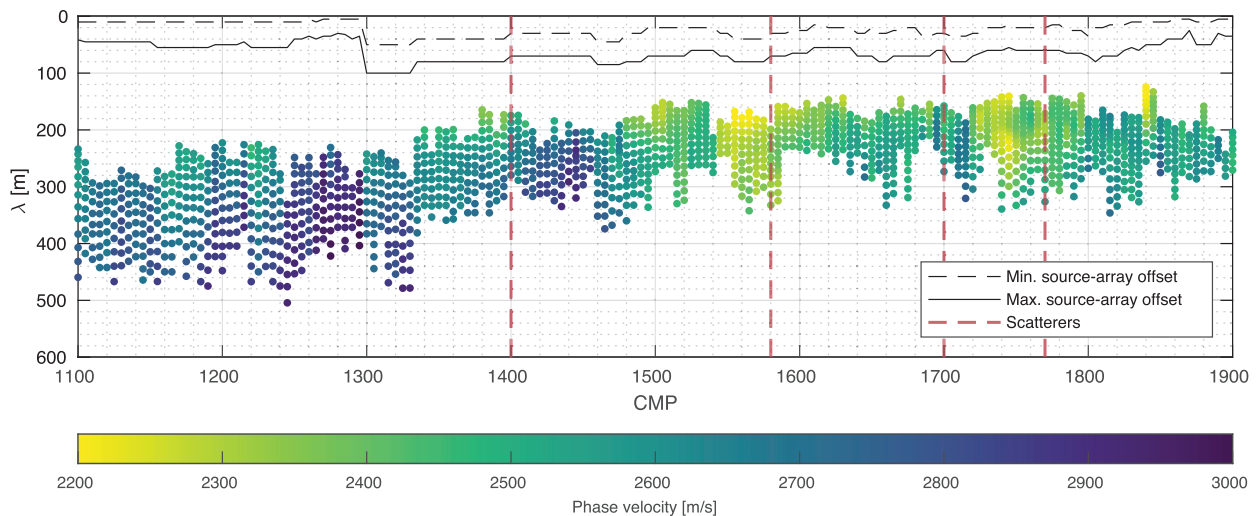
Figure 8. A pseudosection of dispersion curves extracted from ambient noise along the profile with phase velocity colour scaling. The vertical dashed lines present the position of the scatterers observed in the active data (Fig. 3). The black lines (dashed and solid) present the source-array offset and array length, scaled by 1/10 factor for a better display.
