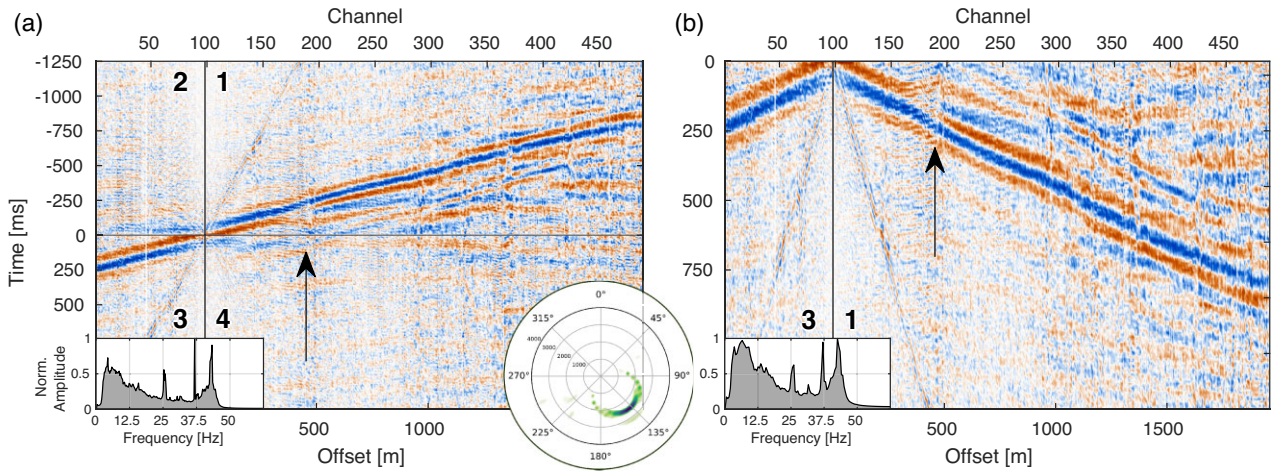
Figure 5. Cross-correlogram for a virtual source point 100, presenting a disruptive event around channel 200 (black arrow), and corresponding normalized amplitude spectra. Numbers mark quarters discussed in the main text. A radial plot in the centre presents a distribution of the back-azimuth of the most energetic sources (upper 60 per cent) in a frequency band of 12–14 Hz. (a) Cross-correlogram with both causal and acausal parts of the correlation. (b) A virtual shot gather constructed of causal and acausal parts of the cross-correlogram.
