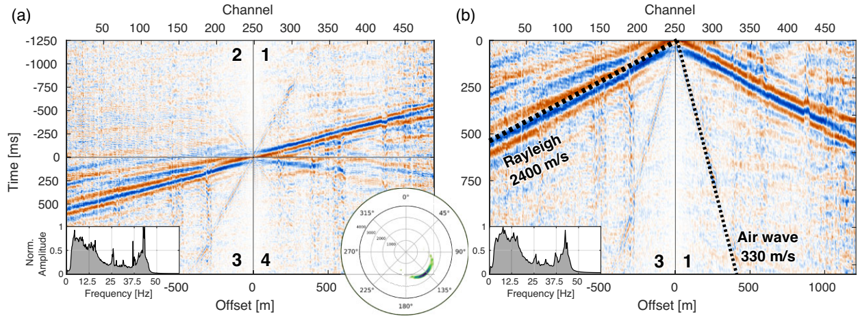
Figure 4. Cross-correlogram for a virtual shot point 251 (centre of the spread) and corresponding normalized amplitude spectra. Numbers mark quarters discussed in the main text. A radial plot in the centre presents a distribution of the back-azimuth of the most energetic sources (upper 60 per cent) in a frequency band of 12–14 Hz. (a) Cross-correlogram with both causal and acausal parts of the correlation. (b) A virtual shot gather constructed of causal and acausal parts of the cross-correlogram. The Rayleigh wave and airwave arrivals are marked with dotted lines.
