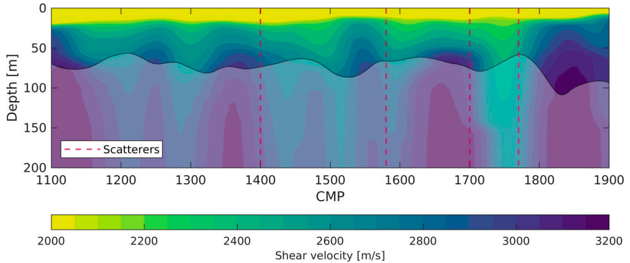
Figure 13. A smoothed active-data 2-D shear-wave velocity section constructed from 1-D models for every fifth CMP. The vertical dashed lines present the position of the scatterers observed in the active data (Fig. 3). The white-shaded area presents the maximum resolution limit according to the \lambda/2 criterion. Colour scale limits were clipped for a better comparison with other data sets.
