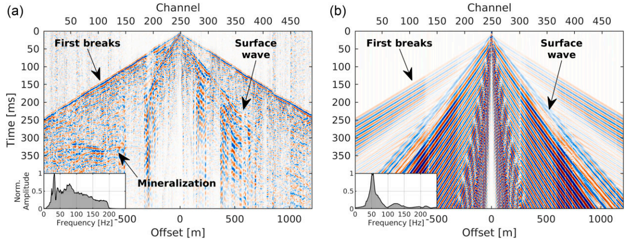
Figure 2. Shot gathers from the centre of the spread (shot point 250) and corresponding normalized amplitude spectra. (a) Active source shot gather with static corrections applied. (b) Synthetic shot gather generated with the velocity model from Table 1.
