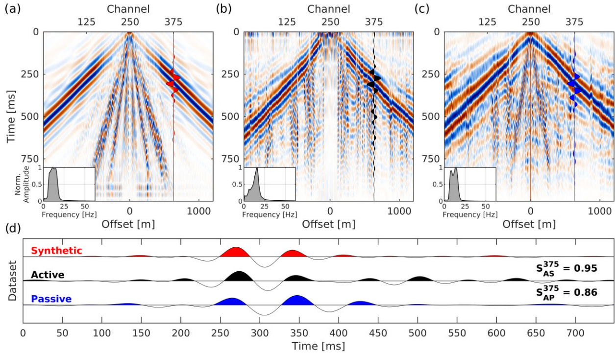
Figure 17. Comparison of the seismic signals in three data sets (shot position 1251). All gathers were bandpass filtered from 6 to 16 Hz. The coloured traces (channel 375) mark the trace used for semblance calculation. (a) Synthetic, generated based on the model in Table 1. (b) Active source data. (c) Passive-retrieved data. (d) Comparison of channels 375 of each gather with calculated semblance: S_{AS}^{375} presents semblance for active and synthetic traces, and S_{AP}^{375} for active and passive traces.
