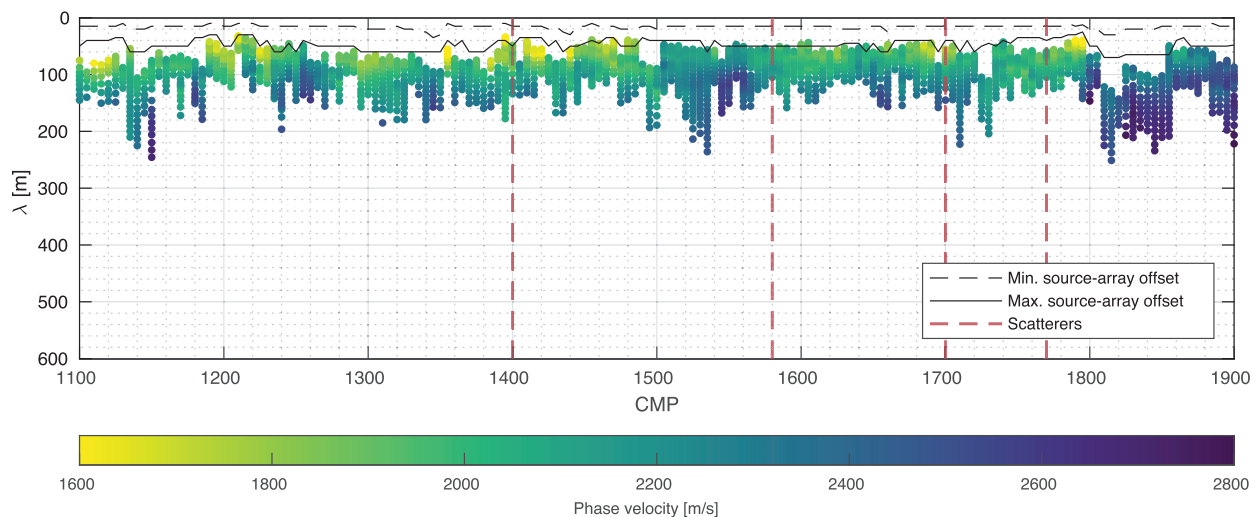
Figure 12. A pseudosection of active source dispersion curves extracted along the profile with phase velocity colour scaling. The vertical dashed lines present the position of the scatterers observed in the active data (Fig. 3). The black lines (dashed and solid) present the source-array offset and array length, scaled by 1/10 factor for a better display.
