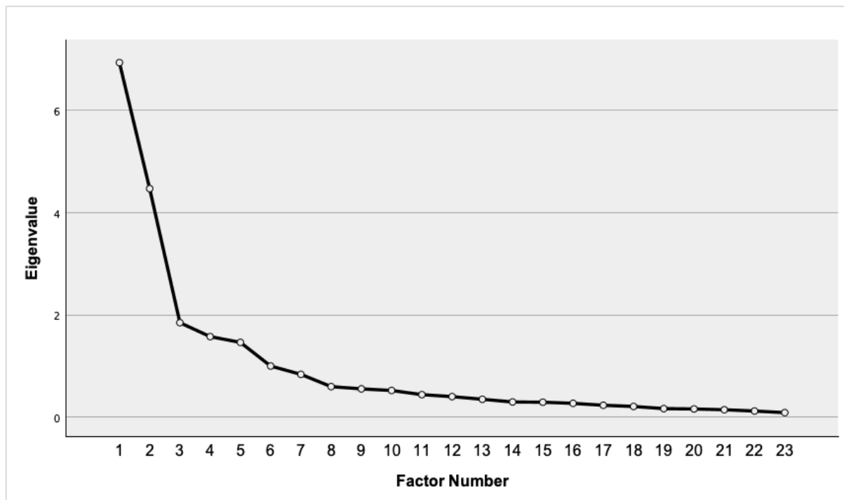
Figure 10: Scree plot
