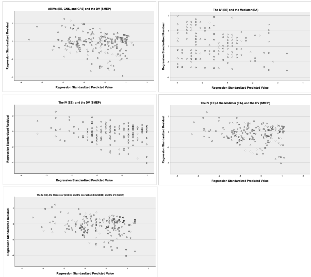
Figure 11: Scatterplot
