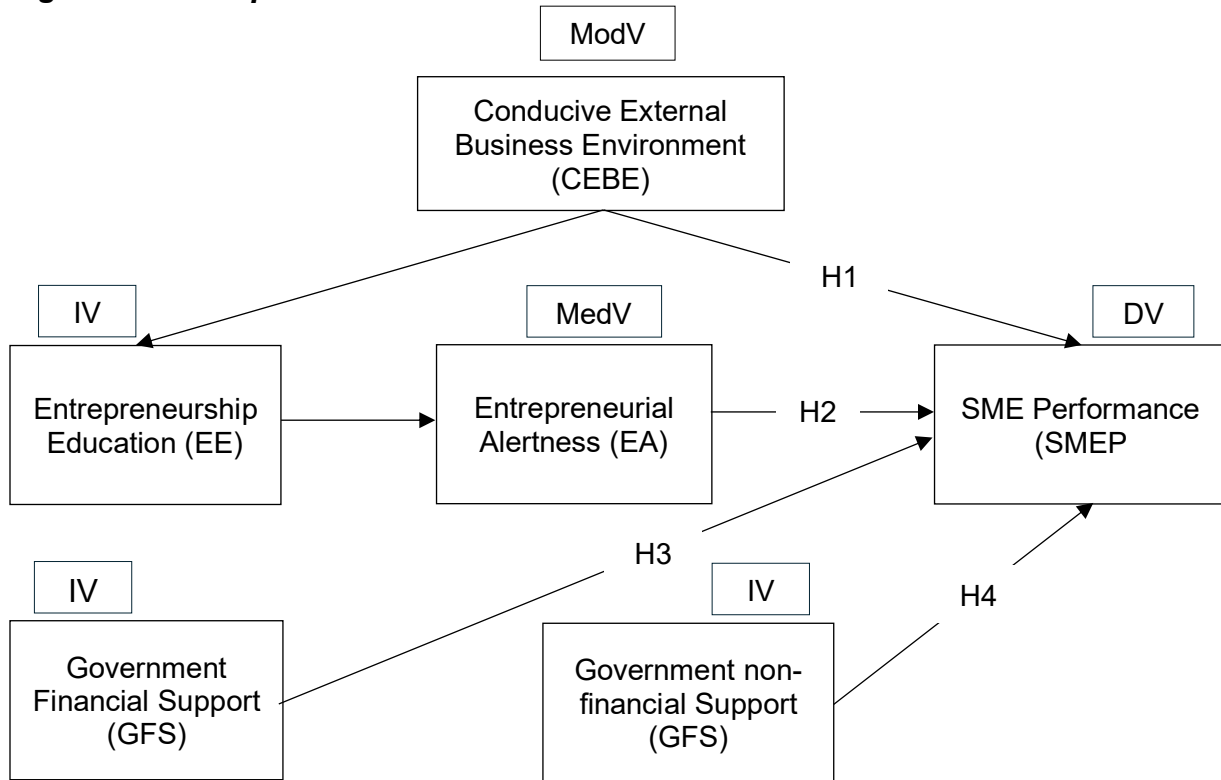
Figure 3: Conceptual framework
