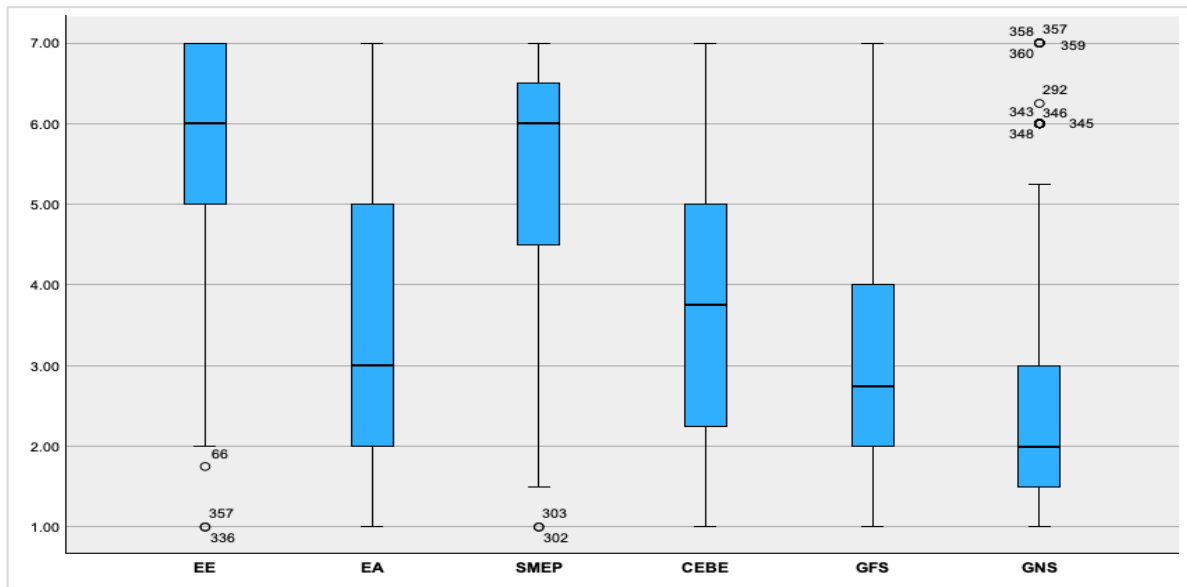
Figure 14: Boxplots
