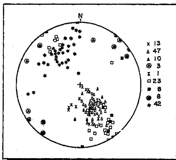
Fig. 4.24: Stereonet showing structural data from metasediments and amphibolites within the Matchless Amphibolite. See Table 4.3 for explanation of symbols; key gives number of measurements.
