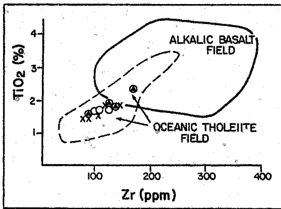
Fig. 5.9: Variation diagram \text{TiO}_2 versus Zr after Floyd and Winchester (1975). The majority of the Matchless metabasites plot within the oceanic tholeiite field. Symbols as for Figure 5.8.
