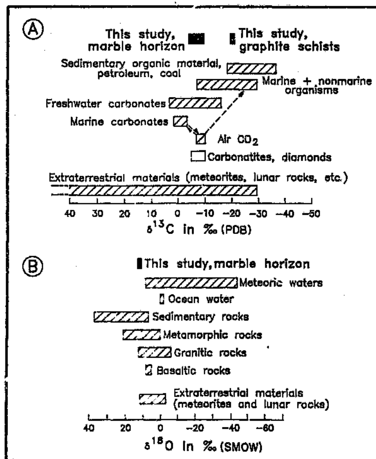
Fig. 3.10: Diagram comparing \delta^{13}\text{C} (A) and \delta^{18}\text{O} (B) data from graphite schists and marble in the Khomas Trough with carbon and oxygen isotope distributions of the lithosphere and hydrosphere (from Hoefs, 1980).
