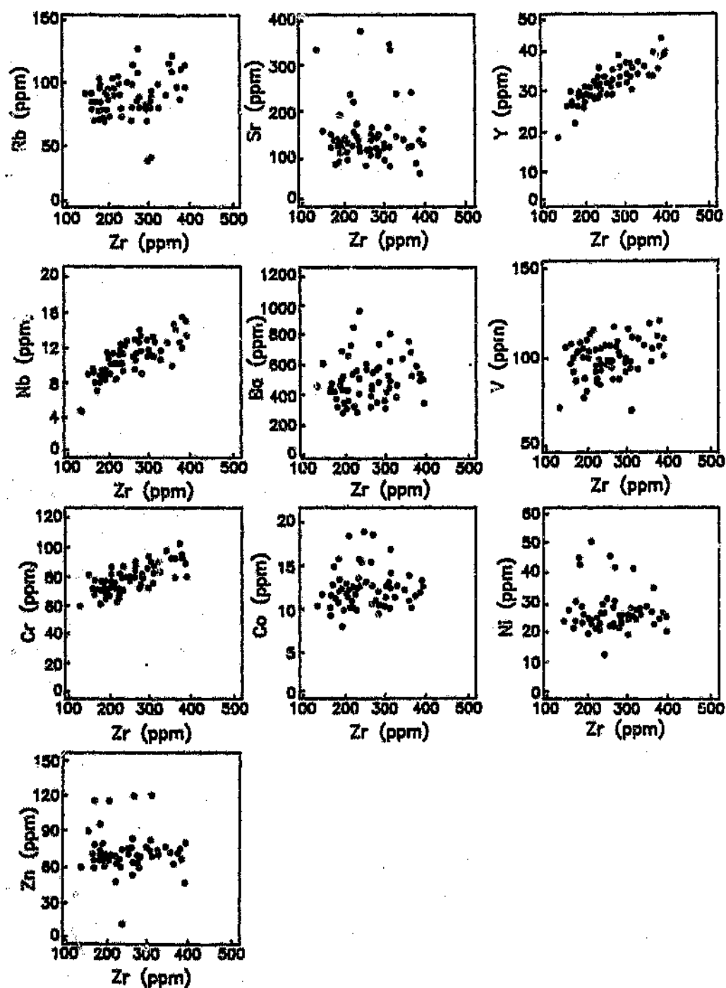
Fig. 3.1 (continued): (B) Geochemical variation diagrams showing minor elements of psammite analyses plotted against an immobile parameter Zr. Note the good correlations with Y, V, Nb and Cr.
