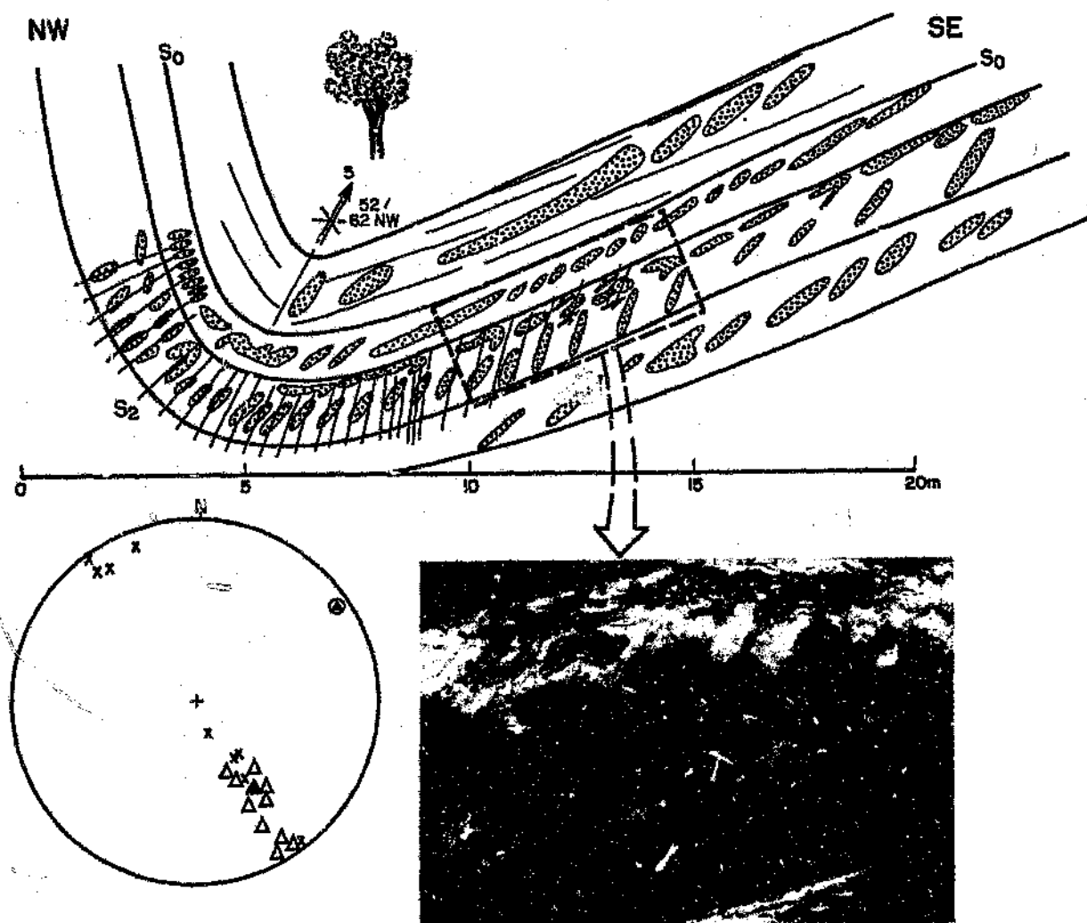
Fig. 4.14: Diagram showing sketch, photograph and stereoplot of an open asymmetric D_2 fold in the area between the graphite schist and the southern scapolite schist (Fig. 4.2). The orientation and shape of calc-silicate layers and spindles respective to S_0 and S_2 is strongly dependent on their positions within the fold. Shear processes parallel to S_0 are also indicated. See Table 4.3 for explanation of symbols. Farm Kaan 309.
