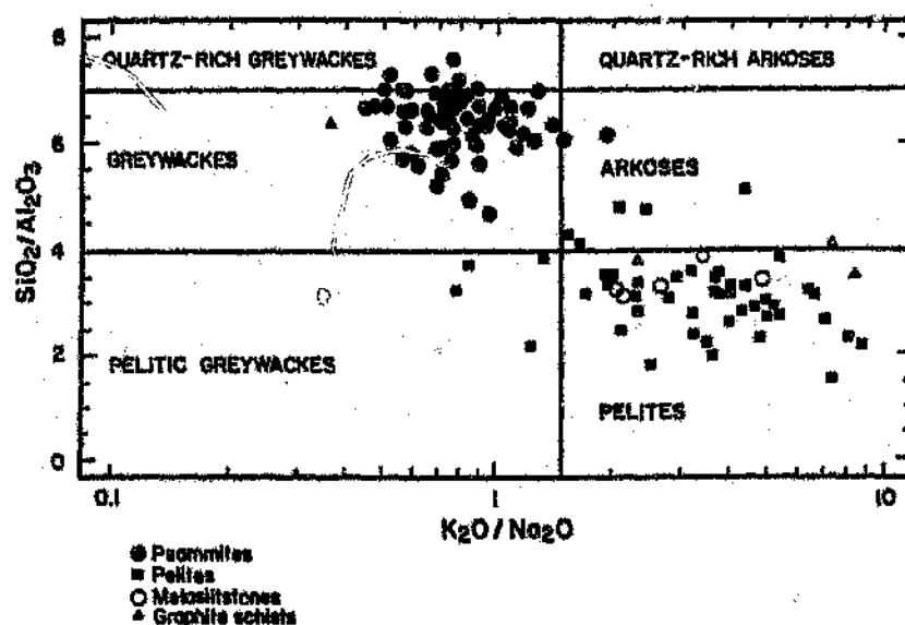
Fig. 3.2: Geochemical grid for discriminating clastic sedimentary protoliths after Wimmenauer (1984), with Kuiseb metagreywackes, pelites, metasiltstones and graphite schists plotted.
