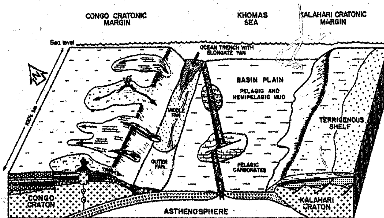
Fig. 3.19: Palaeoenvironmental model of the Khomas Trough. The elongate Khomas Fan is fed primarily from a mixed volcanic-plutonic active continental margin source which is situated to the north-east of the present Khomas Trough. Pelagic and hemipelagic sedimentation dominates the basin plain towards the south. Continental platform and slope sedimentation, partly in submarine fans, occurs on the Congo and Kalahari Cratons on either side of the Khomas Sea.
