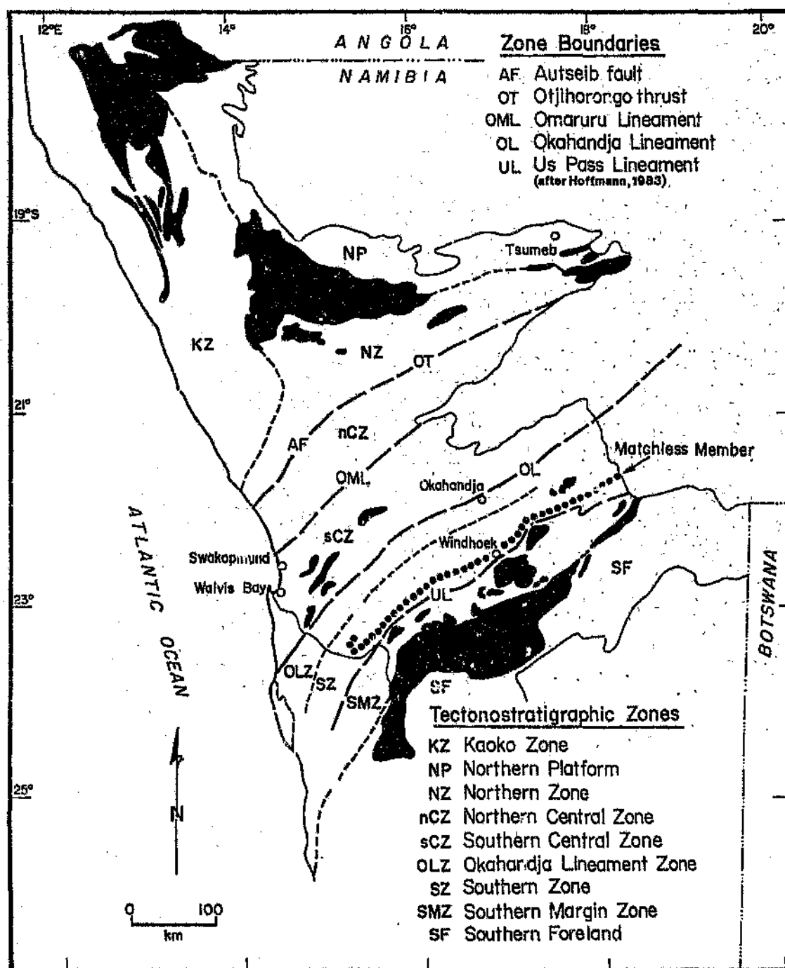
Fig. 2.2: Tectono-stratigraphic zones of the Damara Orogen (from Miller, 1983b).
