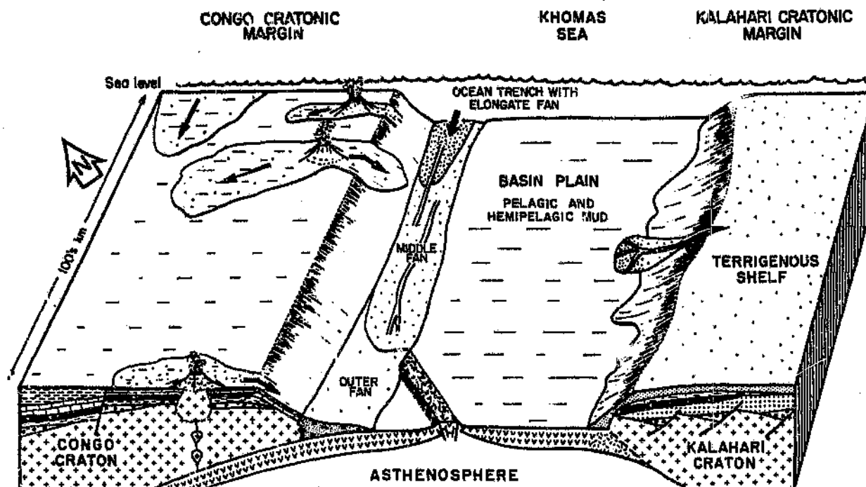
Fig. 7.3: Palaeoenvironmental setting during late continental convergence. High sediment input into the trench maintain shallow subduction and a narrow arc - trench gap. Terrigenous-clastic sedimentation occurs on both adjacent shelves at this stage.
