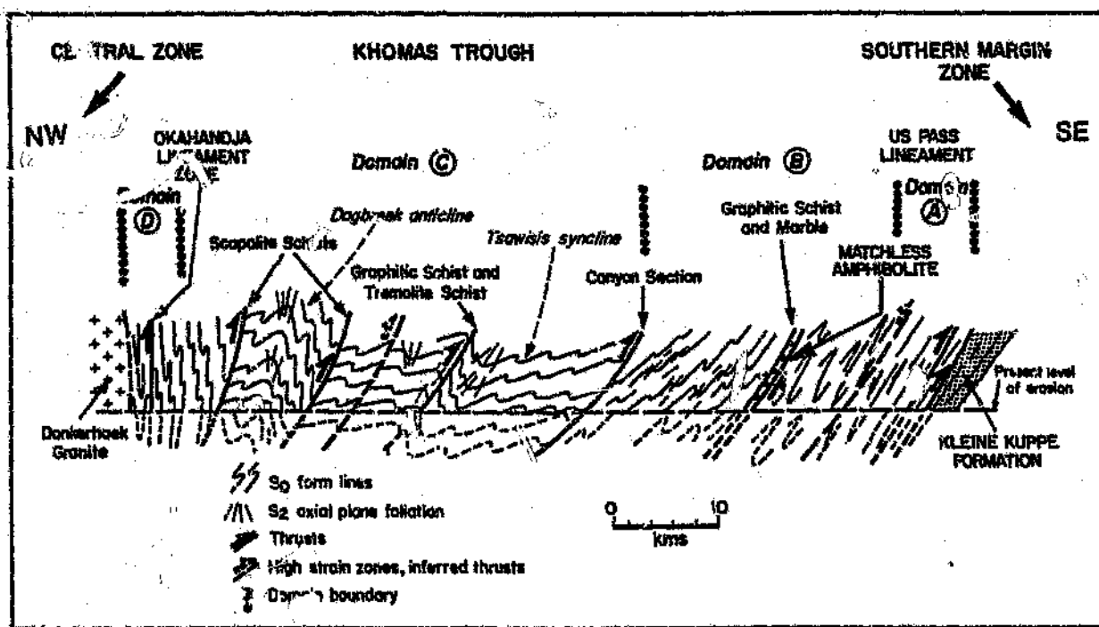
Fig. 4.2: Structural profile across the Khomas Trough showing the size and the style of major D_2 folds.
