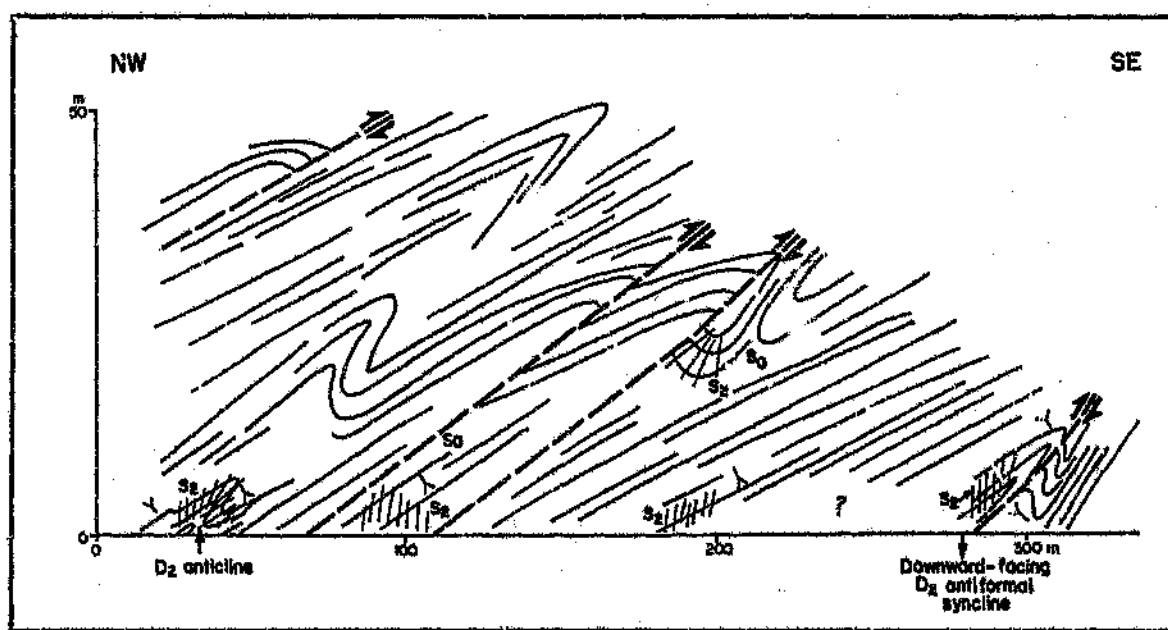
Fig. 4.11: Structural sketch illustrating the style of D_2 folding in the Koam canyon section. S_0 and S_2 form lines are indicated. Note sedimentary younging evidence. Farm Annelie 412.
