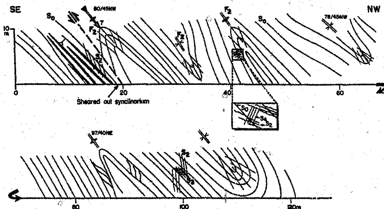
Fig. 4.20: Structural profile illustrating tight to isoclinal, moderately to steeply dipping D_2 folds with axial planar S_2 fabric. Superimposed are the S_3 and S_4 fabrics in this low-strain zone in the southern part of domain D. See Table 4.3 for explanation of symbols. Farm Keises 312.
