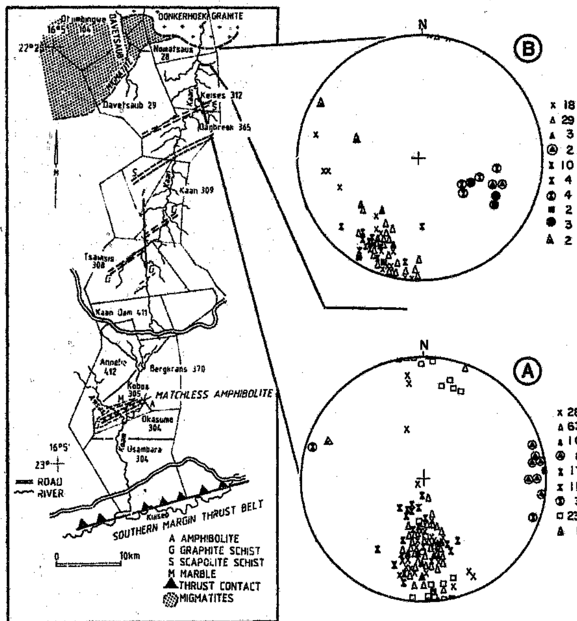
Fig. 4.18: Map of the study traverse showing a selection of structural data for the south (A) and the north (B) of domain D. See Table 4.3 for explanation of symbols; key gives number of measurements.
