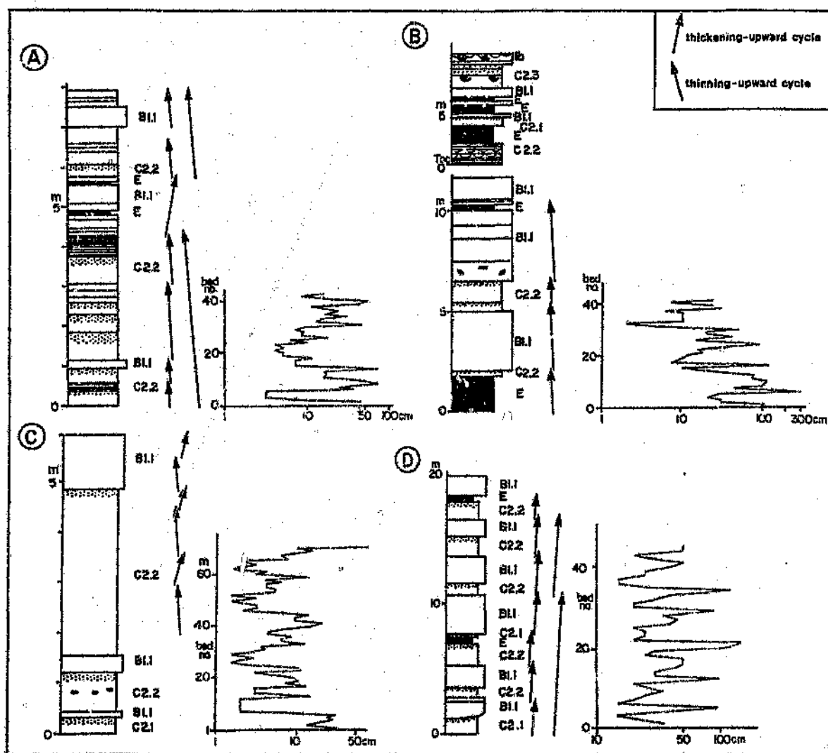
Fig. 3.13: Representative measured sections showing facies analysis, sedimentary cycles and bed thickness plots. Diagrams from A to H confirm the change from small-scale thinning-upward to thickening-upward cycles respectively from north to south. Positions of sections are indicated in Figure 3.12.
