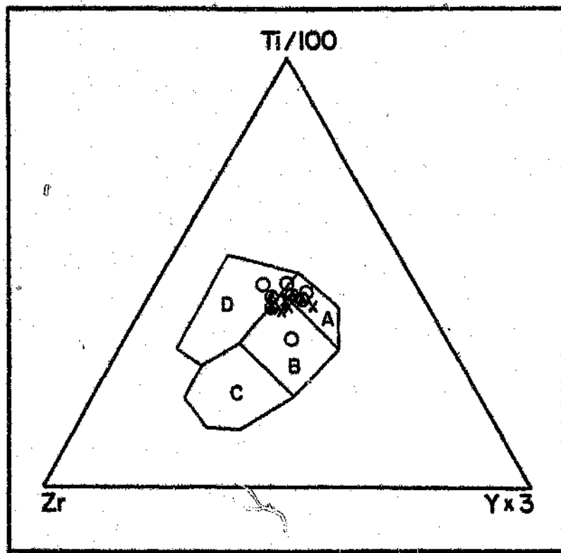
Fig. 5.11: Matchless Amphibolite samples plotted on the triangular variation diagram after Pearce and Cann (1973). Within-plate basalts plot in field D, ocean-floor basalts in field B, island-arc tholeiites in fields A and B and calc-alkali basalts in fields C and B. Symbols as for Figure 5.8.
