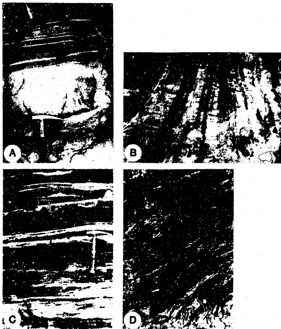
Fig. 3.14: Facies sequences. (A) Thick-bedded facies B turbidite underlying facies E turbidite, northern Khomas Trough, farm Keises 312. (B) Facies B, C and E turbidites in the northern Khomas Trough, farm Keises 312. (C) Facies B, C and E turbidites in the central Khomas Trough, farm Dagbreek 355. (D) Thin-bedded facies E turbidites below the Matchless Amphibolite in the southern Khomas Trough. Height of scale is 1.8 m. Farm Kobos 305.
