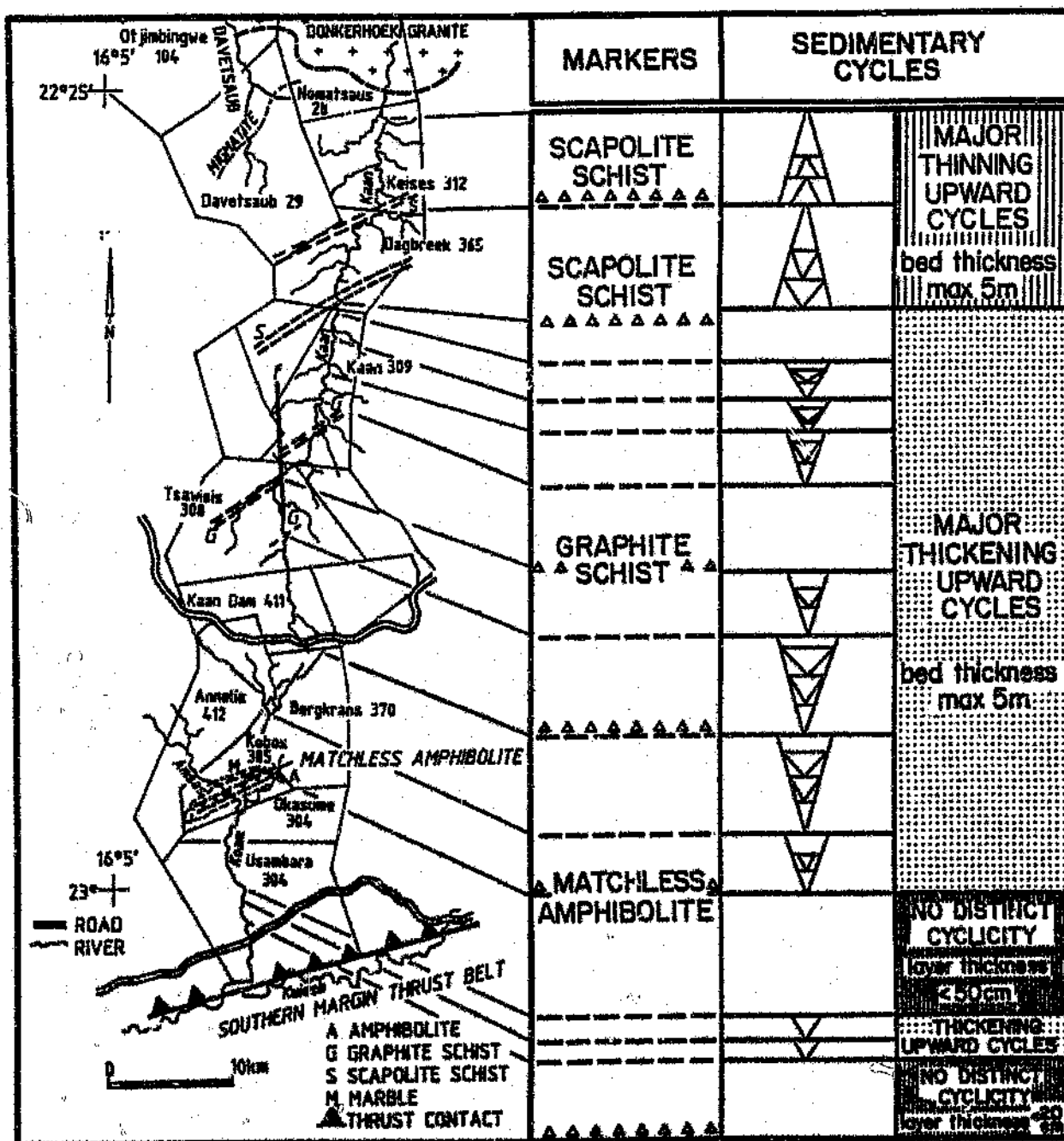
Fig. 3.15: Map of the study traverse showing the position of major sedimentary cycles and non-cyclic sequences in relation to marker units. Note the decrease of bed thicknesses from north to south.
