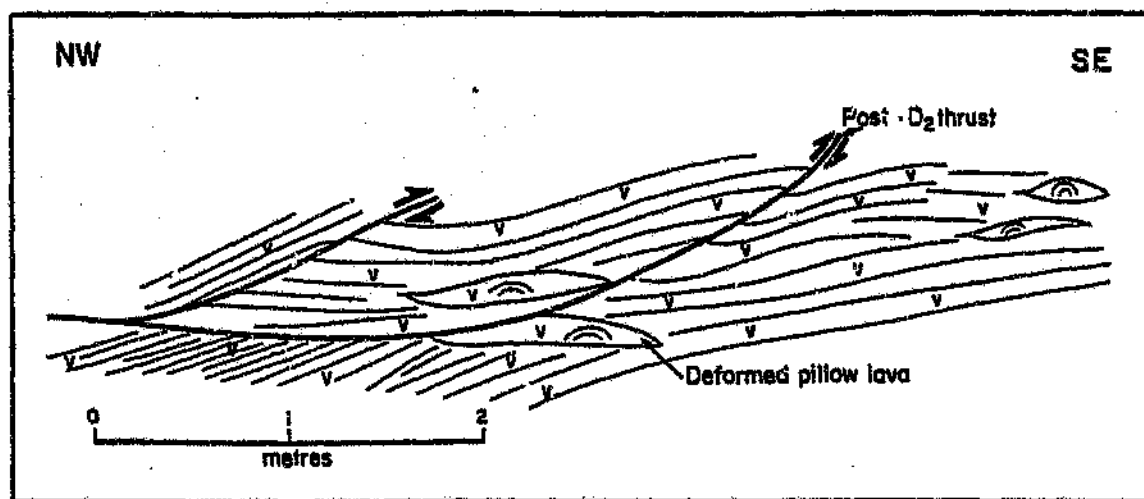
Fig. 5.7: Structural sketch showing post- D_2 thrusting within a pillow lava sequence on the farm Annelie (see Fig. 5.2,A). Note the sheared pillow structures. Form lines represent S_2 structural fabric. For symbols see Figure 5.2.
