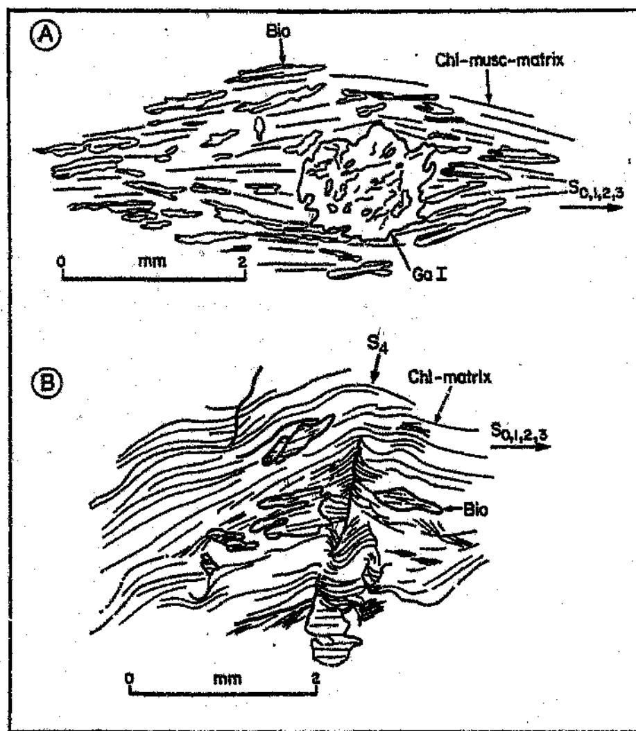
Fig. 4.4: Microtextures in domain A. Tracings from thin sections showing: (A) S_{0,1,2,3} composite cleavage illustrating the parallel to subparallel alignment of biotite within a chlorite-muscovite matrix enclosing garnet I (specimen PK 855, farm Usambara 304, south of Us Pass road); (B) Chlorite-biotite schist showing S_4 crenulation cleavage developed within the S_{0,1,2,3} composite cleavage. Note microfaults at hinge lines (specimen PK 140, farm Usambara 304, south of Us Pass road).
