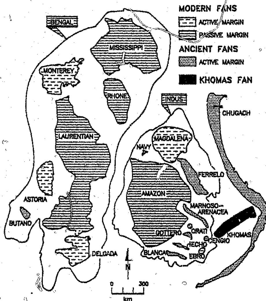
Fig. 3.20: Comparison of the size and shape of the present day outcrop of the Khomas Fan with other ancient and modern fan systems (modified from Barnes and Normark, 1983/84).
