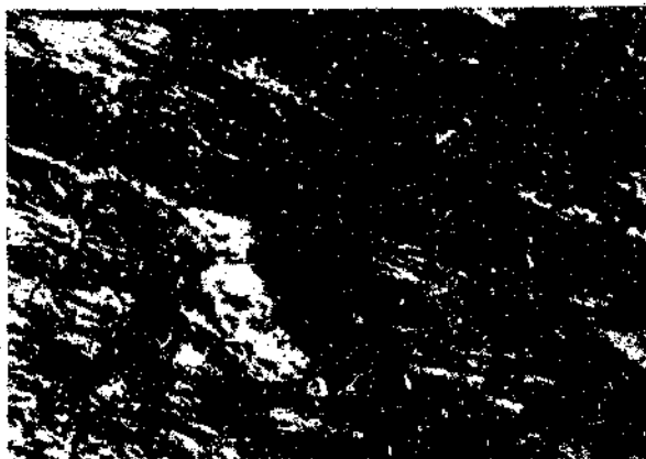
Fig. 4.5: Small-scale ( D_5 ) kink band in domain A, showing quartz-filled dilation space parallel to the S_{0,1,2,3} composite cleavage. Lens cap for scale is circled. Farm Usambara 304, south of Us Pass road.
