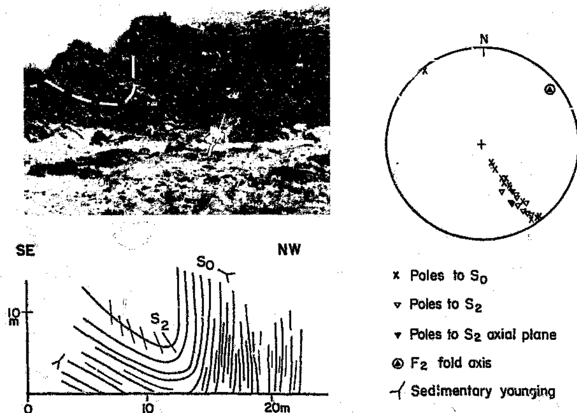
Fig. 4.15: Diagram showing sketch, photograph and stereoplot of an open asymmetric D_2 fold in the area between the graphite schist and the southern scapolite schist (Fig. 4.2). Younging evidence is based on sedimentary structures. Bedding is demarcated by dashed line. Height of scale (circled) is 1.7 m. Farm Kaan 309.
