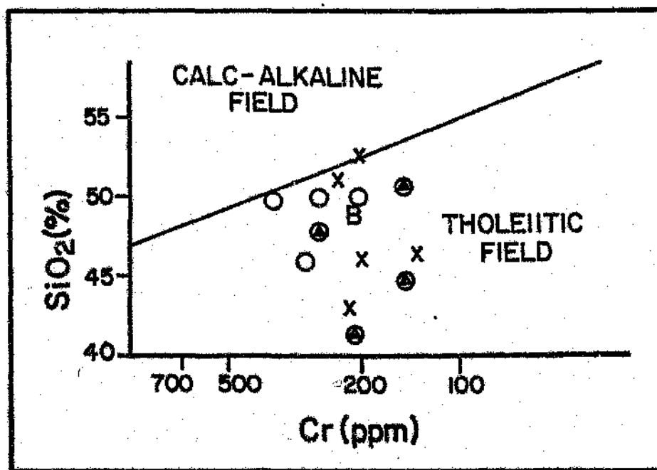
Fig. 5.10: Matchless Amphibolite samples plotted on the variation diagram \text{SiO}_2 versus Cr after Miyashiro and Shido (1975). This shows the tholeiitic character of the Matchless metabasic rock types. Symbols as for Figure 5.8.
