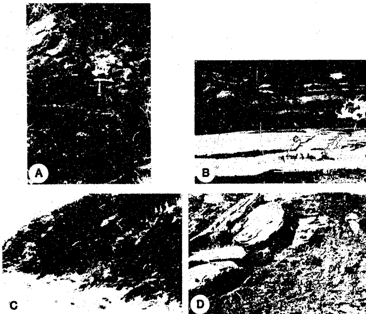
Fig. 3.9: Turbidite and pelagic facies (facies terminology after Pickering et al., 1986). (A) Very thick-bedded (>10 m) facies E pelites. Farm Keises 312. (B) Calc-silicate layer and spindles (facies class 5) in thick-bedded facies B turbidite above facies C turbidite. Farm Dagbreek 365. (C) Very thick-bedded pelagic graphite schist facies (facies class 6). Height of outcrop is about 10 m. Farm Kaan 309. (D) Dolomitic marble facies (facies class 7) on top of a graphite schist in the hangingwall of the Matchless Amphibolite (stratigraphic top towards the left). Hammer for scale. Farm Annelie 412.
