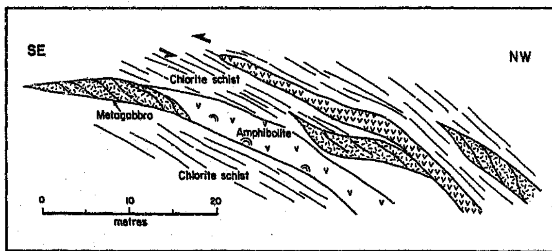
Fig. 5.6: Sketch showing the structural interposition of sheared metagabbro bodies with type I and type II amphibolites and with chlorite schists. Note sigmoidal internal shear fabric of the metagabbros. The location and symbols are shown in Figure 5.2,B.
