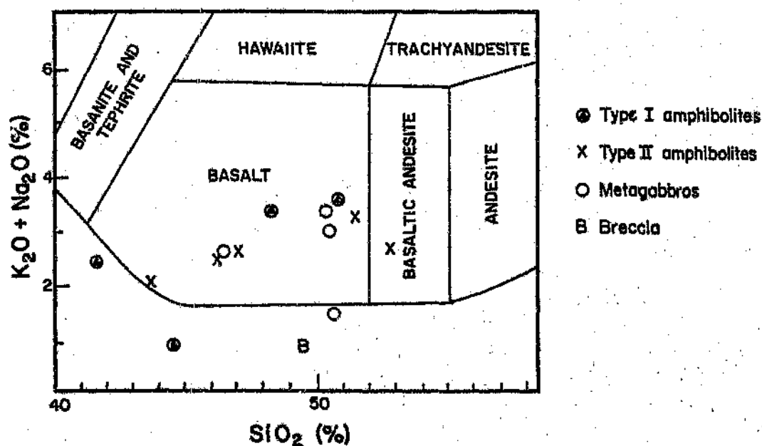
Fig. 5.8: Variation diagram K_2O + Na_2O versus SiO_2 after Cox et al. (1979) classifying amphibolites and metagabbros of the Matchless sequence as basalts.
