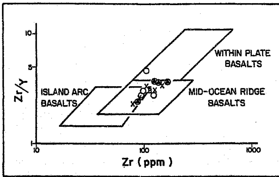
Fig. 5.12: Variation diagram Zr/Y versus Zr after Pearce and Norry (1979) showing the mid-ocean ridge basalt (MORB) affinity of the Matchless metabasites. Symbols as for Figure 5.8.
