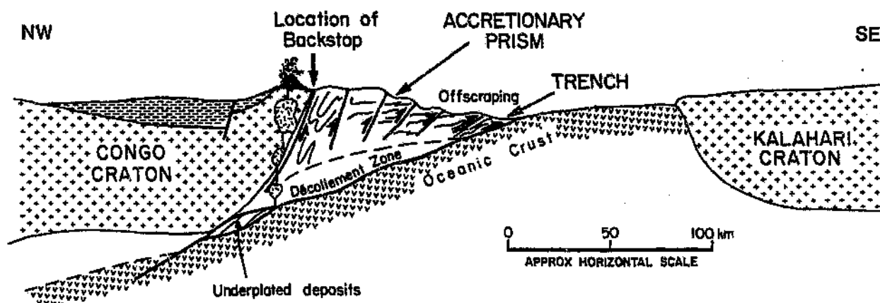
Fig. 7.2: Tectonic setting of the southern Damara Orogen during late convergence of the Congo and Kalahari Cratons. The oceanic trench contains the elongate submarine fan and the accretionary prism evolves through the offscraping of sediment from the descending slab. Early ( D_1 ) folding and thrusting occurs within the prism.
