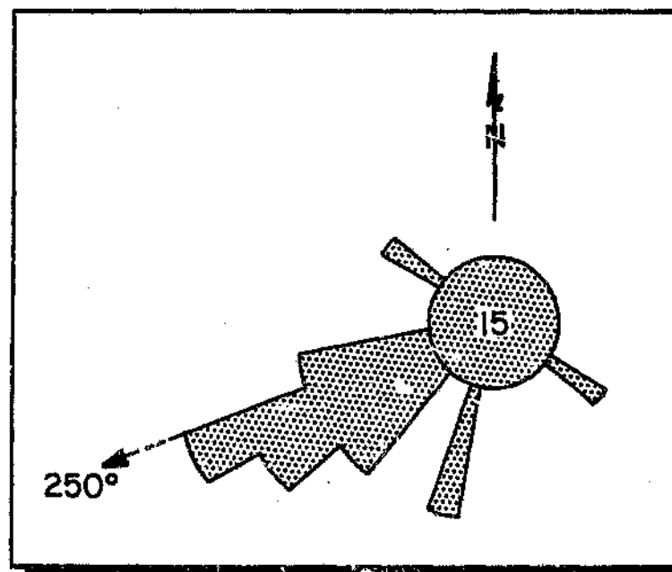
Fig. 3.6: Palaeocurrent data from various measured sections throughout the Khomas Trough. Palaeocurrent directions determined from sets of cross-laminae and flute casts.
