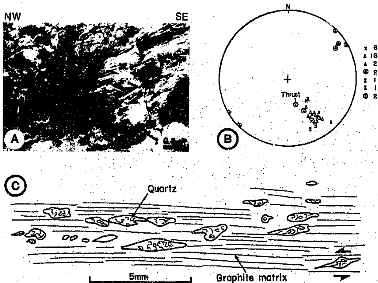
Fig. 4.28: Diagram showing photograph, sketch and stereonet of geological features at the graphite schist in the centre of the Khomas Trough. Kaan river, farm Kaan 309. (A) Photograph showing pre-D 3 thrust fault and sheared-out synform at the base of the graphite schist. Thrust zone is brecciated and iron-stained. (B) Stereonet data for the graphite schist sequence. See Table 4.3 for explanation of symbols. (C) Tracing from thin section showing elongated and sheared quartz in highly sheared graphitic matrix.
