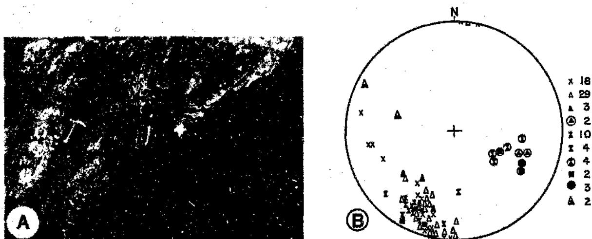
Fig. 4.31: (A) Photograph of parallel-sided D_3 shear zone containing F_3 folds and a pervasive S_3 spaced cleavage. S_0 and S_2 are intensely folded. Note parallelism of S_0 , S_2 and S_3 on either side of the shear zone. Northern margin of the farm Keises 312. (B) Stereonet showing structural data for the northern part of domain D (see Fig. 4.18). Note wide spread of data, clockwise rotation of structural elements compared with domains A-C, and plunging fold axes. See Table 4.3 for explanation of symbols; key gives number of measurements.
