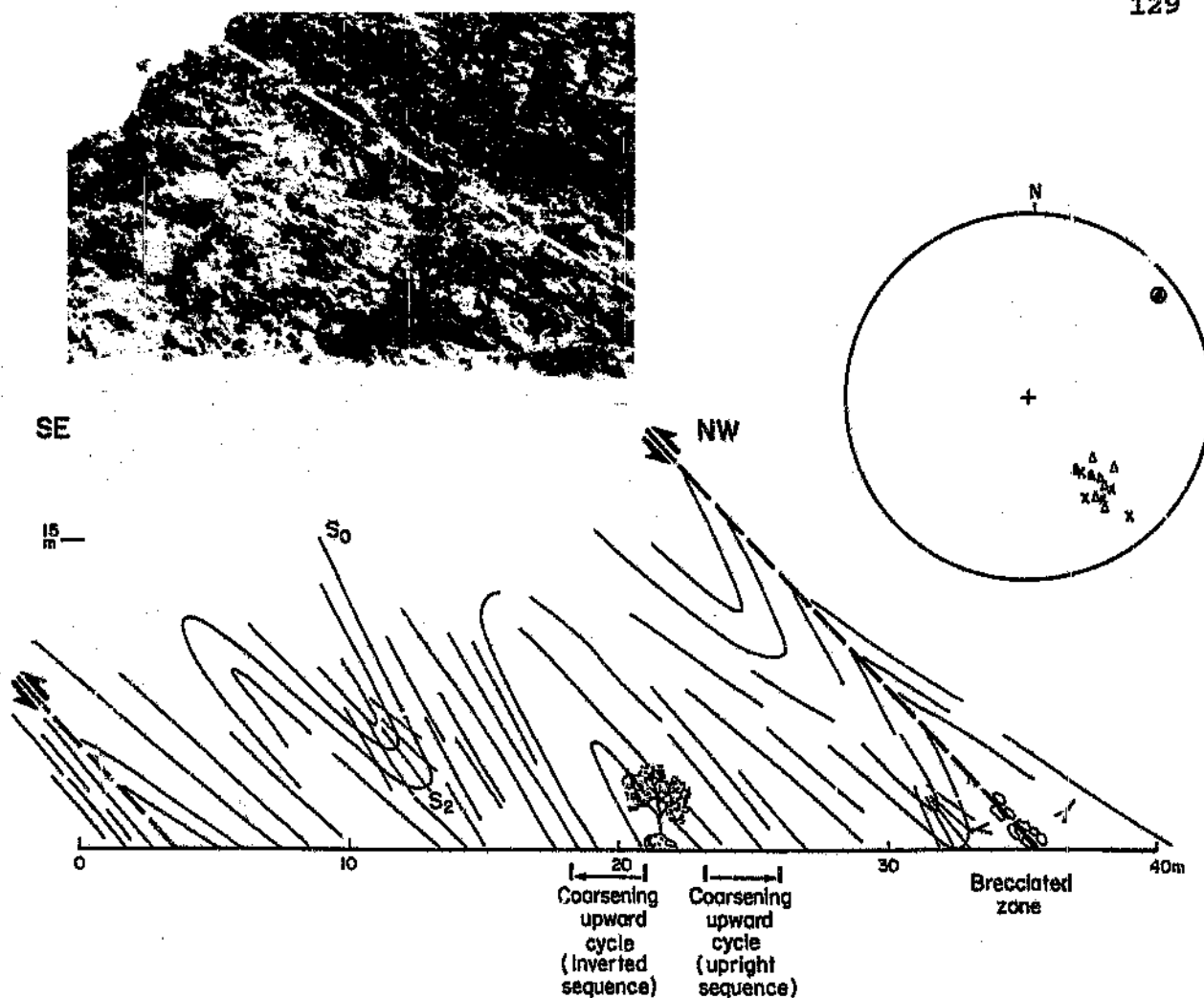
Fig. 4.16: Diagram showing sketch, photograph and stereoplot of tight to isoclinal SE verging D_2 folds on the northern, upright to overturned limb of the Tsawisis syncline (Fig. 4.2). In order to compare sketch and photograph reference may be made to the thrust indicated. Note also sedimentary younging evidence. See Table 4.3 for explanation of symbols. Height of scale (circled) is 1.8 m. Farm Tsawisis 308.
