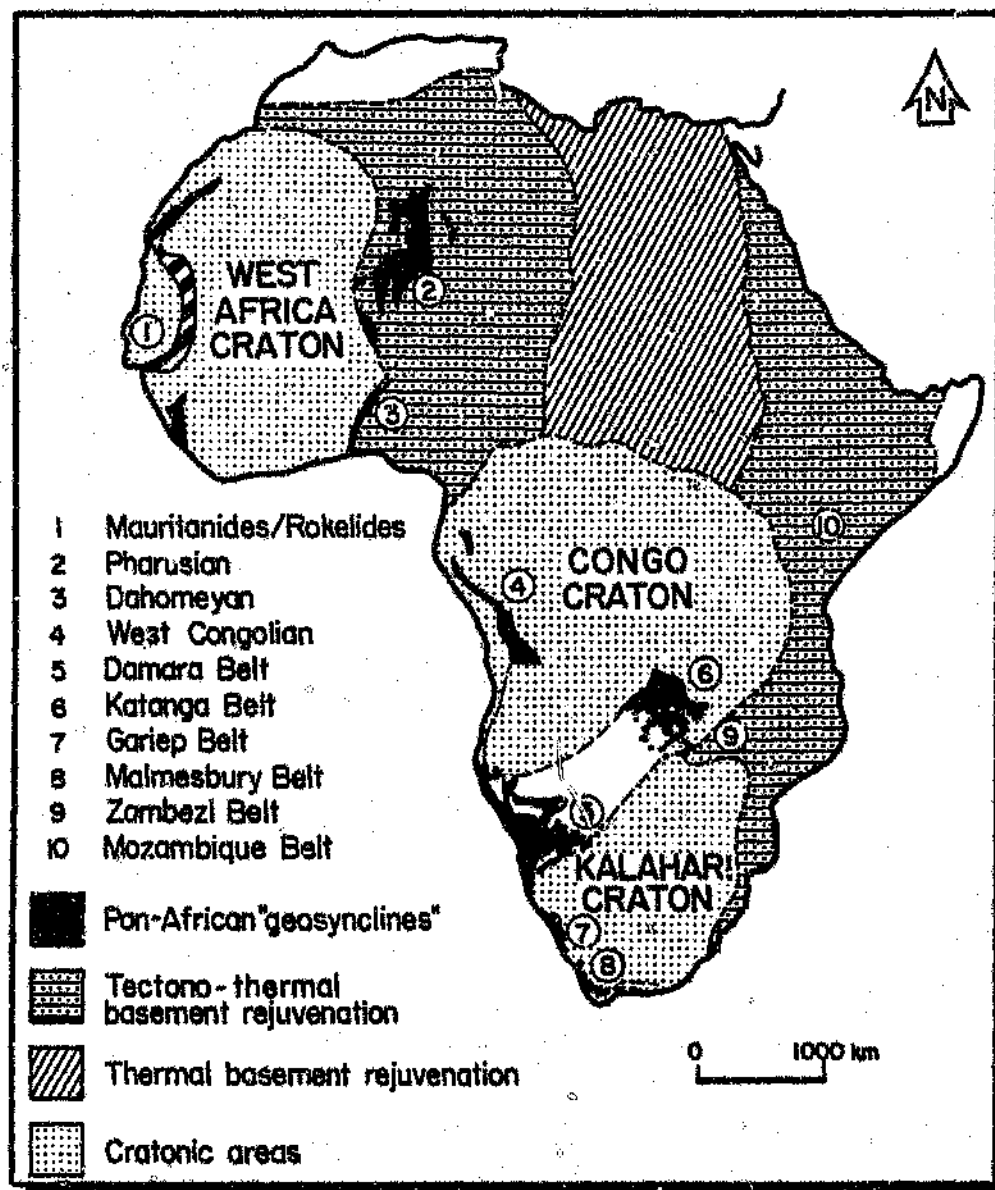
Fig. 2.1: Pan-African orogenic belts and terranes of basement rejuvenation (modified from Porada, 1983).
