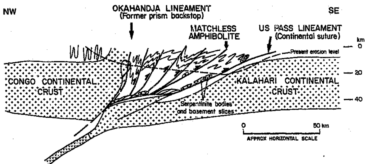
Fig. 7.4: Collision between the Congo and Kalahari Cratons. This was accompanied by strong south-east vergent folding and thrusting, late-tectonic metamorphism, and emplacement of the accretionary prism including the Matchless Amphibolite onto the Kalahari Cratonic Foreland. The post-tectonic Donkerhoek Granite intruded partially along the Okahandja Lineament.
