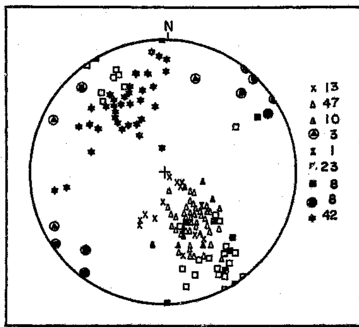
Fig. 5.3: Stereonet showing structural data from amphibolites and metasediments of the Matchless Amphibolite. Note sub-horizontal to plunging attitude of fold axes. (Symbols: X, poles to S_0 ; \Delta , poles to S_2 ; \blacktriangle , poles to D_2 axial plane; \times , poles to S_3 ; \square , poles to S_4 ; \blacksquare , poles to D_4 axial plane; \odot , F_2 fold axis; \otimes , F_4 fold axis; * , L_{2A} lineation; for further details see Chapter 4.4.2).
