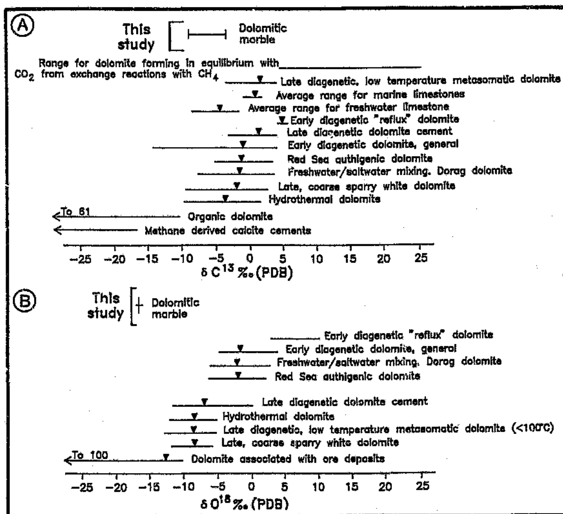
Fig. 3.11: Diagram comparing \delta^{13}\text{C} (A) and \delta^{18}\text{O} (B) data from the dolomitic marble at the Matchless Amphibolite with other species of dolomite (from Mattes and Mountjoy, 1980).
