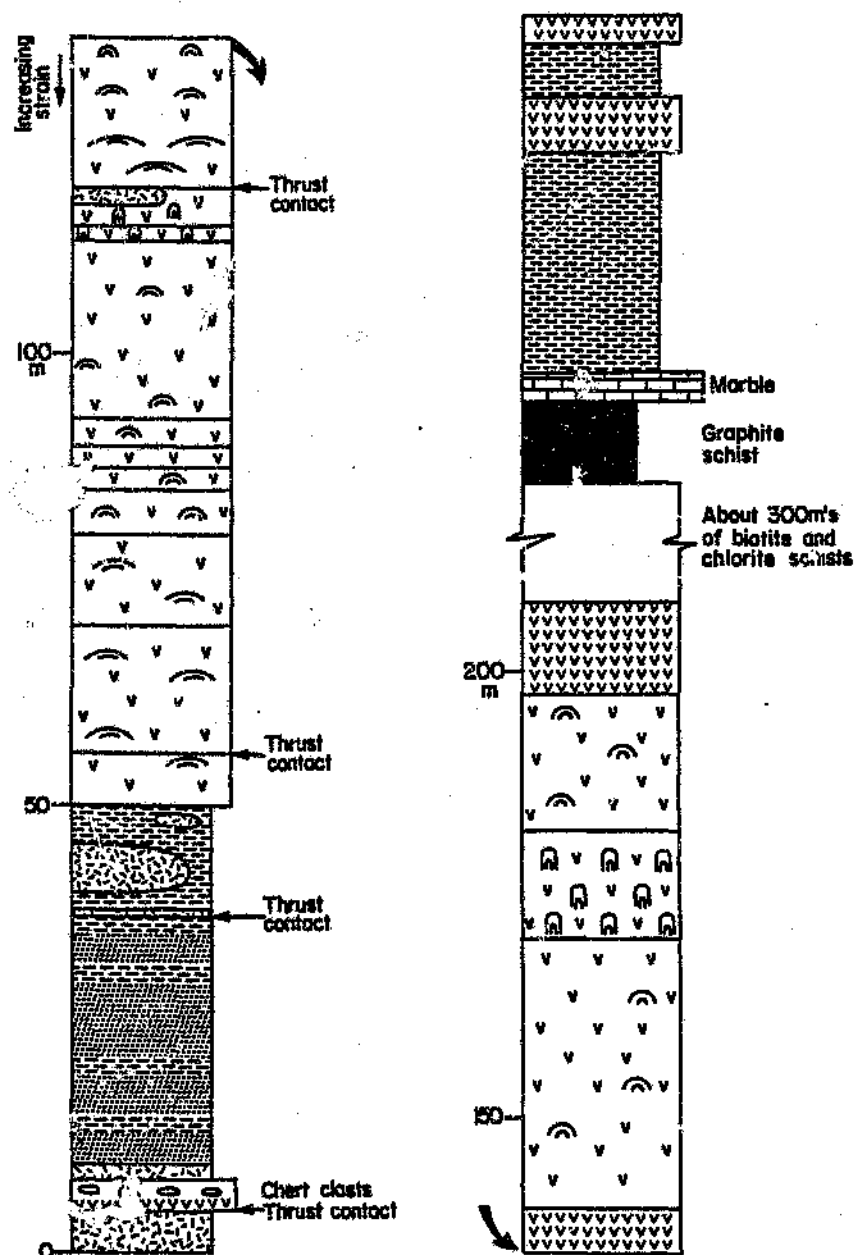
Fig. 5.4: Detailed measured section (profile A in Fig. 5.2) showing the interposition of amphibolites, metagabbros and metasediments. Major thrust contacts are indicated and the spheroidal to elongate shape of pillows lavas (distinguishable by the degree of curvature of the pillow symbol in the figure, e.g. in the top part of the left column) is regarded as a measure of the imposed strain (for symbols see Fig. 5.2).
