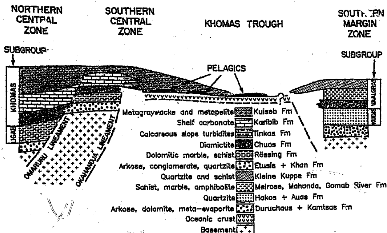
Fig. 2.3: Rock relationships of the Khomas Trough and adjacent areas in the Damara Orogen. Stratigraphic contacts are emphasised in their palinspastic context. Correlations and terminology of the Southern Margin Zone and the southern and northern Central Zone are after Hoffmann (1983), Henry et al. (1990) and Badenhorst (1987) respectively.
