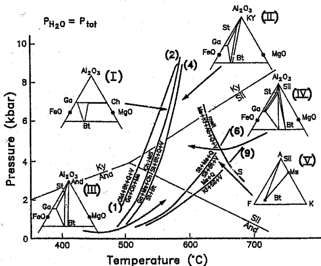
Fig. 6.3: P-T diagram showing the stability fields and assemblages for the assemblage zones 1 to 4. Upper stability limits of chloritoid + biotite + quartz + H_2O (1) after Spear and Cheney (1989); of chlorite + muscovite (2) after Hoschek (1969); of garnet + muscovite + chlorite (4) after Thompson (1976); of staurolite + muscovite + quartz (6) after Hoschek (1969); and of muscovite + quartz (9) after Chatterjee and Johannes (1974). The melting curve (S) is based on experimental data from the Khomas Trough after Hoffmann (1976) and Winkler (1983). Stability field of Al-silicates after Holdaway (1971).
