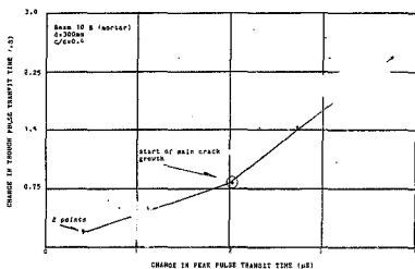
FIG 5.2S (a) & (b) Plots of cumulative change in trough pulse transit time v. cumulative change in peak pulse transit time for beams 9B & 10B
