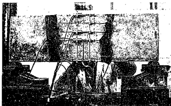
FIG 3.2 View of a fracture beam resting on its support rollers. Note the centrally cut notch and the surface and ultrasonic instrumentation (described elsewhere in the text).
