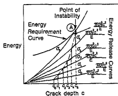
FIG 2.4 Crack propagating in a non-homogeneous brittle material under monotonically increasing stress (from ref 4).
