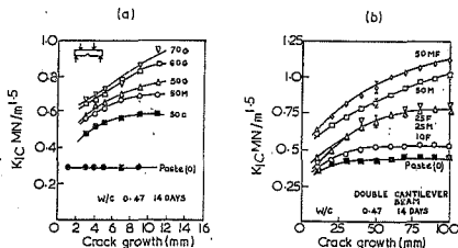
Variation of fracture toughness with crack growth of cement paste, mortar and concrete, (a) Notched beam, 4-point bending test. (b) Double cantilever beam test. Aggregate sizes: F = fine (52-100 mesh), M = medium (14-25 mesh), MP = mixture of equal proportions of M and F, C = coarse (10-5mm) and G = graded (10-100 mesh)
