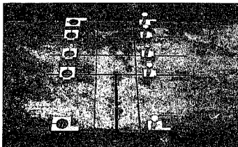
FIG 3.7 View of the LVDT clamps and blocks prior to gluing to the beam. Note the casing clamps on the left and the core support blocks with their adjustable screws on the right.
