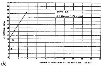
FIG C.2 Plots of the J - integral versus surface displacement at the notch tip for the mortar beams, and linear regression according to the ASTM-B13 method.
