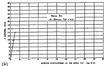
FIG C.1 Plots of the J - integral versus surface displacement at the notch tip for the concrete beams, and linear regression according to the ASTM-813 method.
