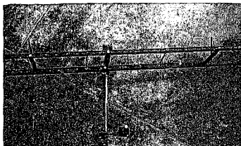
FIG 3.5 View of the deflection measuring rig. Note the supports at either ends and the arm for positioning the midspan deflection LVDT.
