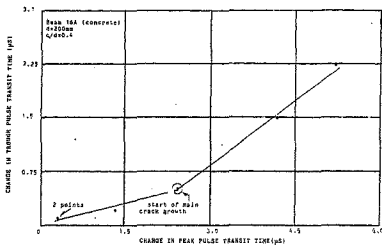
FIG 5.20 (a)&(b) Plots of cumulative change in trough pulse transit time vs cumulative change in peak pulse transit time for beams 15A & 16A
