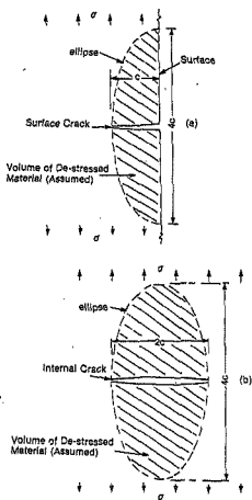
FIG 2.1 Griffith case for (a) surface crack and (b) internal crack (from ref 4)
