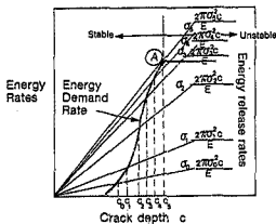
FIG 2.5 Energy rate curve corresponding to FIG 2.4 (from ref 4).
