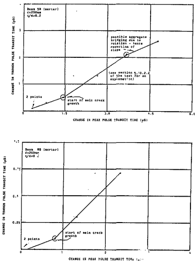
FIG 5.24 (a)&(b) Plots of cumulative change in trough pulse transit time vs cumulative change in peak pulse transit time for beams SB & 8B
