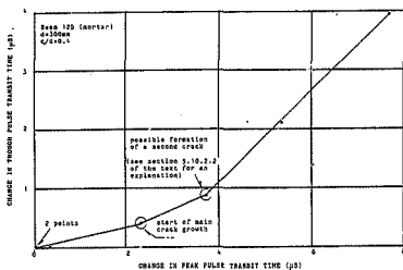
FIG 5.26 (a) & (b) Plots of cumulative change in trough pulse transit time vs cumulative change in peak pulse transit time for beams 11B & 12B
