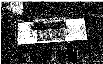
FIG 3.10 View of the rollers greased and ready to be placed between the half-round beam support and the machined steel plate.
