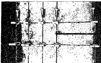
FIG 3.8 View of the LVDT clamps and blocks glued in position on a beam. Note the adjustable screws for the cores lying next to the blocks. (Note: Photograph rotated through 90°).
