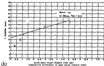
FIG C.3 Plots of the J - integral versus the cumulative difference in peak ultrasonic pulse transit time for the concrete beams, and linear regression according to the ASTM-613 method.
