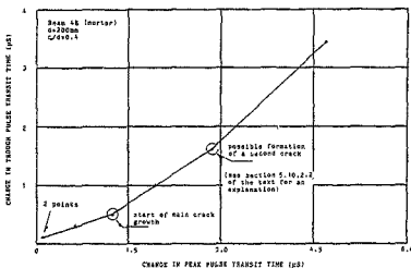
FIG 5.23 (a)&(b) Plots of cumulative change in trough pulse transit time vs cumulative change in peak pulse transit time for beams 3B & 4B
