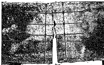
FIG 3.3 View of a cracked fracture beam after testing.
