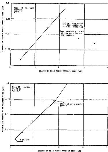
FIG 5.22 (a) & (b) Plots of cumulative change in trough pulse transit time vs cumulative change in peak pulse transit time for beams 1B & 2B
