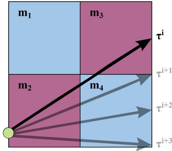
Figure 2.2: Principle of discretisation in seismic tomography. A raypath passes through cells m_2 , m_3 and m_4 . The traveltime ( \tau^i ) is a sum of all model cell properties and the raypath segment distances of x_2 , x_3 and x_4 (modified from Vesnaver and Böhm, 2000).
