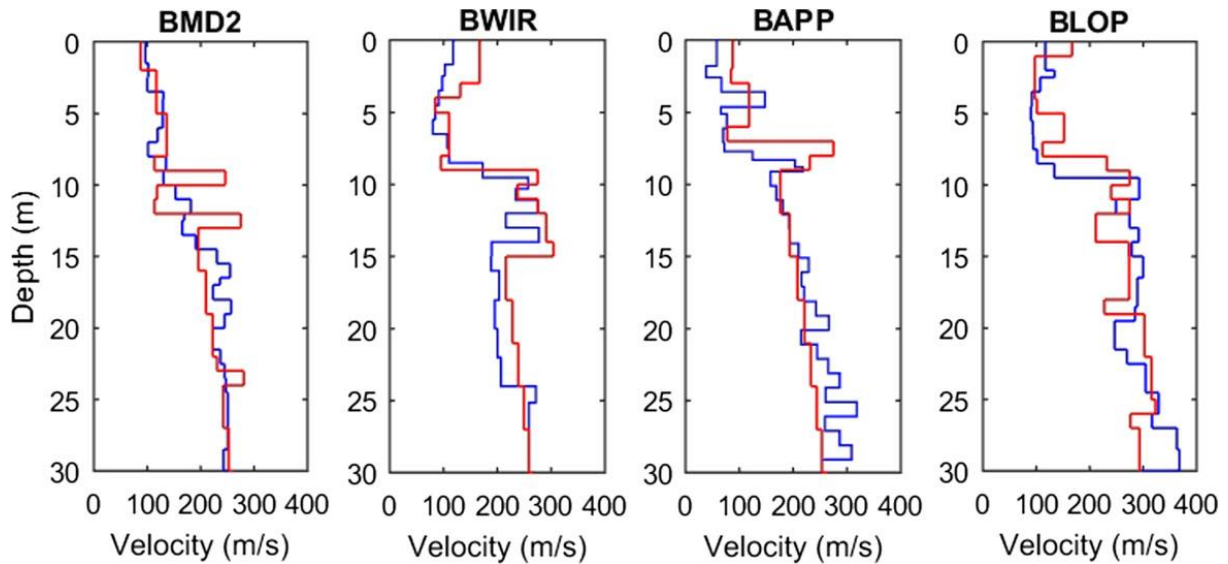
Figure 4.15: V_s profiles at selected B stations. Measured V_s in blue and modelled mean V_s (Kruiver et al., 2017a) in red.
