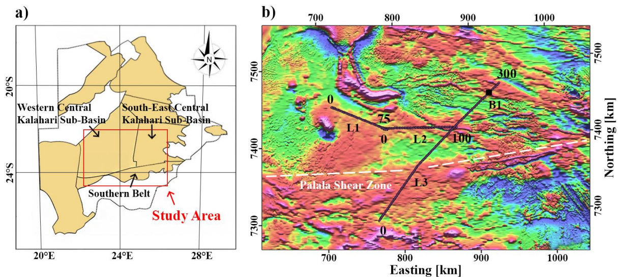
Figure 7.1: The distribution of the Kalahari Karoo Basin in Botswana (a) is shown in light yellow (modified from Smith, 1984). The location of the seismic lines (L1, L2, L3) and borehole B1 are superimposed on the regional total intensity magnetic map (b), Courtesy of the Council for Geosciences of South Africa. The distances along the lines are indicated in kilometres, e.g. line L1 ends at 75 km.
