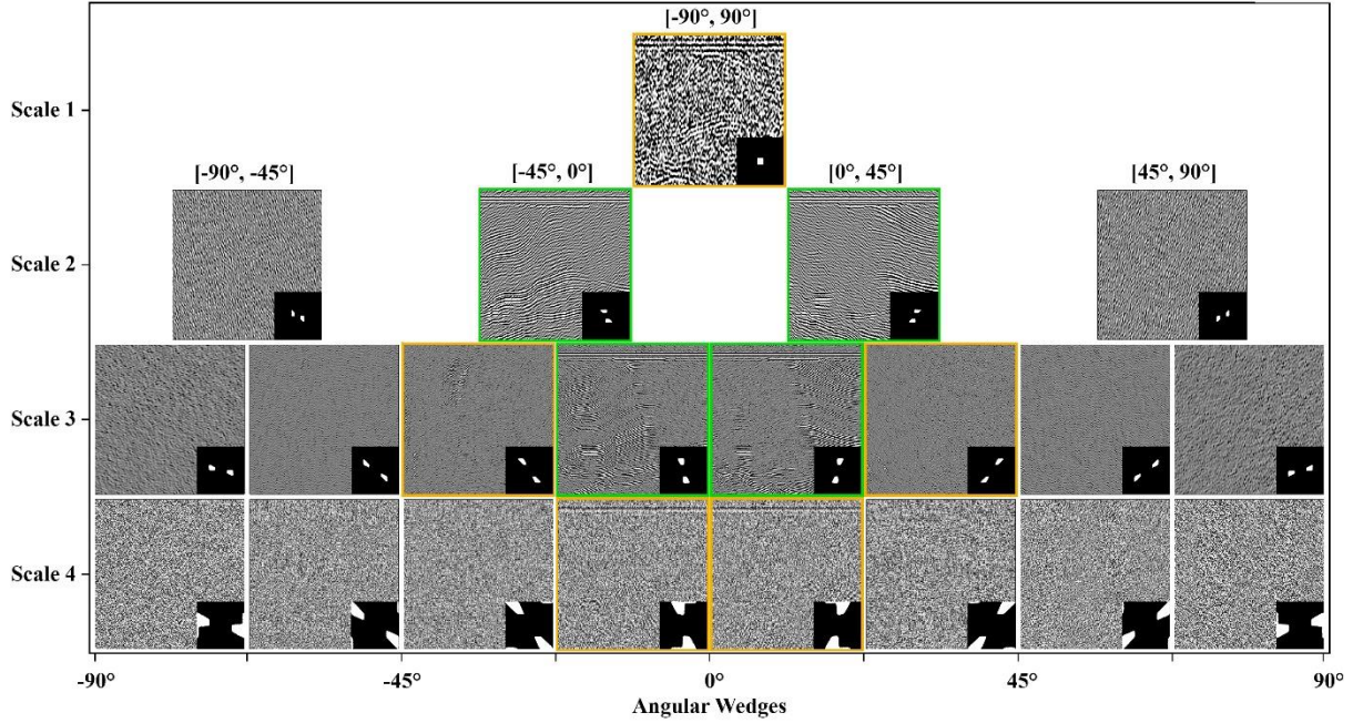
Figure 7.10: Example of the inverse curvelet transform applied to different scales and angular wedges. The reflection horizons of the Marmousi2 data subset can be best represented by scale 2 (angular wedges from -45^\circ to 45^\circ ) and scale 3 (angular wedges from -22.5^\circ to 22.5^\circ ), highlighted in green. Curvelets domains highlighted by yellow also have some reflection data. The f-k spectrum is shown in the bottom right corner of each inverse transform, where black is equal to zero, i.e. no energy content at these frequencies and wavenumbers.
