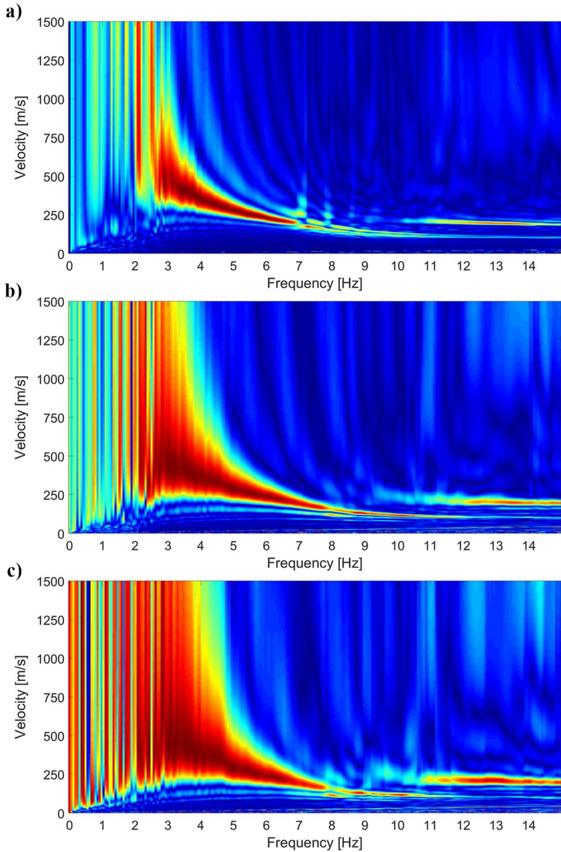
Figure 4.11: Comparison of dispersion plots for station BKAN. 4.5 Hz array of all 96 geophones are shown in (a). 4.5 Hz array of 12 geophones at corresponding locations of 1 Hz array are shown in (b). 1 Hz array of 12 geophones are shown in (c).
