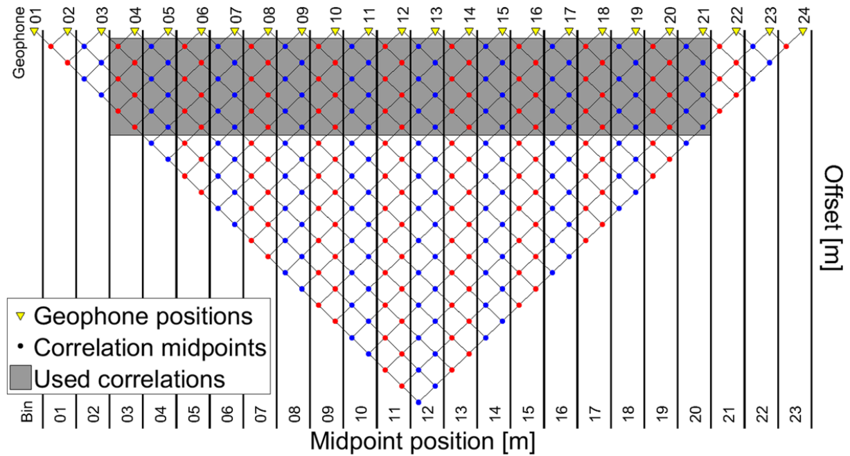
Figure 4.7: Schematic representation of CMPcc binning. Geophones are represented by yellow triangles, and the correlation midpoints are indicated by dots. The correlations within the grey zone are used for analysis. Only bins with a sufficient number of midpoints are used (bins 3 to 20 in this example) and fixed offset range (6 geophones in this example).
