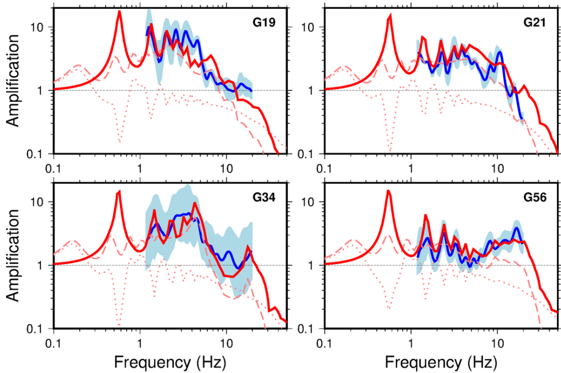
Figure 4.18: Comparison for selected G stations of FAS spectral ratio of surface to 200 m depth from the Groningen earthquake recordings database (blue) and standard deviation (pale blue) along with the spectral ratio of surface to 200 m depth from theoretical 1D SH linear site response analyses (solid red). The dashed red line indicates the 1D SH TF at the surface and dotted red line at 200 m depth.
