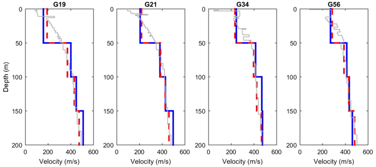
Figure 4.16: V_s profiles at selected G stations. Interval V_s from seismic interferometry in blue, modelled mean V_s (Kruiver et al., 2017a) in grey and harmonic means of modelled V_s in dashed red.
