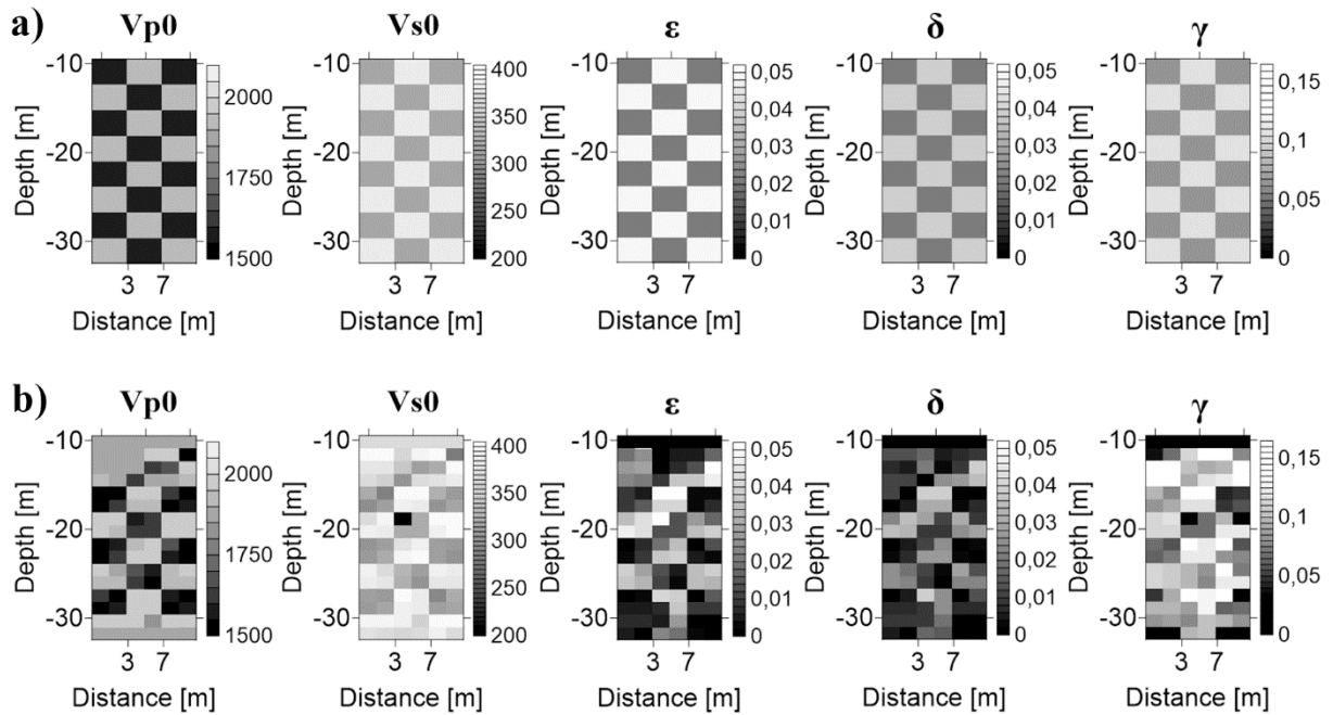
Figure 6.11: Coarse checkerboard VTI-model with approximately 3 \times 3 m cell sizes (a) and the reconstructed model (b).
