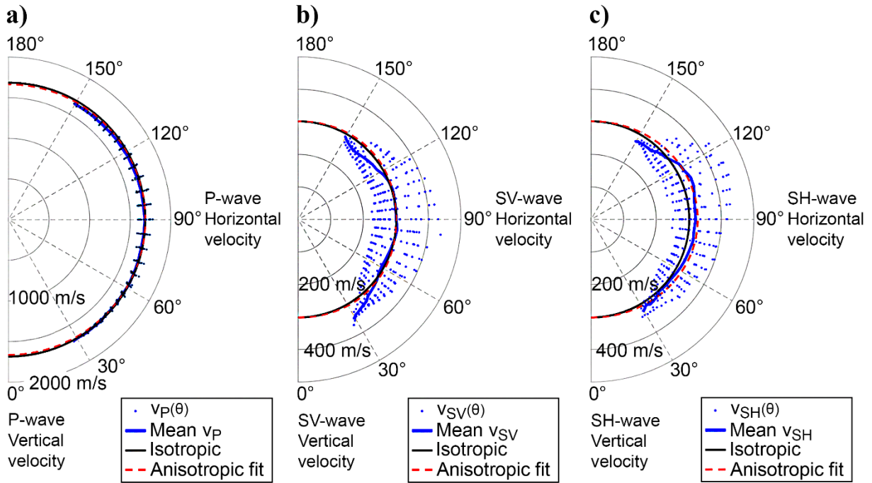
Figure 6.8: Straight ray velocities are shown which are plotted as a function of the ray path angle for P-waves (a), SV-waves (b) and SH-waves (c) in the VTI zone of Plane 2 of the SAFIRA dataset. The mean velocities for a ray path angle are shown by the blue curve. The velocities in a homogeneous isotropic medium would lie on the black curve. The mean velocities and the black isotropic curve deviate marginally for the P-waves and up to about 10% for the S-waves. We invert for VTI parameters which fit angle dependent velocities (red dashed curves) to the mean velocities.
