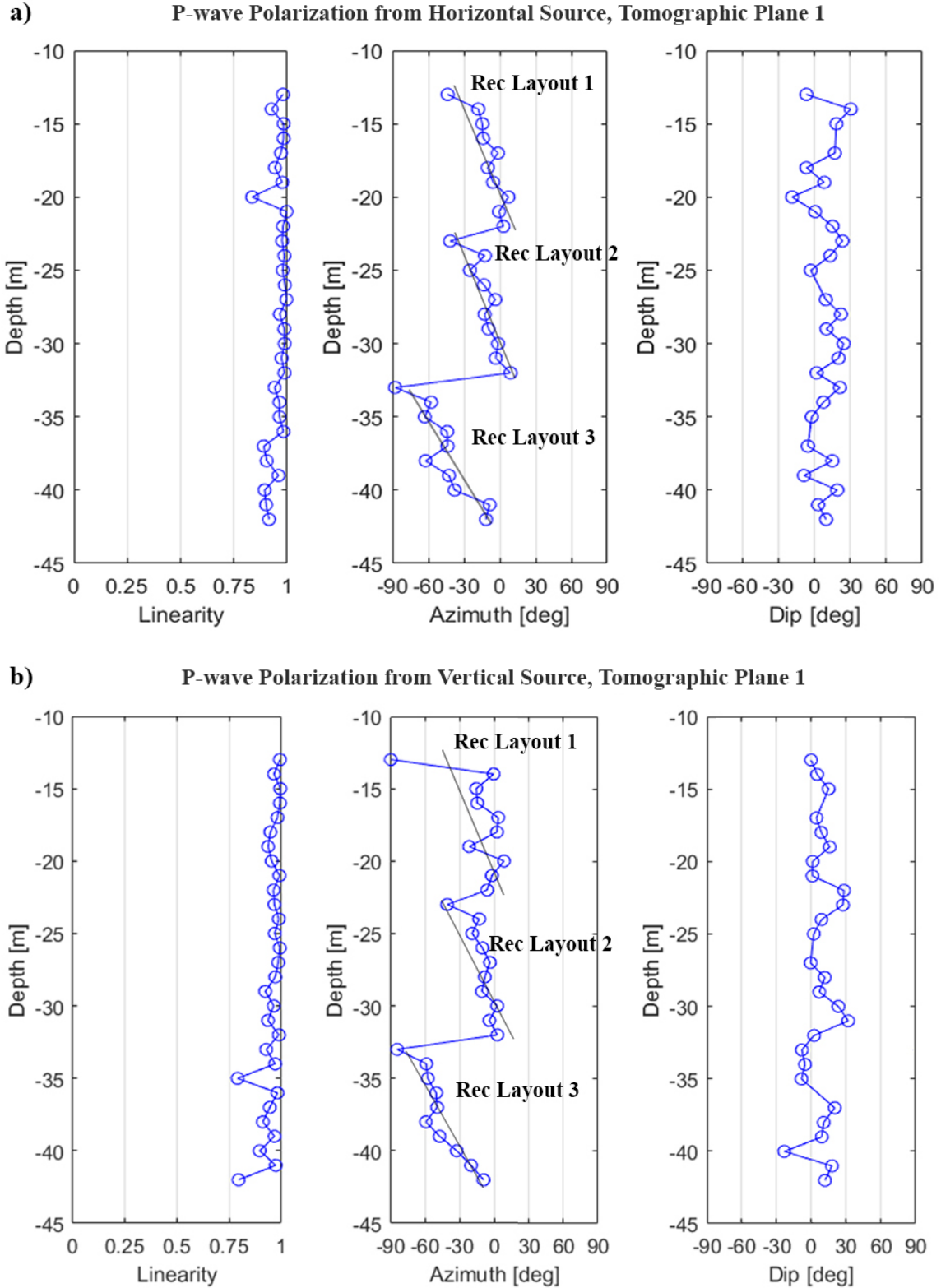
Figure 6.4: P-wave polarization of the crosshole data subset for tomographic Plane 1 (boreholes B44 and B45). The linearity, azimuth and dip is determined from the hodograms as a function of depth. The polarization is determined for both sources: the horizontally polarized source (a) and the vertically polarized source (b). The azimuth of the P-wave is a function of the ten-level receiver spreads.
