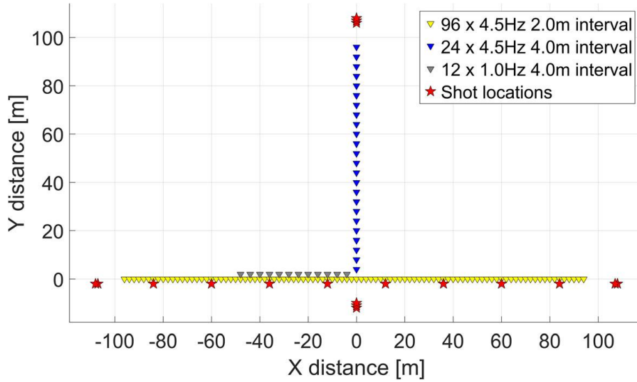
Figure 4.5: Survey setup for MASW and microtremor array with planted geophones. Triangles represent geophone locations, and stars represent shot locations.
