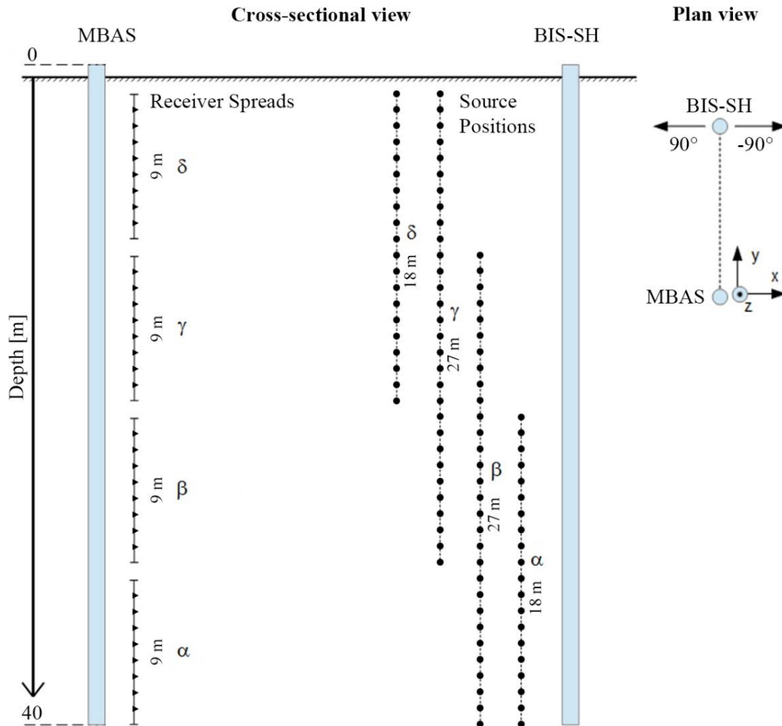
Figure 2.12: Typical S-wave acquisition sequence using the BIS-SH and a 10 station MBAS receiver array. Here the seismic data is gathered for depths of 40 m to 1 m for a total of 4 receiver spreads. The receiver and shot spreads are shown in a cross-sectional view, whereby the Greek letters associate the receiver with the shot spreads. The plan view shows the shooting direction of the BIS-SH, either shooting in a 90° or -90° angle to the receiver borehole, and the receiver orientation of the X-, Y- and Z-channel.
