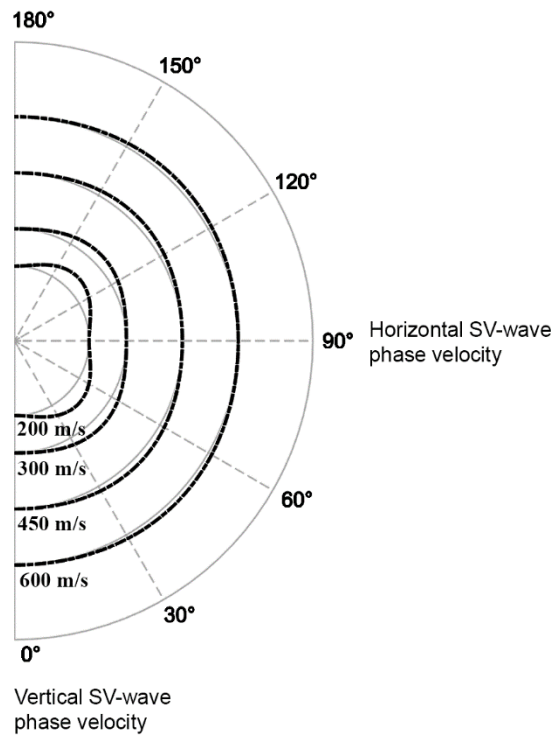
Figure 6.14: SV-wave velocity as a function of the raypath angle for different V_p/V_s ratios is shown. The P-wave velocity and the difference between \varepsilon and \delta were kept constant at 1800 m/s and 0.01. High V_p/V_s ratios amplify SV-wave anisotropy severely, even if the anisotropy parameters \varepsilon and \delta are small in magnitude.
