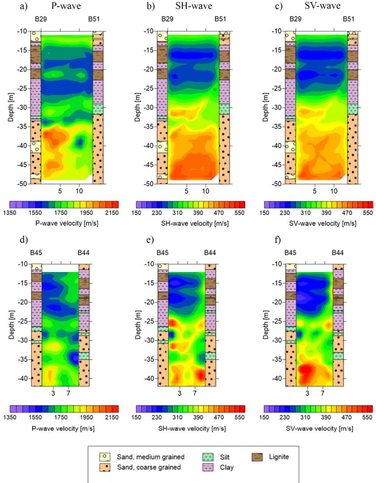
Figure 5.5: Jointly inverted P-, SH- and SV-wave tomograms between boreholes B29 and B51 (a-c) and between boreholes B44 and B45 (d-f) at the SAFIRA research site. The joint-inversion couples the S-wave tomograms (b, c, e, f) to the more accurate P-wave tomograms (a,d) and thereby reduces the artefacts in the S-wave tomograms.
