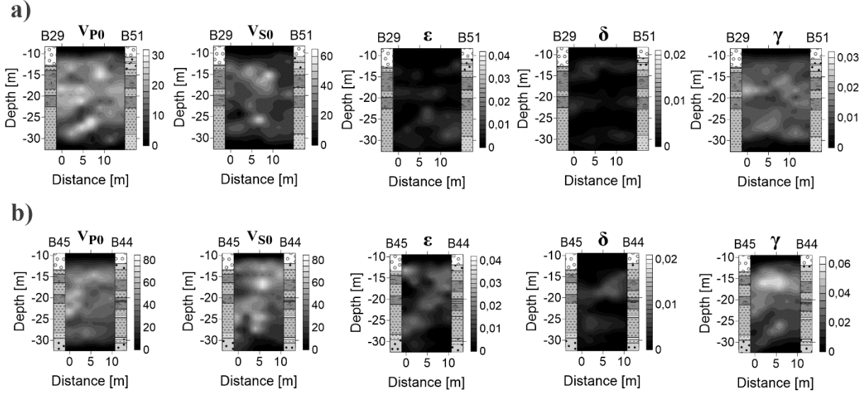
Figure 6.13: The absolute error estimated for the VTI parameters for Plane 1 (a) and Plane 2 (b). First, inversions were performed with perturbed traveltimes, i.e. normally distributed noise was added. Subsequently, an error was determined from the original inversion results (see Figure 6.9 and Figure 6.10). This procedure was repeated 100 times, i.e. 100 inversions with random errors. Finally, the absolute error is determined as two standard deviations from the error distributions.
