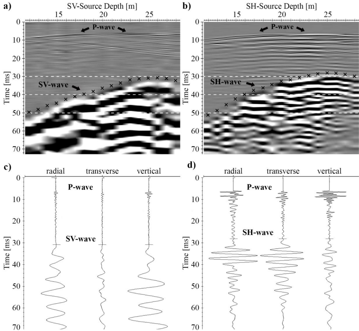
Figure 6.7: Receiver gather at a depth of 22 m, generated with the vertically (a) and horizontally polarized source (b) in borehole B44. The data are shown in variable density visualization. Vertical component data is shown for the vertically polarized source (a) and transverse component data is shown for the horizontally polarized source (b). The S-wave traveltimes are indicated by the crosses (SV-wave traveltimes (a), SH-wave traveltimes (b)). An example of three component data is shown in (c) and (d) for a source depth of 25 m and a receiver depth of 22 m (vertically polarized source (c) and horizontally polarized source (d)).
