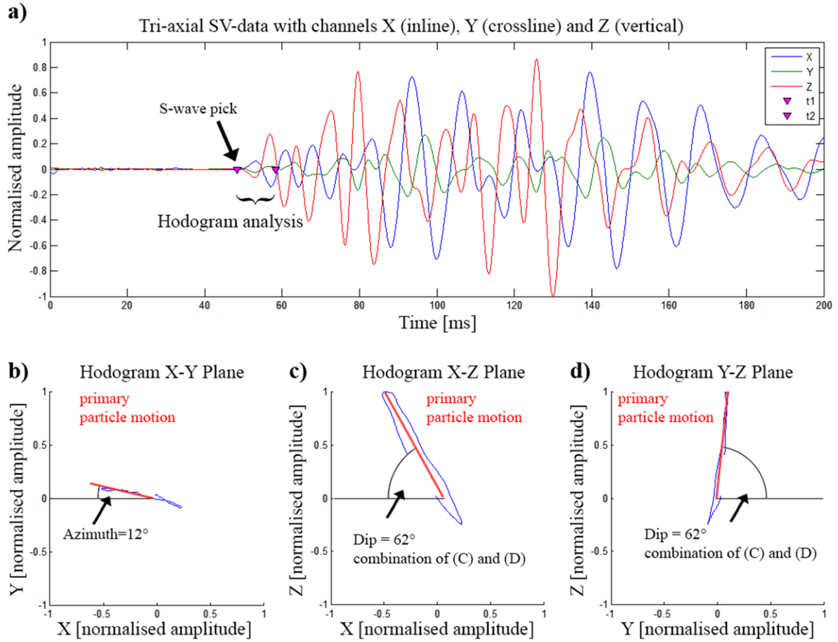
Figure 6.3: Example hodogram analysis with the primary particle motion indicated by the red line in the bottom three hodograms. The hodograms with calculated primary particle motion (b) to (d) depict particle motion for different 2D planes and are determined for a 10 ms window, starting with the S-wave traveltimes pick from the vertically polarized source data.
