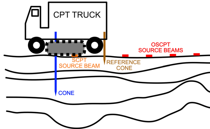
Figure 4.2: Schematic illustration of offset SCPT setup (not to scale).
