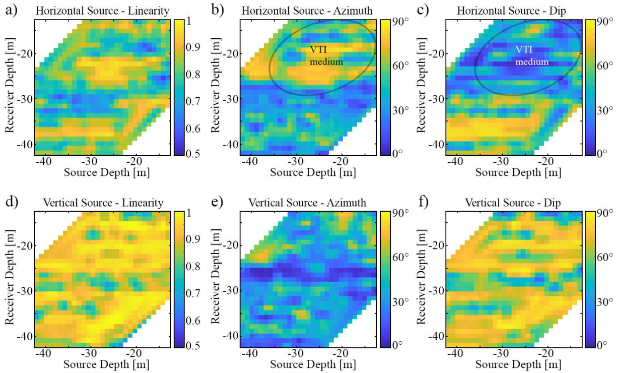
Figure 6.6: S-wave polarization is shown for the horizontally (a-c) and vertically polarized source (d-f). The linearity, azimuth and dip is shown as a function of the receiver and source depth for tomographic Plane 2, between boreholes B44 and B45.
