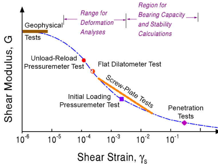
Figure 2.3: Relationship between the Shear modulus ( G ) and the shear strain ( \gamma_s ), modified after Mayne (2001) is shown. Note the inverse relationship between G and \gamma_s and the flattening out of G for very small \gamma_s . This flattening out is referred to as the maximum Shear modulus G_0 . The Shear modulus axis is linear and magnitudes of G are dependent on the material.
