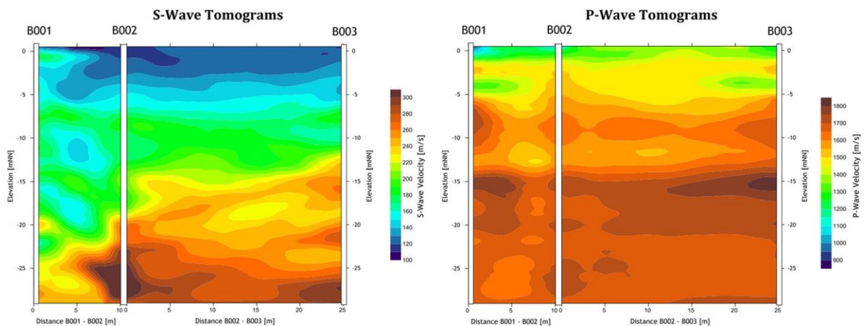
Figure 4.12: V_S and V_P images from cross-hole tomography for station BUHZ.
