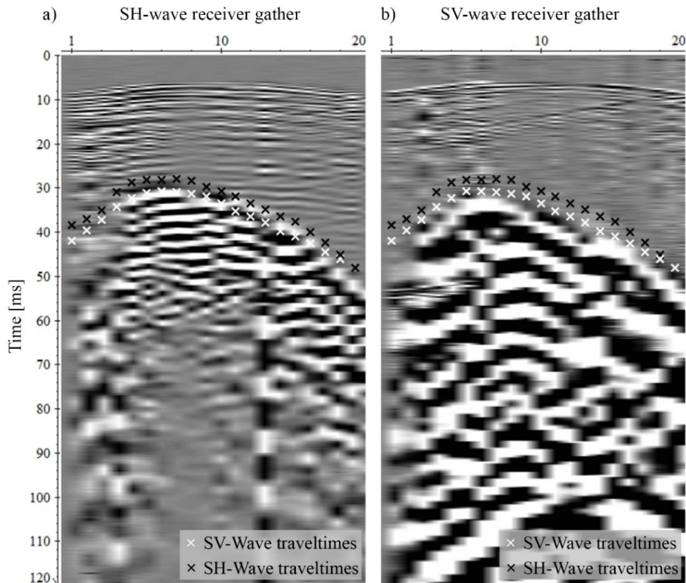
Figure 5.7: Receiver gathers at a depth of 22 m in variable density visualisation for the SH-wave source (a) and the SV-wave source (b). There is a considerable difference from SH-wave traveltimes (black crosses) to SV-wave traveltimes (white crosses). The presence of anisotropy is unlikely due to a deficient picking accuracy.
