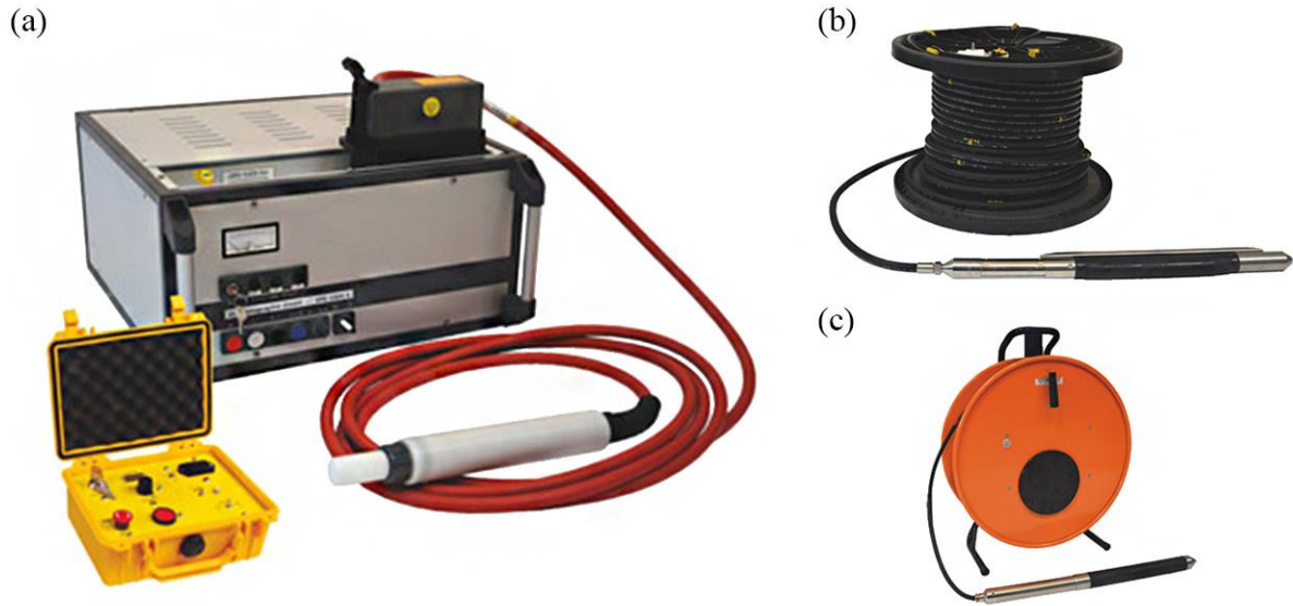
Figure 2.9: P- and S-wave generating equipment using the 5000 V generator IPG5000 (a). Triggering occurs remotely, using the yellow remote control unit. The horizontal source BIS-SH (b) generates both P- and S-waves, and the sparker source SBS42 (c) generates high-amplitude P-waves. (photos provided by Geotomographie GmbH)
