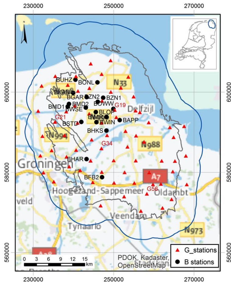
Figure 4.1: Location of recording stations in the Groningen field in the north of the Netherlands: 18 surface stations and 68 vertical array stations. Labels are shown for all 18 surface stations (coded B) characterised in this study and for the vertical array stations (coded G) from the examples in this paper (Figs. 16 and 18). Grid coordinates refer to the Dutch Ordnance System. The inset shows the location of the gas field in the northern part of the Netherlands.
