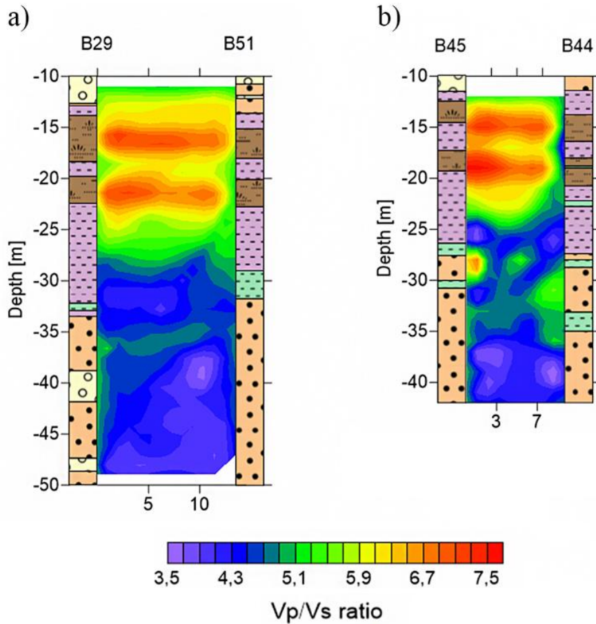
Figure 5.6: Ratio of the jointly inverted P-wave to S-wave velocities for boreholes B29-B51 (a) and B44-B45 (b).
