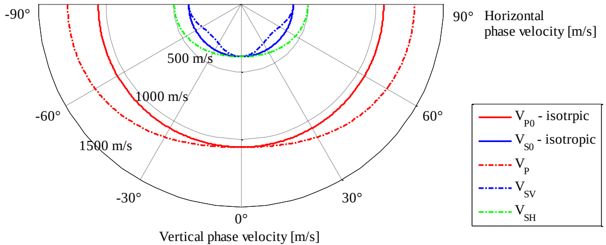
Figure 2.6: Re-produced forward modelling of anisotropy parameters by measuring angle dependent P- and S-wave phase velocities in Wills Point shale (Robertson and Corrigan, 1983). The VTI parameters are v_{P0} = 1058 m/s, v_{S0} = 387 m/s, \epsilon = 0.215 , \delta = 0.315 and \gamma = 0.280 .
