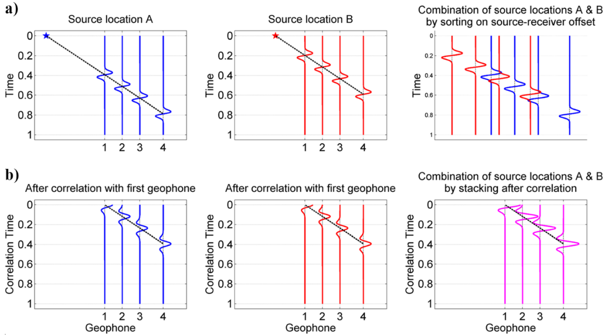
Figure 4.6: Sorting and pre-processing of MASW data to obtain offset gathers (a) and geophone correlation gathers (b) to prepare for CMPcc binning.
