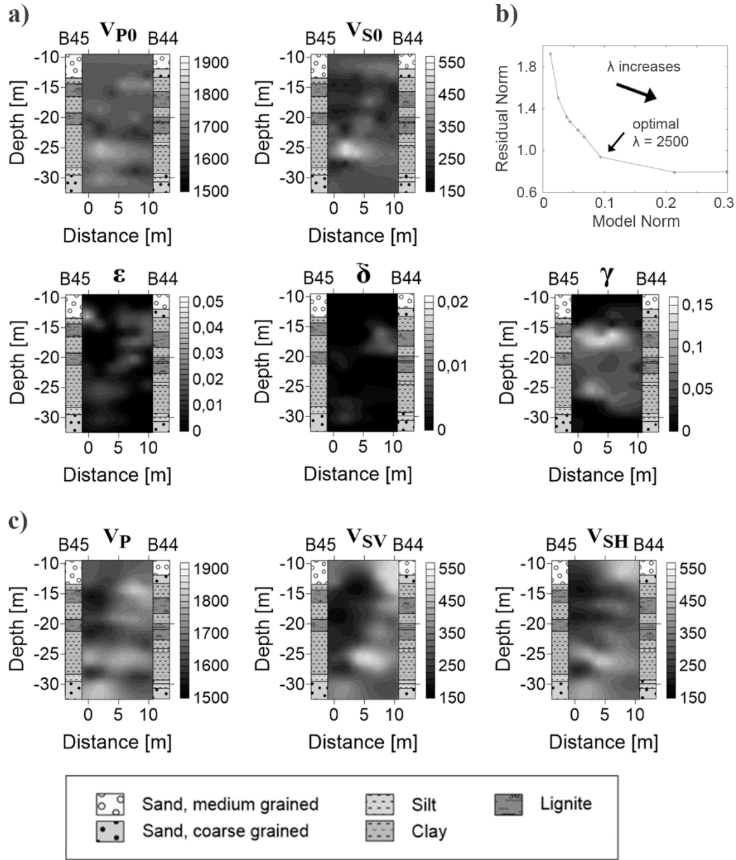
Figure 6.10: Joint-inversion for VTI parameters for tomographic Plane 2 (between boreholes B44 and B45) is shown in (a). We chose the cross-gradient parameter ( \lambda = 2500 ) by trading off between the model norm and the residual norm for inversions with different values for \lambda (b). Separate isotropic inversions of the P-, SV- and SH-wave data is shown in (c).
