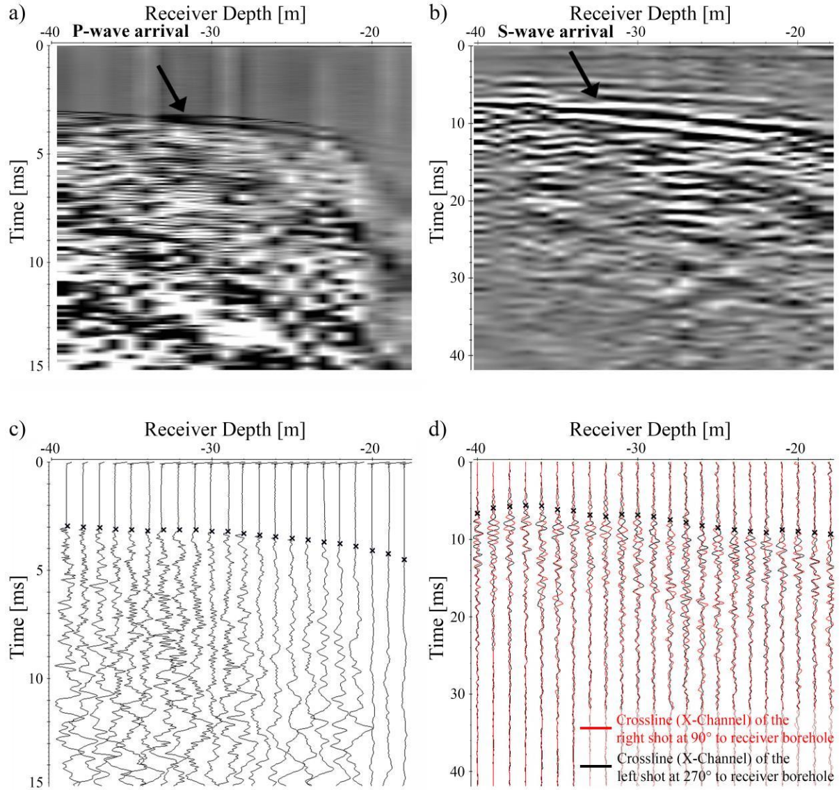
Figure 3.1: Examples of the shot gathers shown in variable density mode for the P-wave source (a) and the S-wave source (b), both at 36 m depth. The traveltime picking is shown, whereby the data are displayed in variable amplitude mode for the P-wave (c) and the S-wave (d). The traveltime picks are shown by the black crosses.
