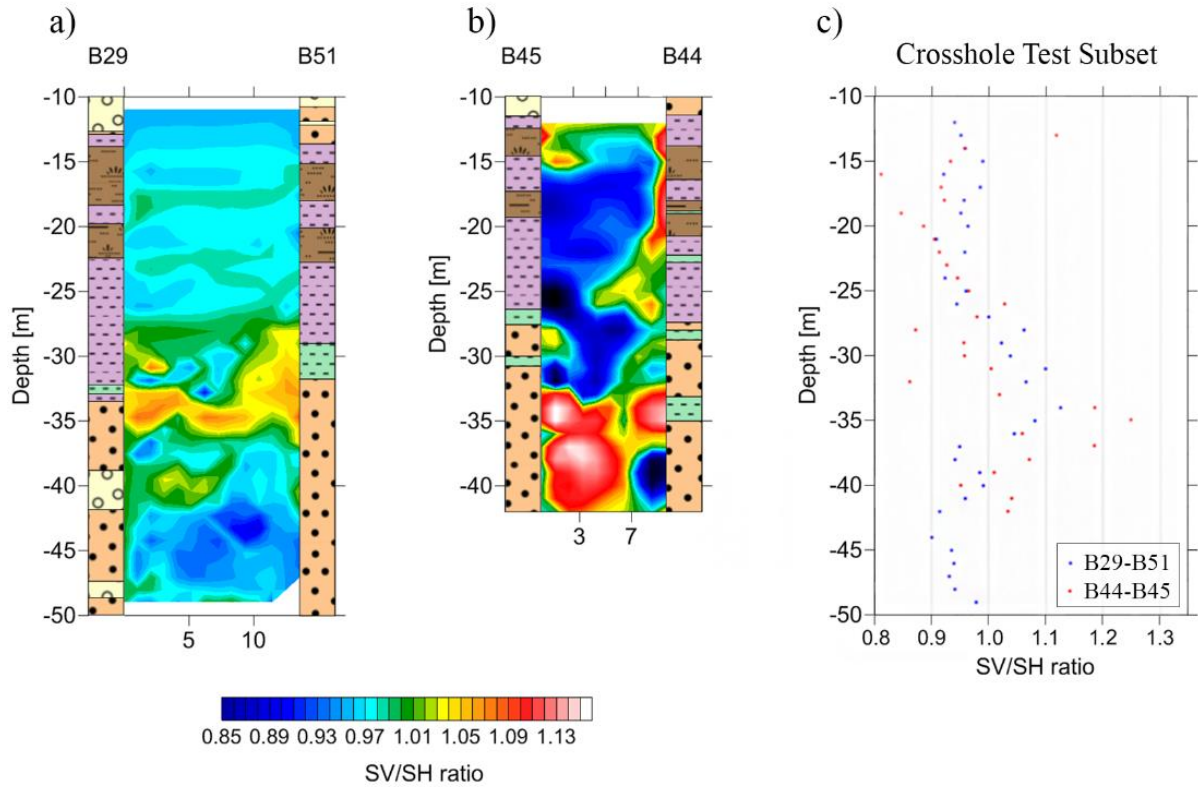
Figure 5.8: Ratio of the jointly inverted SV- and SH-wave tomograms for tomographic plane B29-B51 (a) and B44-B45 (b). The general trend is similar to the one suggested by the velocities of the horizontal raypaths (c).
