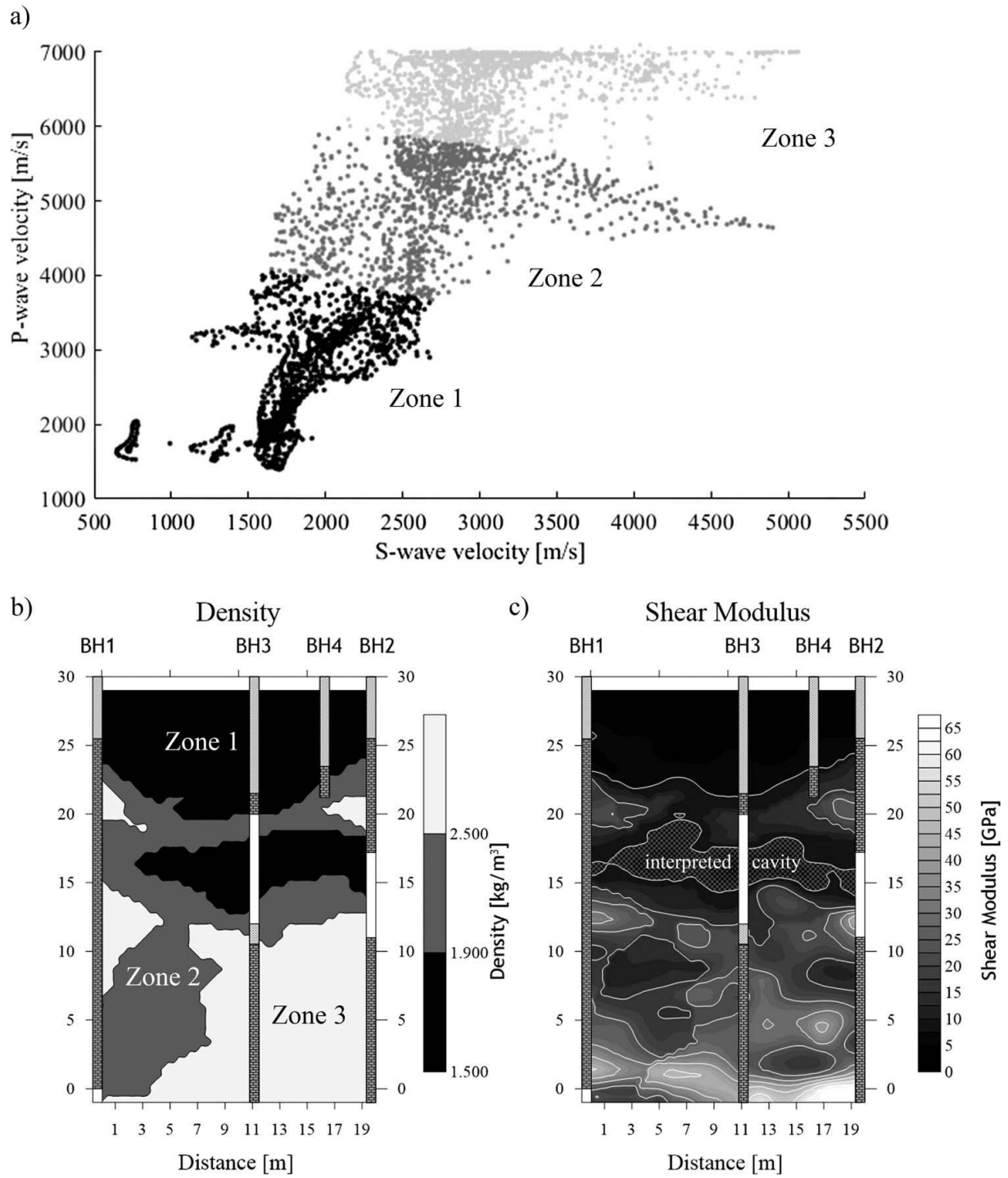
Figure 3.4: Density zonation and Shear Modulus: (a) k-means clustering to partition the tomograms into three zones, (b) the assignment of density values to three zones, and (c) calculated shear modulus.
