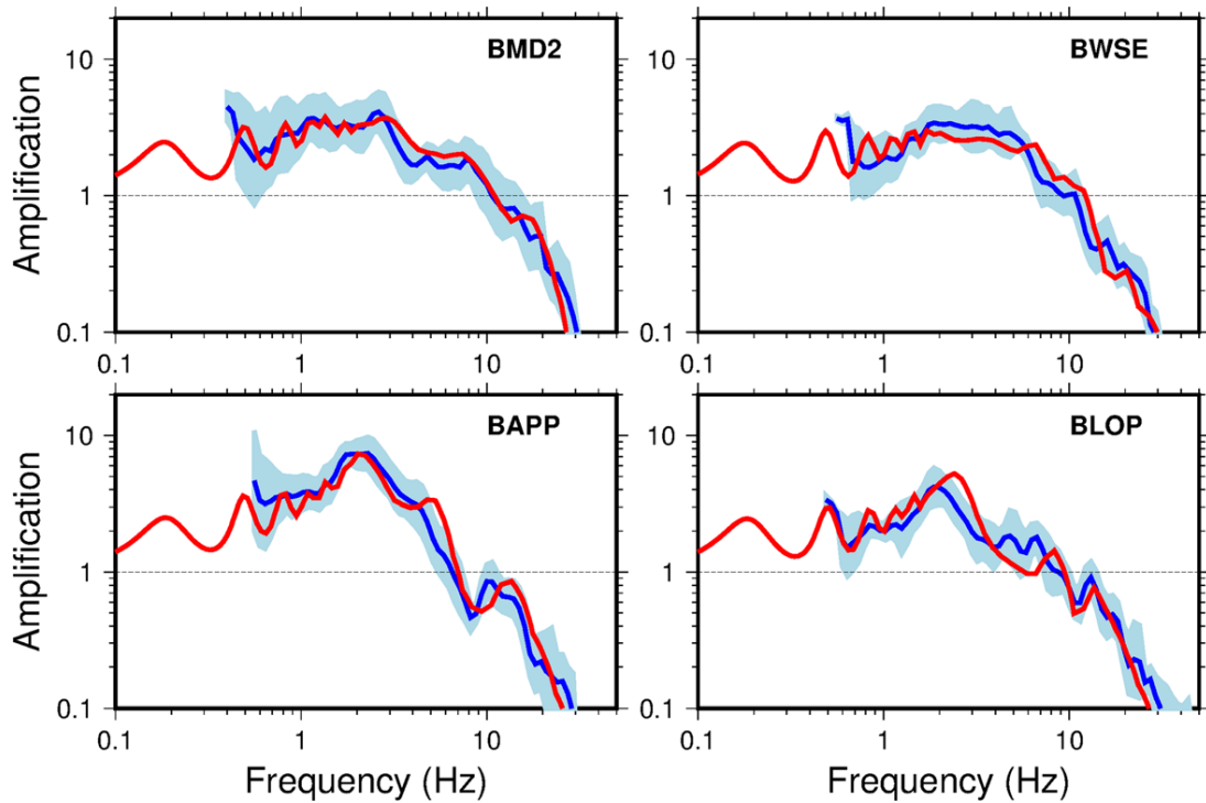
Figure 4.17: Comparison for selected B stations of empirical amplification (reservoir to surface amplification) from the Groningen earthquake recordings database (blue) and standard deviation (pale blue) along with the theoretical vertical 1D SH amplification between the reference and surface (red) based on numerical linear site response analyses.
