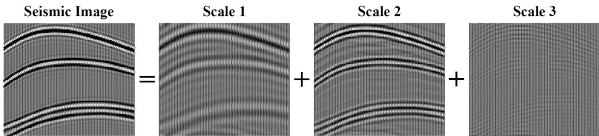
Figure 7.4: Example of a seismic image and its deconstruction into multi-scale curvelets.
