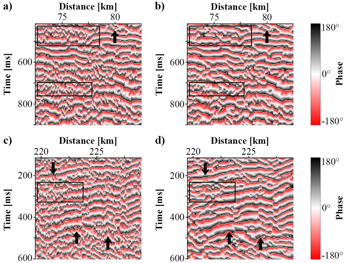
Figure 7.14: Instantaneous phase computed for a selection of Line 2 (a, b) and for a selection of Line 3. The selections are indicated by the white boxes in Fig. 7.12 (Line 2) and Fig. 7.13 (Line 3). The curvelet denoised sections (b, d) show better instantaneous phase continuities compared to the original data sections (a, c).
