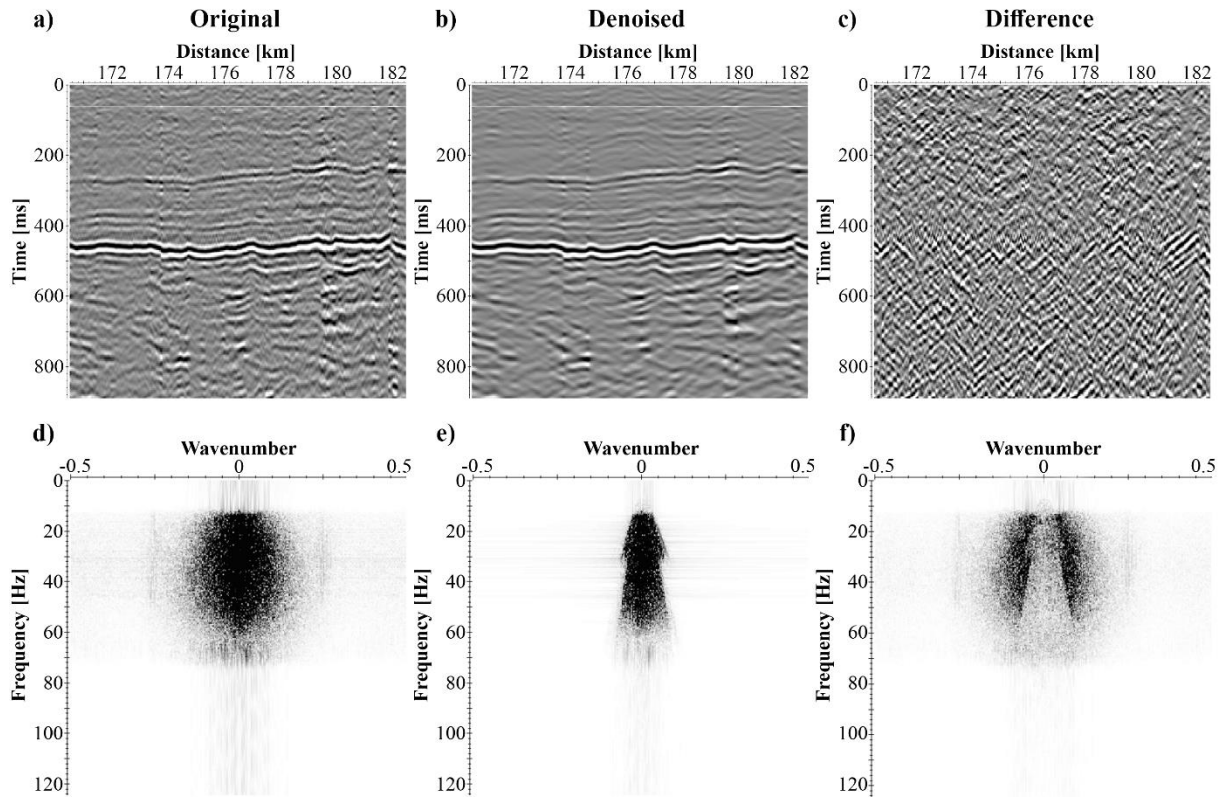
Figure 7.11: Curvelet denoising applied to the CBM Botswana dataset. The original data (a) is enhanced by curvelet denoising (b). The difference between the original and denoised data is shown in (c), which mainly consists of dipping events that interfere with the horizontal reflection horizons. The corresponding frequency-wavenumber domains are shown in (d) to (f).
