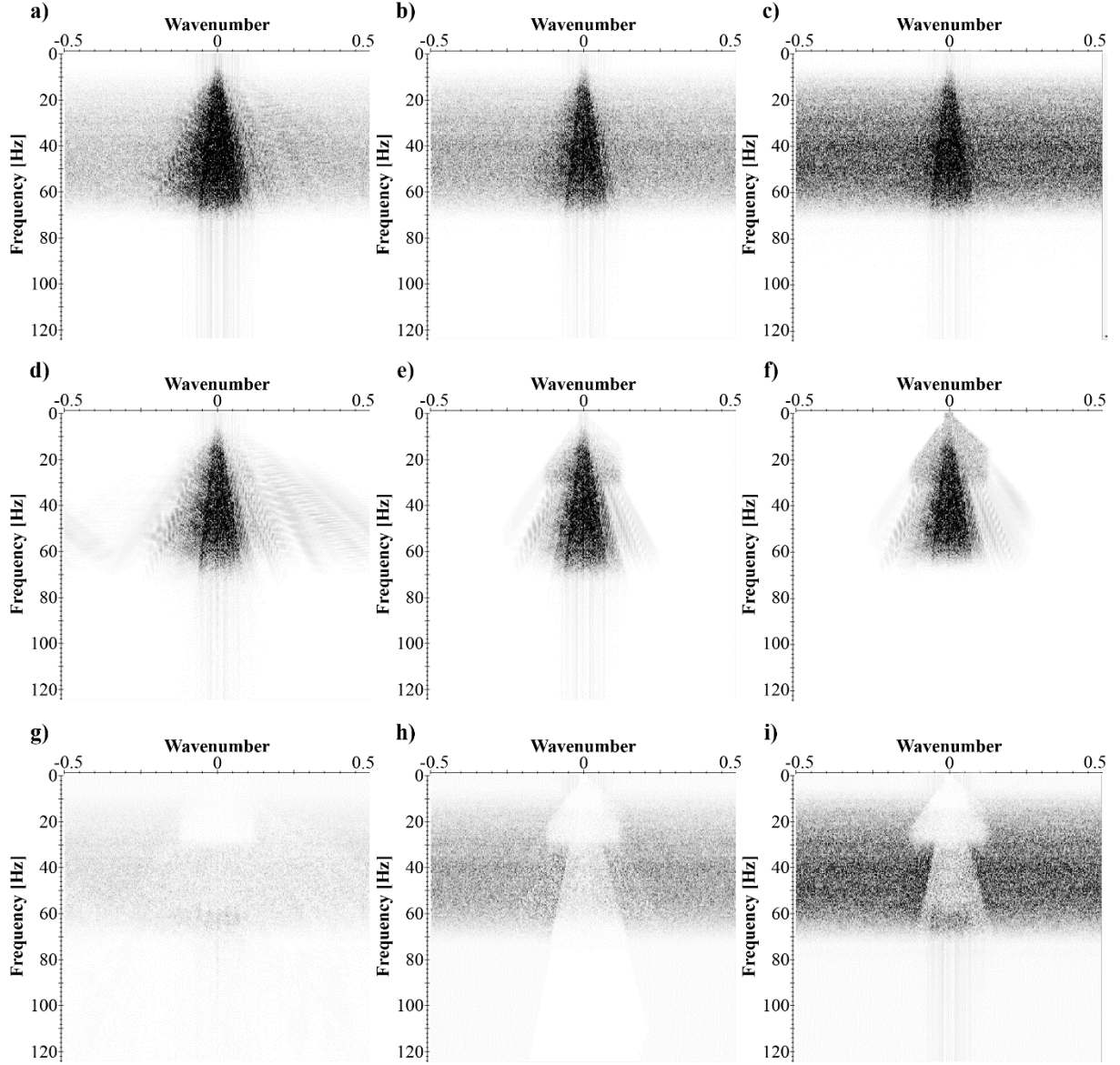
Figure 7.9: The frequency-wavenumber domains corresponding to the curvelet denoising applied to the Marmousi2 subset with added self-similar noise (Fig. 7.7).
