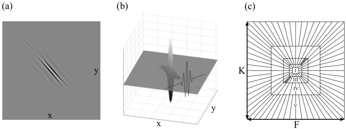
Figure 7.3: A curvelet is shown in the spatial domain (a). A different visualisation in the spatial domain is shown in (b), where a Gaussian function constrains the curvelet in the smooth direction and a wavelet constrains the curvelet in the oscillatory direction. The rapidly decaying amplitude of the curvelet in the spatial domain makes its localisation possible. The frequency domain of the curvelet has the form of two wedges around the origin (c). This curvelet is of scale 3, with the other scales indicated by Roman numerals, in this example from scale I to scale V. For every other scale, the number of angular wedges doubles (second dyadic coroneae structure).
