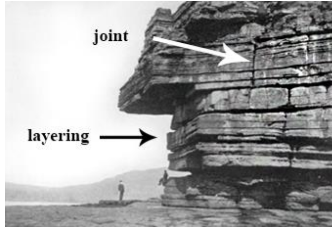
Figure 2.4: Example of a (most likely) seismic anisotropic rock. Here, Muckcross Head, Ireland, is shown with the layering of the sandstone and joints causing probably either an orthorhombic or monoclinic symmetry (modified from Thomsen, 2002).
