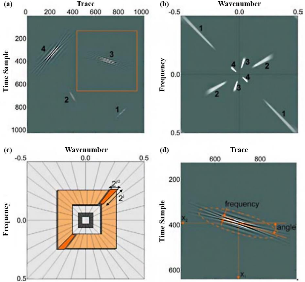
Figure 2.13: Curvelets of different scales and angular directions are shown in the spatial (a) and Fourier domain (b). The construction of the curvelets takes place in the Fourier domain, which is partitioned into angularly and radially constrained windows (c). Curvelets of scale 1 are at the centre, and the highlighted curvelet (d) is of scale 4. (modified after Górszczyk et al., 2014).
