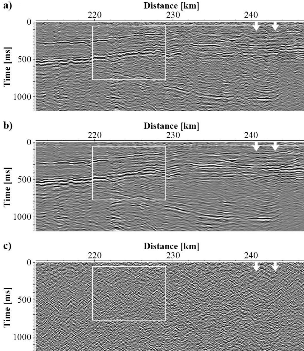
Figure 7.13: Curvelet denoising applied to the original data of Line 3 (a), with improvements shown after the denoising in (b). The difference between the original data and the denoised data is shown in (c). Both continuity (white arrows) can be enhanced and high frequency noise (white box) can be removed by applying the transform to the data, without compromising the quality of the reflection horizons. Attribute analysis of the data in the white box is shown in Fig. 7.14 (c) and (d).
