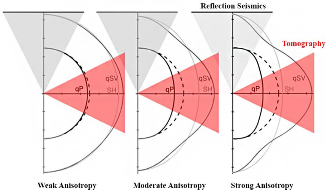
Figure 2.8: Cross-borehole measurements, with the angular domain highlighted in red, are severely more affected by anisotropy compared to surface seismic reflection surveys, with the angular domain highlighted in grey. The slowness ( qP , qSV , qSH ) as a function of polar angle illustrates this (modified after Helbig and Thomsen, 2005).
