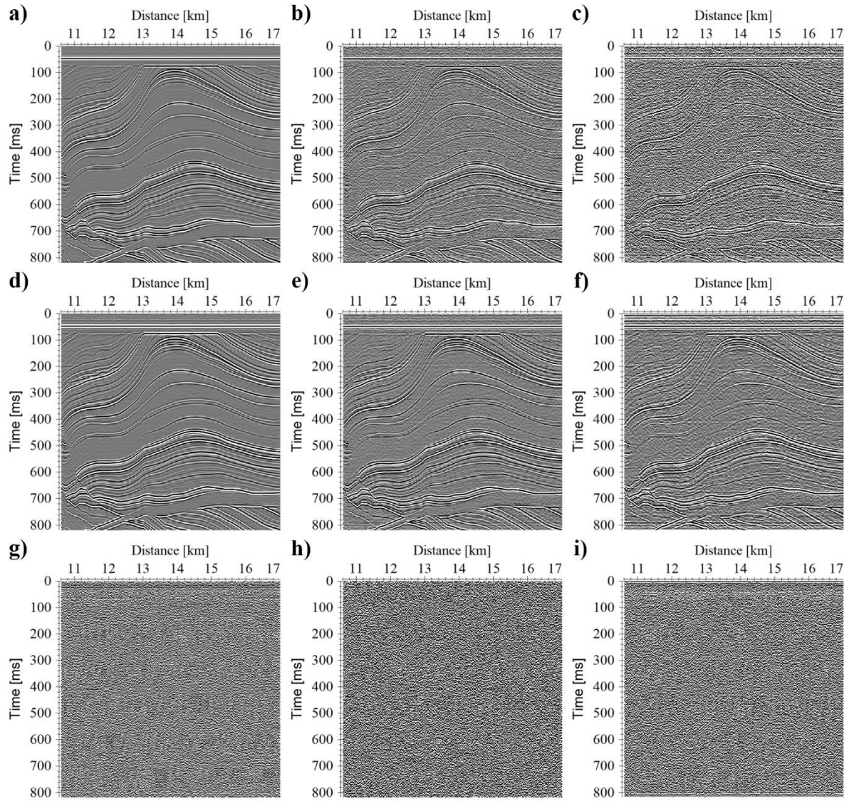
Figure 7.7: We add 20% (a), 50% (b) and 100% (c) self-similar noise to the Marmousi2 data subset (Fig. 7.5) and denoise using the curvelet transform, with 20% noise: (d), 50% noise: (e), 100% noise (f). The difference of the noisy datasets and the denoised datasets are shown in (g) to (i). The corresponding frequency-wavenumber domains are shown in Fig. 7.9.
