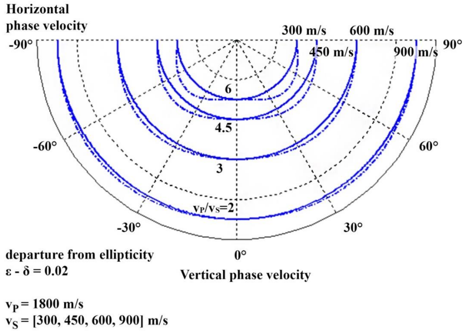
Figure 2.7: Forward modelling of SV-wavefront anisotropy effects for varying v_{P0}/v_{S0} ratios. The P-wave velocity was kept constant at 1800 m/s, as well as the small departure from ellipticity ( \epsilon - \delta ) at 0.02. The isotropic wavefront is shown by the semi-circular solid blue line and the anisotropic wavefront is shown by the dashed line. We can see that for high v_P/v_S ratios the wavefront departs substantially from the isotropic circular reference, even for such minor anisotropy.
