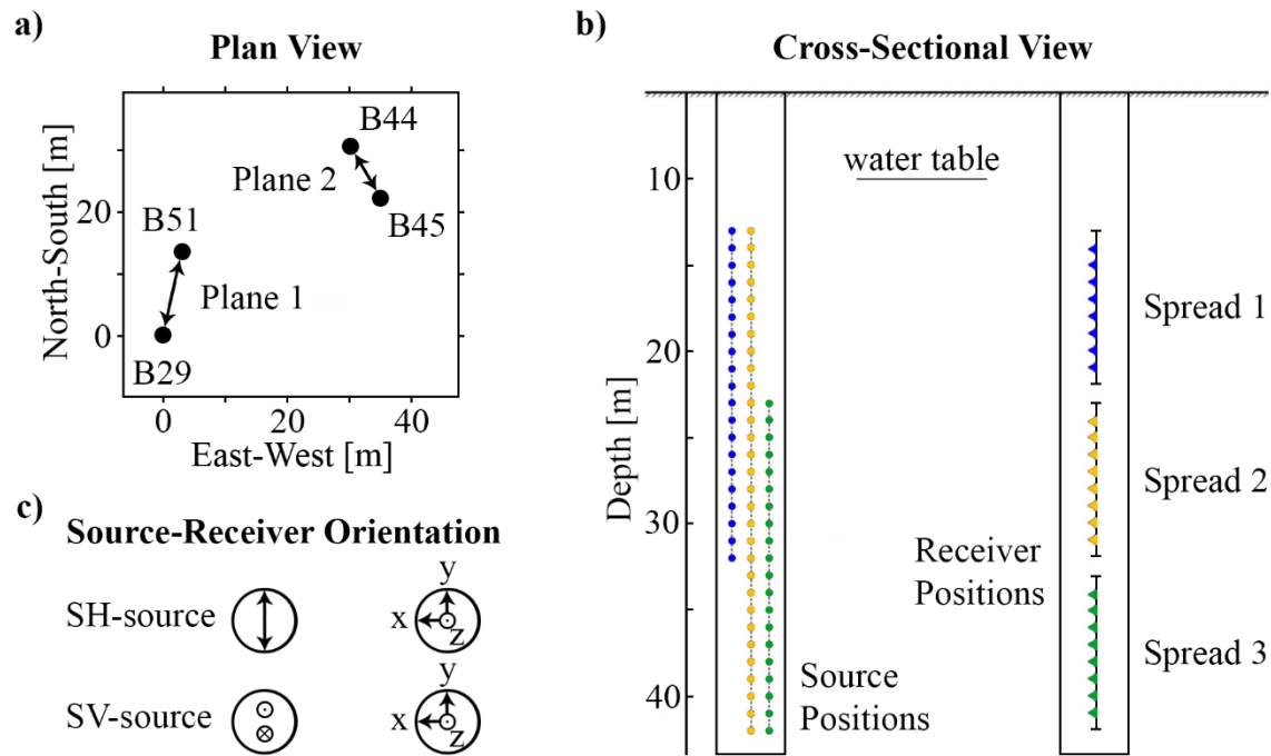
Figure 6.2: Overview of boreholes employed for the seismic acquisition (a) for Plane 1 (14 m between boreholes B29 and B51) and Plane 2 (10 m between boreholes B44 and B45). A cross-sectional view is shown in (b) with example source and receiver positions for different ten-level receiver spreads. The horizontally and vertically polarized source striking directions and three-component receiver orientations are shown in plan view in (c).
