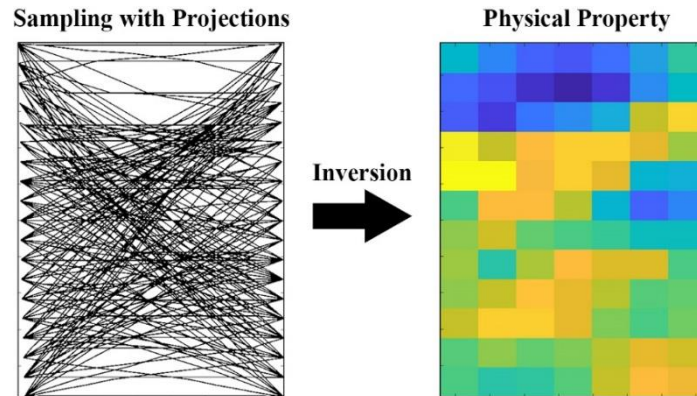
Figure 2.1: Principle of cross-borehole seismic traveltimes tomography. The lines show the sampling of the medium and are the raypaths, i.e. the projections. From a traveltimes inversion a physical property distribution, for example a 2D P-wave slowness distribution, can be estimated.
