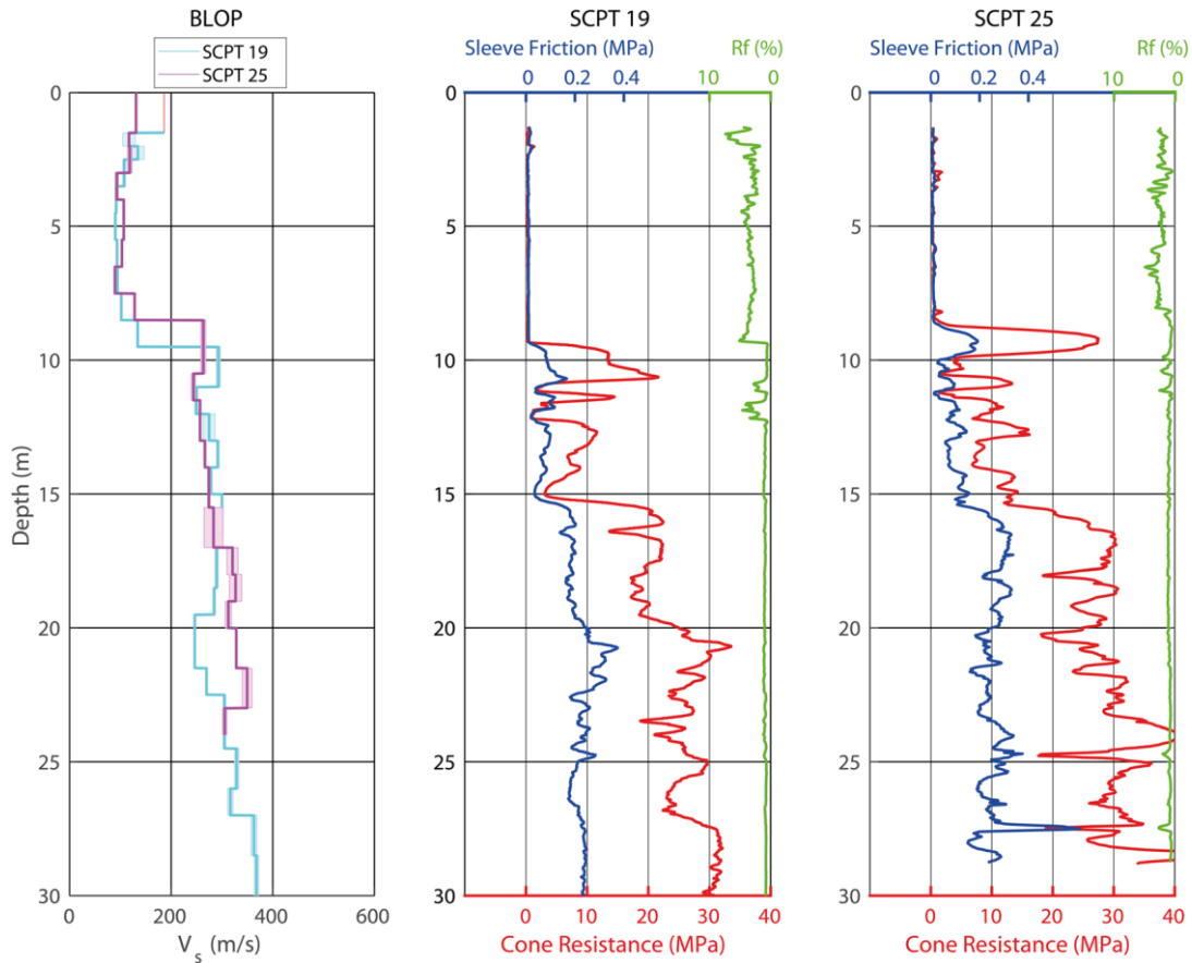
Figure 4.3: CPT and SCPT data for station BLOP. Left: V_s profiles of SCPT 19 (blue) and SCPT 25 (purple). The shaded band indicates the results from the left and the right blow. Middle and right: CPT soundings of SCPT 19 and SCPT 25, with cone resistance in red, sleeve friction in dark blue and friction ratio R_f in green.
