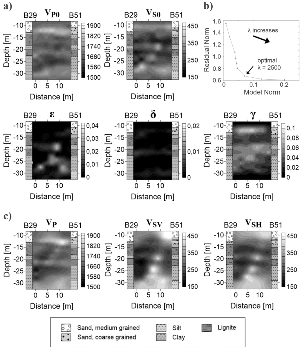
Figure 6.9: Joint-inversion for VTI parameters for tomographic Plane 1 (between boreholes B29 and B51) is shown in (a). We chose the cross-gradient parameter ( \lambda = 2500 ) by trading off between the model norm and the residual norm for inversions with different values for \lambda (b). Separate isotropic inversions of the P-, SV- and SH-wave data is shown in (c).
