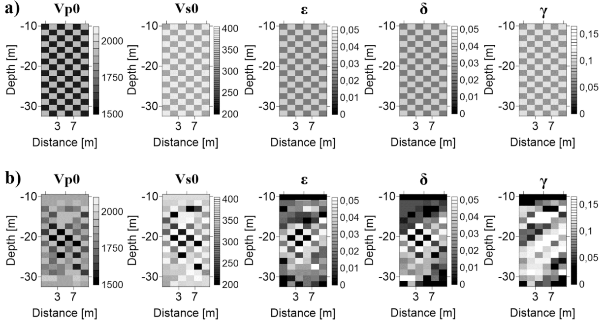
Figure 6.12: Fine checkerboard VTI-model with approximately 1.5 \times 1.5 m cell sizes (a) and the reconstructed model (b).
