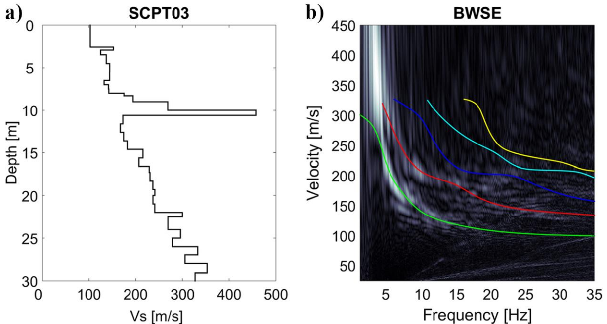
Figure 4.14: Example of SCPT profile on MASW for station BWSE. SCPT03 V_s profile with the top 3 layers replaced by the minimum value (a). Theoretical dispersion curves of the V_s profile for fundamental (green) and higher modes (red, blue, cyan and yellow) plotted on top of the MASW dispersion plot (grey scale) for station BWSE (b).
