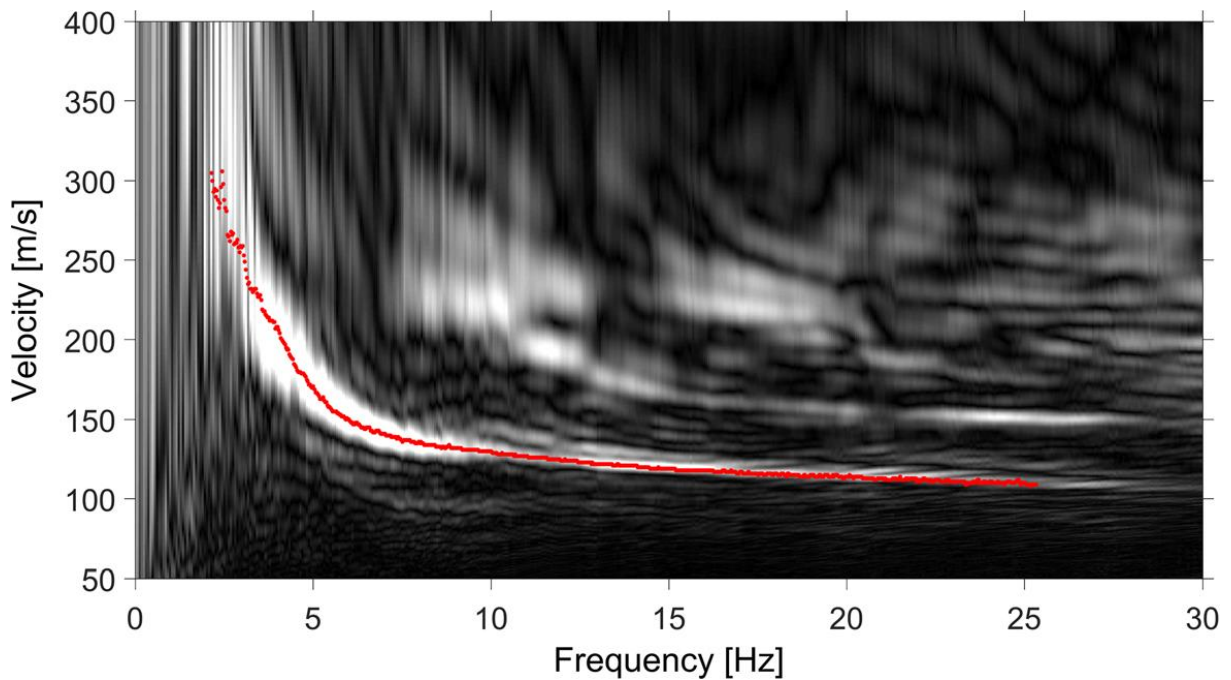
Figure 4.10: Dispersion curves determined with the ESAC method applied on the passive data at BGAR (red dots) plotted on top of the (black and white) dispersion plot determined for the active data using the MASW method.
