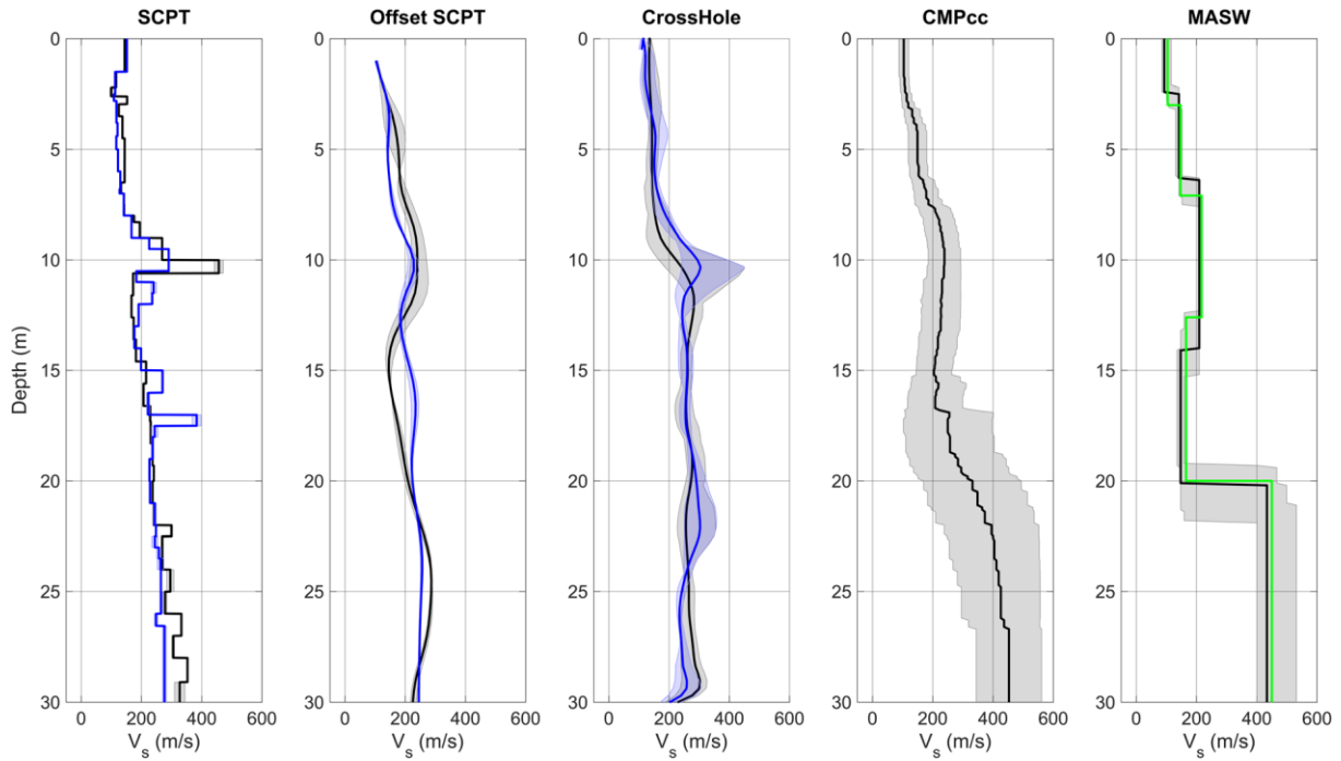
Figure 4.13: V_s profiles for station BWSE from different measurement techniques, including uncertainty bands. From left to right: SCPT03 (grey) and SCPT04 (blue) with band indicating variation between left and right blow; average profile for offset SCPTs between 1 and 5 m offset with shaded band indicating the minimum and the maximum V_s ; cross-hole average profiles for long leg (blue) and short leg (grey) with shaded band indicating the minimum and the maximum V_s ; CMPcc based on MASW array, shaded band indicates standard deviation of the 72 best models; MASW with manual fit in green and automatic inversion using the genetic algorithm in black with grey shaded band indicating the minimum and the maximum V_s .
