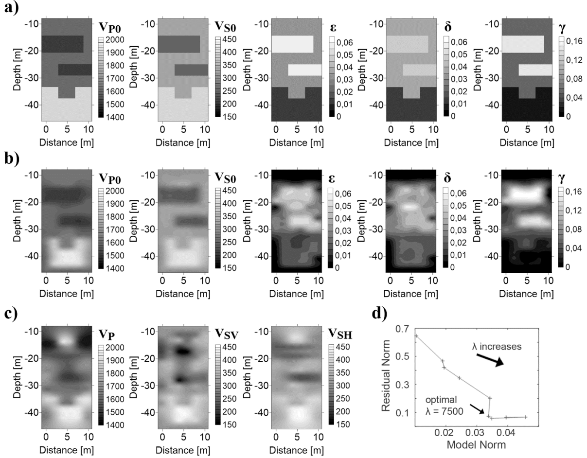
Figure 6.1: Synthetic anisotropic models (a) are reconstructed using the joint-inversion approach (b), whereby the optimal cross-gradient parameter was chosen with \lambda = 7500 (d). Separate isotropic inversions of the P-, SV- and SH-wave data are shown in (c).
