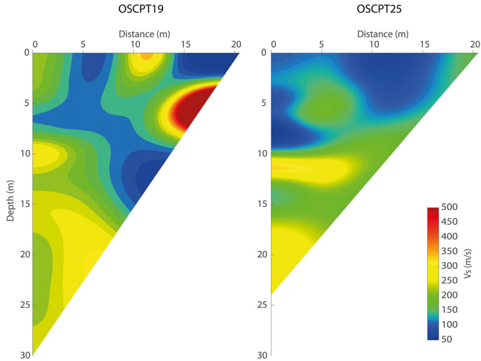
Figure 4.4: OSCPT result for SCPT19 (left) and SCPT25 (right) for station BLOP.
