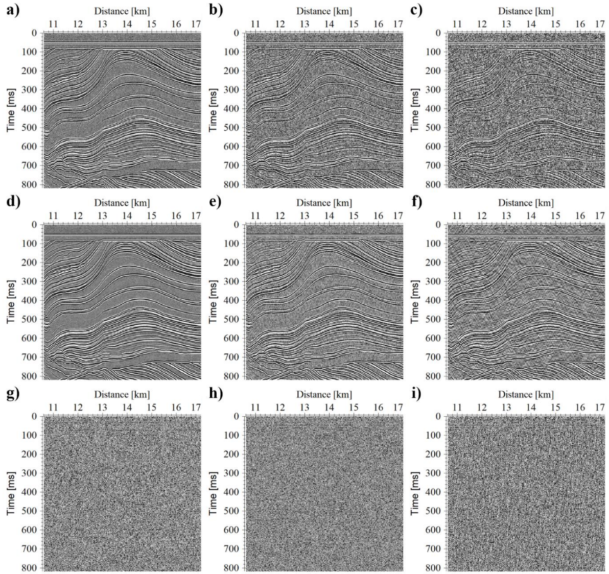
Figure 7.6: We add 20% (a), 50% (b) and 100% (c) broadband white noise to the Marmousi2 data subset (Fig. 7.5) and denoise using the curvelet transform, with 20% noise: (d), 50% noise: (e), 100% noise (f). The difference of the noisy datasets and the denoised datasets are shown in (g) to (i). The corresponding frequency-wavenumber domains are shown in Fig. 7.8.
