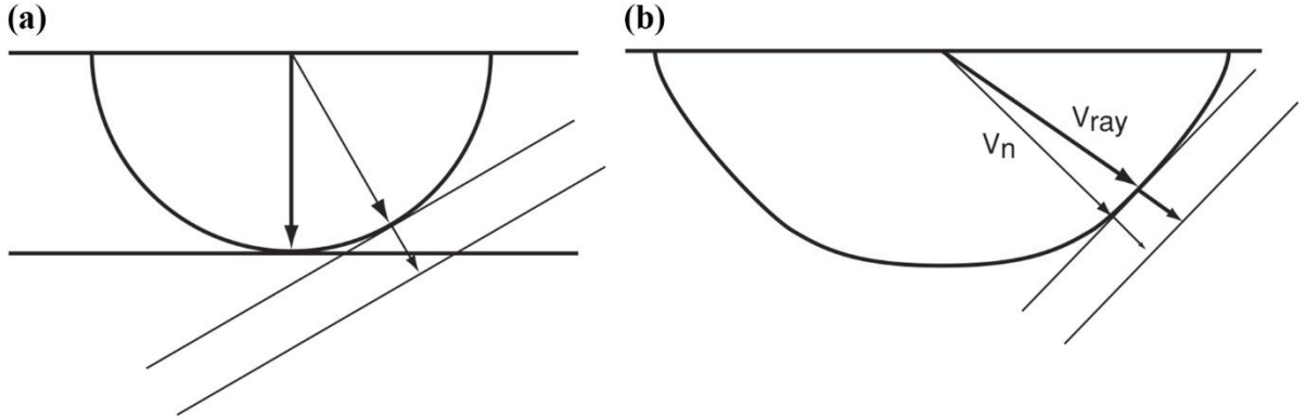
Figure 2.5: The velocity of the wavefront ( V_n ) is different from the velocity of the raypath ( V_{ray} ) for an anisotropic medium (b). For an isotropic medium (a), the two velocities are the same. (Helbig and Thomsen, 2005).
