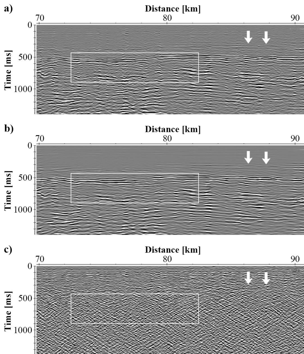
Figure 7.12: Improvements to interpretation after curvelet denoising applied to Line 2. The continuity of the reflections is enhanced after curvelet denoising (b), compared to the original stacked data (a). The difference between the original data and the denoised data is shown in (c). Attribute analysis of the data in the white box is shown in Fig. 7.14 (a) and (b).
