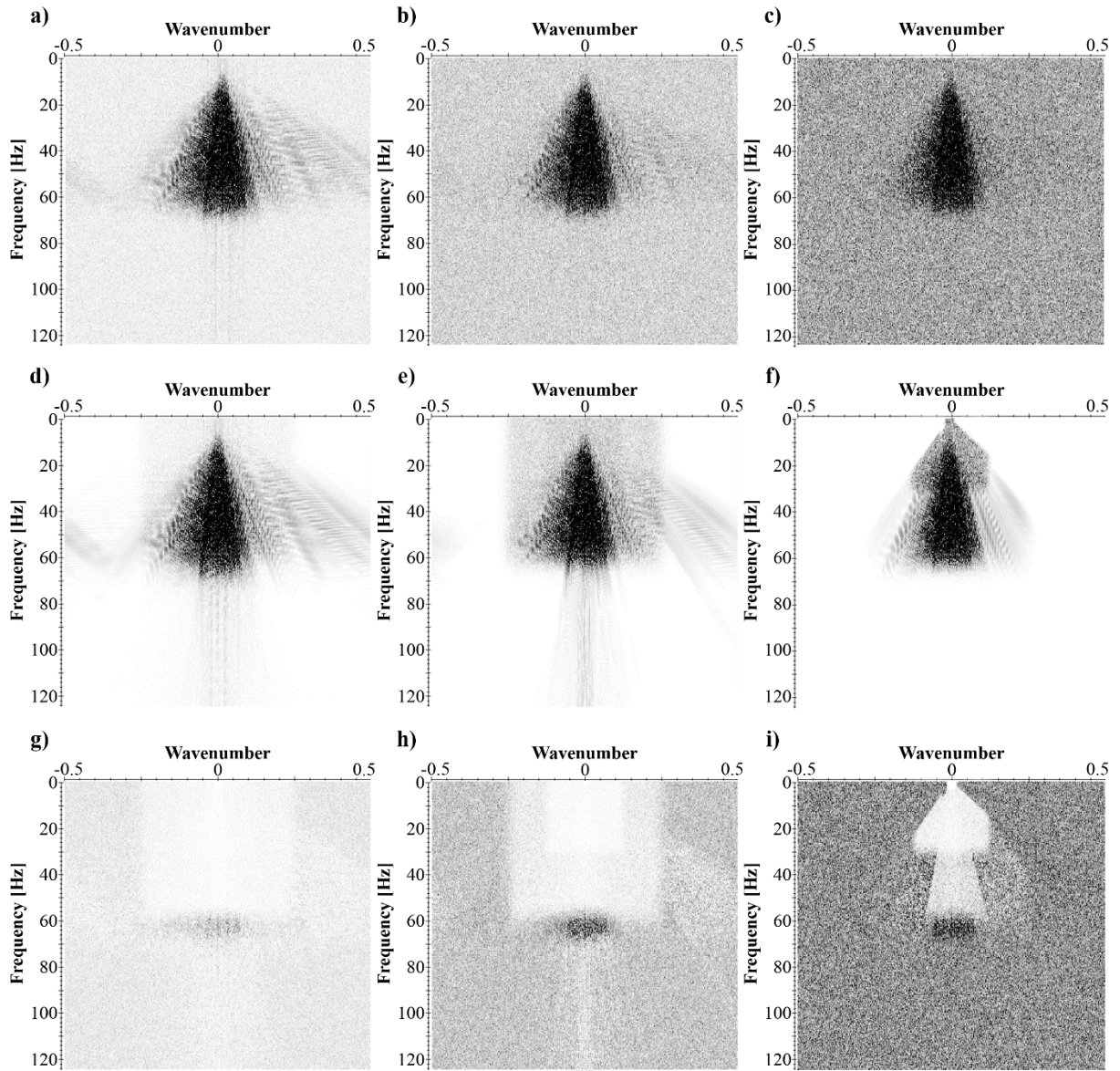
Figure 7.8: The frequency-wavenumber domains corresponding to the curvelet denoising applied to the Marmousi2 subset with added broadband white noise (Fig. 7.6).
