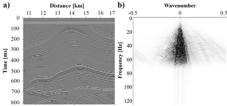
Figure 7.5: We use a subset of the Marmousi2 model (Martin et al., 2006) (a) with the frequency-wavenumber domain (b) is used to illustrate our curvelet denoising scheme.
