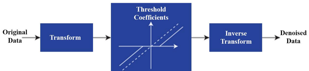
Figure 2.14: Denoising procedure using curvelet thresholding (modified after Hennenfent and Herrmann, 2006).
