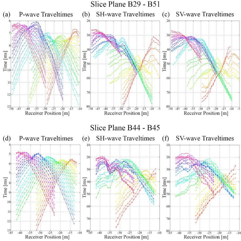
Figure 5.3: SV-, SH- and P-wave traveltimes of the SAFIRA research site sorted by receiver depth for the two slice planes B29-B51 (a-c) and B44-B45 (d-f). SH-wave and P-wave traveltimes were determined from a horizontally polarising S-wave source and the SV-waves were determined from a vertically polarising S-wave source.
