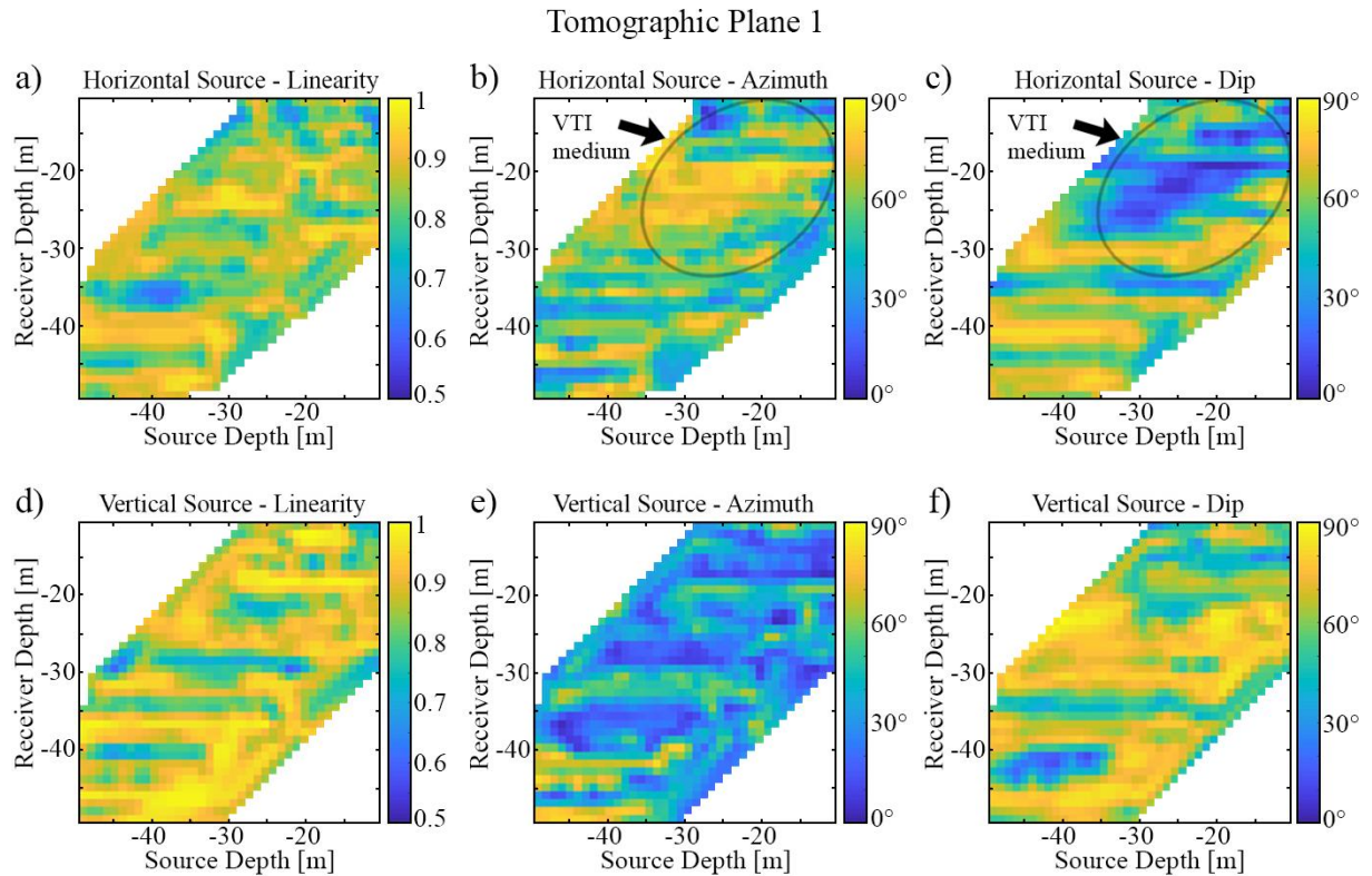
Figure 6.5: S-wave polarization is shown for the horizontally (a-c) and vertically polarized source (d-f). The linearity, azimuth and dip is shown as a function of the receiver and source depth for tomographic Plane 1, between boreholes B29 and B51.
