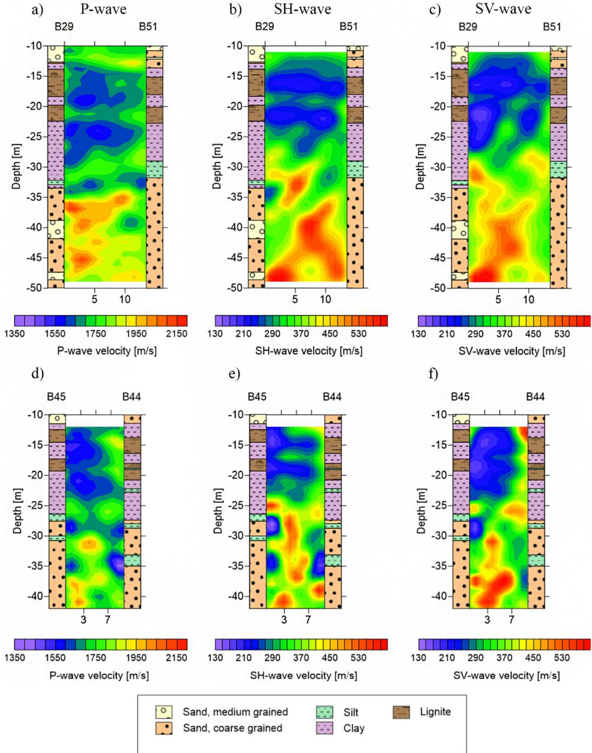
Figure 5.4: Individually inverted P-, SH- and SV-wave tomograms between boreholes B29 and B51 (a-c) and between boreholes B44 and B45 (d-f) at the SAFIRA research site. The SH- and SV-wave tomograms (b, c, e, f) exhibit artefacts and correlate less with the borehole logs than the more accurate P-wave tomograms (a, d).
