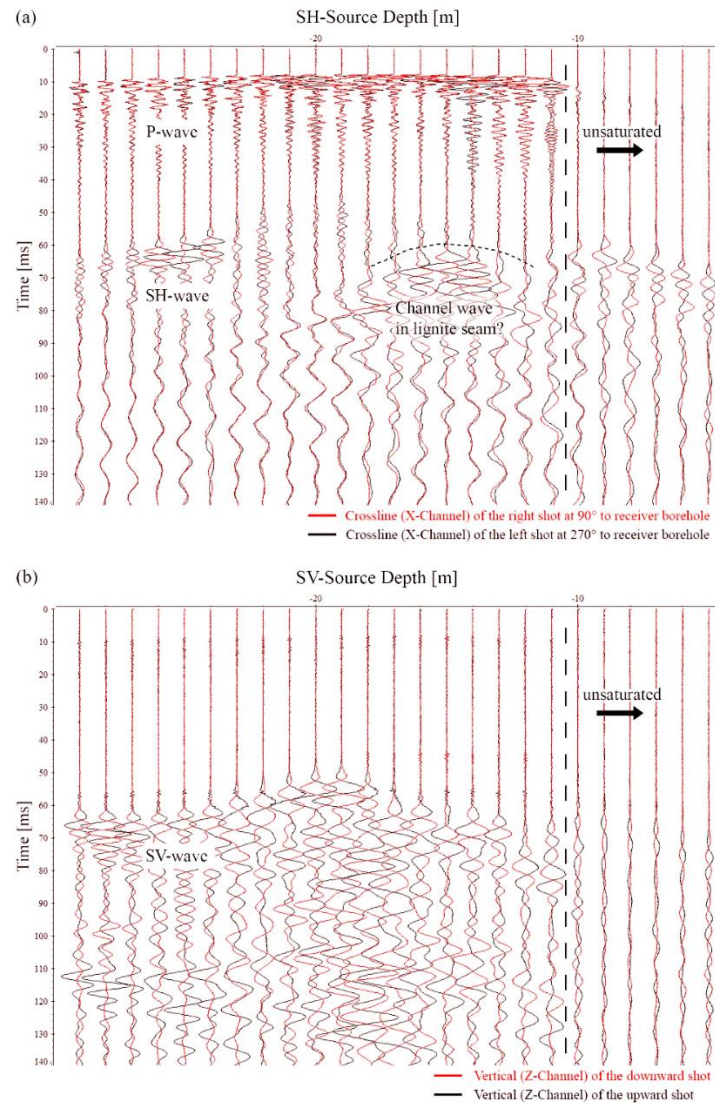
Figure 5.2: Example of a raw receiver gather for tomographic slice plane B29-B51 at 18 m depth of the horizontally-polarising S-wave source (a) and the vertically-polarising S-wave source (b) at the SAFIRA site. For the SH-wave source (a), the horizontal channel perpendicular (90°) to the source borehole is shown for the two opposing strike directions (90° and 270° to the receiver borehole). Both SH-wave and P-wave are clearly visible. For the SV-wave source (b), the vertical channel is shown for the two opposing strike directions up and down. The SV-wave is clearly distinguishable.
