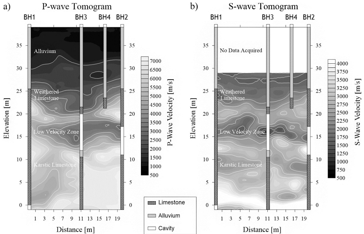
Figure 3.2: Tomographic inversions for the P-wave (a) and the S-wave traveltimes (b), showing a good correlation with the boreholes.
