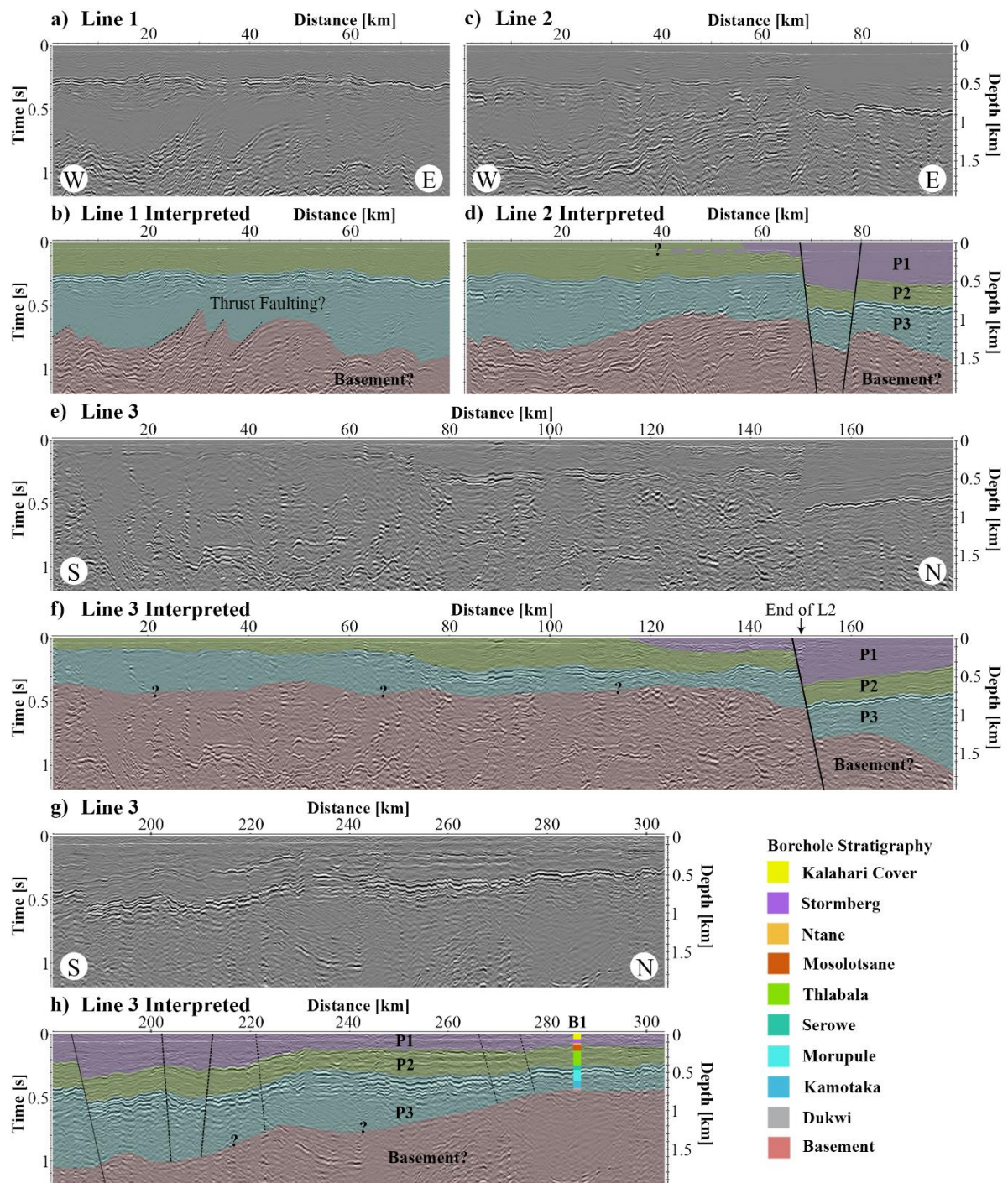
Figure 7.15: Stacked and denoised seismic sections for Lines 1 (a), 2 (c), and 3 (e, g) are shown, as well as the corresponding interpretations (b, d, f, h). The interpreted seismic sections comprise three distinct reflections, thereby enabling the division of the sections into three different sedimentological packages (P1, P2, P3) and underlying basement. Verified faults are indicated by a bold line and non-verified faults by a dotted line.
