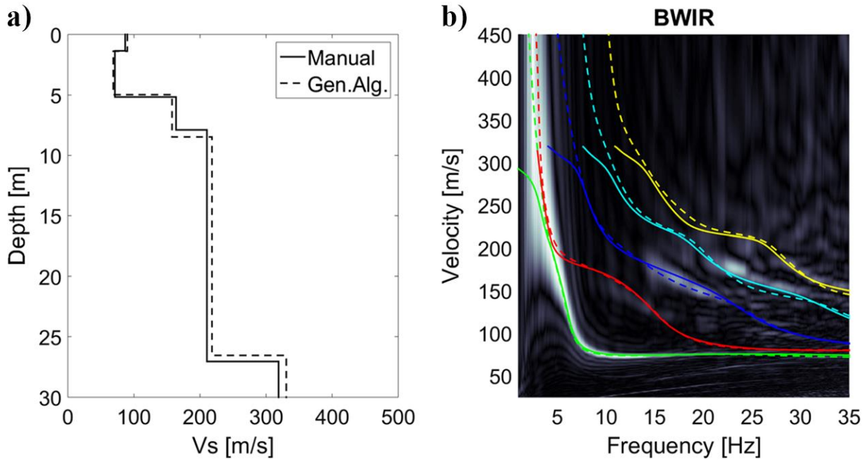
Figure 4.8: MASW result for station BWIR. V_s profiles from the manual optimisation (solid line) and the genetic algorithm (dashed line) are shown in (a). Dispersion plot showing the energy in the velocity-frequency domain in grey scale and the theoretical dispersion curves for the V_s profiles of the left panel for the manual optimisation (solid line) and the genetic algorithm (dashed line), shown in (b). The fundamental mode is shown in green; the higher modes in red, blue, cyan and yellow.
