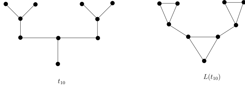
Figure 2.6: t_{10} and L(t_{10}) .
