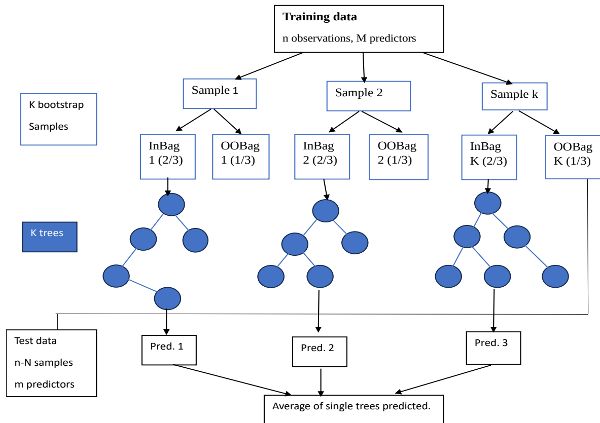
Figure 3.4: Random Forest decision trees overview, adapted from Rodriguez-Galiano et al. (2016).
