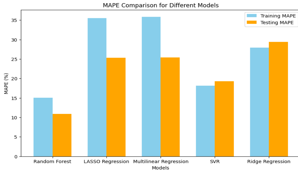
Figure 4.3: MAPE comparison for different machine learning models
