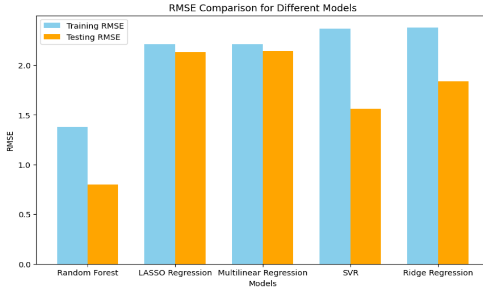
Figure 4.2: RMSE comparison for different machine learning models.
