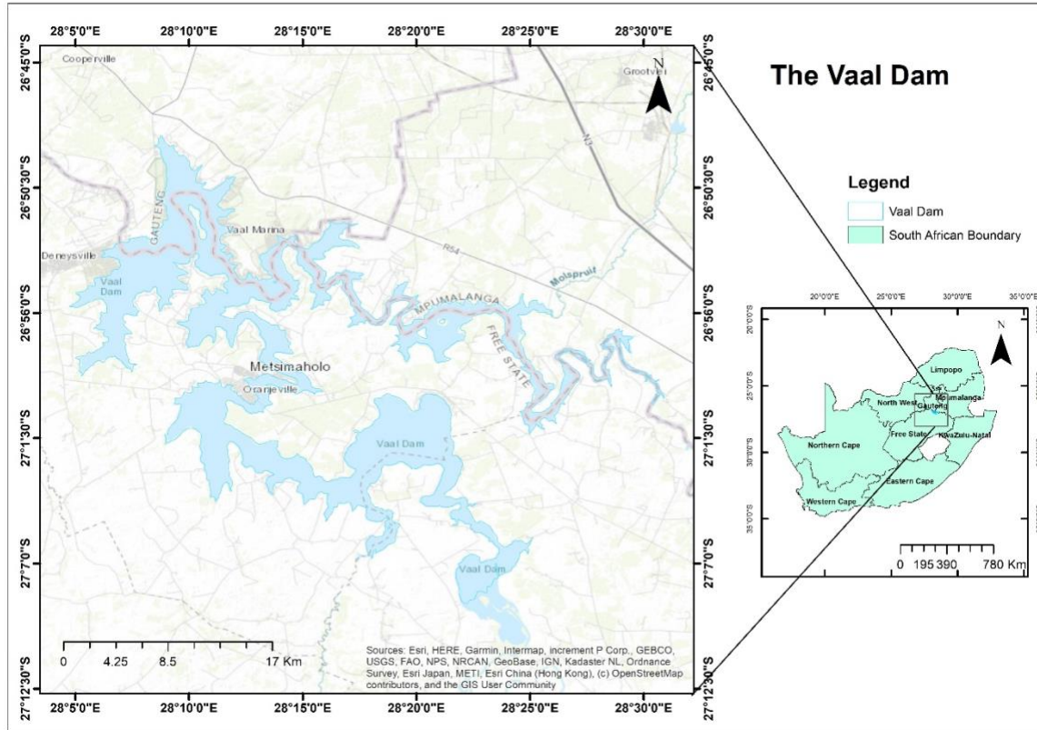
Figure 3.2: Map indicating the Vaal Dam study site.
