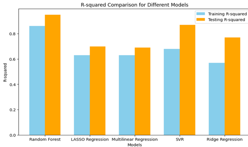
Figure 4.1: R-squared comparison for different machine learning models.
