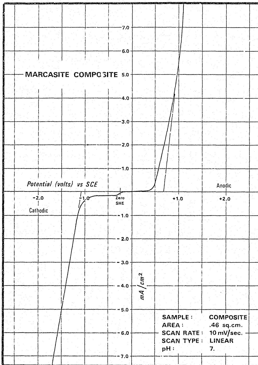
Fig. 3.5. Composite of the marcassite current-voltage curves. Area is given as the average area.
