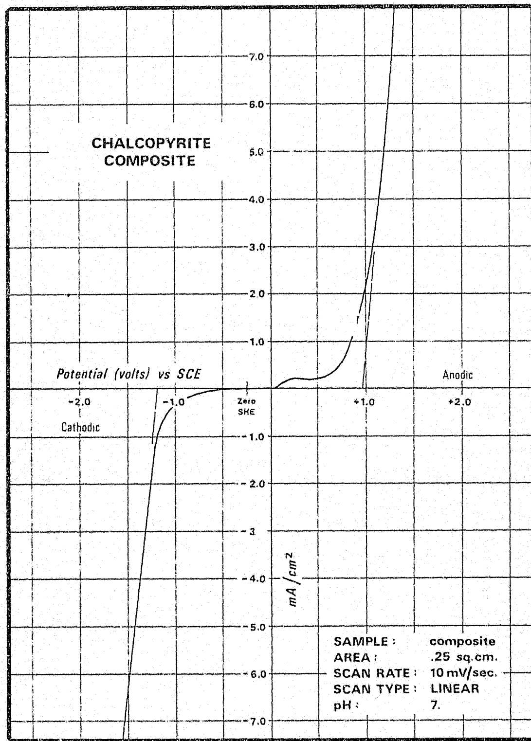
Fig. 3.7. Composite of the chalcopryrite current-voltage curves. Area is given as the average area.
