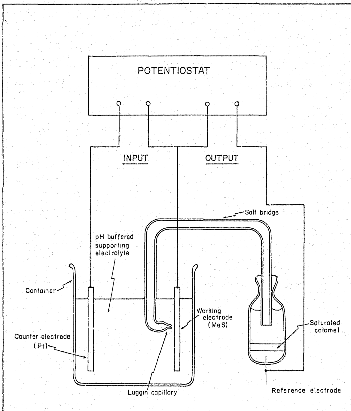
Fig. 2.1. Schematic representation of an electrochemical cell designed for experimental observation of interfacial phenomena.
