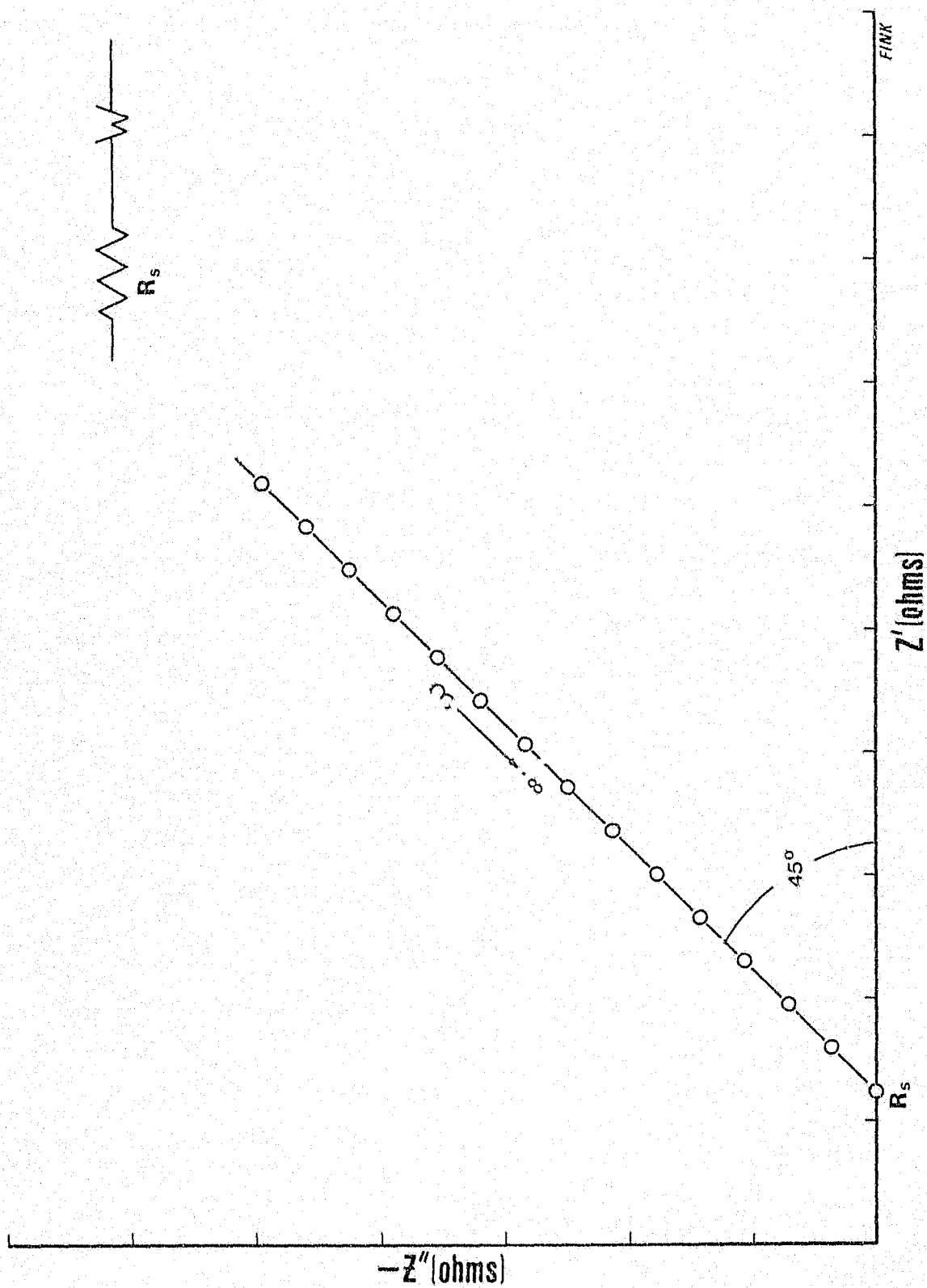
Fig. 4.8. Complex plane plot of a resistor in series with the Warburg impedance.
