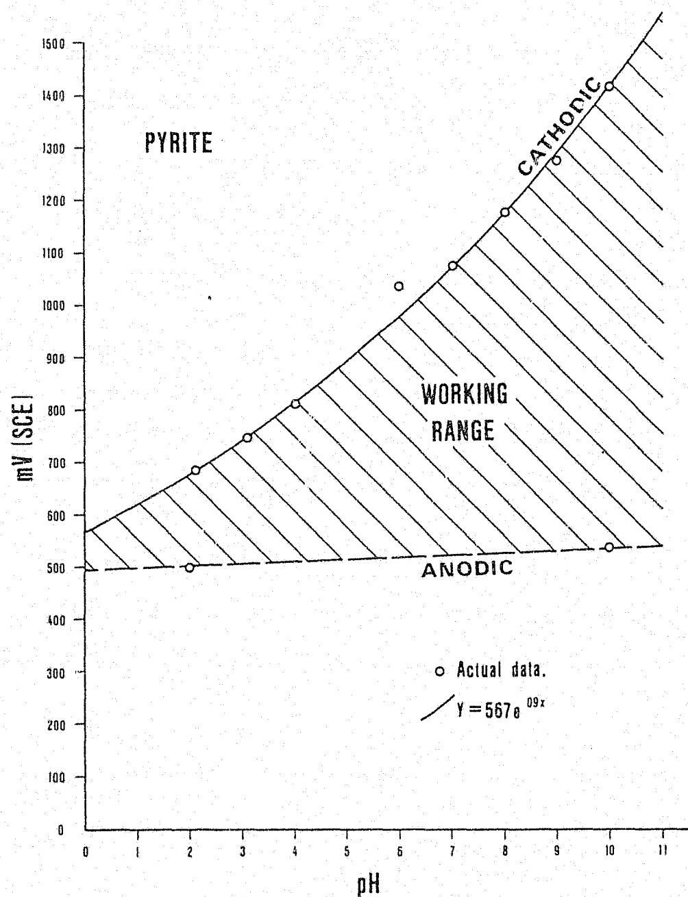
Fig. 3.4. Plot of anodic and cathodic limiting potentials for pyrite. Data are from Fig. 3.3.
