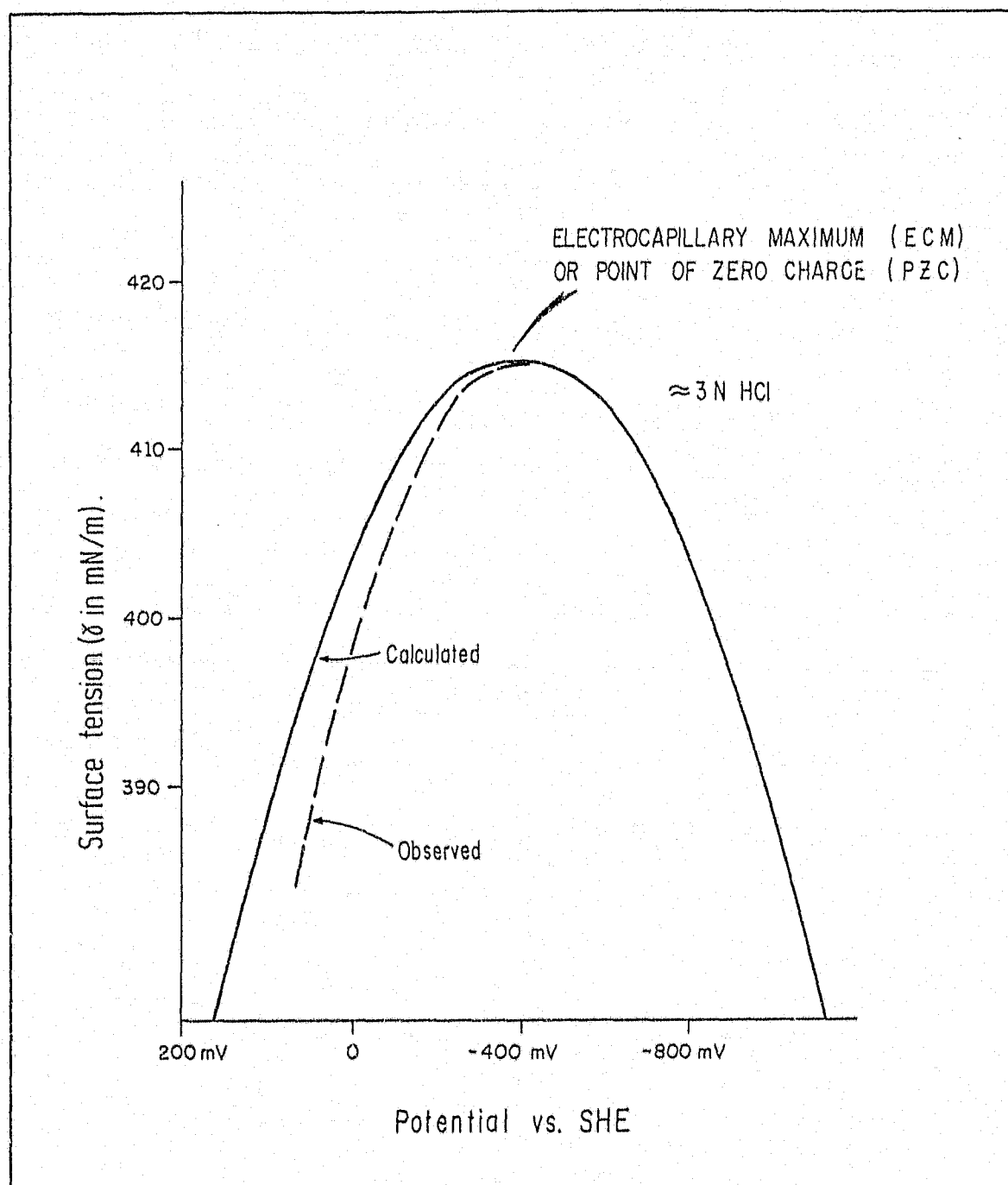
Fig. 2.5. Comparison of ideal parabola with observed electrocapillary measurements on a mercury electrode.
