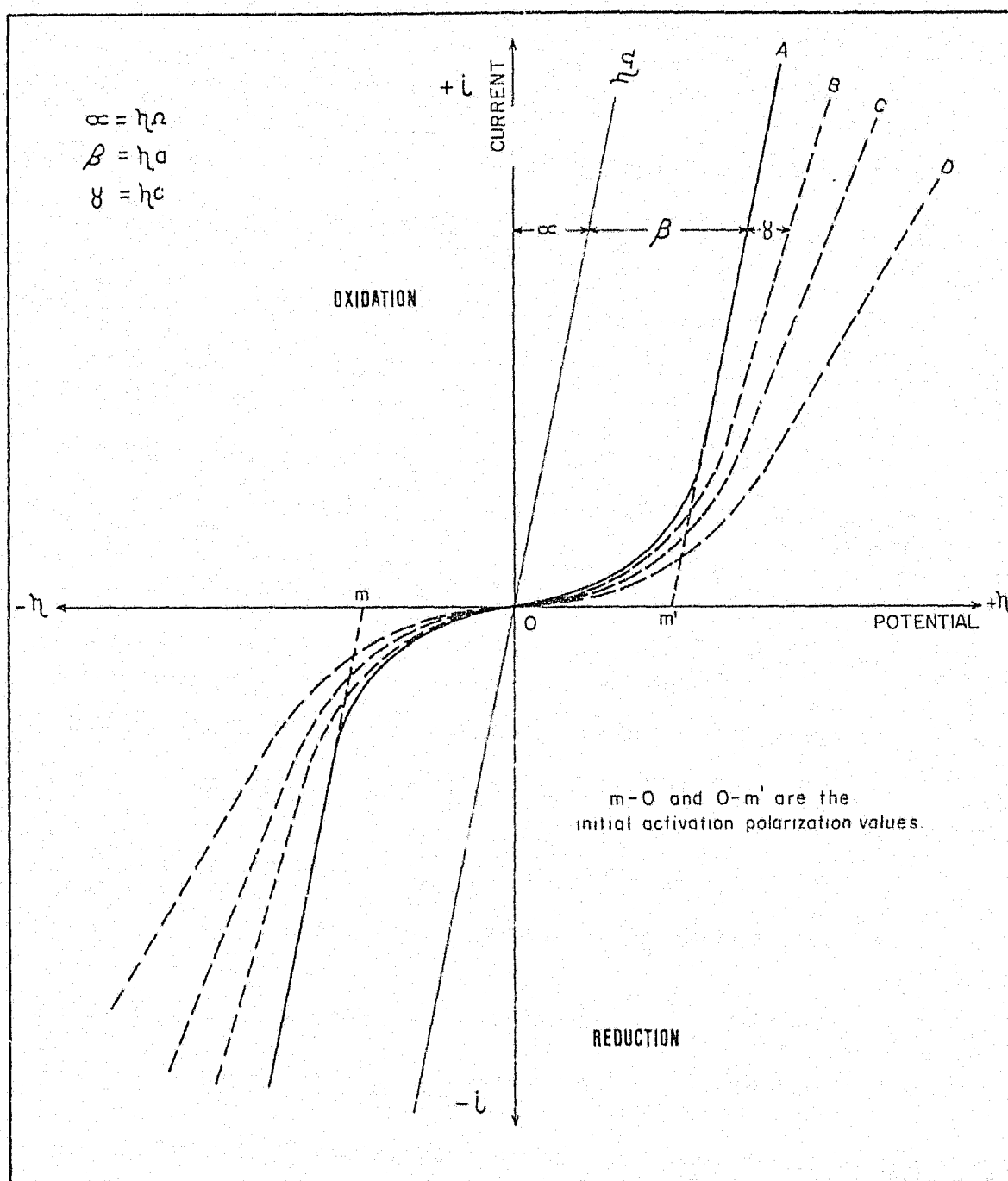
Fig. 2.6. Schematic current-voltage curves for a cell with identical irreversible electrodes. A, B, C and D represent instantaneous initial values after increasing times of current flow, \eta_\Omega is the ohmic polarisation curve and \alpha + \beta + \gamma is the total polarisation at current density i .
