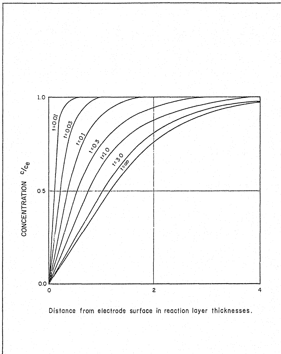
Fig. 2.7. The concentration of oxidant normalized to the equilibrium value plotted against the distance from the electrode surface in reaction layer thicknesses where t represents various elapsed times of electrolysis. Due to convection, the reaction layer thickness is finite for very large t .
