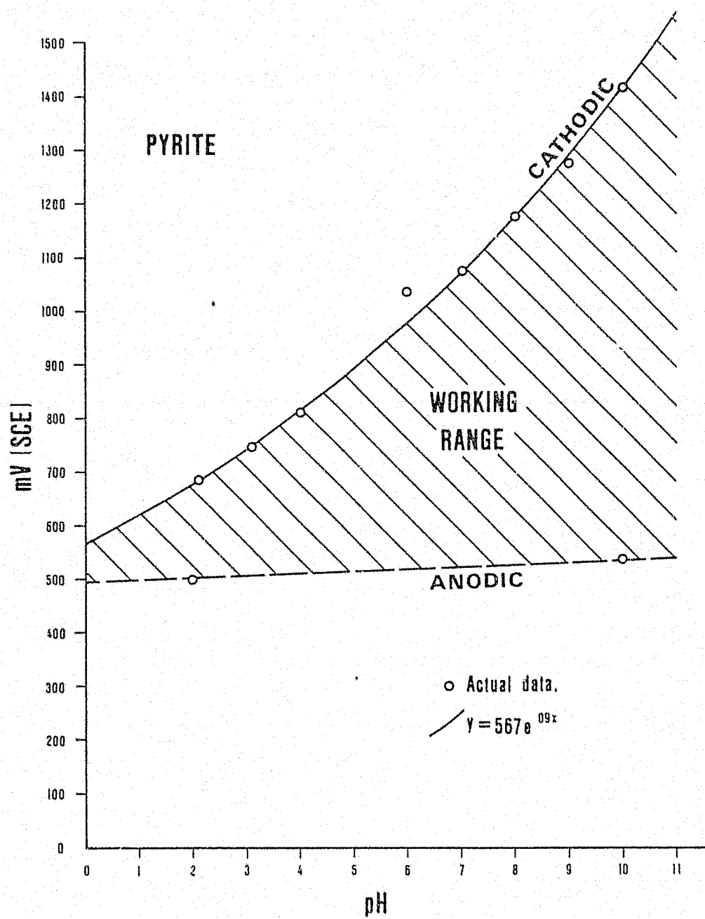
Fig. 3.4. Pl. of anodic and cathodic limiting potentials for pyrite. Data are from Fig. 3.3.
