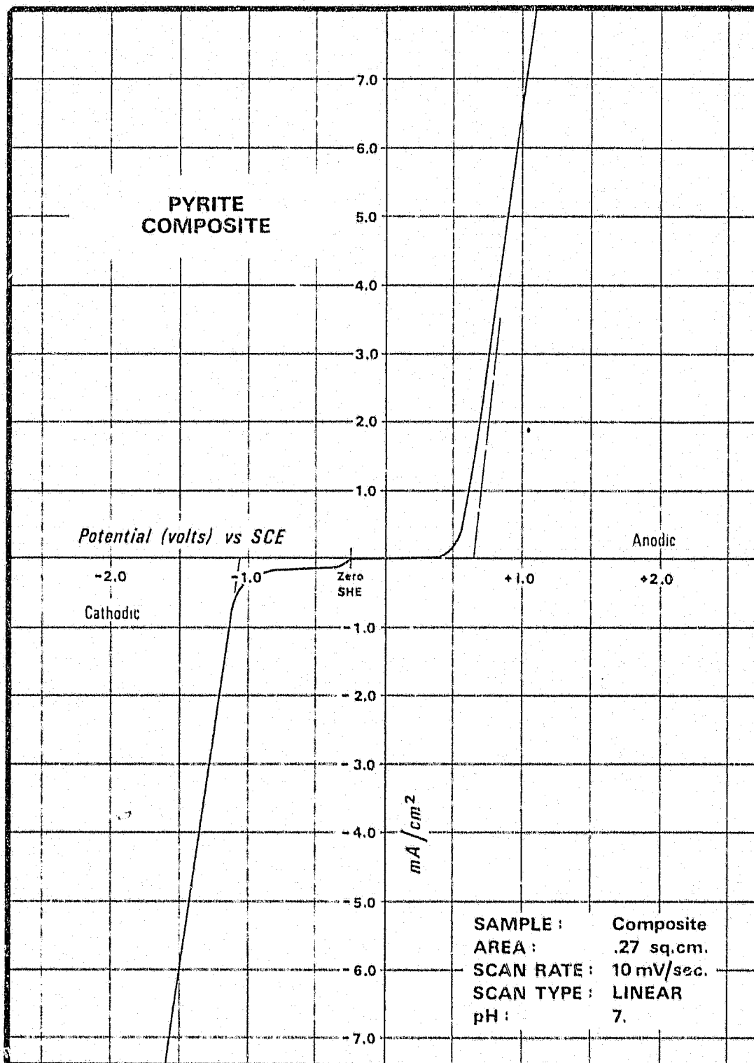
Fig. 3.2. Composite of the pyrite current-voltage curves. Area is given as the average area.
