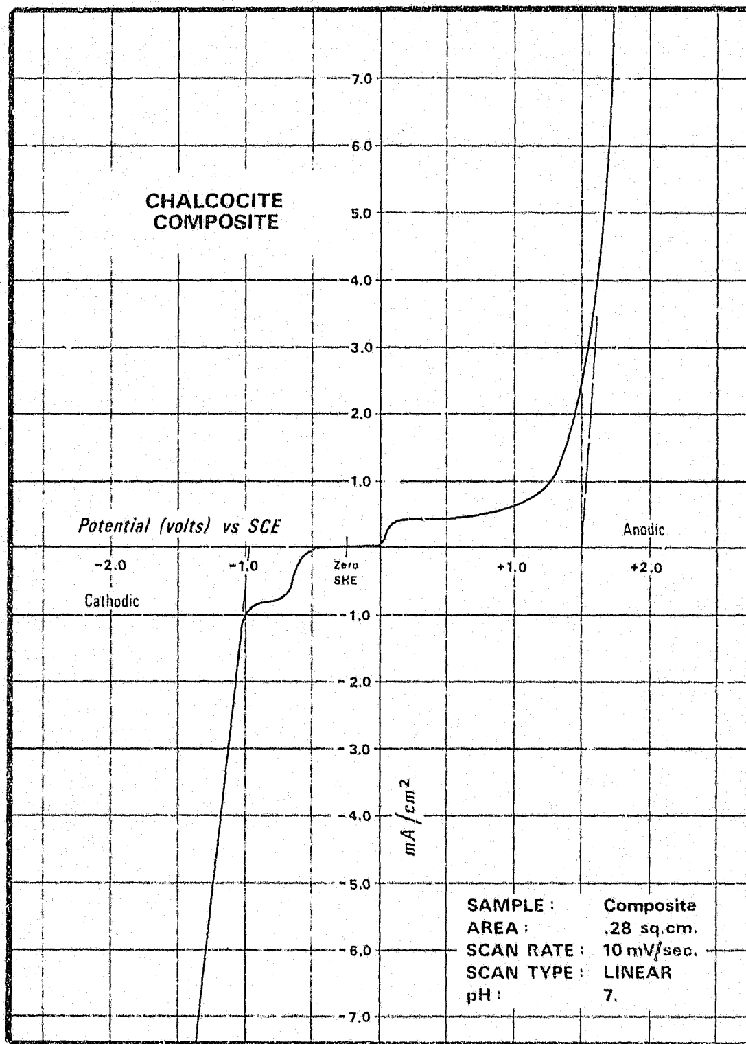
Fig. 3.8. Composite of the chalcocite current-voltage curves. Area is given as the average area.
