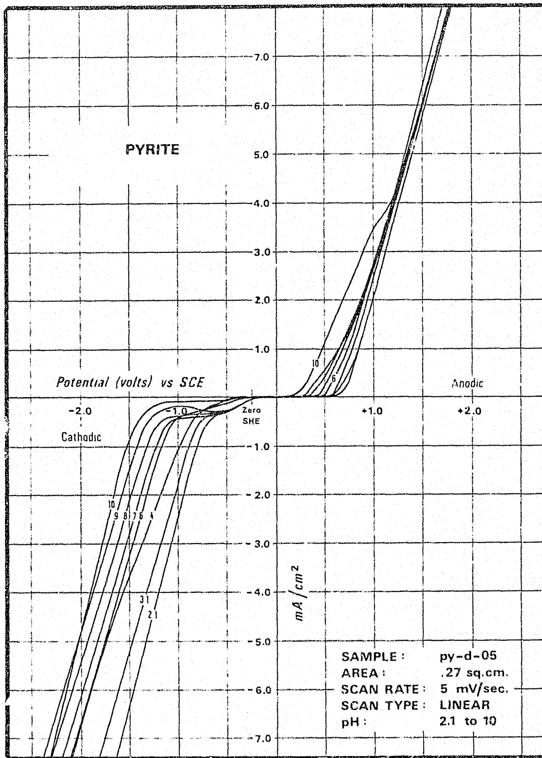
Fig. 3.3. Pyrite current-voltage curves for multiple pH's.
