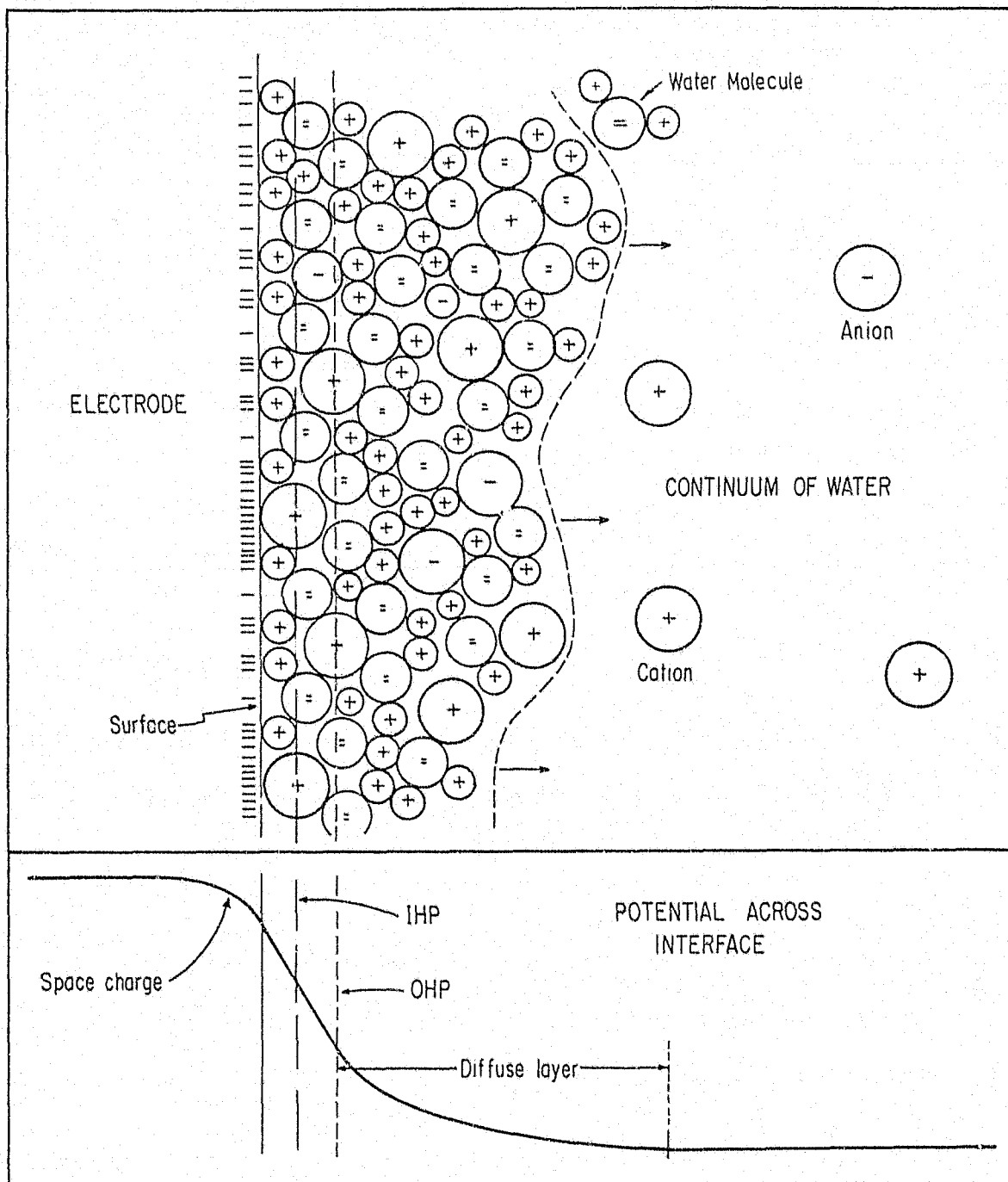
Fig. 2.4. A diagrammatic depiction of the distribution of cations, anions and water molecules at a hypothetical interface. The lower figure is a plot of the relative potential across the interface.
