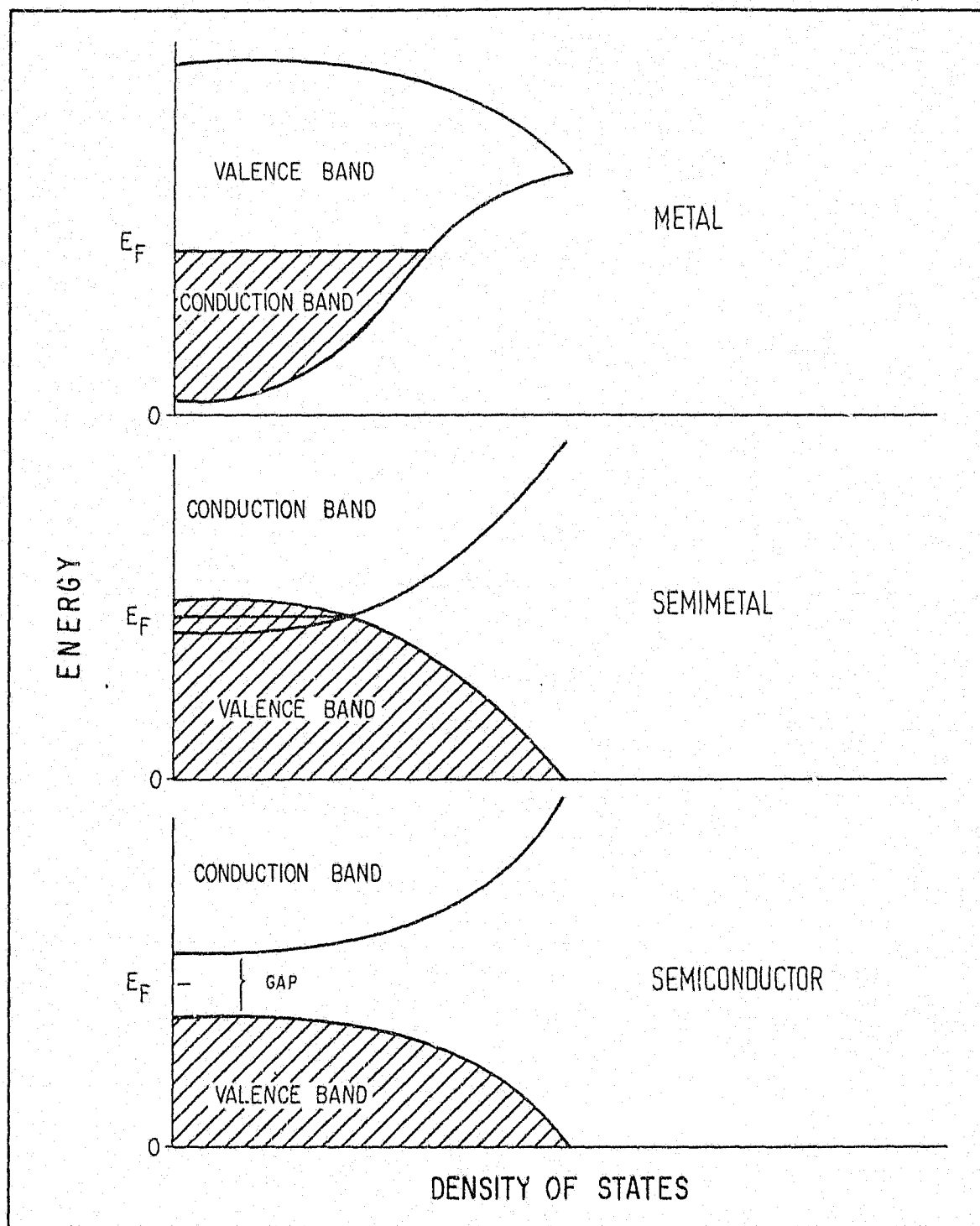
Fig. 2.3. Density of states (abscissa) versus energy (ordinate) for three types of solids.
