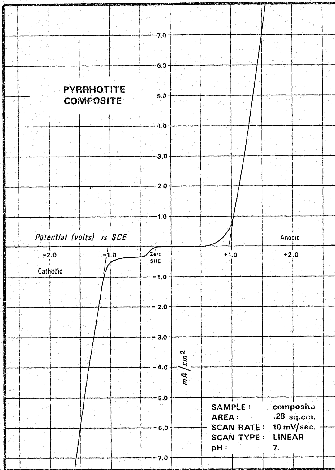
Fig. 3.6. Composite of the pyrrhotite current-voltage curves. Area is given as the average area.
