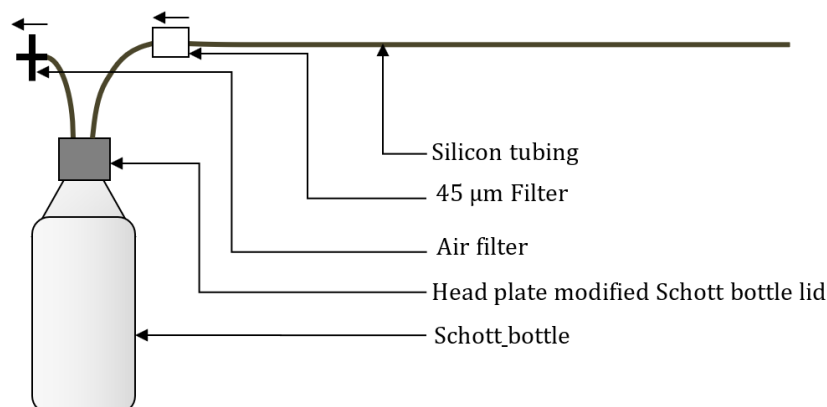
Figure 23: Diagrammatic depiction of the autoclavable filtration rig.
