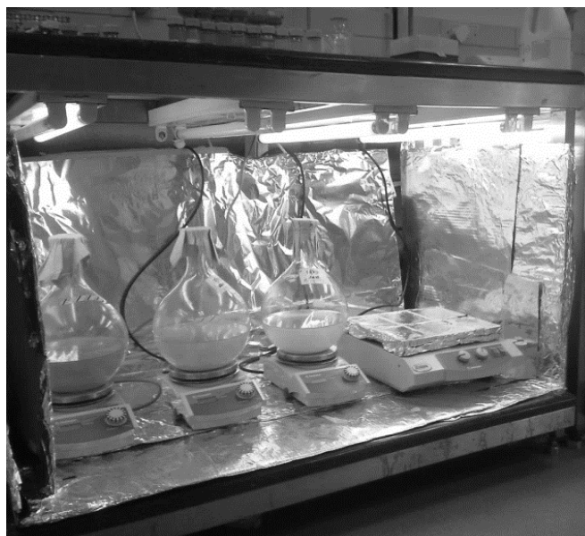
Figure 16: Neon light and magnetic stirrer setup for the flask study, under the work benches.
