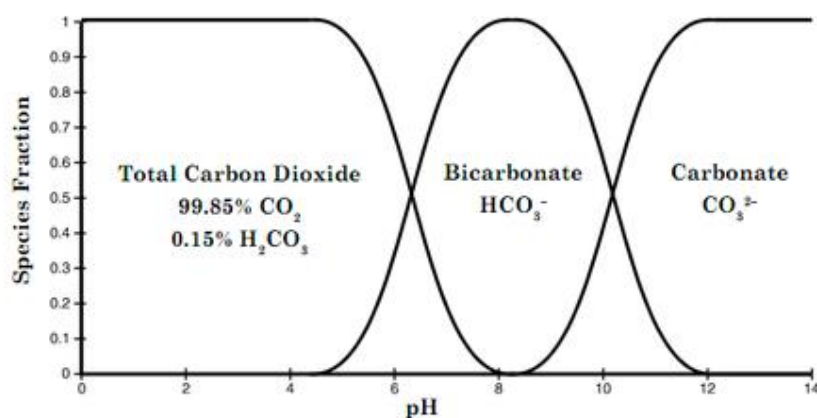
Figure 14: Fluctuation of CO 2 , HCO 3 - and CO 3 2- concentrations vs pH (Wojtowicz, 2001).
