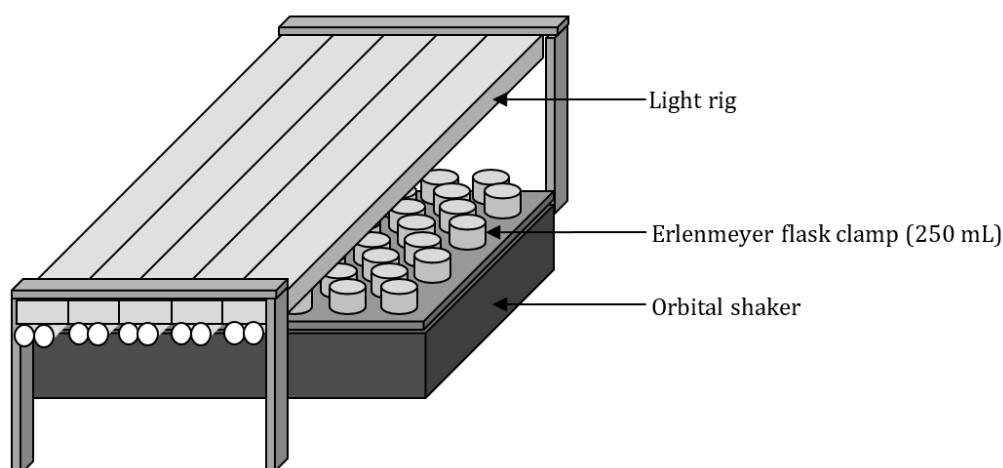
Figure 24: Diagrammatic depiction of the incubation setup including the light rigs and orbital shaker.
