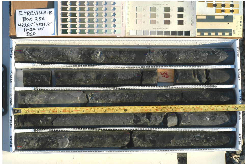
A) Box 256, box depth = 1471.12 to 1474.07 m and B) Box 257, box depth = 1474.07 to 1476.76 m.
