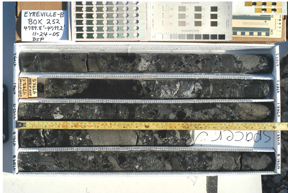
A) Box 252, box depth = 1459.93 to 1462.80 m and B) Box 253, box depth = 1462.80 to 1465.54 m.
