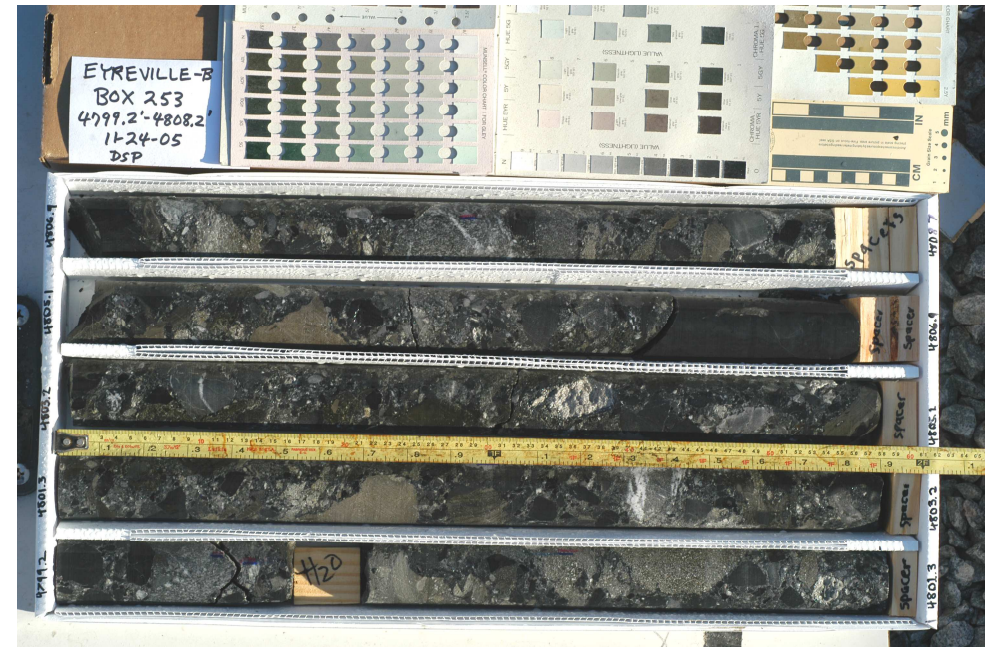
A) Box 252, box depth = 1459.93 to 1462.80 m and B) Box 253, box depth = 1462.80 to 1465.54 m.
