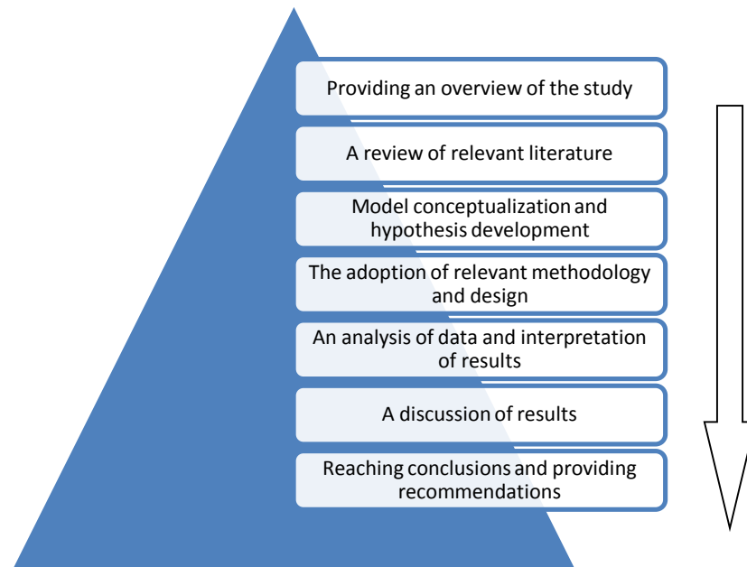
Figure 1: Research flow
