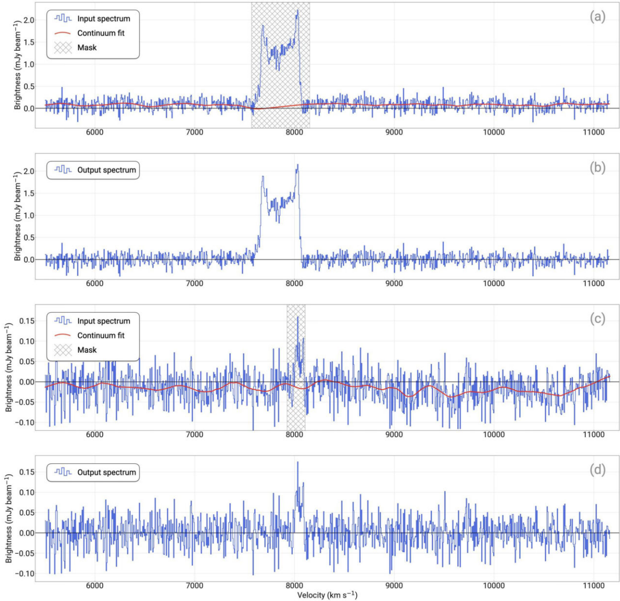
Figure 2. Two examples (upper and low pairs of panels) of the image-domain continuum subtraction at work on two galaxies with differing H I masses. Each pair of panels shows a sightline (through a subset of channels) that intersects the H I discs of the two galaxies, extracted from the robust 0.5 L2 cube. The region that is automatically masked by the continuum subtraction procedure is shown by the hatched area. The upper panel for each pair (panels a and c) shows the input spectrum, with the continuum estimation shown by the continuous red line. The lower panels in each pair (b and d) show the output spectra following continuum subtraction. Note that for clarity these spectra only show 1000 channels, approximately one eighth of the total spectral coverage of the L2 cubes. Please refer to Section 3.6 for further details.
