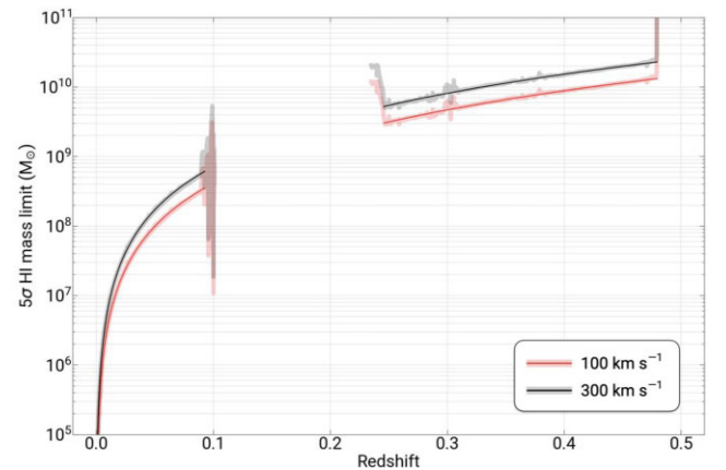
Figure 7. The estimated 5\sigma HI mass limits for the MIGHTEE-HI DR1 data, assuming boxcar line profiles with rest-frame velocity widths of 100 \text{km s}^{-1} (red) and 300 \text{km s}^{-1} (black). The lighter coloured traces exhibiting more variation are mass limits calculated using the measured sensitivity values (discussed in Section 4.2), whereas the darker continuous trace uses the median 1\sigma RMS channel noise values of 40 and 74 \mu\text{Jy beam}^{-1} for L1 and L2 respectively.
