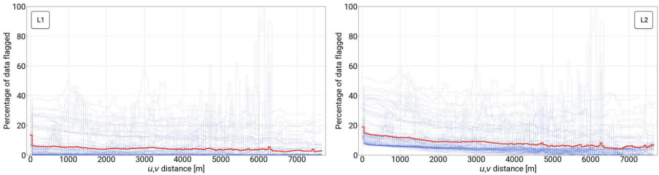
Figure A2. The flagging percentages as a function of u, v distance for the L1 (left panel) and L2 (right panel) sub-bands. The blue and red histograms represent the individual scans and the overall percentages for the COSMOS observations as a whole, as per Fig. A1. Note that for these plots the channels at the L1 and L2 band edges where the data encroach on the persistent satellite RFI bands are excluded.
