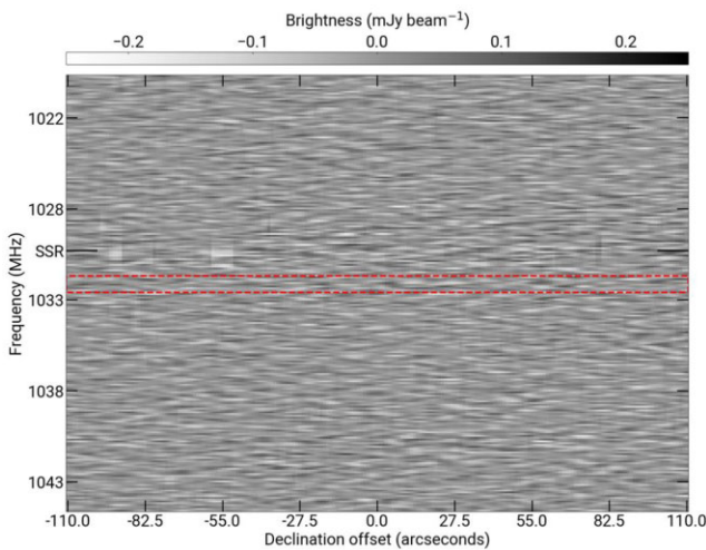
Figure 14. A frequency / declination slice through the r = 0.5 MIGHTEE-HI data, centred at RA = 10^{\text{h}}00^{\text{m}}54^{\text{s}}.83 , Dec = +02^{\circ}31'26''.2 . The frequency range is the same as that covered in Fig. 13, and the declination slice covers \pm 110 arcsec, or \pm 5 synthesized beam widths. The 1030 MHz SSR transmission is marked with the large tick mark, and the dashed lines show the reported width of the z = 0.37 line emitter.
