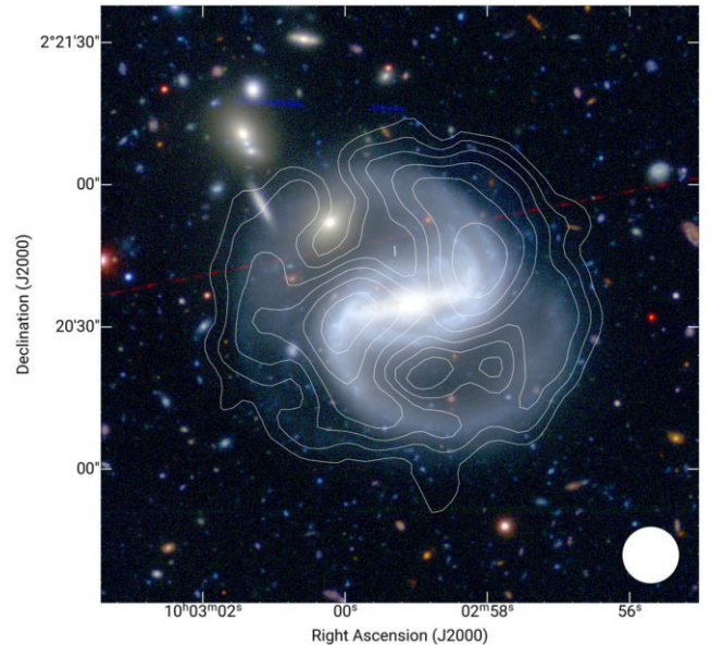
Figure 10. The robust-0 moment-0 contour map of the H I source J100259.0+022035 at z = 0.044256 , coincident with a barred spiral galaxy. The background image is a 3-colour rendering of the g , r , and i band photometric imaging from the Subaru Hyper Suprime-Cam data (Aihara et al. 2018, 2019). The contours on this figure correspond to H I column densities of (0.56, 0.94, 1.49, 2.26, 3.35, 4.88) \times 10^{20} atoms \text{cm}^{-2} . The restoring beam is shown in the lower right hand corner of the plot, with a diameter of 12 arcsec.
