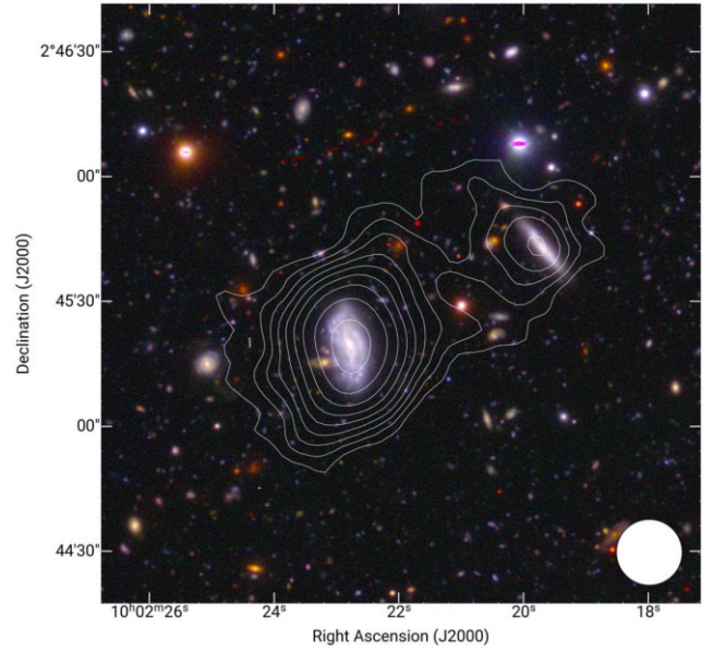
Figure 9. The robust-0.5 moment-0 contour map of the H I-detected galaxy pair J100222.8+024519 and J100219.8+024543, z = 0.072266 , overlaid on a 3-colour image from the g , r , and i bands of the Subaru Hyper Suprime-Cam data (Aihara et al. 2018, 2019). The contours on this figure correspond to H I column densities of (0.31, 0.56, 0.91, 1.4, 2.1, 3.1, 4.5, 6.35, 9.4) \times 10^{20} atoms \text{cm}^{-2} . The circle in the lower right shows the extent of the restoring beam, which has a diameter of 15'' .
