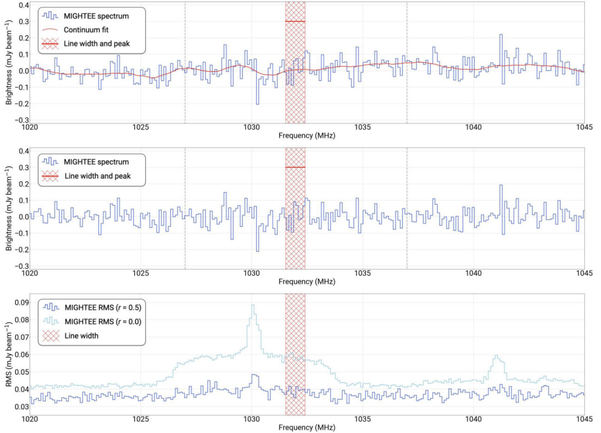
Figure 13. The upper panel shows a spectrum from the L1 ( r = 0.5 ) sub-band, extracted at the position of the z = 0.3764 HI detection from the CHILES survey reported by Fernández et al. (2016). The width (red hatched region) and peak (red horizontal bar) of the reported detection are also shown. The continuous red trace is the image-domain continuum subtraction’s estimation of the spectral baseline. The central panel shows the spectrum that results following subtraction of the estimate. The lower panel shows the RMS of the MIGHTEE data, measured over a circular aperture of 9 arcmin diameter centred on the same position for the r = 0.5 data (dark blue) as well as the r = 0.0 data (pale blue) in order to emphasize the presence of the 1030 MHz secondary surveillance radar transmissions used for aviation.
