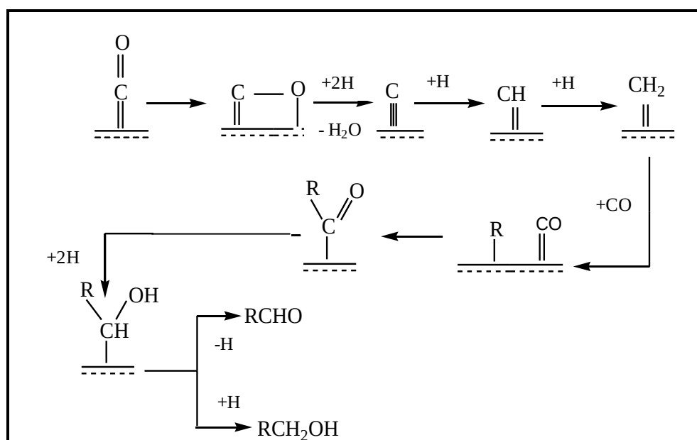
Figure 2.7: CO insertion mechanism [47].
