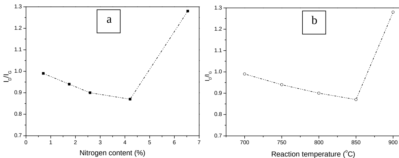
Figure 8.6: I D /I G ratio as function of (a) nitrogen content and (b) reaction temperature
