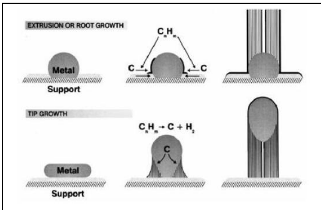
Figure 2.10: Possible carbon nanotube growth mechanism [128, 188].
