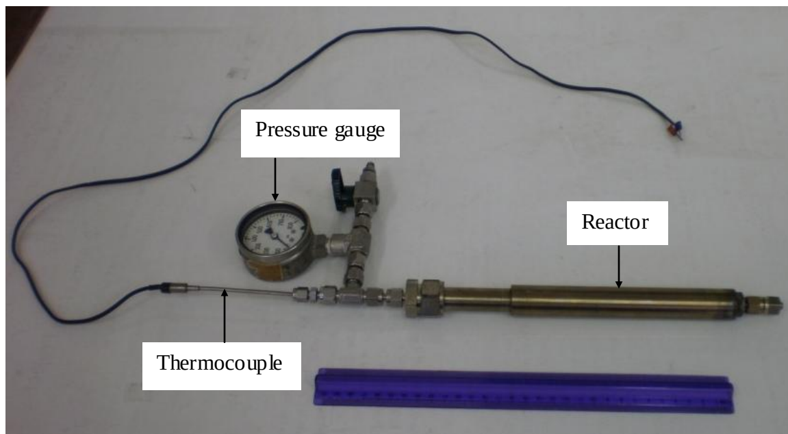
Figure 3.5: Photograph of the assembled fixed-bed micro reactor
