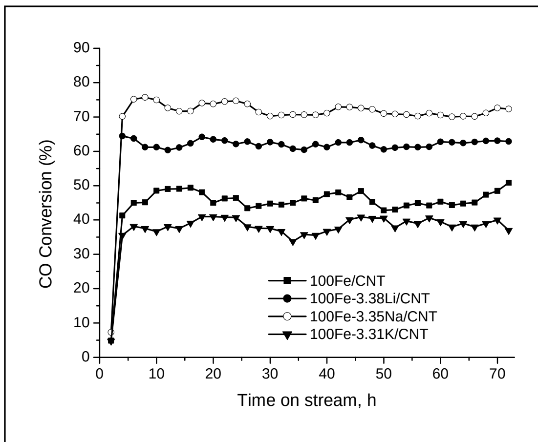
Figure 7.10: % CO conversion versus time on stream for unpromoted and alkali promoted Fe/CNT catalysts.
