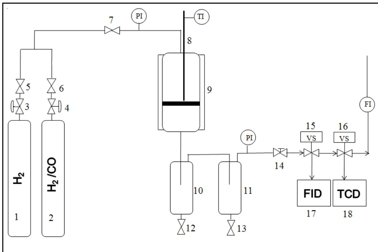
Figure 3.2: Schematic diagram of the Fischer-Tropsch single fixed-bed micro reactor system set up (not to scale)
