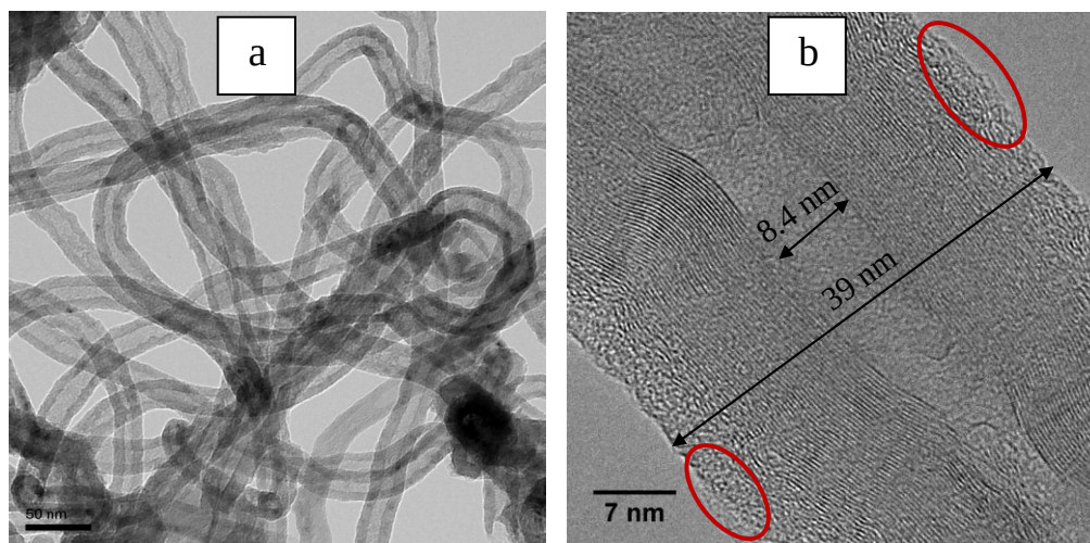
Figure 6.2: CNT-as grown: a) TEM, b) HRTEM with ovals representing amorphous carbon
