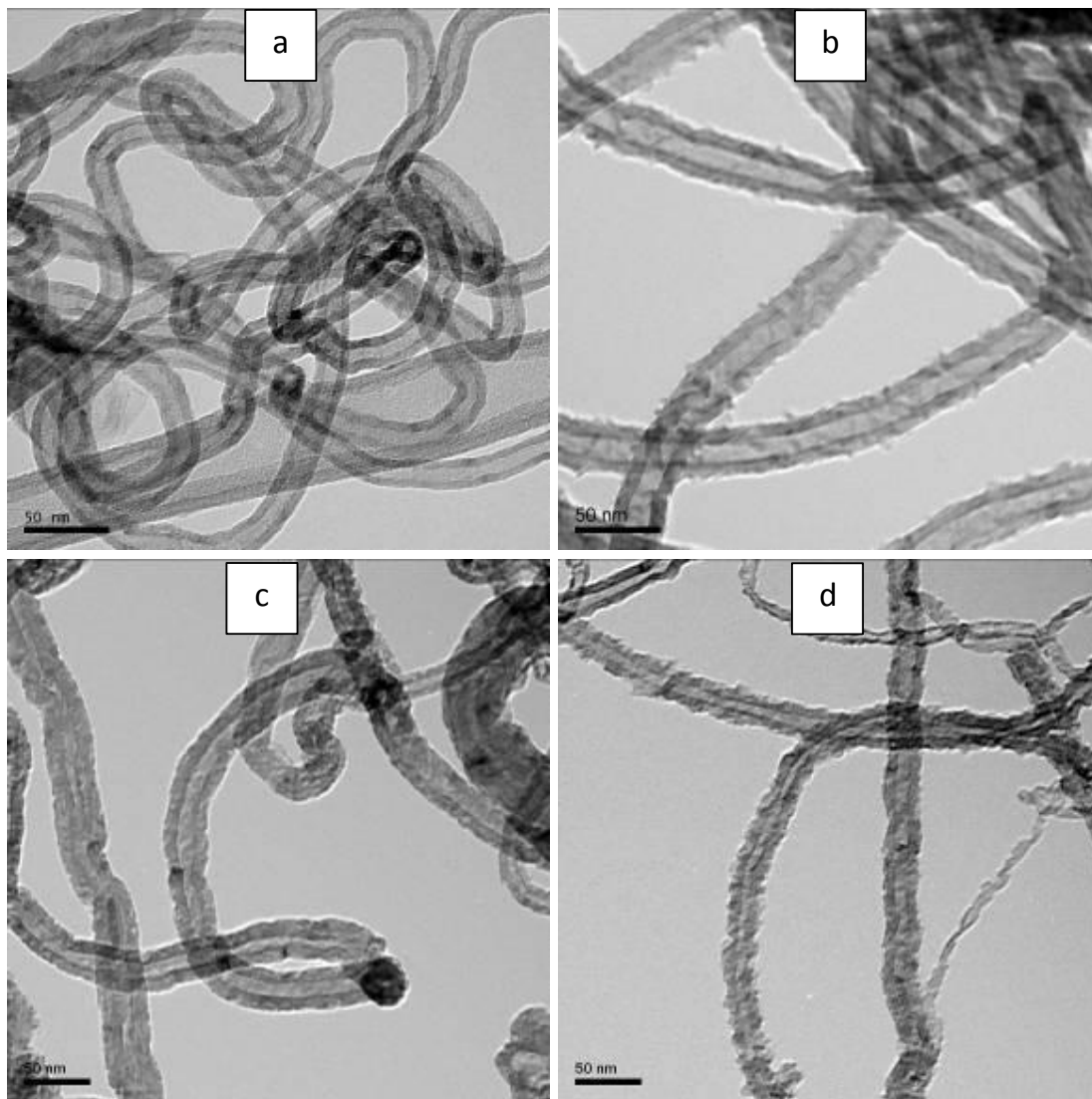
Figure 5.3: Effect of acid treatment on the texture and morphologies of CCVD synthesized CNTs: a) CNTs-30R2; b) CNT-30R6; c) CNT-55R2; d) CNT-55R6.
