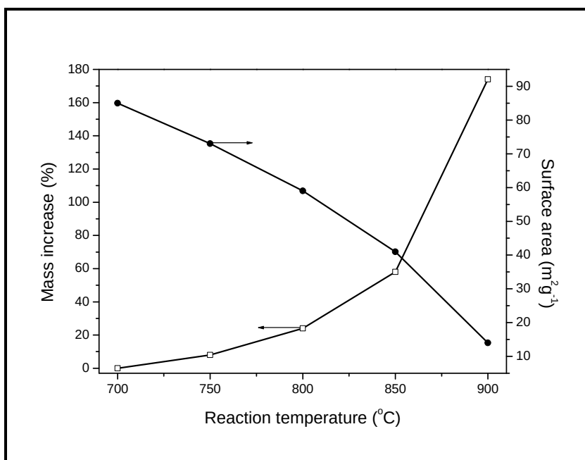
Figure 8.2: Dependence of the % mass increase and surface area in N-CNTs on reaction temperature.
