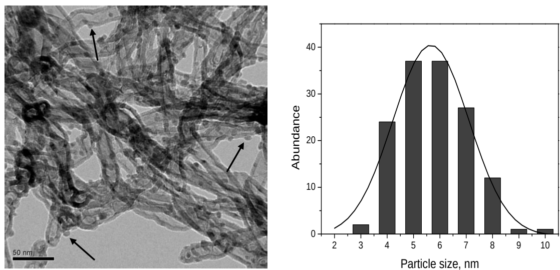
Figure 6.10: TEM image with arrows indicating the Fe particles, and Fe particle size histogram for the Fe-acac-350 catalyst.
