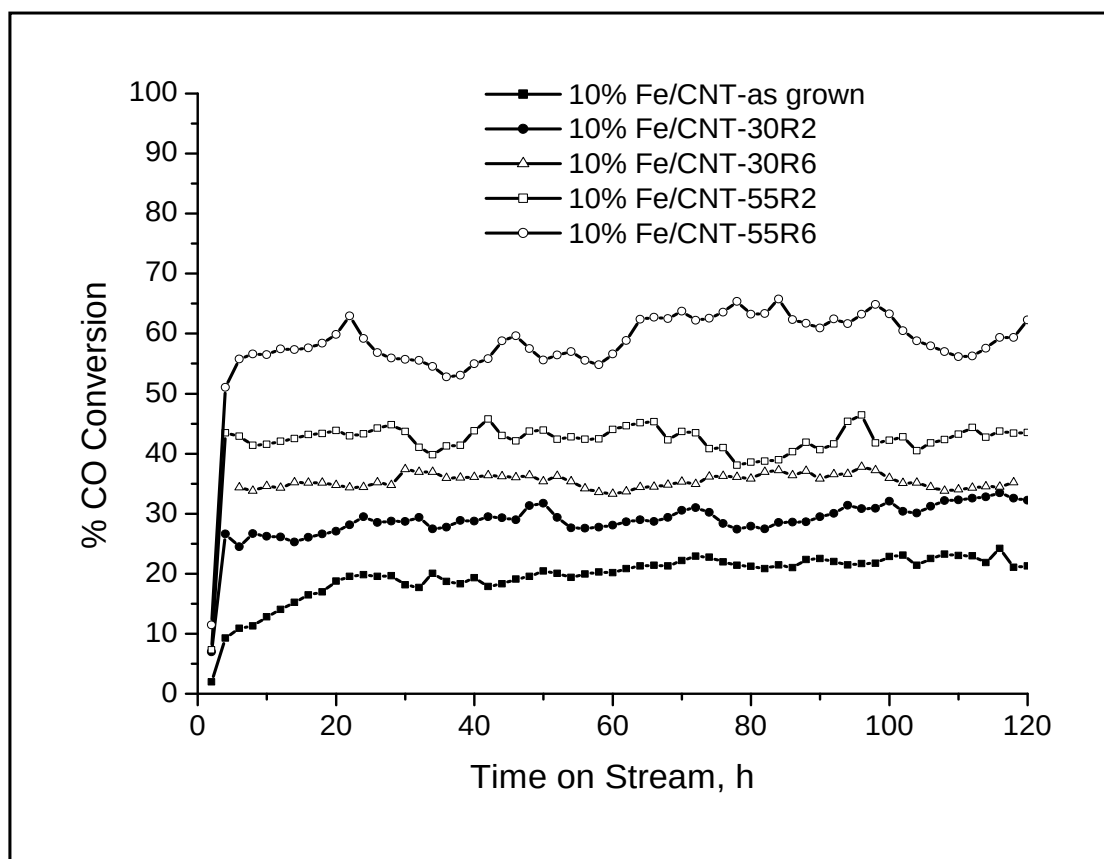
Figure 5.16: CO conversion with time on stream.
