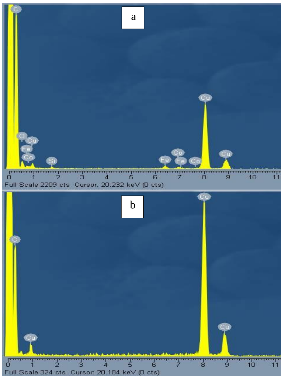
Figure 5.4: EDX spectrum of: (a) as grown CNT showing the presence of residual metal and (b) acid treated, CNT-55R6 showing that most of the residual metal particles are removed.
