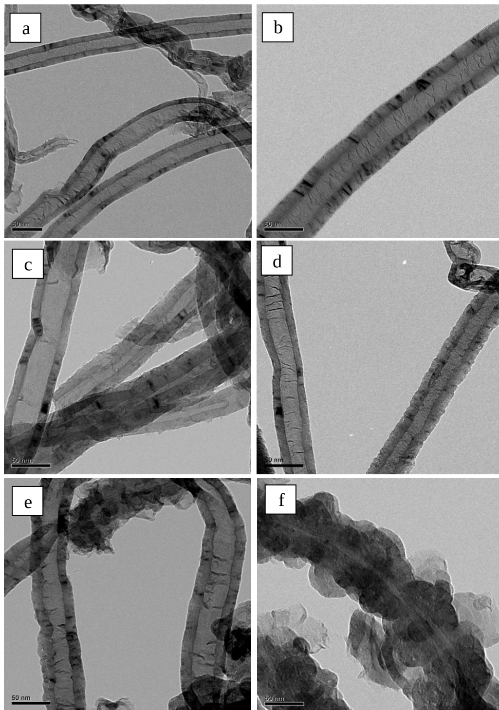
Figure 8.3: TEM images of CNTs and N-CNTs (prepared by post-doping at different temperatures): a) purified CNTs; b) N-CNT-700°C; c) N-CNT-750°C; d) N-CNT-800°C; e) N-CNT-850°C; f) N-CNT-900°C (Duration of deposition in all cases is 2 h)
