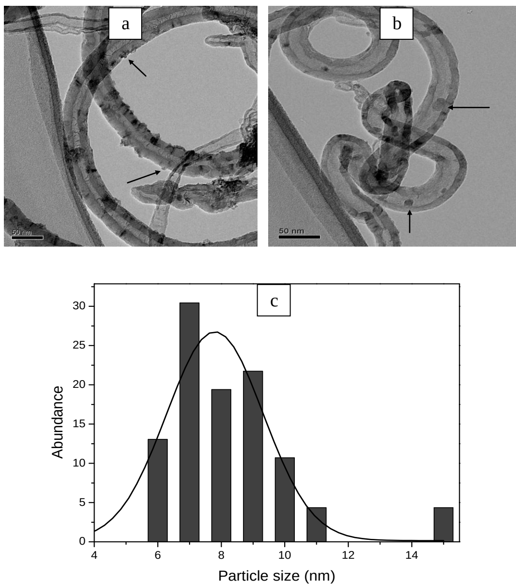
Figure 8.8: (a) and (b) TEM images and (c) Fe particle size histogram of the Fe/N-CNT-750-55R2 catalyst, (arrows on the TEM images show iron particles)
