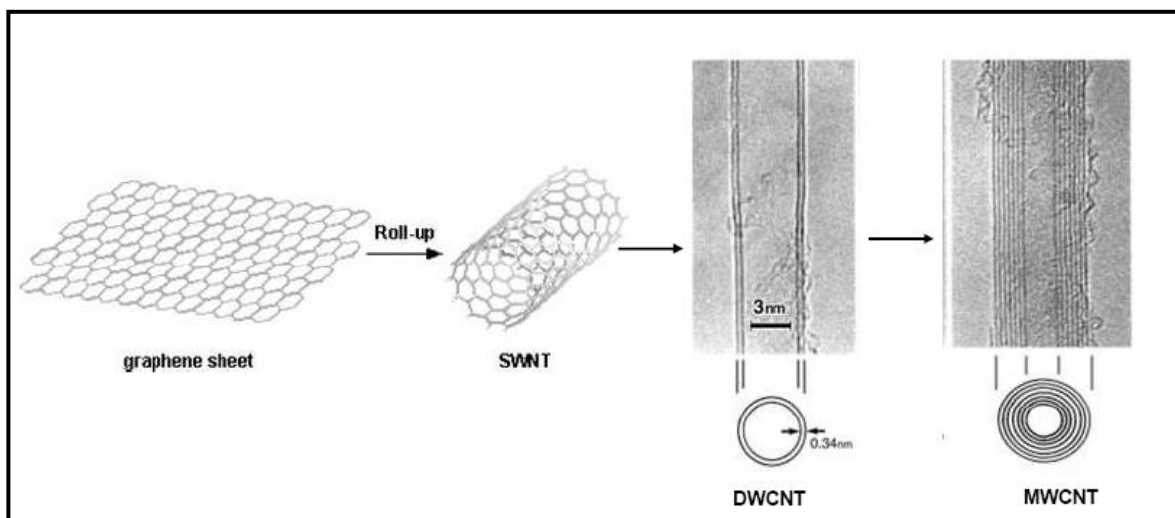
Figure 2.9: Different types of carbon nanotubes [139].
