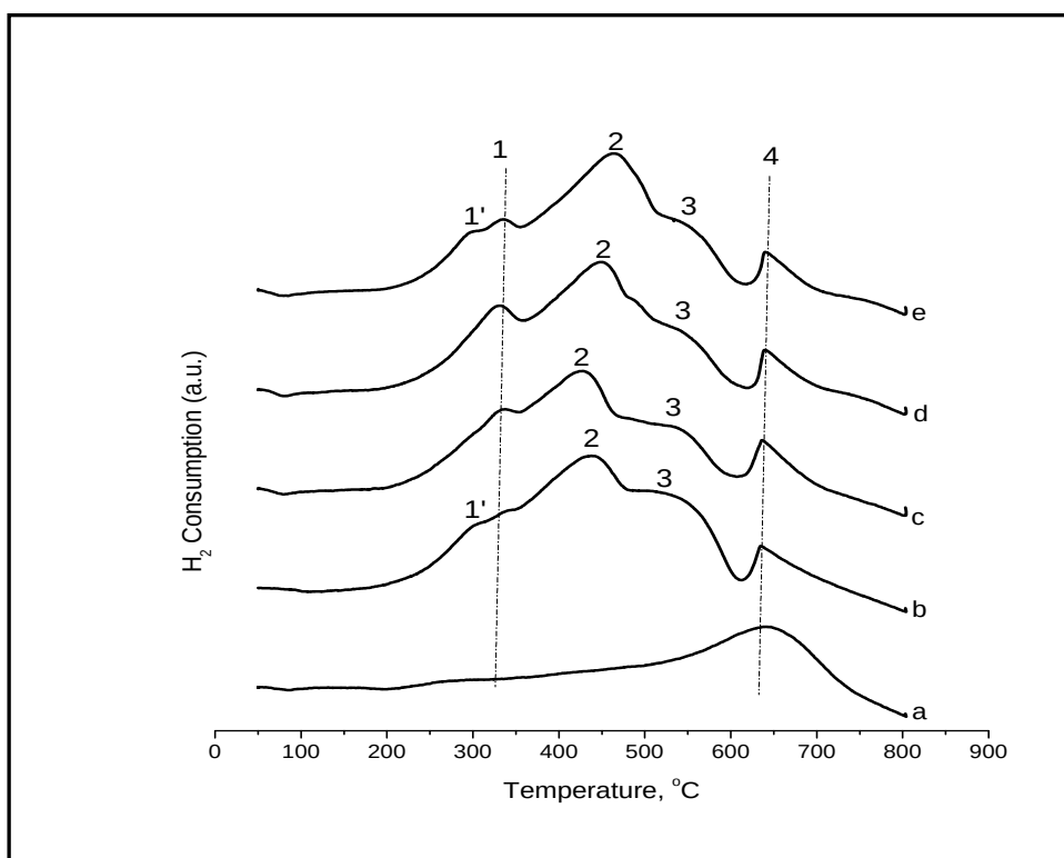
Figure 7.8: TPR profiles of the CNT, unpromoted and alkali-promoted Fe-catalysts:
