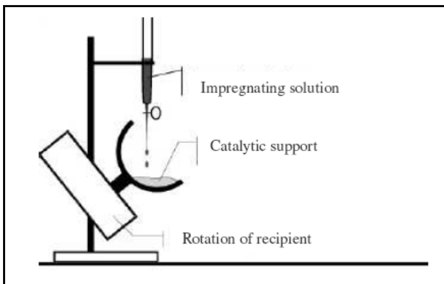
Figure 2.12: Schematic representation of experimental set up for incipient wetness impregnation method [63].
