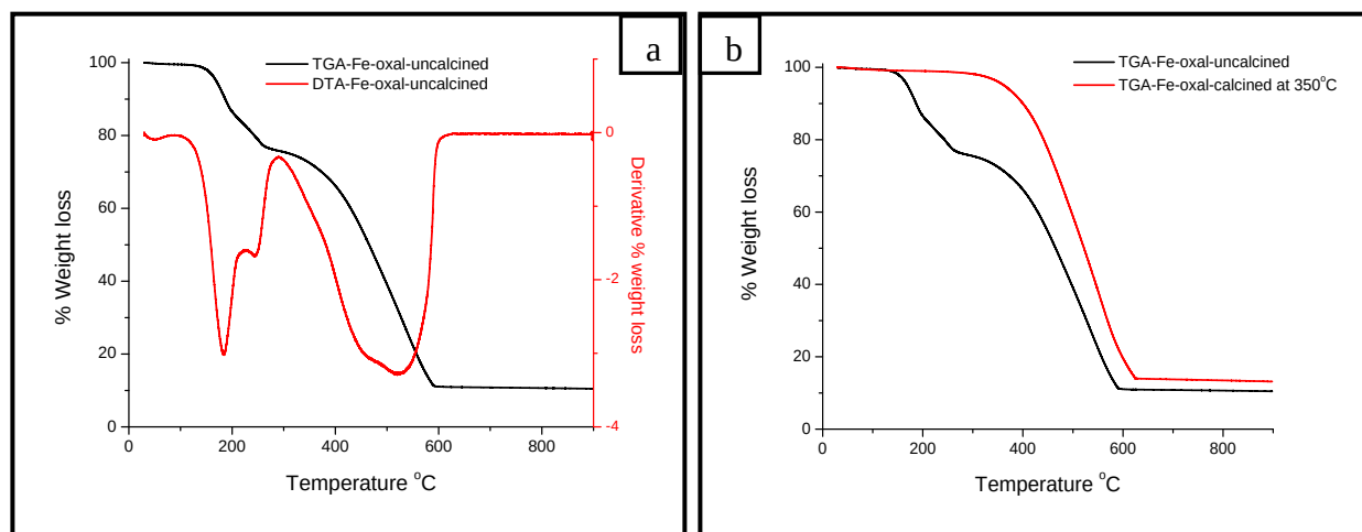
Figure 6.12: TGA profile for the Fe-oxal catalyst in air atmosphere; a) before heat treatment together with the derivative plot and b) before heat treatment and after heat treatment (350°C, 150 min).
