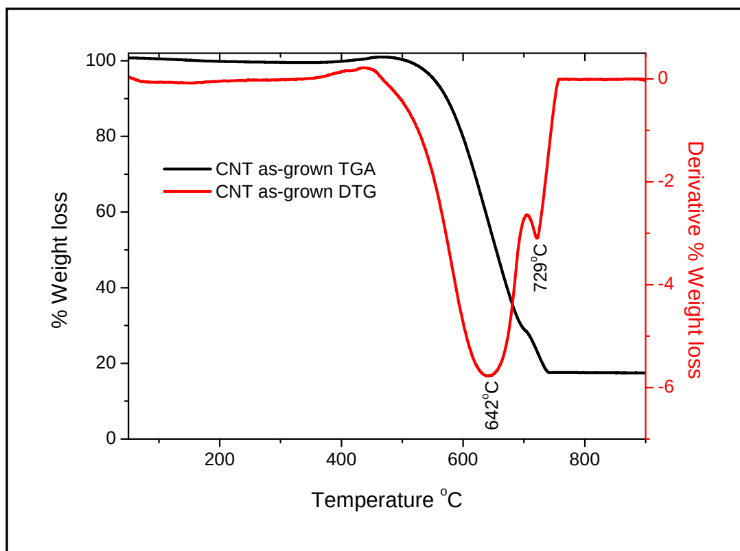
Figure 5.6: TGA and DTG profiles of as-grown CNTs under air atmosphere.
