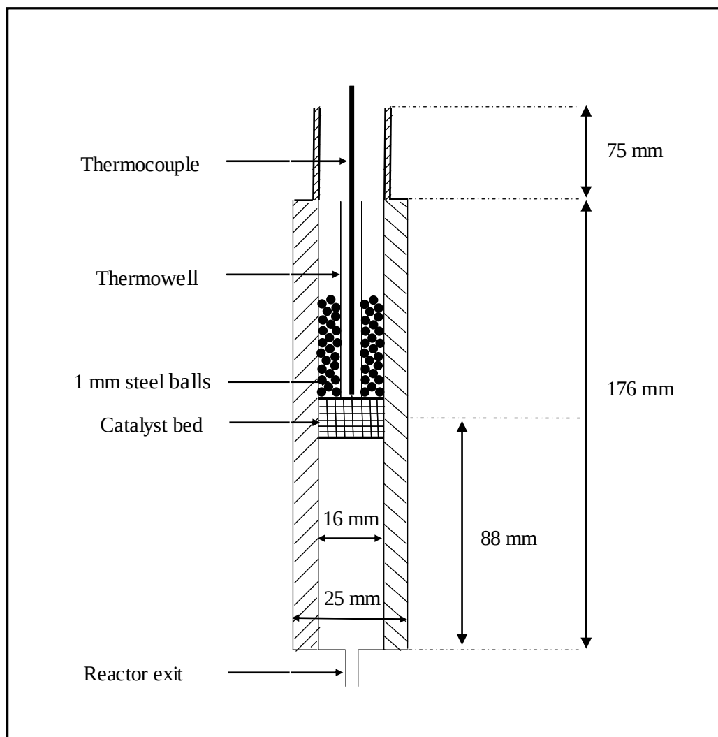
Figure 3.4: Schematic diagram of the fixed-bed micro reactor
