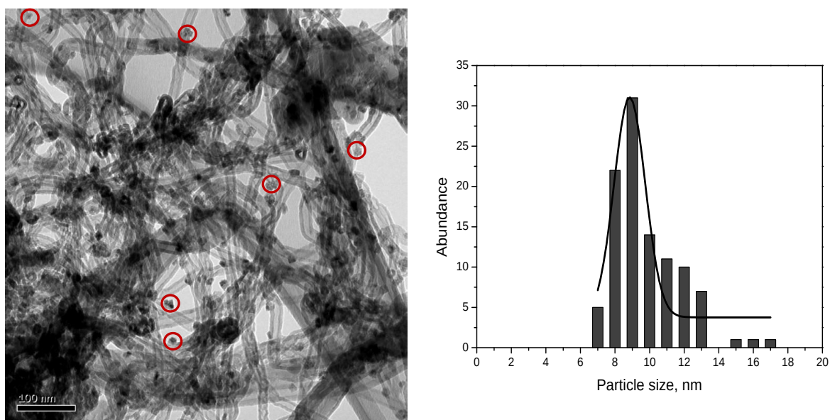
Figure 9.3: TEM image and cobalt particle size histogram for Co-A/CNT (average cobalt particle size = 8.9 nm): some Fe particles are indicated by the circles
