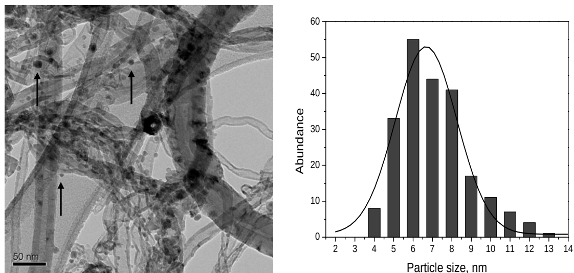
Figure 6.17: TEM image with arrows indicating the Fe particles, and Fe particle size histogram for the Fe-nitr-1 after 12 h time on stream (particle size: 5-10 nm).
