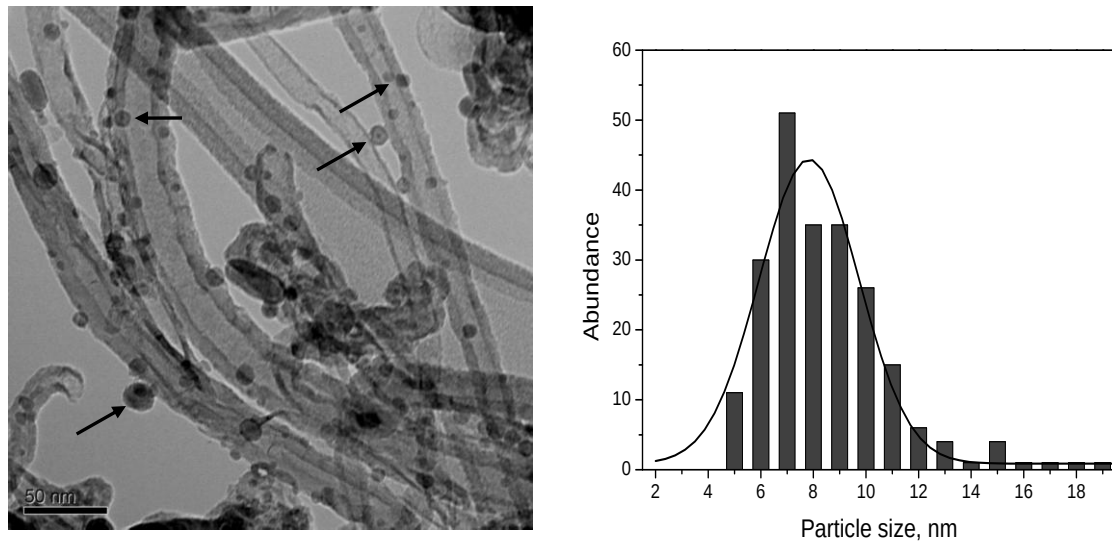
Figure 6.19: TEM image with arrows indicating the Fe particles, and Fe particle size histogram for the Fe-acet after 120 h time on stream (particle size: 5-12 nm).
