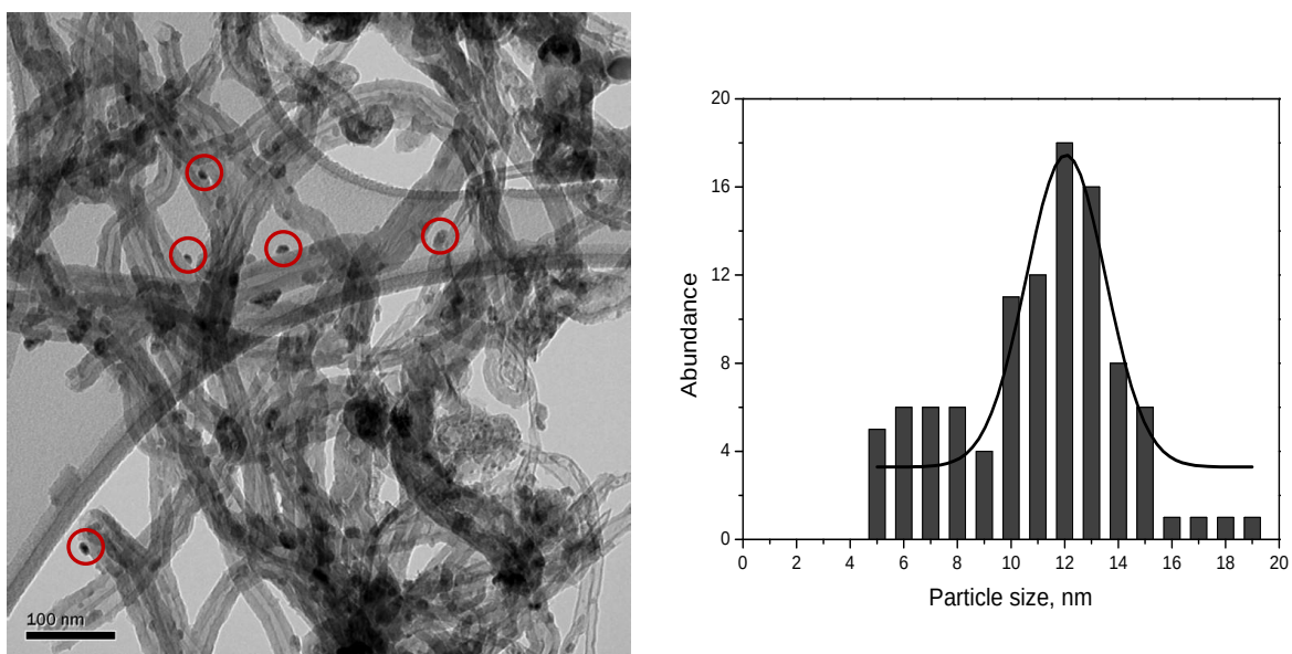
Figure 9.2: TEM image and cobalt particle size histogram for Co-N/CNT (average cobalt particle size = 12 nm): some Fe particles are indicated by the circles
