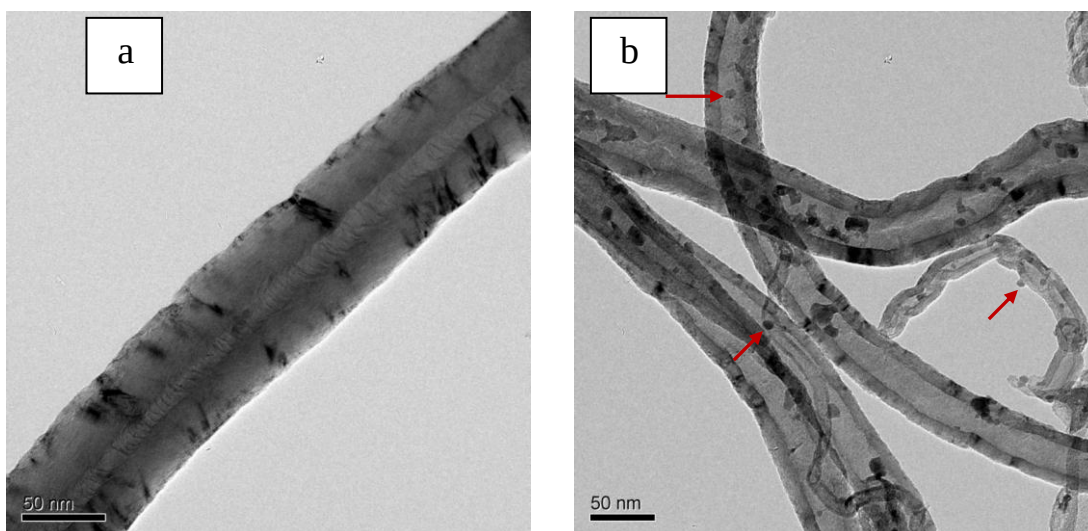
Figure 7.5: a) and b) TEM images of Na promoted Fe/CNT catalysts (100Fe-3.35K/CNT) with arrows indicating the Fe particles
