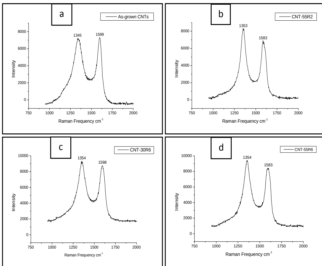
Figure 5.11: Raman spectra of CNTs: a) as-grown CNTs, b) CNT-55R2, C) CNT-30R6, d) CNT-55R6.
