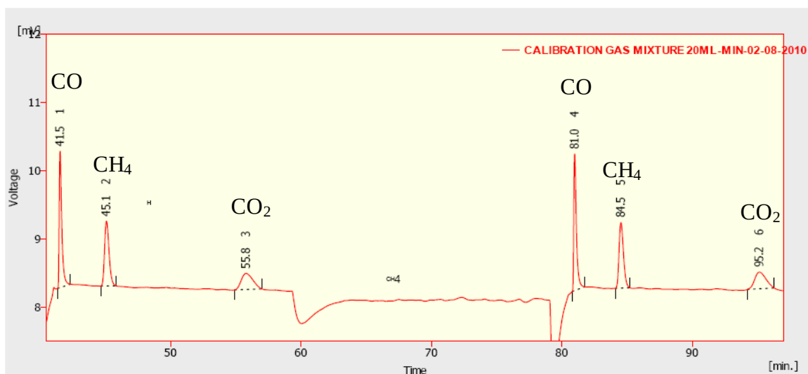
Figure 4.1: A trace for the calibration gas using the TCD GC and argon as a carrier gas
