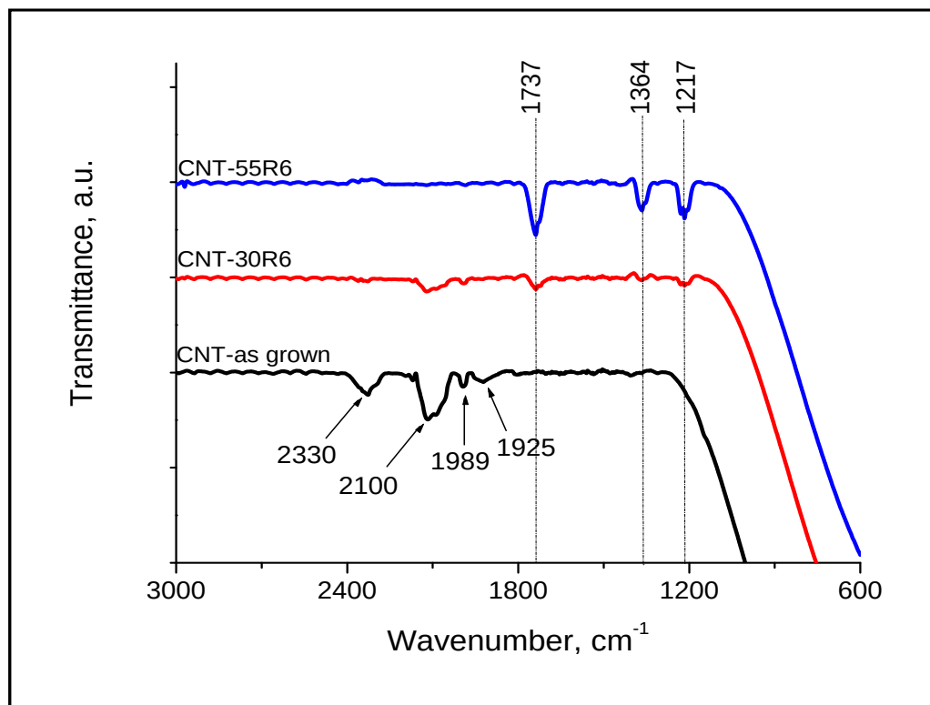
Figure 5.12: FTIR spectra of untreated (CNT-as grown) and oxidized carbon nanotubes.
