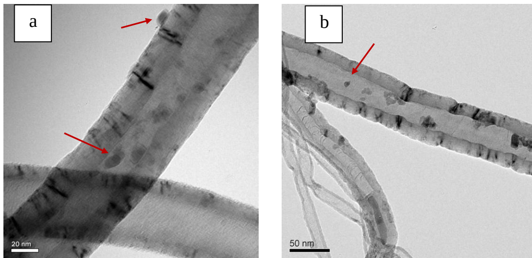
Figure 7.4: a) and b) TEM images of Li promoted Fe/CNT catalysts (100Fe-3.38K/CNT) with arrows indicating the Fe particles
