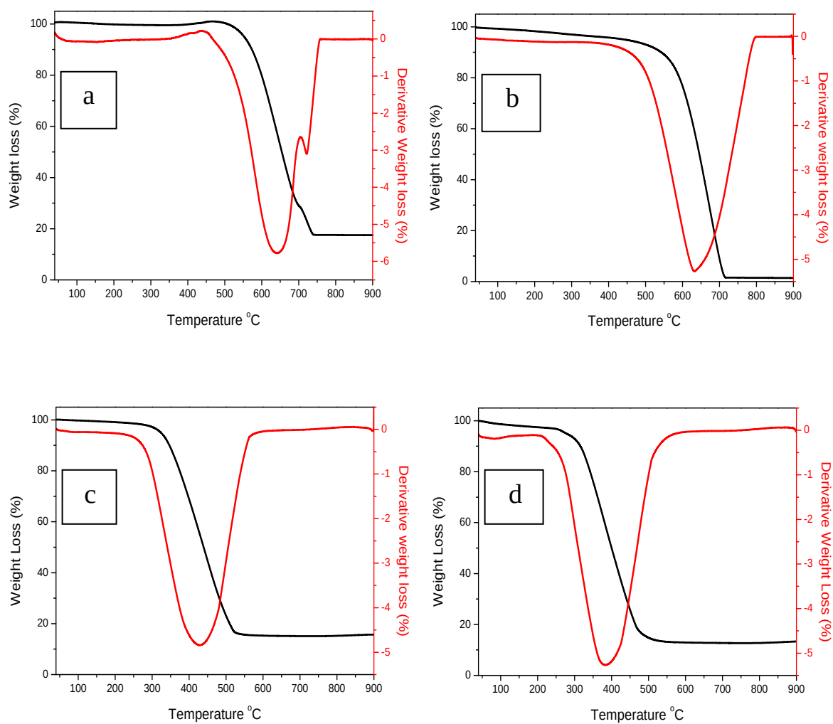
Figure 9.6: TGA curves of as-grown and purified carbon nanotubes and cobalt catalysts under air: (a) As-grown CNTs; (b) purified CNTs; (c) Co-N/CNT; and (d) Co-A/CNT.
