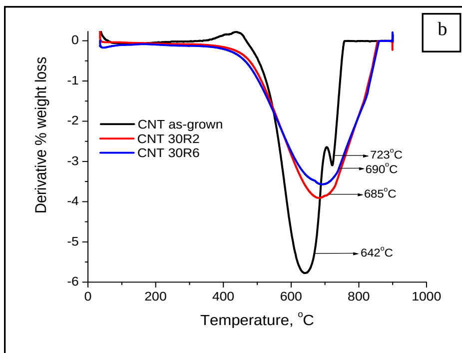
Figure 5.7: a) TGA and b) DTG profiles of as-grown CNTs as well as purified CNTs in 30% \text{HNO}_3 under air atmosphere.
