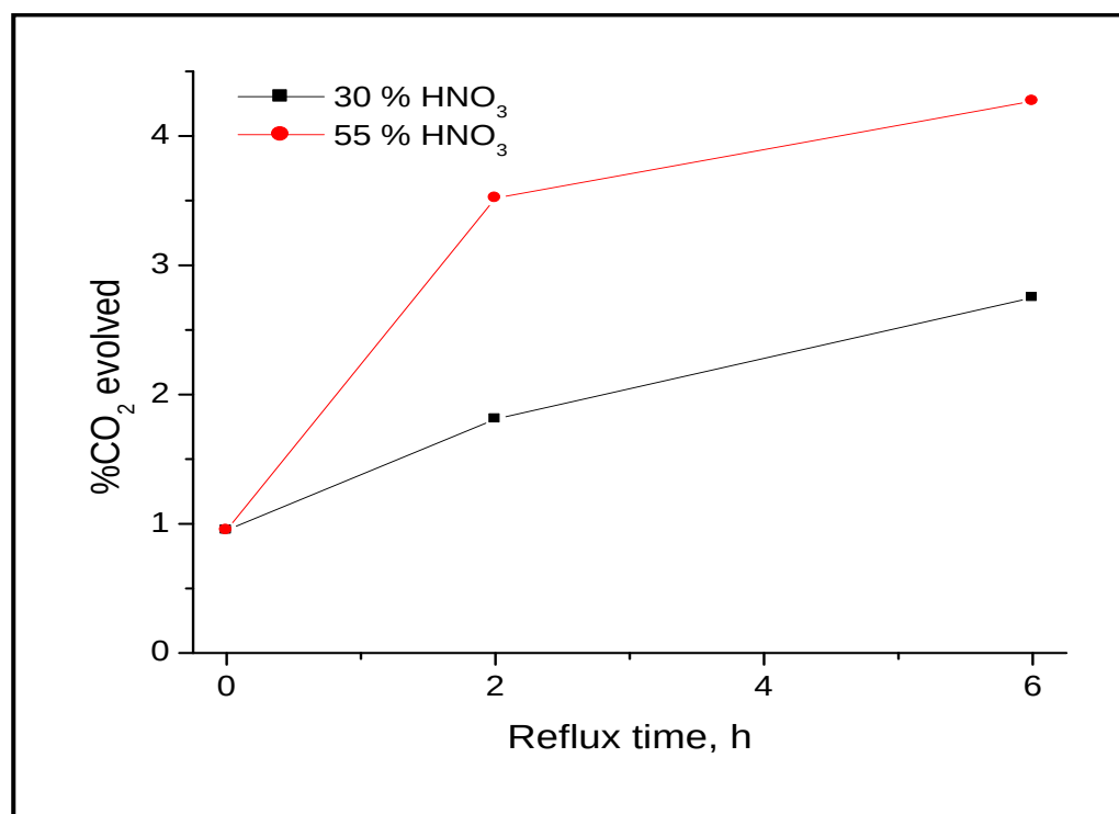
Figure 5.10: Evolution of oxygen as CO 2 versus reflux time.
