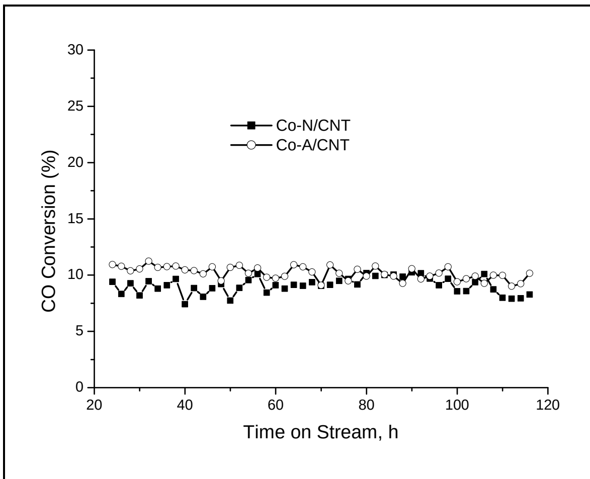
Figure 9.7: CO conversion versus time on stream (reaction conditions: T = 220^{\circ}\text{C} , P = 8 \text{ bar} , \text{H}_2 : \text{CO} = 2 , \text{GHSV} = 2400 \text{ h}^{-1} )
