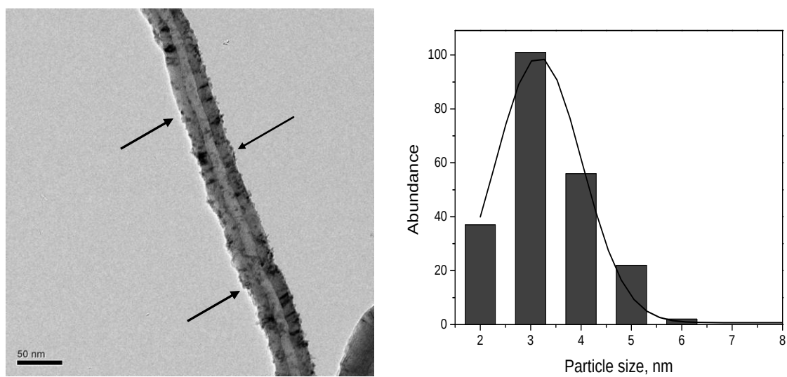
Figure 6.8: TEM image with arrows indicating the Fe particles, and Fe particle size histogram for the Fe-nitr-1 catalyst.
