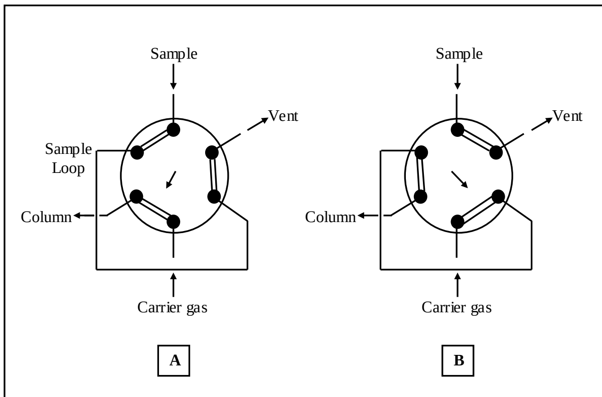
Figure 3.6: A schematic diagram of the valves viewed from the preload end (VICI Valco Instruments Co. Inc. Technical Note 203)
