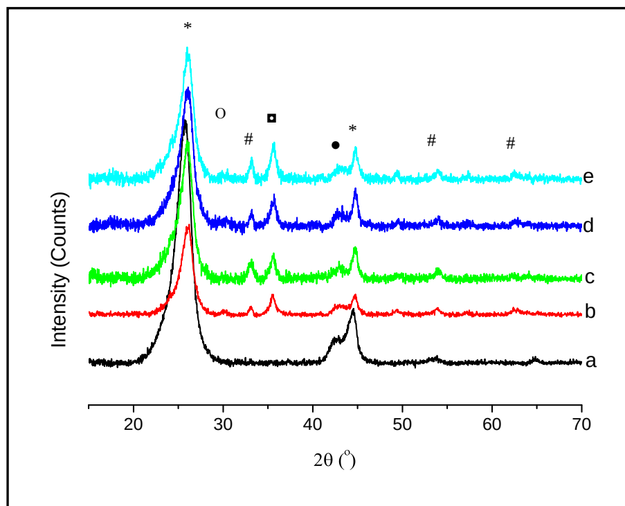
Figure 7.9: XRD patterns of CNTs, unpromoted and alkali promoted Fe/CNT catalysts: a) CNT support, b) 100Fe/CNT, c) 100Fe-3.38Li/CNT, d) 100Fe-3.35Na/CNT, e) 100Fe-3.31K/CNT; * = graphite; o = \text{Fe}_3\text{O}_4 ; # = \text{Fe}_2\text{O}_3 ; ■ = \text{Fe}_2\text{O}_3 and \text{Fe}_3\text{O}_4 ; ● = Co-Fe, \text{Fe}_3\text{C} , \text{Co}_3\text{C} or \text{Co}_2\text{C} [19, 27].
