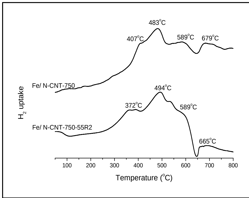
Figure 8.10: H_2 -TPR profiles of Fe/N-CNT-750-55R2 and Fe/N-CNT-750 catalysts.
