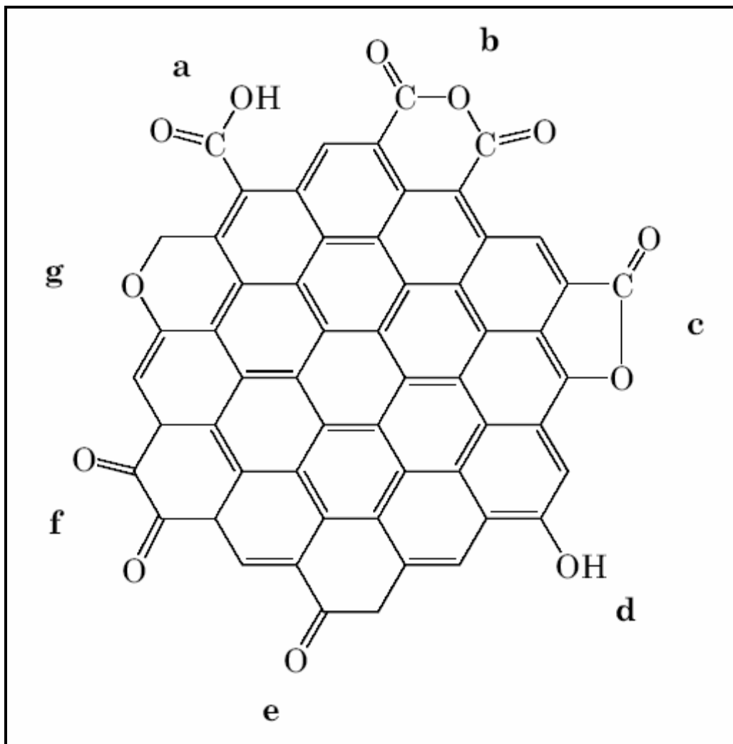
Figure 2.11: Different oxygen-containing surface groups on carbon. a) carboxyl groups, b) carboxylic anhydride groups, c) lactone groups, d) phenol groups, e) carbonyl groups, f) quinone groups, g) xanthene or ether groups [238].
