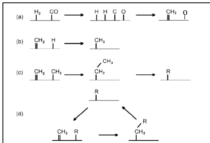
Figure 2.4: an Alkyl FT reaction mechanism for initiation and propagation of hydrocarbon chain: (a) methylene formation, (b) initiation, (c) initiated chain growth, (d) propagation [51]
