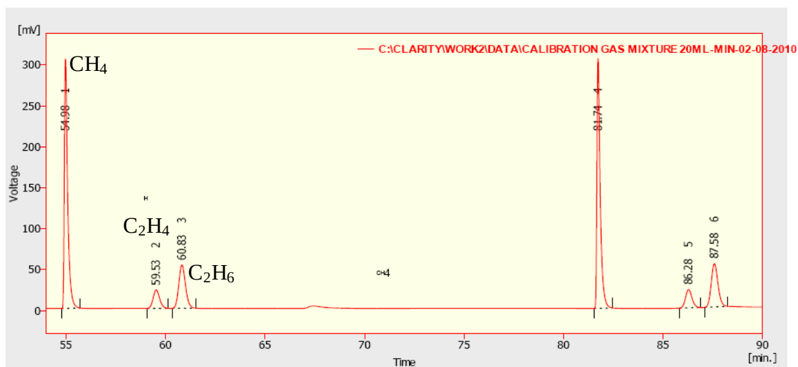
Figure 4.2: A trace for the calibration gas using the FID GC and nitrogen as a carrier gas
