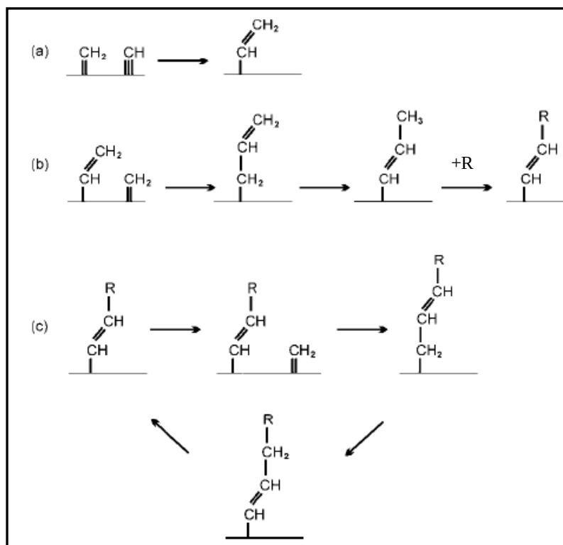
Figure 2.6: Alkenyl mechanism: (a) chain initiation, (b) chain growth including insertion of methylene and isomerization, (c) chain propagation [51].
