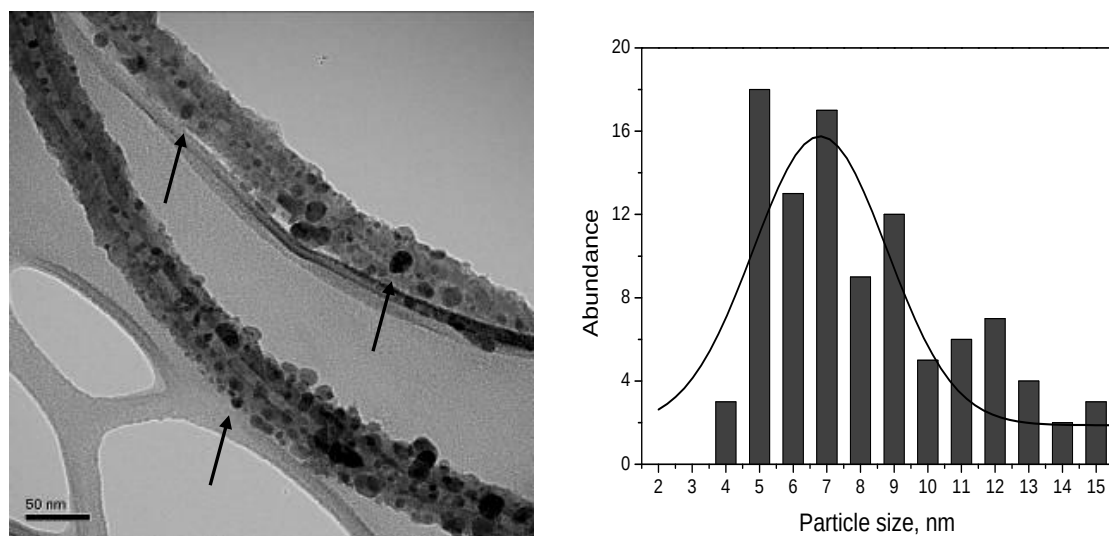
Figure 6.6: TEM image with arrows indicating the Fe particles, and Fe particle size histogram for the Fe-oxal catalyst.
