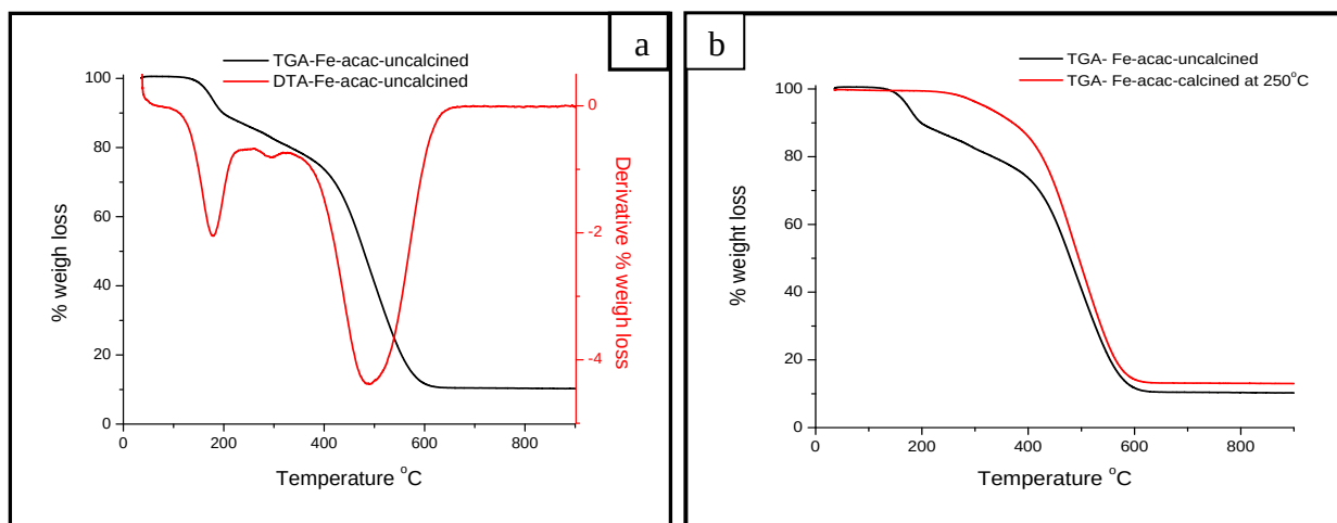
Figure 6.11: TGA profile in air atmosphere for the Fe-acac catalyst: a) before heat treatment together with the derivative plot and b) before heat treatment and after heat treatment (250°C, 150 min).
