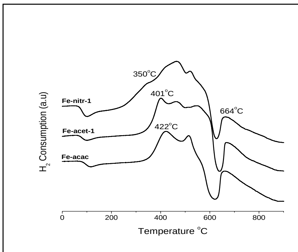
Figure 6.15: TPR profiles of Fe/CNT catalysts prepared using acetone as the solvent.
