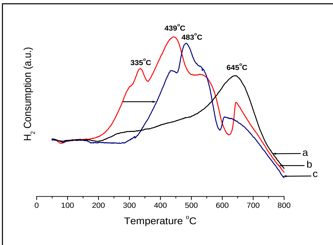
Figure 5.14: TPR profiles of a) CNT-55R2 support, b) 10%Fe/CNT-55R2 catalyst and c) 10%Fe/CNT-55R6 catalyst.
