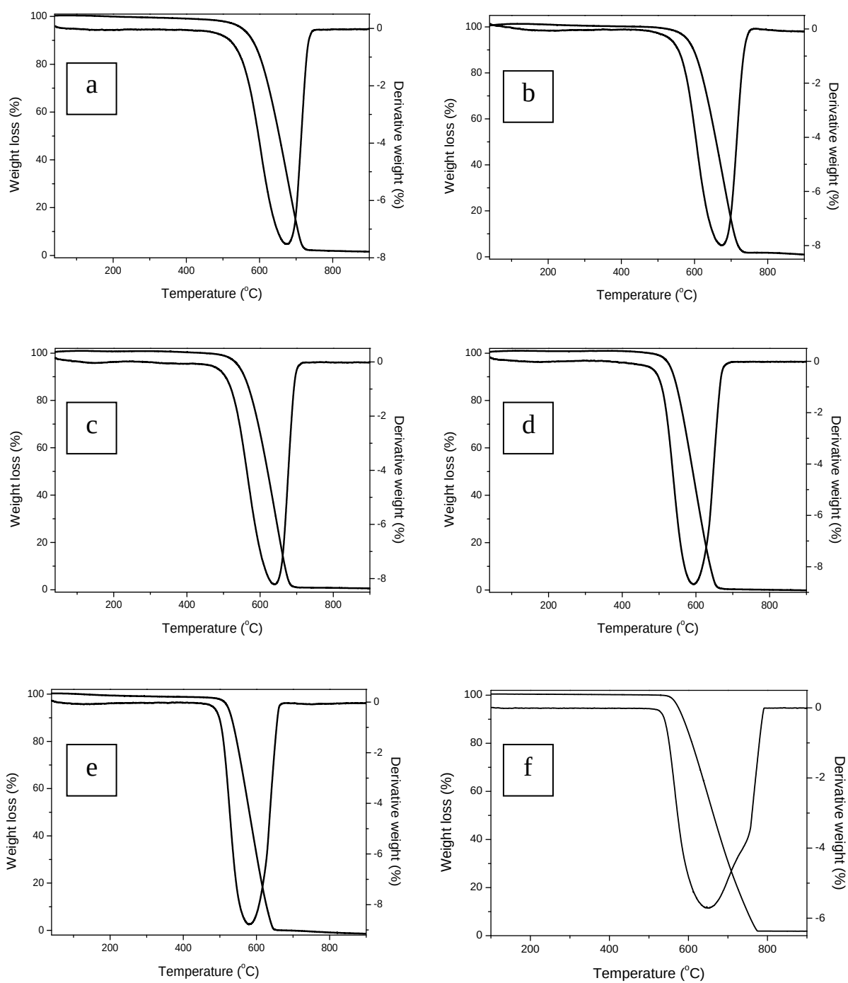
Figure 8.4: TGA and DTA profiles of the purified CNTs and N-CNTs (obtained at different post treatment temperatures): a) purified CNT; b) N-CNT-700°C; c) N-CNT-750°C; d) N-CNT-800°C; e) N-CNT-850°C; f) N-CNT-900°C.
