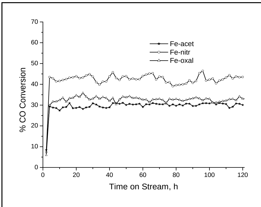
Figure 6.16: CO conversion as a function of time on stream.
