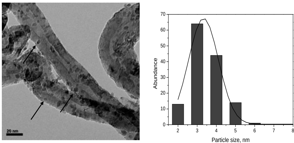
Figure 6.4: TEM image with arrows indicating the Fe particles, and Fe particle size histogram for the Fe-acet catalyst.
