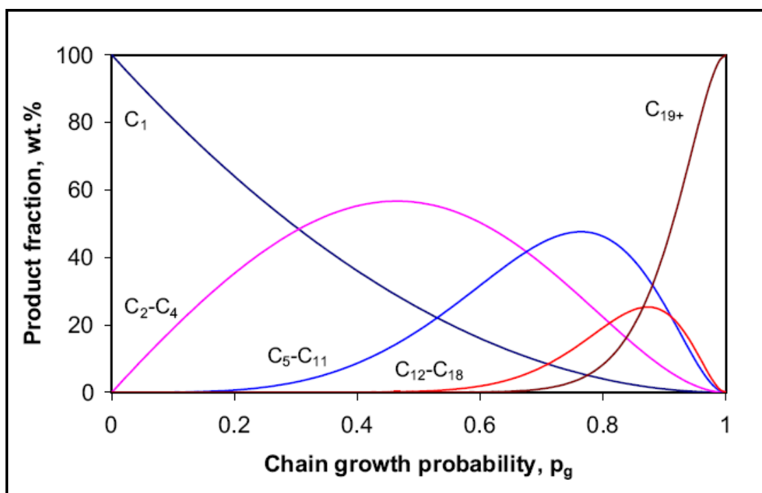
Figure 2.3: Theoretical product distribution as a function of the chain growth probability assuming ideal ASF kinetics [3].
