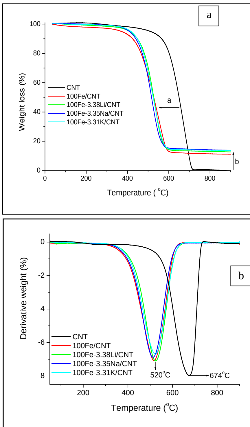
Figure 7.7: a) TGA and b) DTA of CNTs, and promoted and unpromoted Fe catalysts
