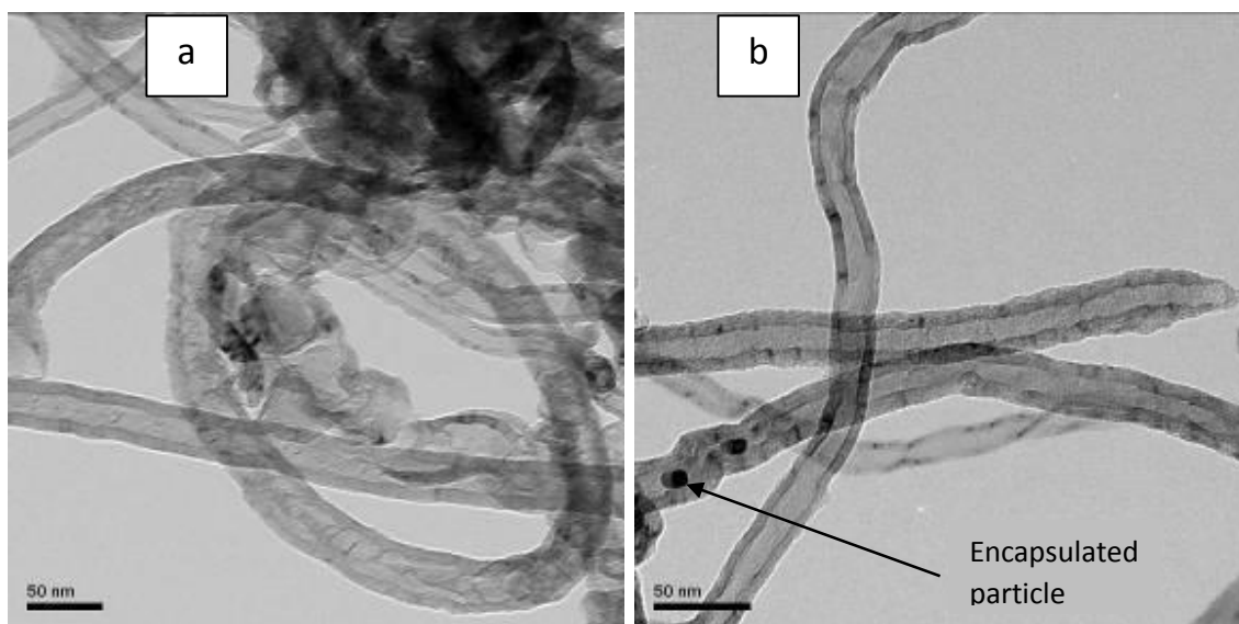
Figure 5.1: a) TEM image of as-grown CNTs and b) TEM image of as-grown CNTs showing some encapsulated metal particles indicated by arrow.
