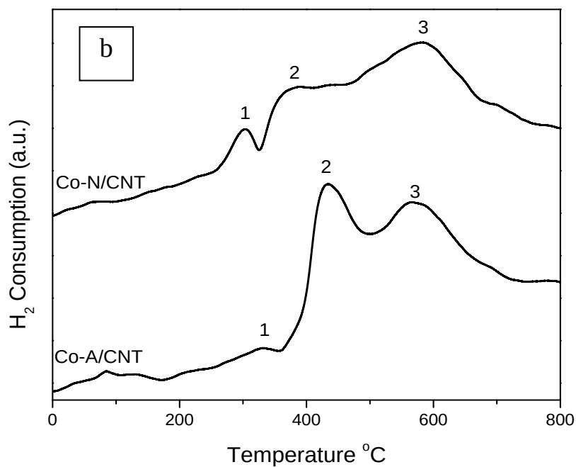
Figure 9.5: TPR profiles of (a) \text{Co}(\text{NO}_3)_2 \cdot 6\text{H}_2\text{O} calcined at 250^\circ\text{C} for 2 h and (b) 10 wt% Co/CNT prepared using cobalt nitrate and cobalt acetate precursors.
