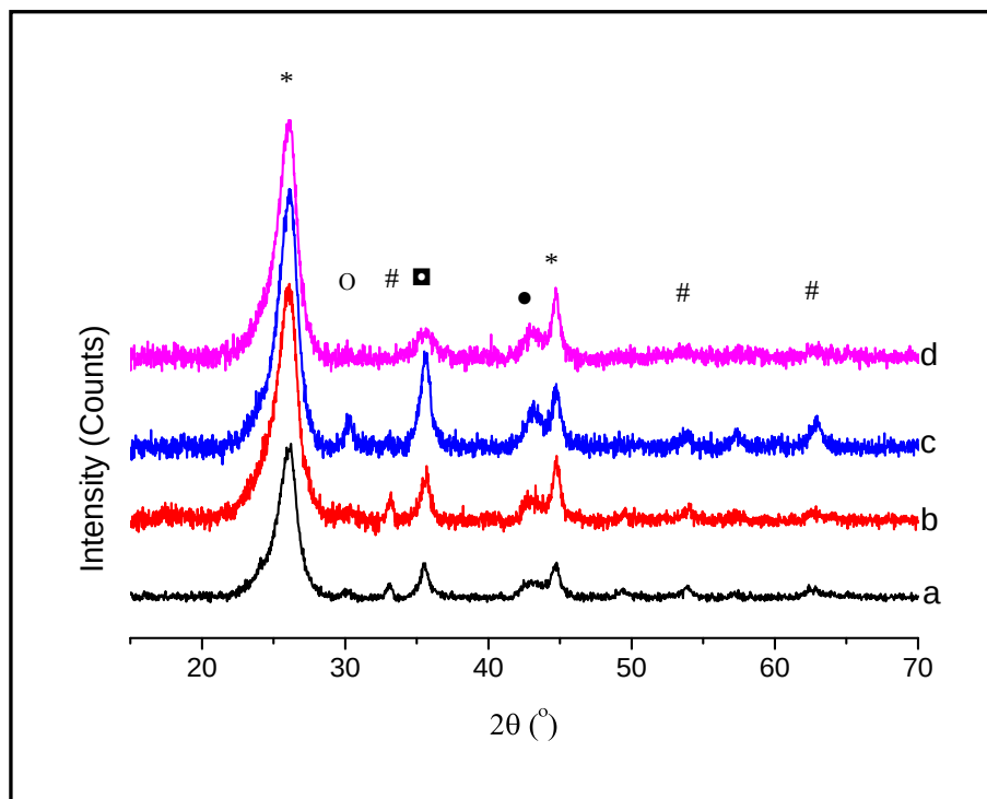
Figure 7.11: XRD patterns of unpromoted and Na promoted Fe/CNT catalysts: a) 100Fe/CNT, b) 100Fe-3.35Na/CNT, c) 100Fe-12Na/CNT, d) 100Fe-24Na/CNT; * = graphite; O = \text{Fe}_3\text{O}_4 ; # = \text{Fe}_2\text{O}_3 ; ■ = \text{Fe}_2\text{O}_3 and \text{Fe}_3\text{O}_4 ; ● = Co-Fe, \text{Fe}_3\text{C} , \text{Co}_3\text{C} or \text{Co}_2\text{C} ;
