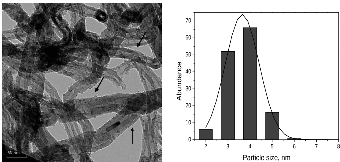
Figure 6.9: TEM image with arrows indicating the Fe particles, and Fe particle size histogram for the Fe-acac catalyst.
