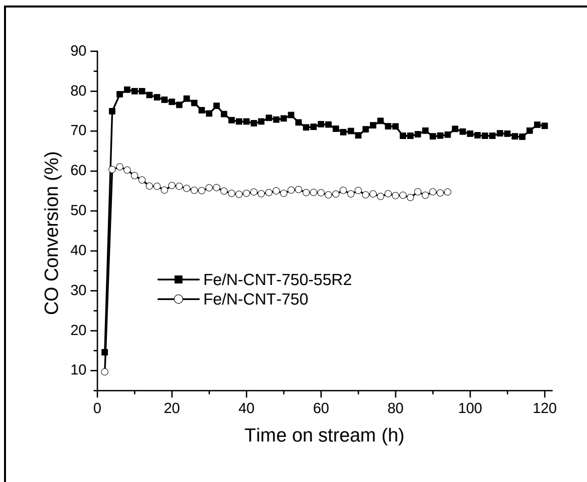
Figure 8.11: CO conversion versus time on stream.
