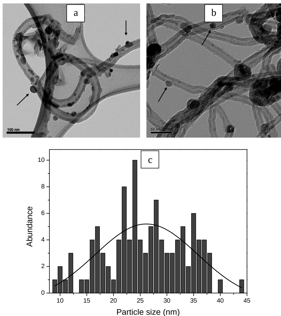
Figure 8.7: (a) and (b) TEM images and (c) Fe particle size histogram of the Fe/N-CNT-750 catalyst, (arrows on the TEM images show iron particles)
