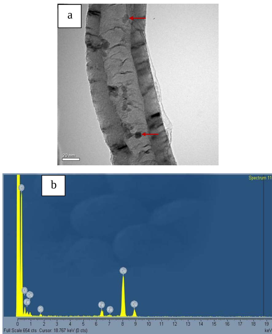
Figure 7.6: Potassium promoted Fe/CNT catalyst (100Fe-3.31K/CNT): a) TEM image with arrow indicating an Fe particle and b) EDX spectrum
