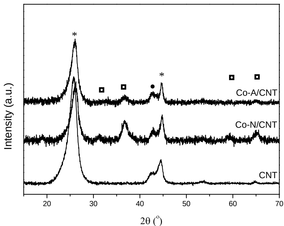
Figure 9.4: XRD patterns of the CNT support and Co/CNT catalysts: * = CNT; ■ = \text{Co}_3\text{O}_4 ; • = Co-Fe, \text{Co}_3\text{C} , \text{Co}_2\text{C} or \text{Fe}_3\text{C} .
