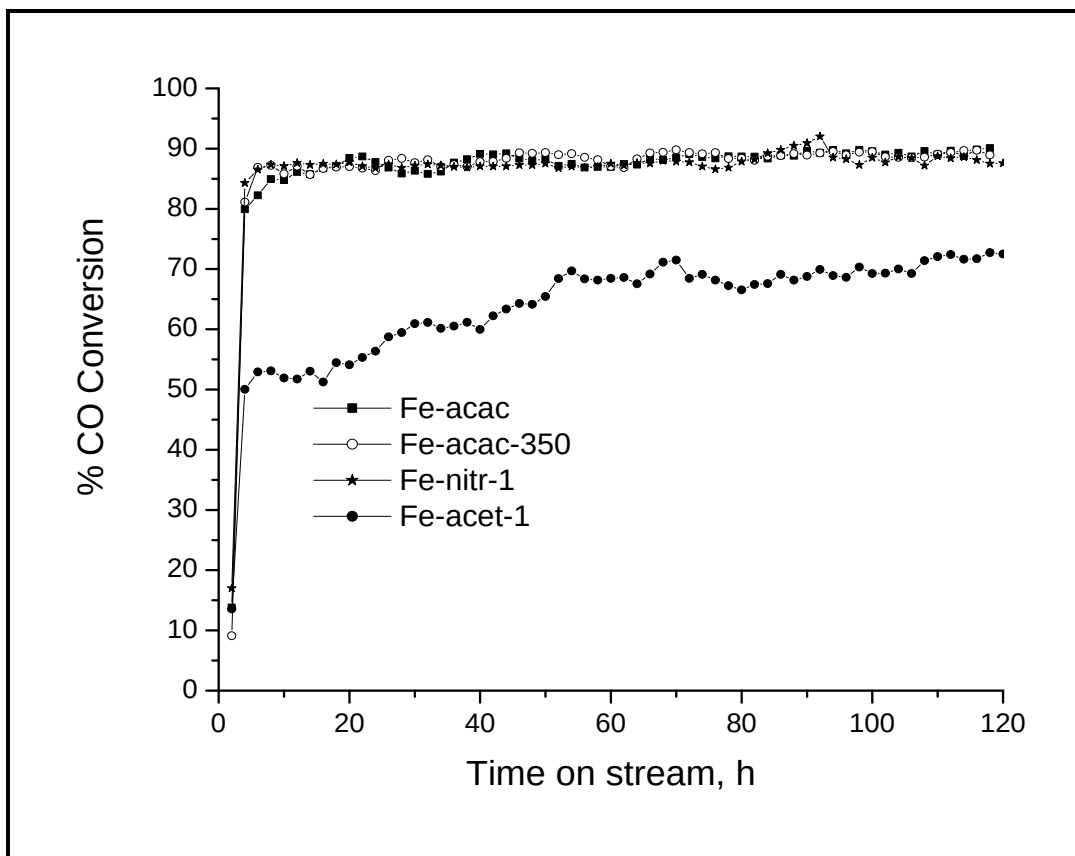
Figure 6.16: CO conversion with time on stream for catalysts prepared using acetone as solvent.
