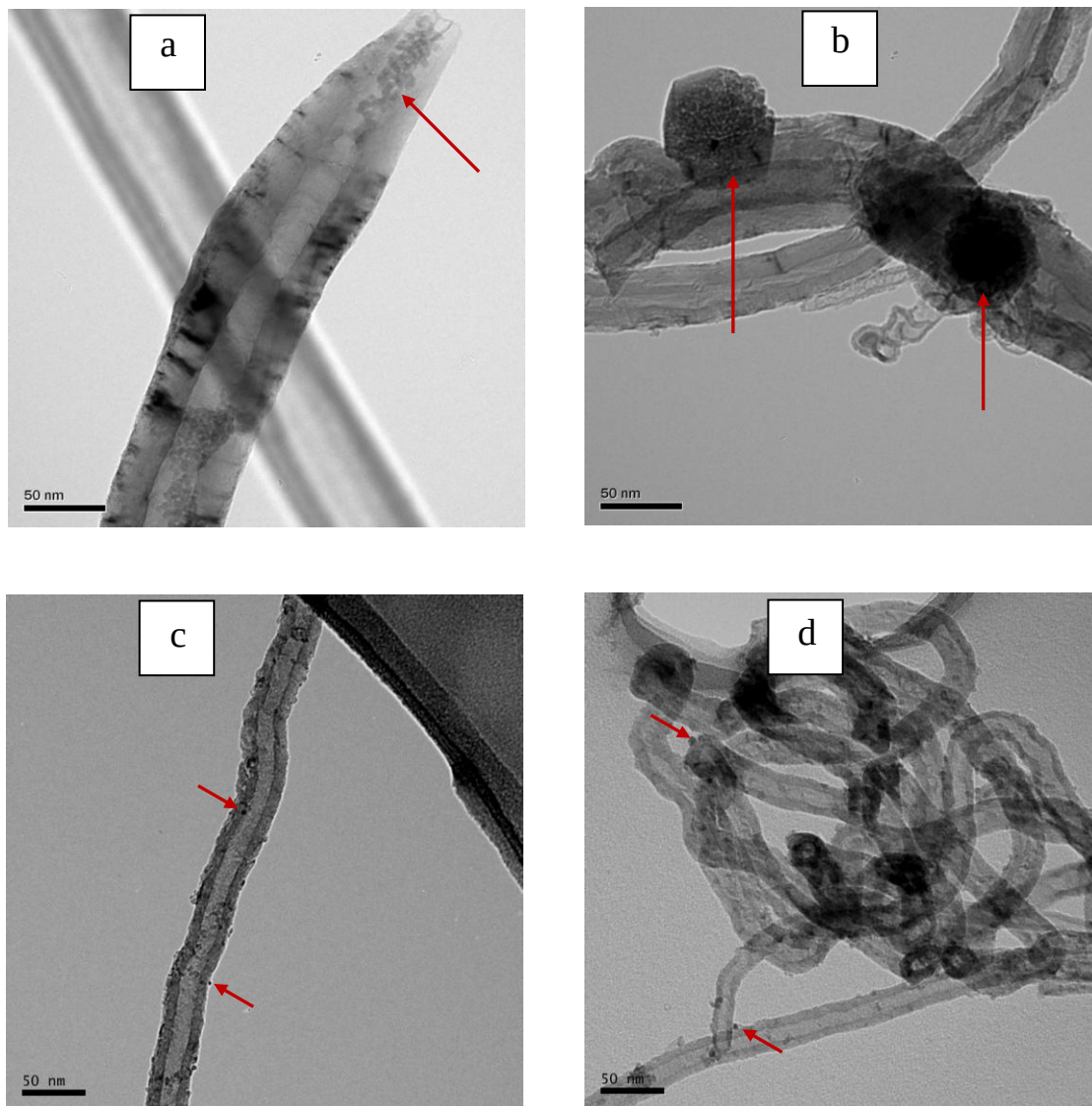
Figure 5.13: a) and b) TEM images of 10%Fe/CNT-as grown with arrow indicating large Fe clusters (iron cluster size \sim 35 \pm 5 nm based on 10 particles) ; c) and d) TEM images of 10%Fe/CNT-55R6 with arrow indicating small Fe particle (iron particle size \sim 6 \pm 1 nm based on 50 particles);
