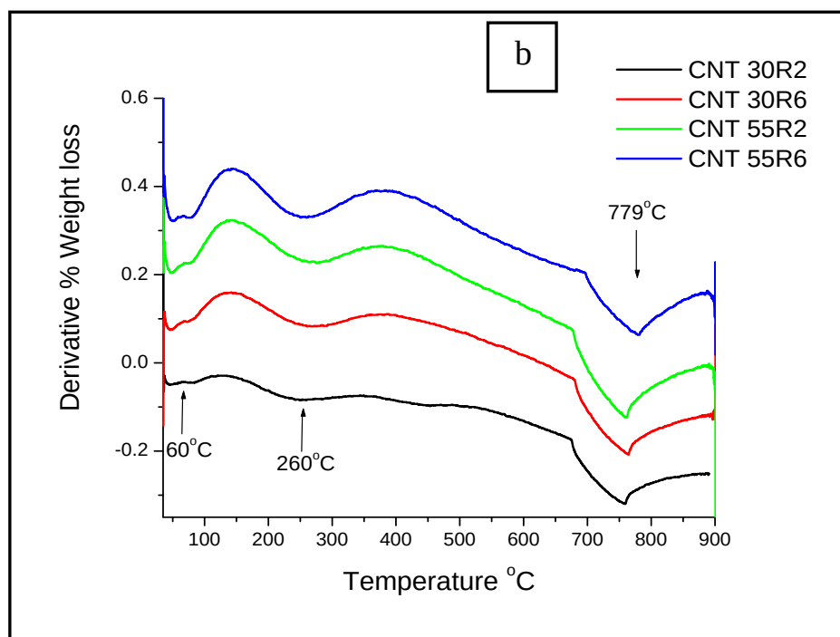
Figure 5.9: a) TGA and b) DTG profiles of as-grown and acid treated CNTs under N_2 atmosphere.
