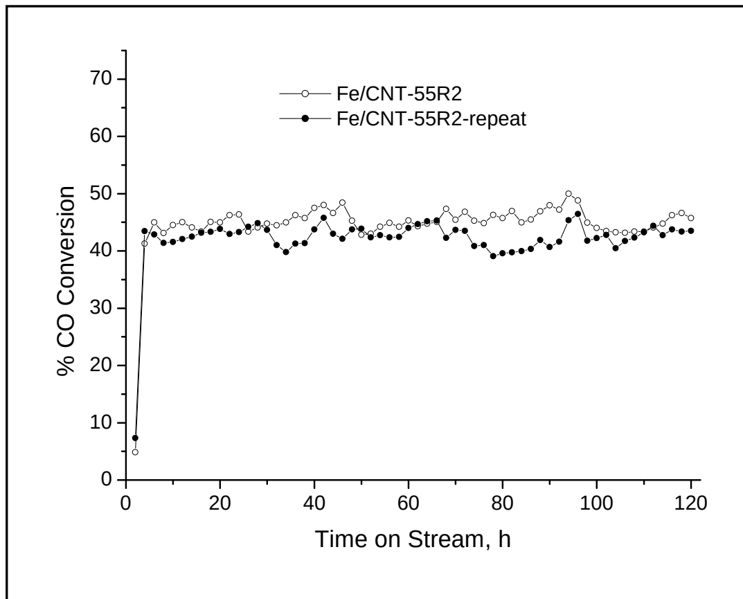
Figure 5.15: CO conversion with time on stream showing reproducibility of results
