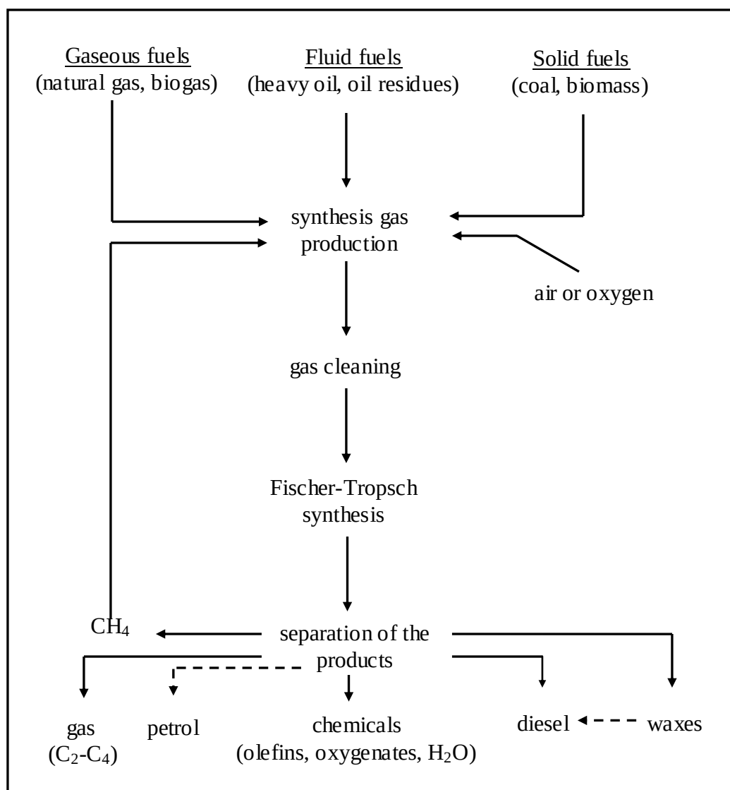
Figure 2.1: Fischer-Tropsch process overview after [3]
