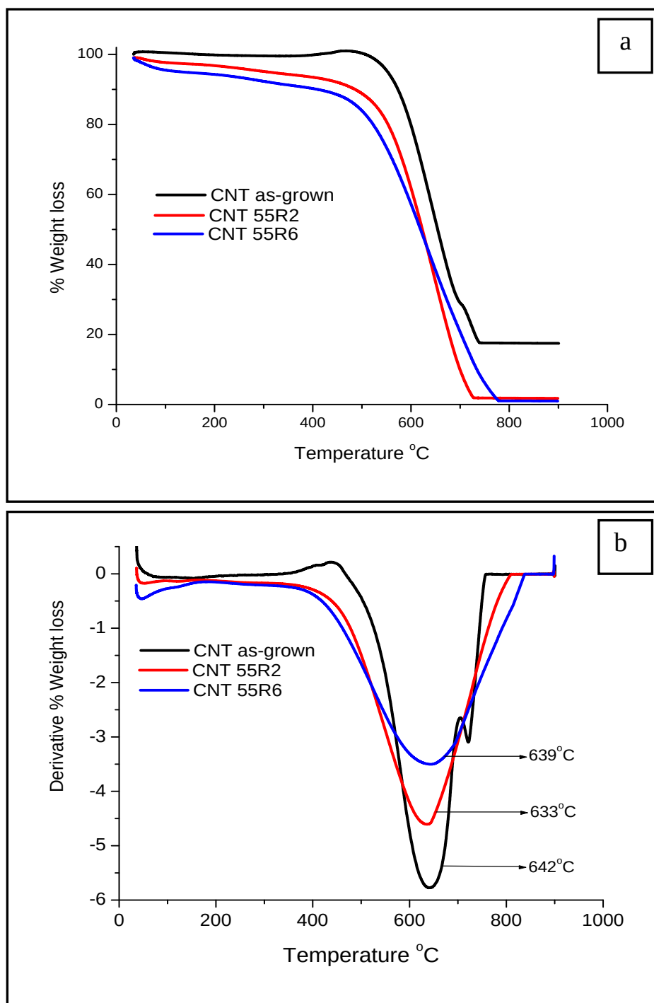
Figure 5.8: a) TGA and b) DTG profiles of as-grown CNTs as well as purified CNTs in 55% \text{HNO}_3 under air atmosphere.
