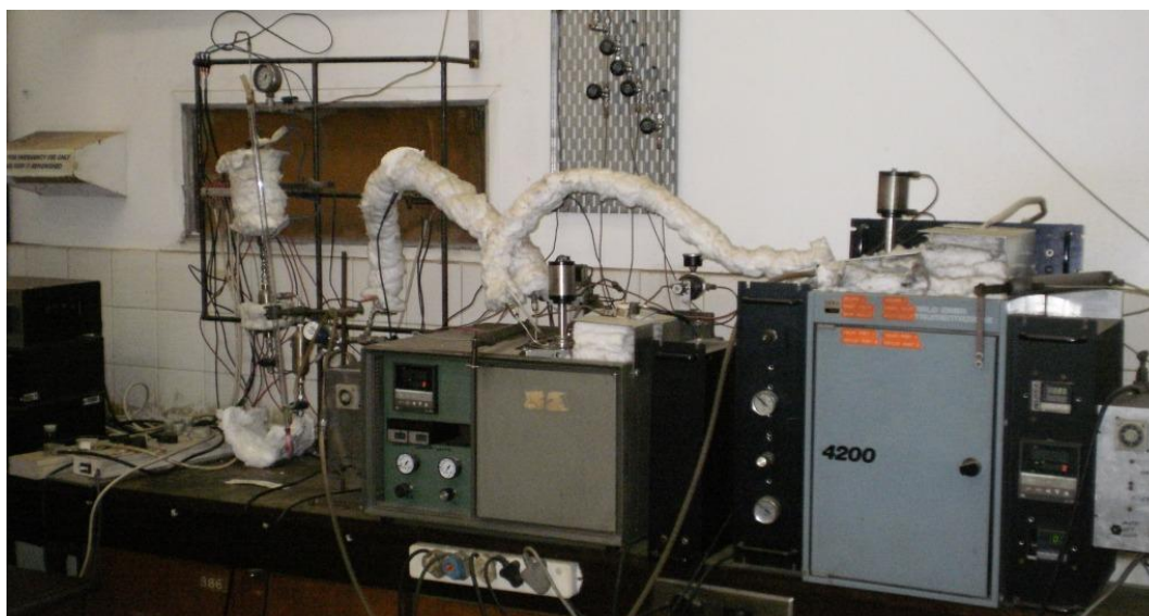
Figure 3.3: Photograph of the FT single micro reactor system set up
