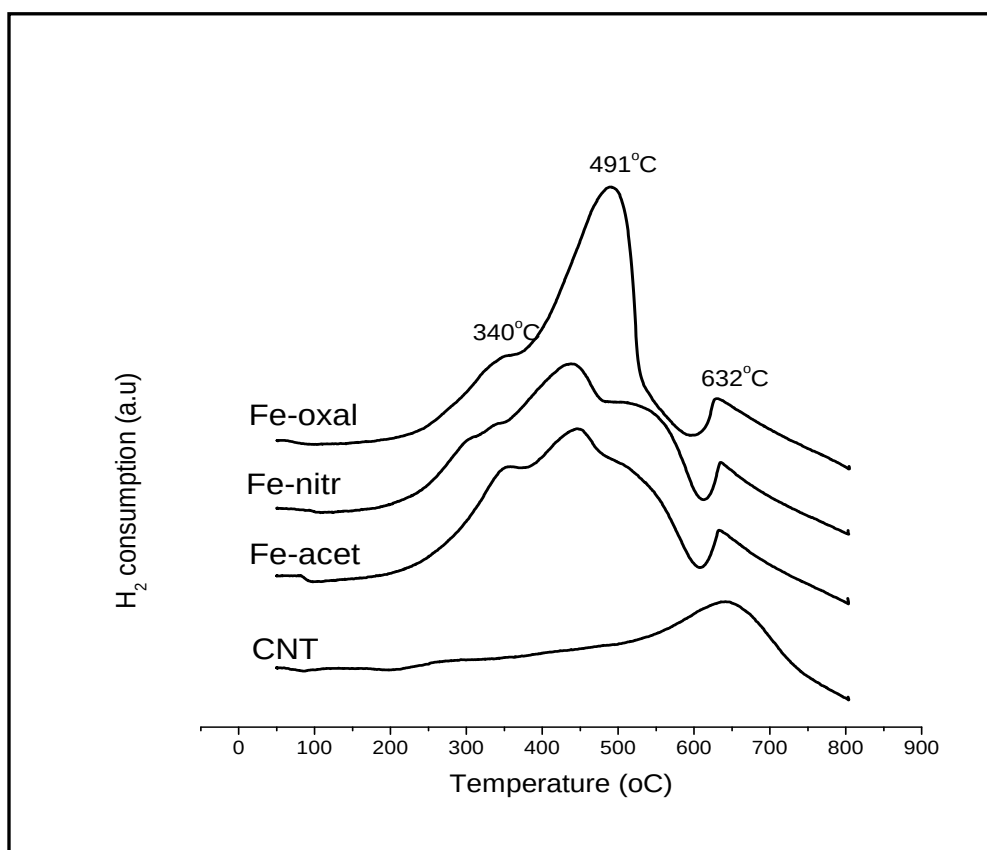
Figure 6.14: TPR profiles of the support and the Fe/CNT catalysts prepared using water as the solvent.
