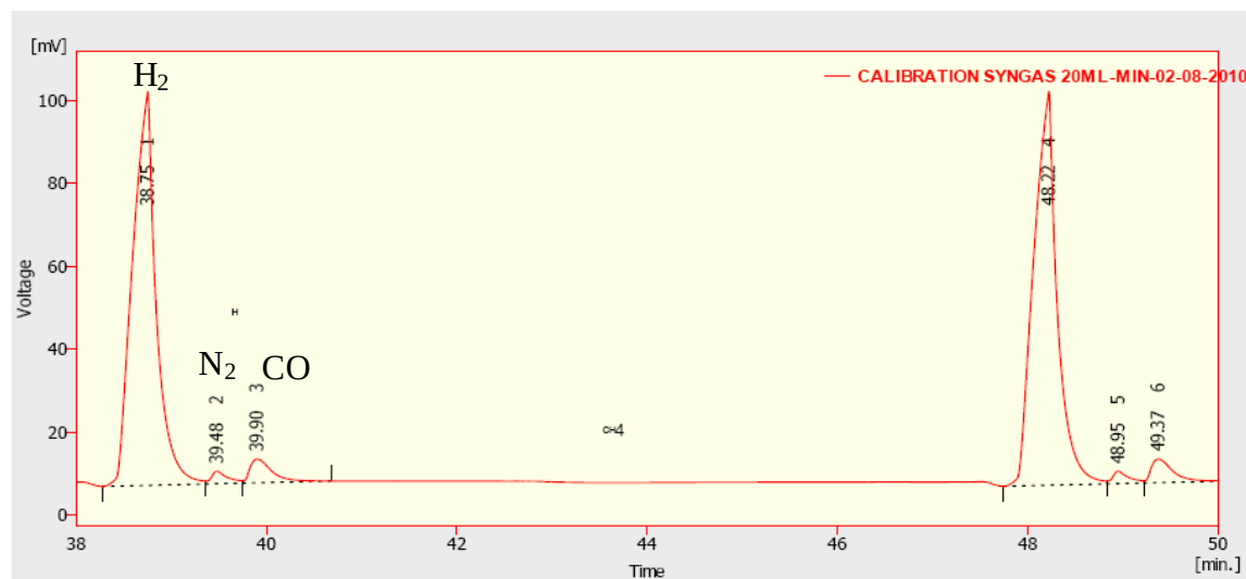
Figure 4.3: A trace for the syngas calibration using the TCD GC and argon as a carrier gas
