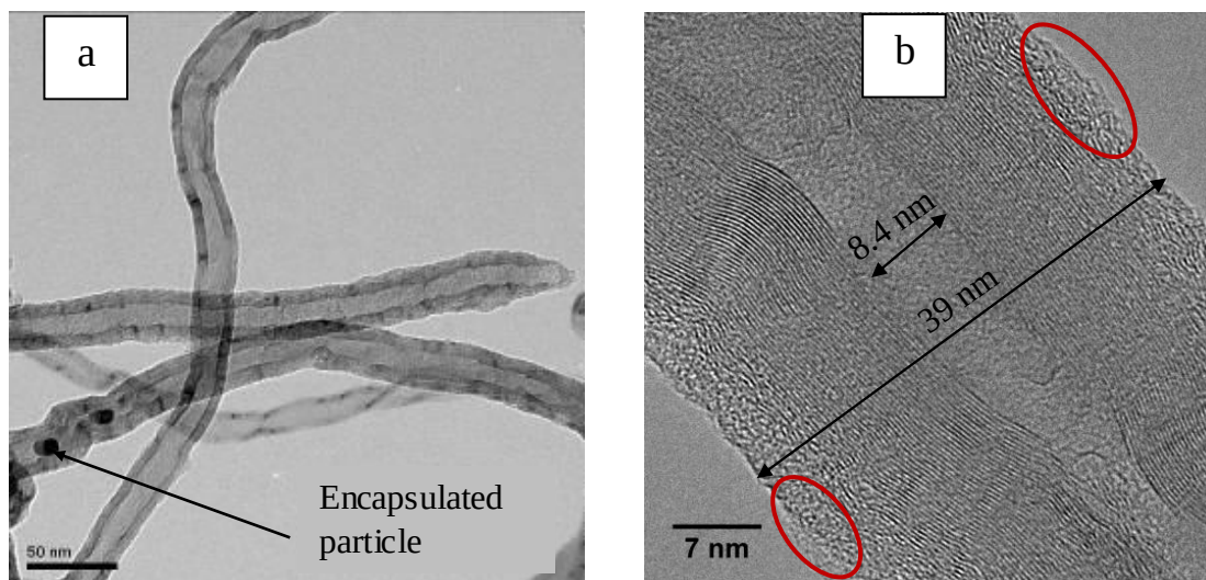
Figure 7.1: CNTs as-grown - a) TEM, b) HRTEM with red oval representing amorphous carbon.
