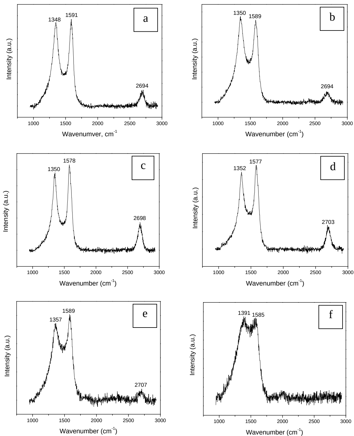
Figure 8.5: Raman spectra of CNTs and N-CNTs (obtained at different post treatment temperatures): a- purified CNT; b- N-CNT-700°C; c- N-CNT-750°C; d- N-CNT-800°C; e- N-CNT-850°C; f- N-CNT-900°C.
