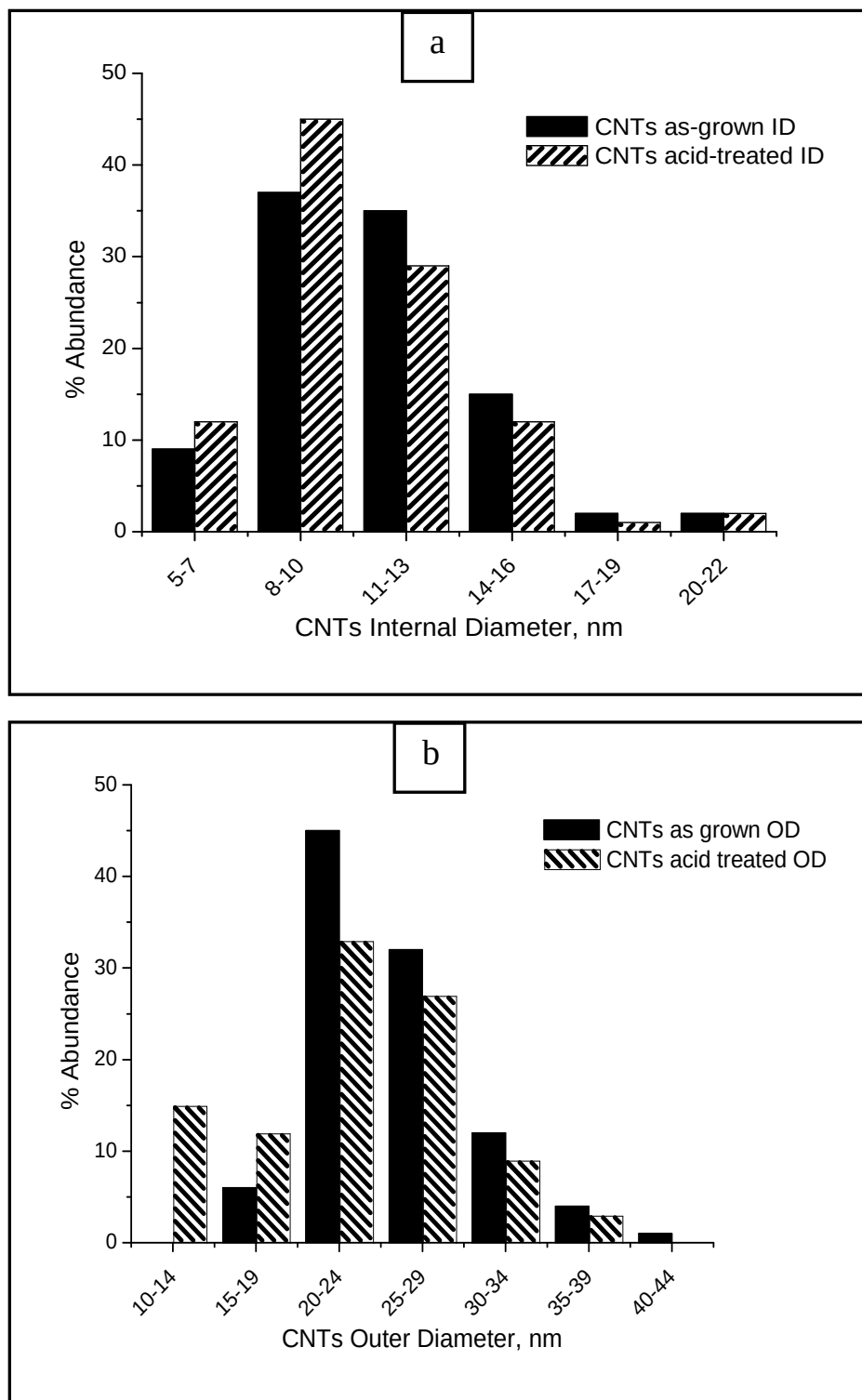
Figure 5.2: Diameter size distribution before and after acid treatment. a) Comparison of inner diameters; b) comparison of outer diameters.
