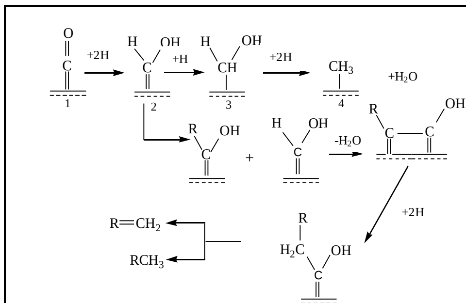
Figure 2.5: Enol mechanism [52].
