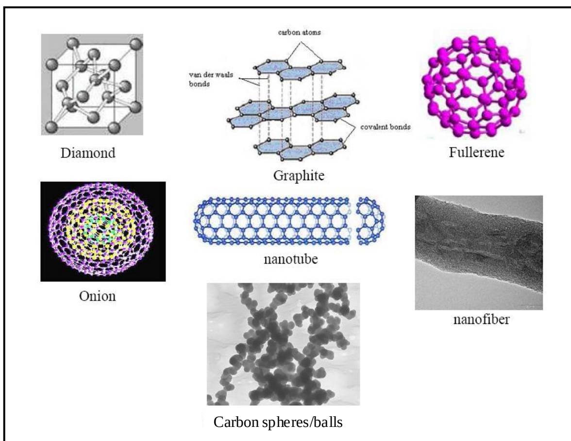
Figure 2.8: Carbon allotropes [128].
