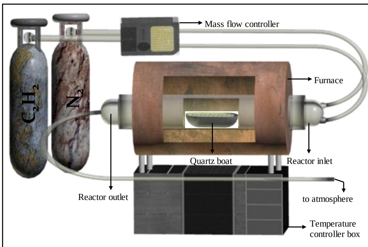
Figure 3.1: The horizontal CVD set up for the synthesis of carbon nanotubes
