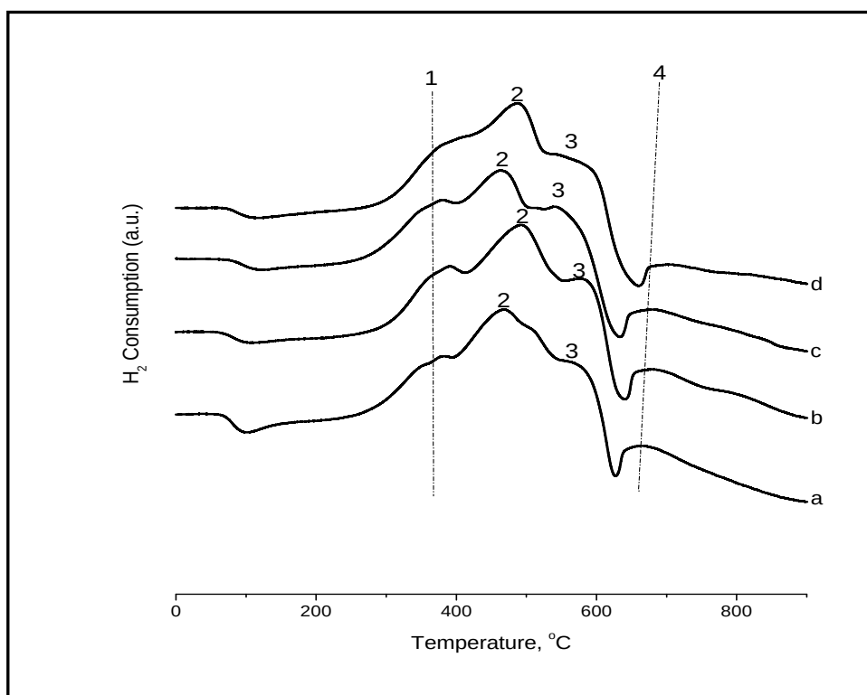
Figure 7.12: H 2 -TPR profiles of the unpromoted and Na-promoted Fe-catalysts supported on CNTs: a) 100Fe/CNT, b) 100Fe-3.35Na/CNT, c) 100Fe-12Na/CNT; d) 100Fe-24Na/CNT.
