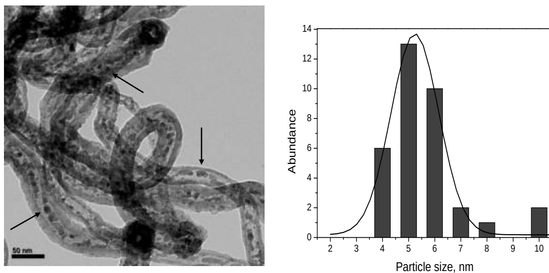
Figure 6.5: TEM image with arrows indicating the Fe particles, and Fe particle size histogram for the Fe-nitr catalyst.
