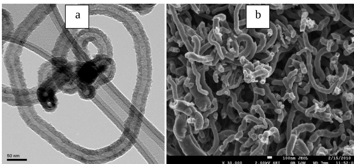
Figure 7.2: Purified CNTs a) TEM, b) SEM
