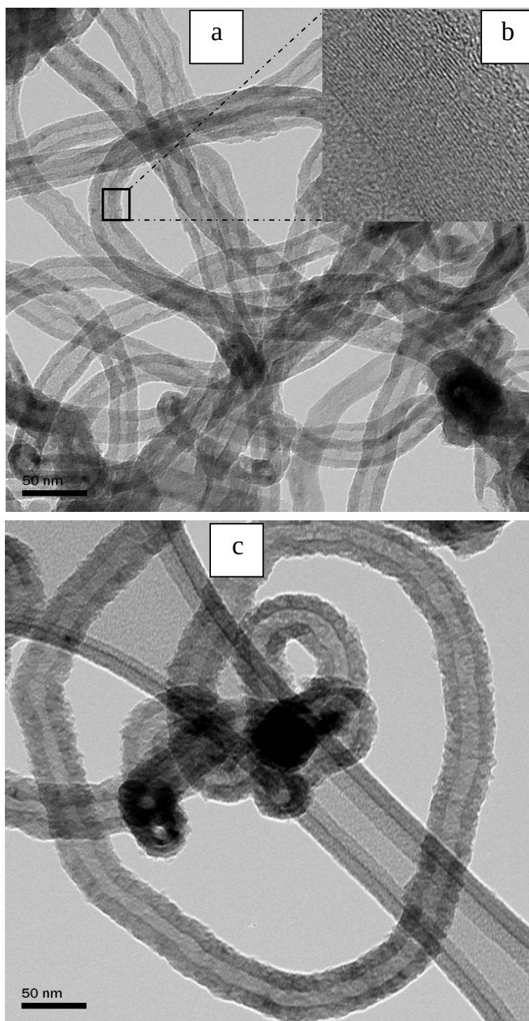
Figure 9.1: (a) TEM image of as-grown CNTs; (b) HRTEM of CNTs showing multi-walls and (c) TEM image of purified CNTs
