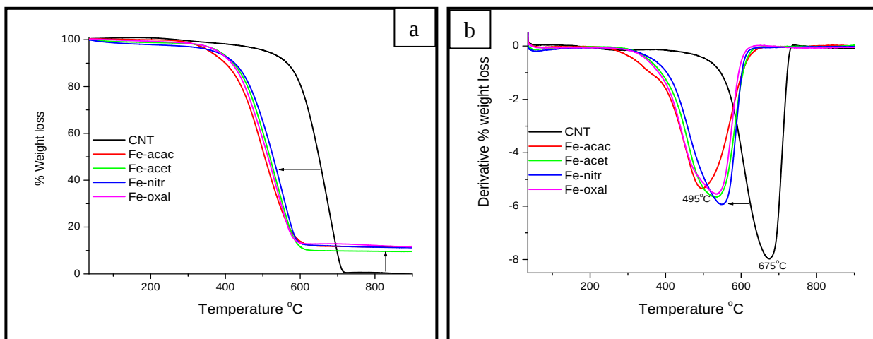
Figure 6.13: a)-TGA and b)-DTA of Fe-acac, Fe-acet, Fe-nitr and Fe-oxal.
