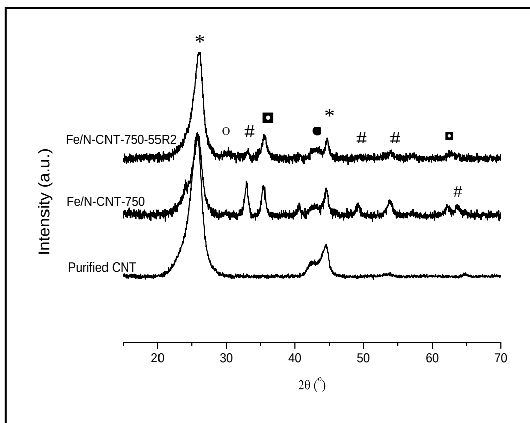
Figure 8.9: XRD patterns of the purified CNTs and Fe supported on N-CNTs: * = graphite; o = \text{Fe}_3\text{O}_4 ; # = \text{Fe}_2\text{O}_3 ; ■ = \text{Fe}_2\text{O}_3 and \text{Fe}_3\text{O}_4 ; ● = Co-Fe, \text{Fe}_3\text{C} , \text{Co}_3\text{C} or \text{Co}_2\text{C} [33, 34].
