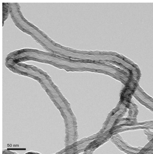
Figure 6.3: TEM image of CNTs after reflux in 55% HNO 3 for 2 h
