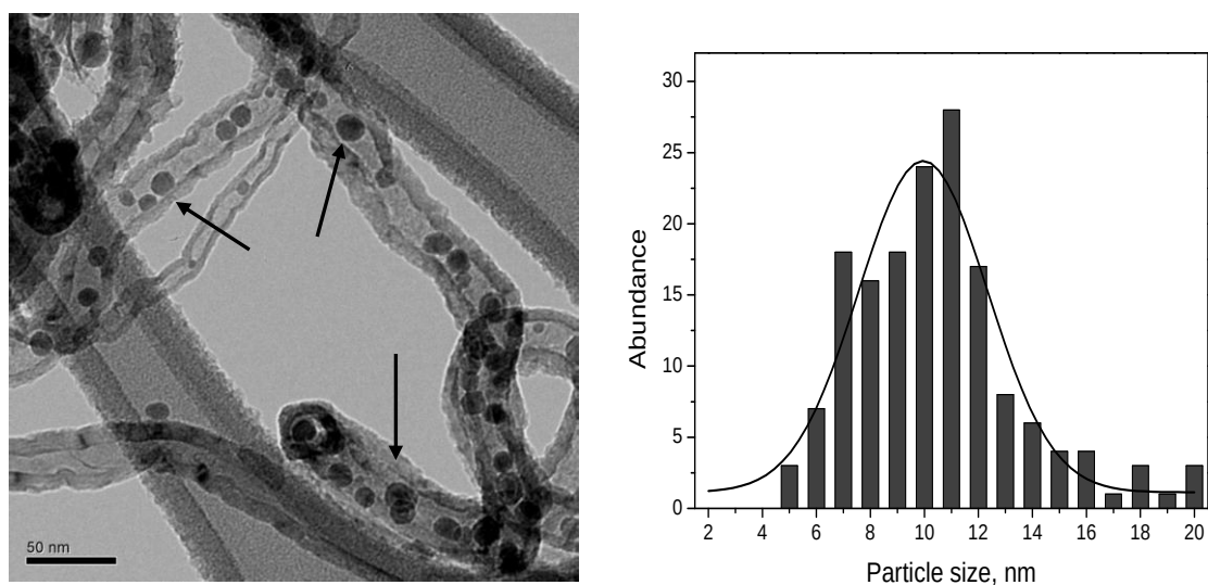
Figure 6.18: TEM image with arrows indicating the Fe particles, and Fe particle size histogram for the Fe-nitr-1 after 120 h time on stream (particle size: 7-14 nm).
