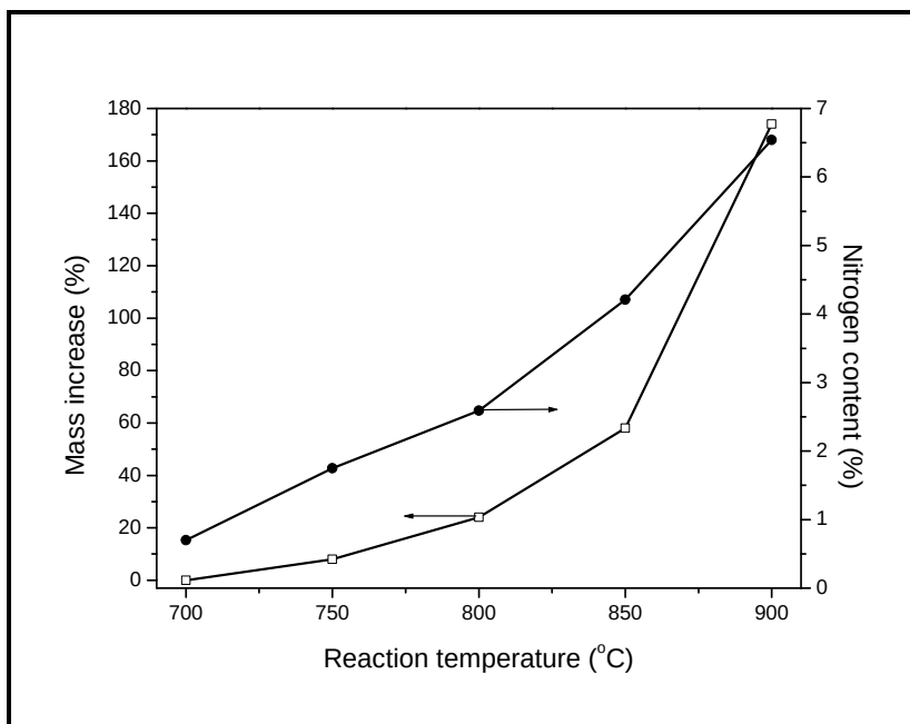
Figure 8.1: Dependence of the % mass increase and nitrogen content in N-CNTs on reaction temperature
