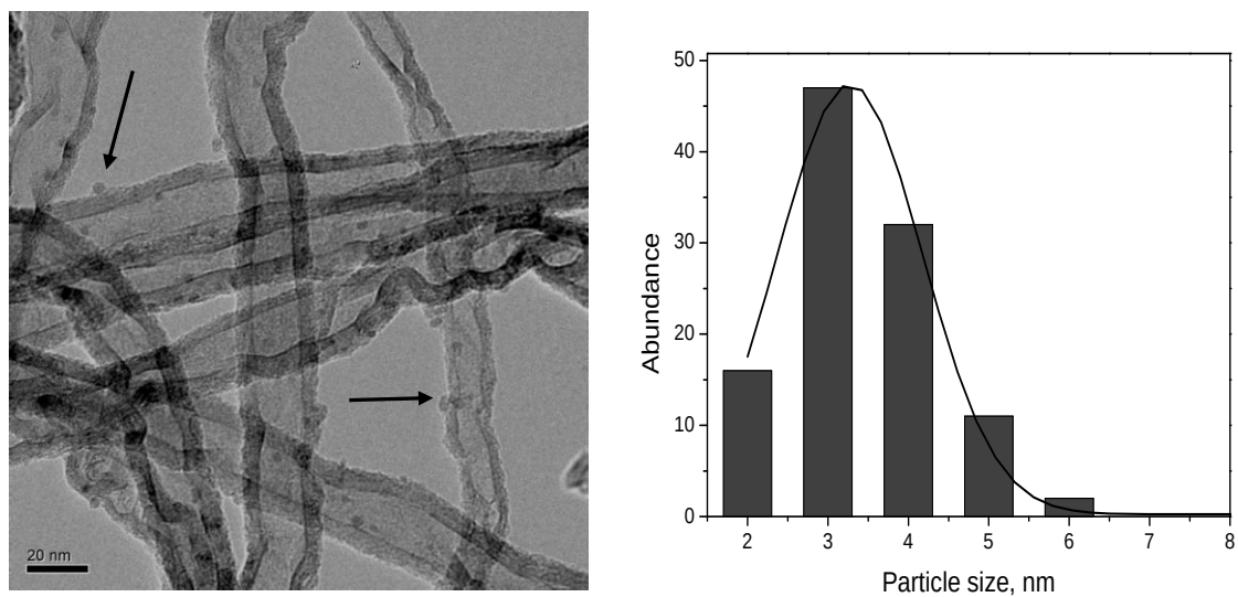
Figure 6.7: TEM image with arrows indicating the Fe particles, and Fe particle size histogram for the Fe-acet-1 catalyst.
