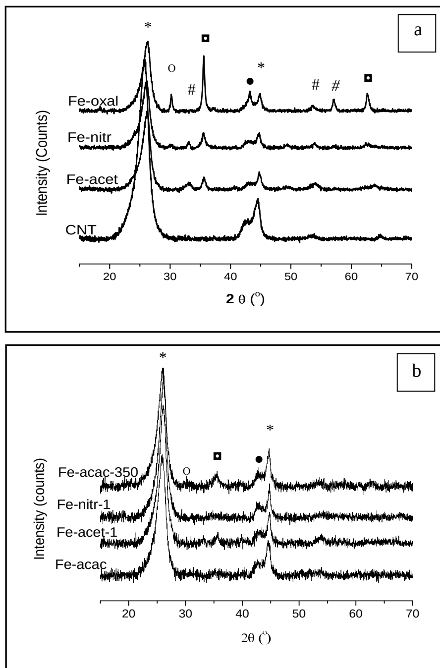
Figure 6.1: XRD data of Fe/CNT catalysts prepared using different iron precursors and either a) water or b) acetone as solvents: * = graphite; o = \text{Fe}_3\text{O}_4 ; # = \text{Fe}_2\text{O}_3 ; ■ = \text{Fe}_2\text{O}_3 and \text{Fe}_3\text{O}_4 ; • = Co-Fe, \text{Fe}_3\text{C} , \text{Co}_3\text{C} or \text{Co}_2\text{C} [13, 27]
