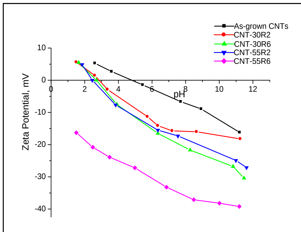
Figure 5.5: Zeta potential measurements of as-grown and acid treated CNTs as a function of pH.
