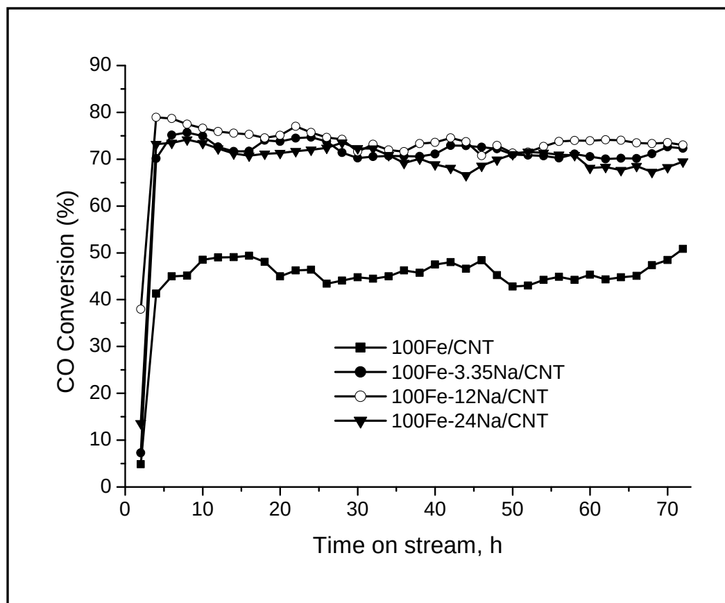
Figure 7.13: CO conversion versus time on stream for unpromoted and sodium promoted Fe/CNTs catalysts.
