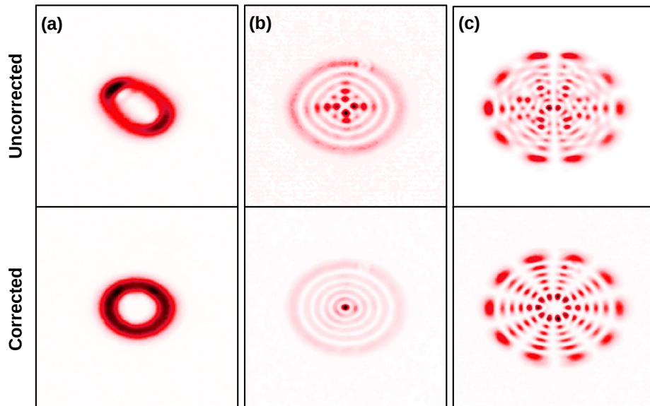
Fig. 2.12 The effect of the aberration correction procedure for the 3000 series DMD. The top row shows: (a) an LG_5^0 ; (b) an LG_0^5 ; and (c) a superposition of an LG_5^5 and LG_{-5}^5 beam. The bottom row shows the beams after correction. The colourmap is the same as that used in Fig. 2.9.
