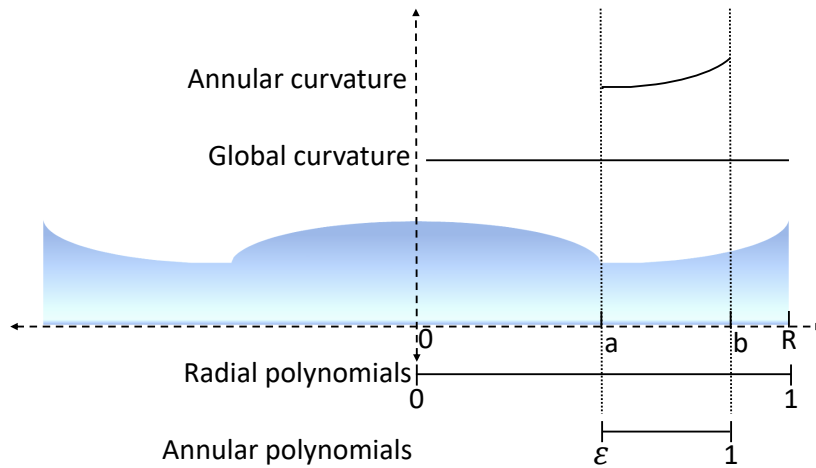
Fig. 4.6 A convergent lens embedded in the centre of a divergent lens. The global curvature over the radius for which the Radial Zernike polynomials are defined is flat. The annular region [\epsilon, 1] over which the Annular Zernike polynomials are defined retains its local curvature.
