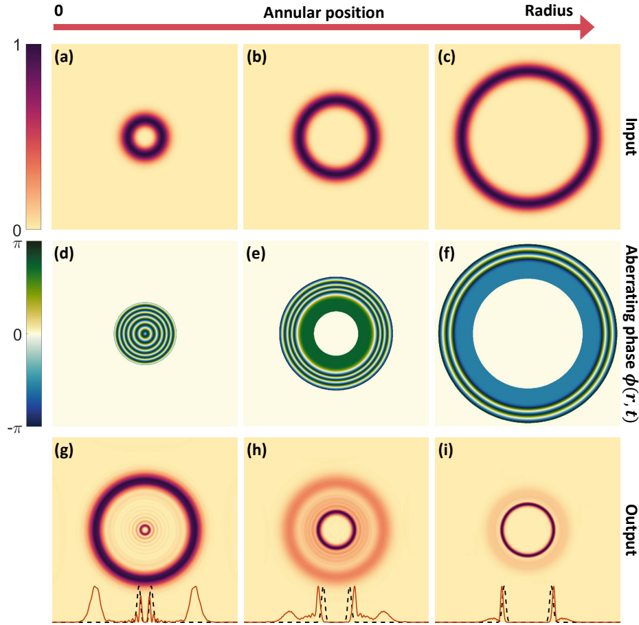
Fig. 4.7 (a),(b) and (c), input LG beams spatially matched to annular heat sources with an outer boundary at \omega = 0.3 \times, 0.5 \times , and 0.83 \times R of a rod. (d),(e) and (f), the phase profiles associated with the heat sources as described by the Annular Zernike polynomials. (g),(h) and (i), the intensities of the aberrated input beams at the focal plane of a lens, the inset line plots show the unaberrated and aberrated profiles as black dashed and orange solid lines respectively. Note that the output beams have been independently normalised to aid in the visualisation.
