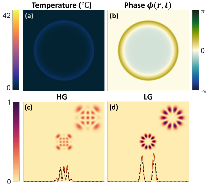
Fig. 4.13 The global action of an annular source on superpositions of HG (c) and LG (d) beams. (a) the temperature u(r, t) of the rod for an annular heat source at its radius. (b) the aberrating phase \phi(r, t) of the hologram. The insets in (c) and (d) show the input beams. The line plots show the profiles of unaberrated beams and the measured beams as black dashed and orange solid lines respectively.
