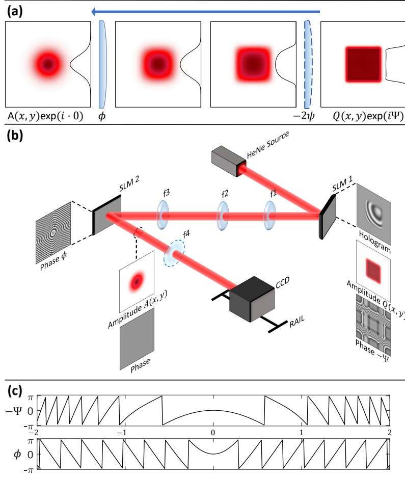
Fig. 3.7 (a) A step-wise depiction of the two-step approach corresponding to the subsequent panels. (b) The experimental setup consisted (conceptually) of two SLMs to implement the desired phase transformations. SLM 1 acted as the second phase element creating a beam of amplitude Q(x, y) with phase -\psi . The beam passed through a lens f_1 and was imaged ( f_2 and f_3 ) onto the first phase element (SLM 2) with phase \phi . The final beam, having a Gaussian amplitude A(x, y) and a flat phase front was imaged by a camera. (c) The phase profiles -\psi and \phi encoded on SLM 1 and SLM 2 respectively. The elements match the case depicted in panels (a) and (b) and are plotted on a shared transverse axis in millimetres.
