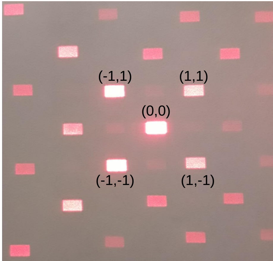
Fig. 2.4 The observed diffraction pattern for the TI 3000 DMD aligned at an incident angle of 0 rad with all mirrors in the on state. Note that the diffraction orders labelled (-1, 1) and (-1, -1) are brighter than those labelled (1, 1) and (1, -1) .
