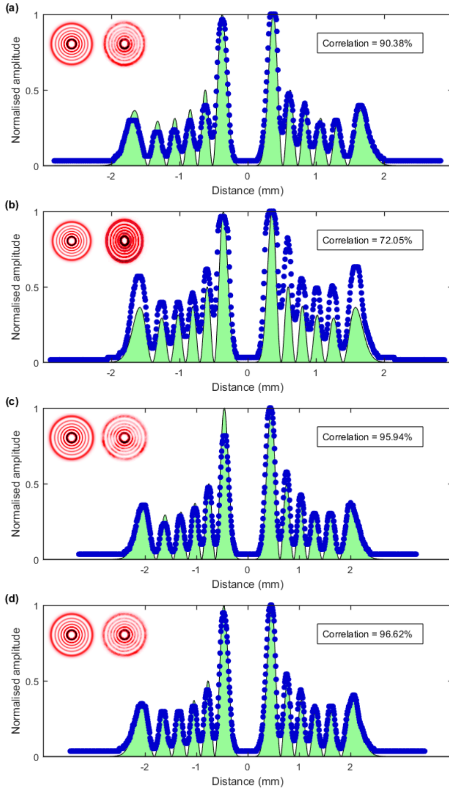
Fig. 2.10 Correlation between the theoretical (green solid) and experimental (blue dots) LG_5^5 beam for both alignments and encoding schemes. The inset shows a side by side comparison of the beams with the ideal beam on the left and the measured beam on the right. (a) the initial encoding scheme at an angle of 0 rad. (b) the initial encoding scheme at an angle of \pi/15 rad. (c) the optimised encoding scheme at an angle of 0 rad. (d) the optimised encoding scheme at an angle of \pi/15 rad.
