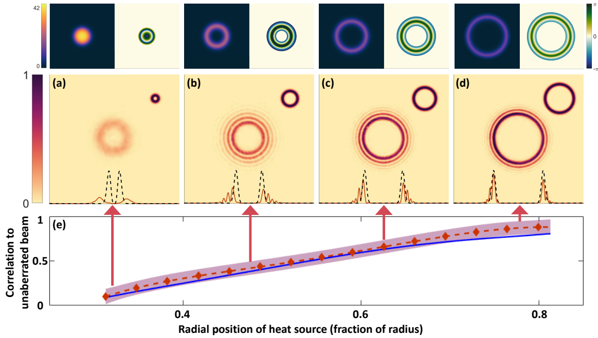
Fig. 4.11 The self action of an annular heat source on an LG beam. The upper insets show the temperature of the rod u(r, t) and aberrating phase \phi(r, t) of the hologram. Panels (a) through (d) show the measured beams for an annular source with its outer edge at \omega = 0.31 \times , \omega = 0.47 \times , \omega = 0.64 \times and \omega = 0.81 \times R respectively. The insets in these panels show the input beams. The line plots show the profiles of an unaberrated beam and the measured beams as black dashed and orange solid lines respectively. Panel (e) shows the correlation between the measured beam and the simulation of an unaberrated beam as a function of heat source position. The red dashed line indicates the line of best fit for the experimental data with the shaded region indicating the 95% confidence interval. The blue solid line is the theoretical prediction.
