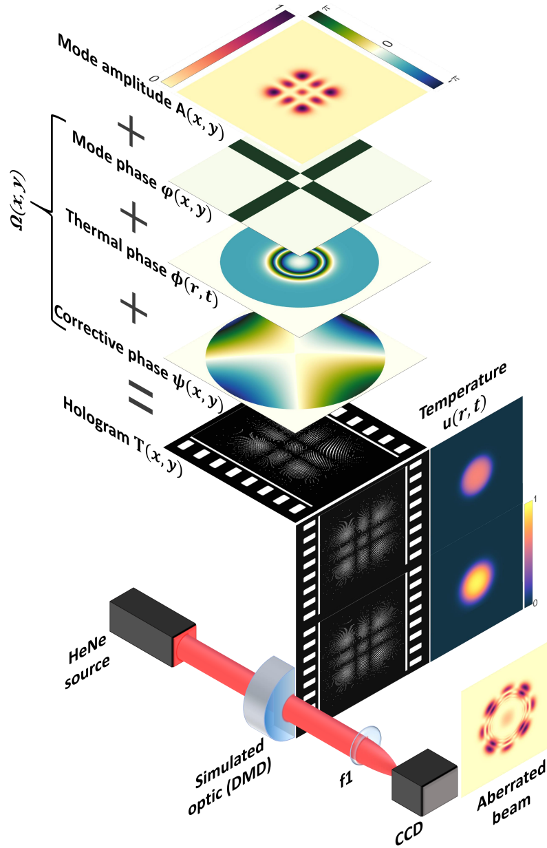
Fig. 4.9 The experimental setup shown conceptually. The DMD was used as though it was an old film projector, i.e. dynamically simulating the heated optic by displaying an ordered set of holograms corresponding to the temperature profile of the optic. Each hologram encodes an amplitude A(x, y) and a phase, where the total phase \Omega(x, y) is made up of three components: the phase inherent to the desired mode \varphi(x, y) ; the phase of the thermal aberration \phi(r, t) , and the corrective phase accounting for the deformations to the DMD \psi(x, y) . A well expanded and collimated beam from a HeNe source was incident on the DMD. The beams created by the holograms were recorded at the focal plane of a lens by a camera.
