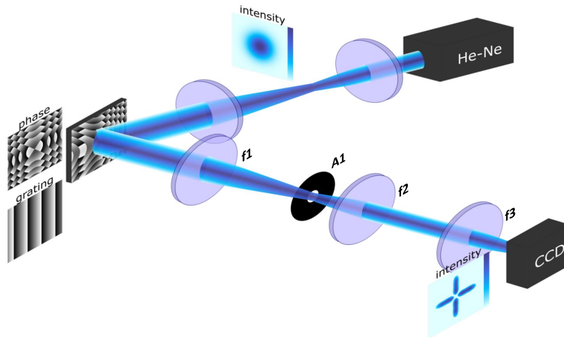
Fig. 3.3 Conceptual design of the experimental setup used to implement the method. A well expanded and collimated beam from a HeNe source was incident on the SLM. The beam from the SLM passed through lens f_1 forming the desired profile |Q(x)|^2 at the plane of the black aperture A_1 . The plane of A_1 was imaged to camera by a 4f system (lenses f_2 and f_3 ). Here, the second beam shaping element described in Sec. 3.2.3 would be placed at the plane of the black aperture A_1 .
