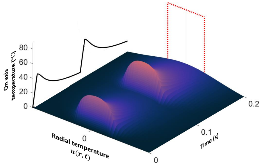
Fig. 4.2 The spatial and temporal temperature profile of a Tm:YLF rod with a central quasi-continuous uniform-intensity source, where each pulse lasts 0.01 s with a 0.09 s cooling period. The raised panels at the boundaries of the surface plots show line plots of the on axis temperature over time for the uniform-intensity source together with the structure of the heat source (red dotted).
