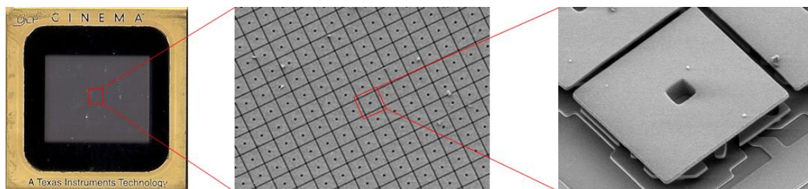
Fig. 1.5 The structure of the mirror array of a DMD. Panel 2 and 3, micrographs courtesy of University of Rochester/URnano.
