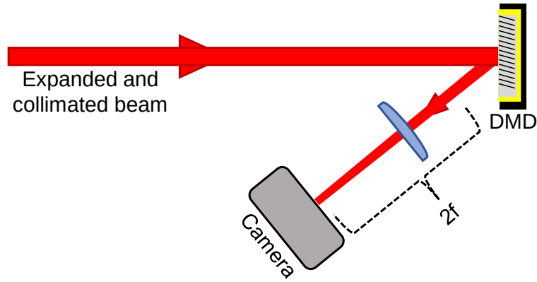
Fig. 2.11 The setup to demonstrate the efficacy of the wavefront correction method. An expanded and collimated beam was incident on a DMD. The first order holographic diffraction was then focused through a lens. A camera was placed at the focal plane of the lens.
