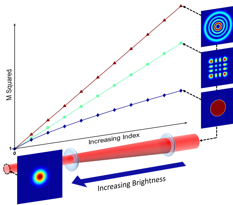
Fig. 3.6 The beam quality of structured light fields decreases with increasing mode index (see Table. 1.1), resulting in an increase in the beam quality factor, M^2 , shown here for the examples of Hermite-Gaussian, Laguerre-Gaussian and Super-Gaussian beams, with the mode index plotted as 2m + 2n + 1 , 2p + |\ell| + 1 and k , respectively. By using the lossless reshaping technique presented in the first part of the chapter it is possible to move ‘down the curve’ towards a Gaussian ( M^2 = 1 ) using an optical system with two phase-only elements, thus enhancing the brightness, shown here conceptually.
