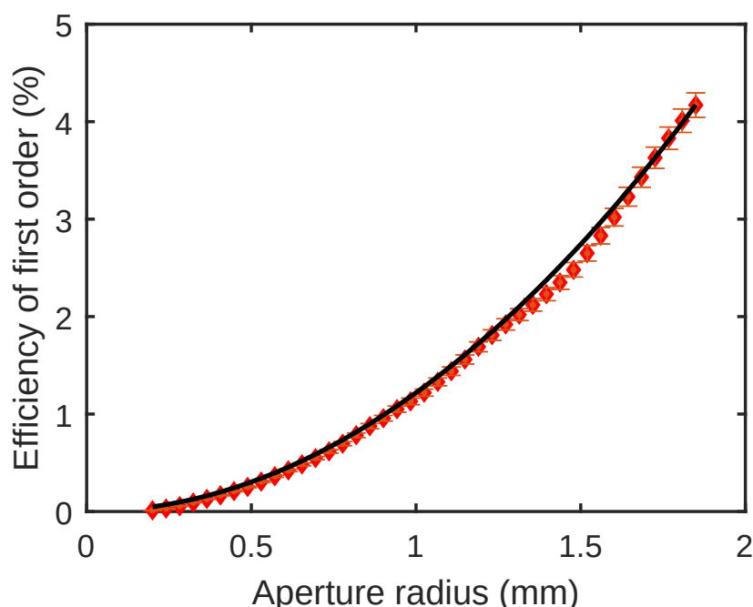
Fig. 2.7 Efficiency of the first order holographic diffraction as a function of aperture radius. The black line is predicted by Eq. 2.19 based on the number of mirrors in the on state in the hologram. The red diamonds are the experimentally measured values.
