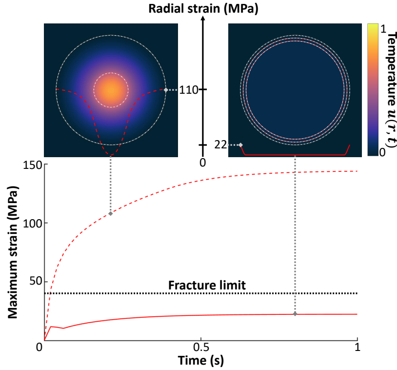
Fig. 4.4 The stress experienced by a rod when heated by a central (red dashed) and annular (solid red) source. The insets show: the temperature profile of the rod at 0.25 s and 0.75 s; the concentric circles indicate the boundary of the rod and the location of the heat source; and the line plots show the radial stress profile.
