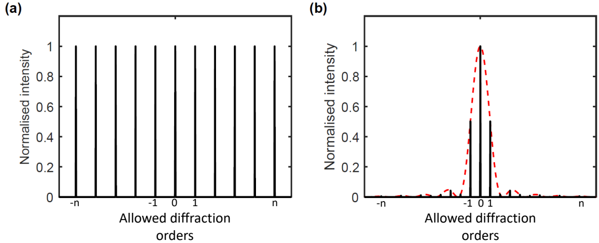
Fig. 2.3 (a) The set of diffraction peaks allowed by the second sinc factor in each summation. (b) Shows how the envelope function (in red) defined by \text{sinc}(w \frac{m}{\Delta}) modulates the intensity of the allowed peaks to produce the observed diffraction pattern.
