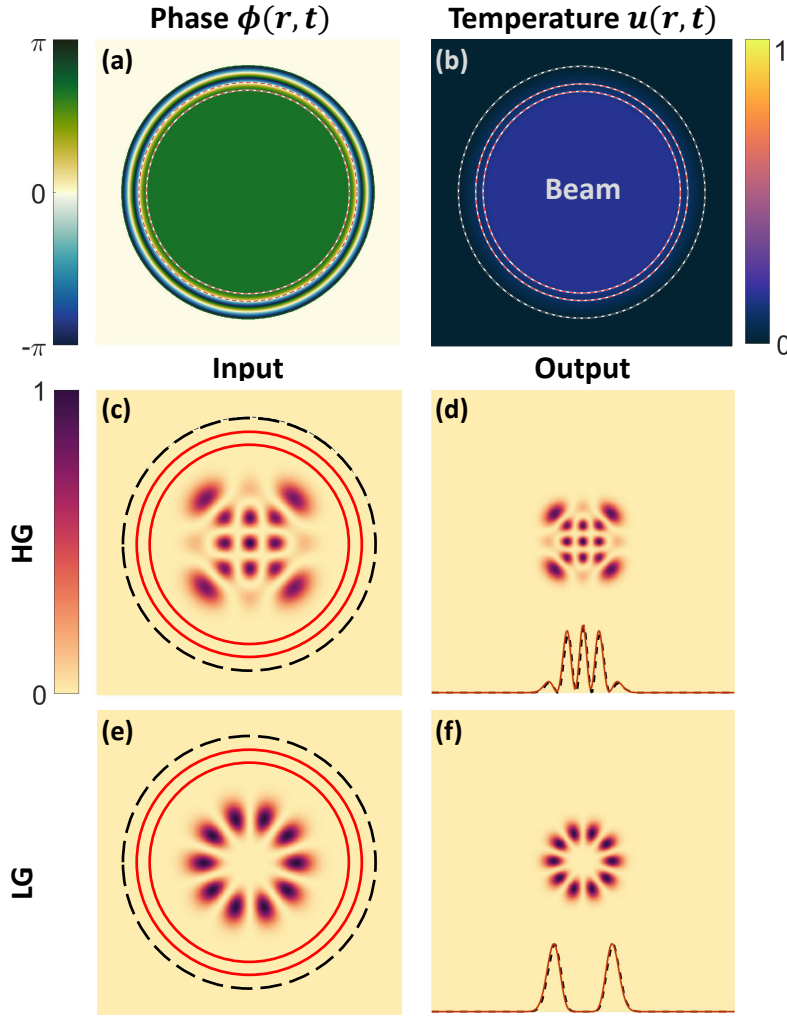
Fig. 4.8 (a) and (b), the aberrating phase \phi(r, t) and corresponding temperature u(r, t) for a heat source with \omega = 0.86 \times R . The outermost black dashed circle indicates the radius of the rod. The annular heat source is indicated by the two innermost red circles. (c) and (e), the super-positions of HG and LG beams respectively. (d) and (f) the intensities of the beams at the focal plane of a lens. The inset line plots show the unaberrated and aberrated profiles as black dashed and orange solid lines respectively.
