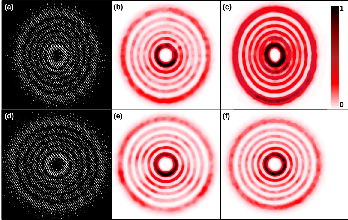
Fig. 2.9 (a) the computed hologram as displayed on the DMD screen. (b) the measured beam with the DMD aligned at 0 rad. (c) the measured beam with the DMD aligned at \pi/15 rad, when using the initial encoding scheme. (d), (e) and (f) show the same but using the optimised encoding.
