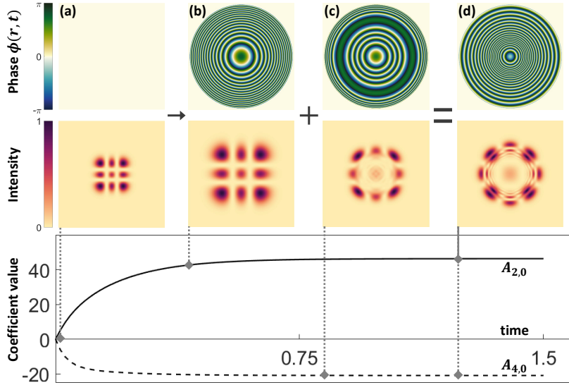
Fig. 4.3 The values of the A_{2,0} and A_{4,0} Zernike coefficients over time. The insets show the intensity (at the focal plane of a lens) and the aberrating phase \phi(r, t) for: (a) The unaberrated HG mode; (b) The A_{2,0} aberration on the HG mode; (c) The A_{4,0} aberration on the HG mode, and (d) The cumulative effect of all A_{\tilde{n},0} coefficients.
