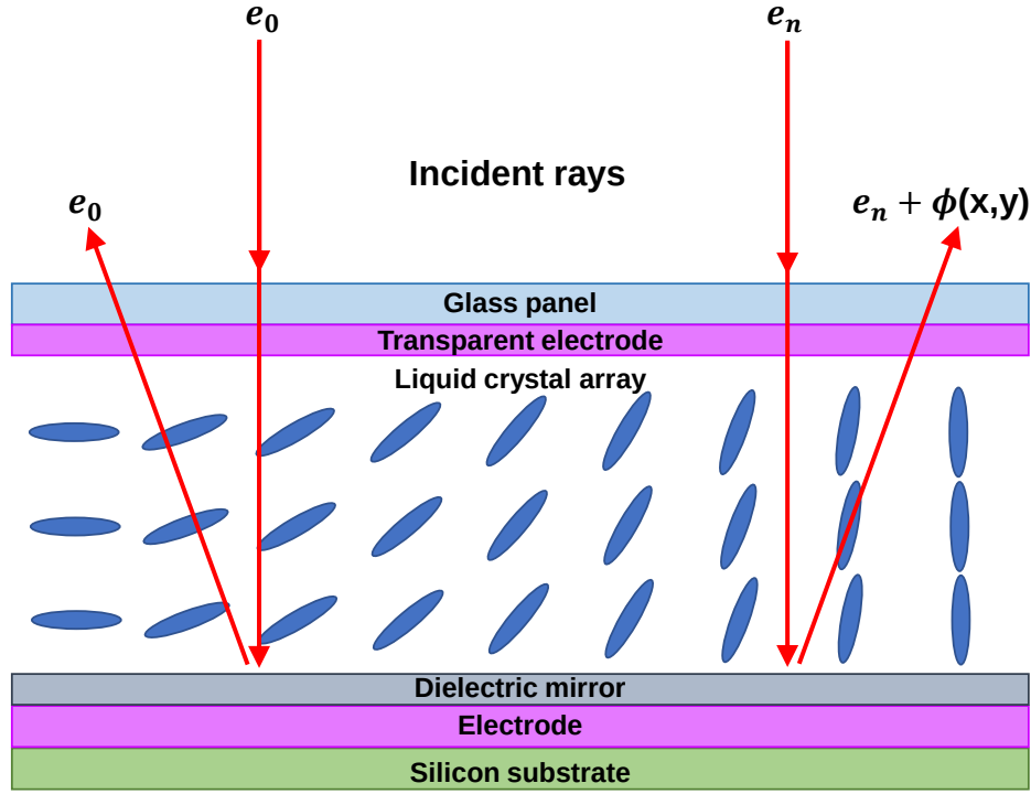
Fig. 1.4 A conceptual cross section of a LCoS SLM. For an incident beam with polarisation components e_0 and e_n a spatially variable phase delay \phi(x, y) can be imparted to one polarisation component of the beam by rotating the liquid crystals.
