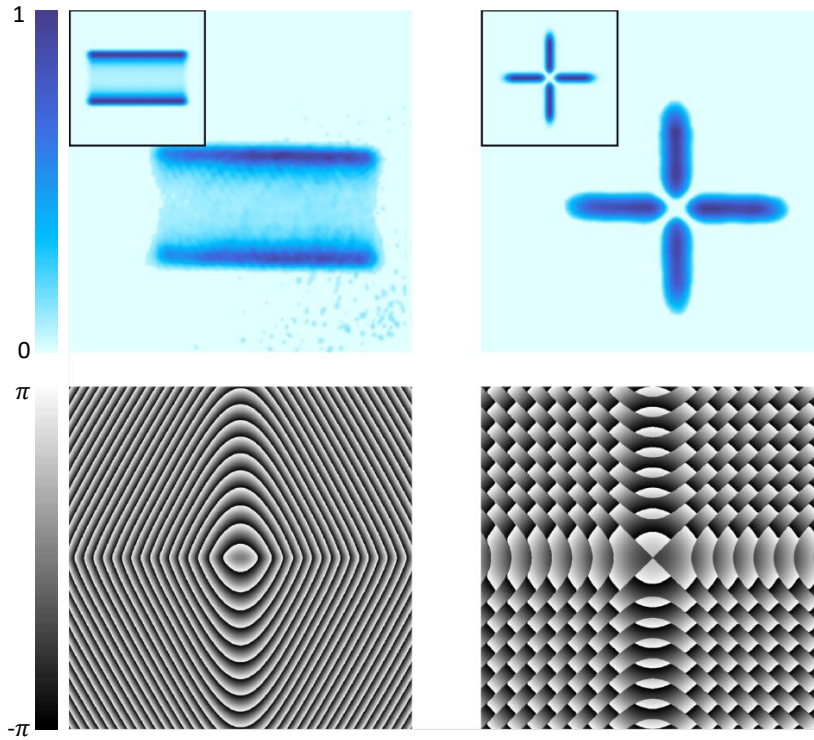
Fig. 3.5 The 'double bar' and 'cross hair' profiles. These profiles are the result of superpositions of modes at right angles to each other in a Cartesian symmetry.
