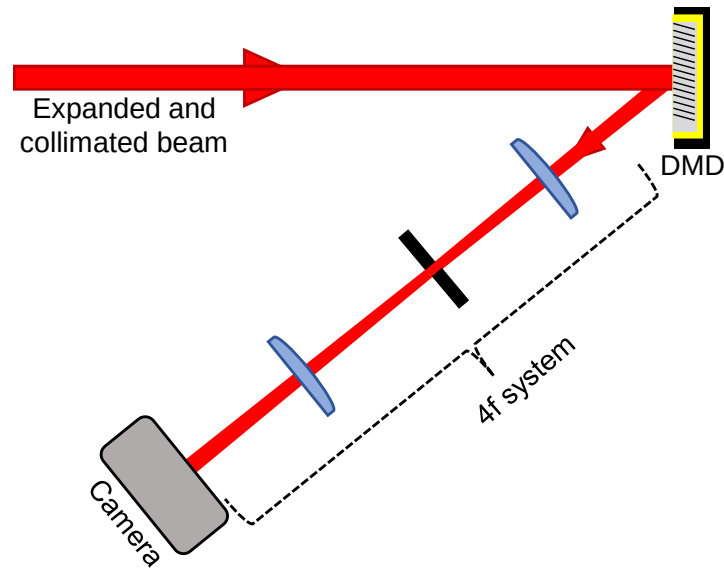
Fig. 2.8 To determine the mode quality, an expanded and collimated beam was incident on a 3000 series DMD. The holographic first order diffraction was then imaged, via a 4f system to a camera.
