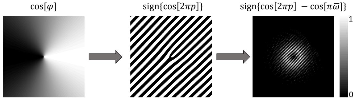
Fig. 1.7 The transmission function derived by Eq. 1.41 for an LG_1^0 beam. Note how in comparison to Fig. 1.3 the transmission function is binarised, i.e. equals either 0 or 1.
