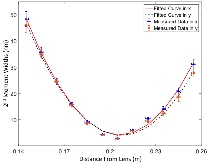
Fig. 3.9 The 2 nd moment width for the Gaussian beam as a function of propagation distance from the focusing lens, shown as measured data and fitted curves. Fitting the data to the equation W^2(z) = W_0^2 + (M^2)^2 \times [\lambda / (\pi W_0)]^2 (z - z_0)^2 allows the unknown parameters to be inferred, including the M^2 . This example plot is for the radial Super-Gaussian to Gaussian case and shows a beam quality factor improvement from M^2 = 3.64 to M^2 = 1.06 \pm 0.05
