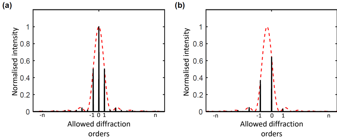
Fig. 2.5 (a) The relationship between the envelope function (in red) and the allowed diffraction orders for a pure amplitude grating. Note how in (a) the envelope function is fixed around the zero order diffraction peak. (b) The effect of decoupling the envelope function from the zero order. Energy can now be moved into the first order diffraction without changing the relative positions of the orders in space.
