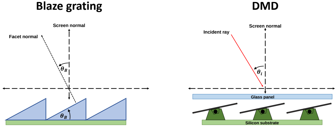
Fig. 2.1 A comparison between a blaze grating (left) and a DMD with the mirrors in the on state (right). The tilt angle \theta_B and the incident angle \theta_i are measured relative to the screen normal of the DMD with counter-clockwise as the positive direction.
