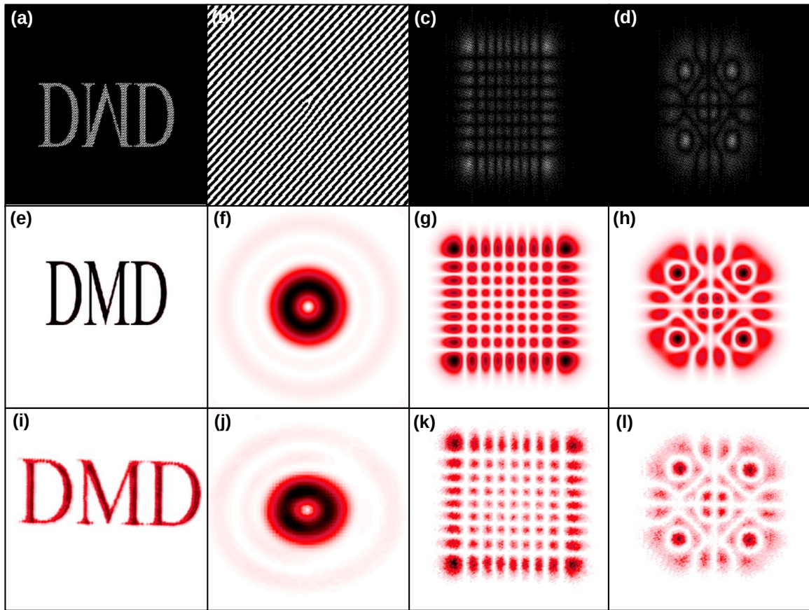
Fig. 2.14 (a), (b), (c) and (d) show the computed holograms to generate: the text "DMD" using amplitude only modulation; a phase singularity at the focal plane of a lens; an HG_8^8 mode using complex amplitude modulation; and a superposition of an HG_3^7 and an HG_7^3 mode using complex amplitude modulation. Note the apparent elongation of the holograms, this is a result of the optimised encoding scheme used to generate the holograms. When displayed on the DMD, the pixel arrangement of the screen causes the holograms to be drawn out to the correct aspect ratio. (e), (f), (g) and (h) show the intended intensity profiles of the beams generated by the holograms in the first row. (i), (j), (k) and (l) show the experimentally measured beams.
