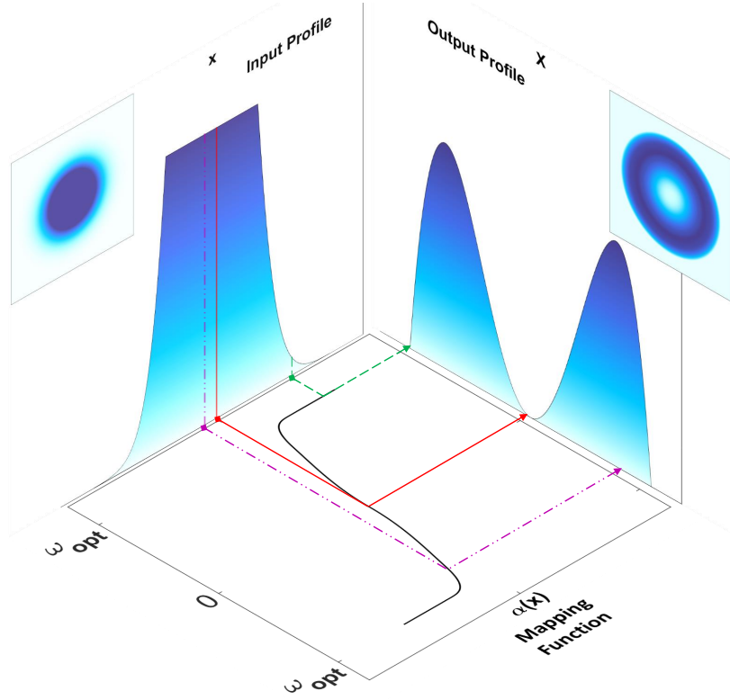
Fig. 3.2 The mapping function \alpha for a truncated Gaussian input to an annular polynomial output. The insets show the intensities of the input and output beams while the panels show the beam profiles.
