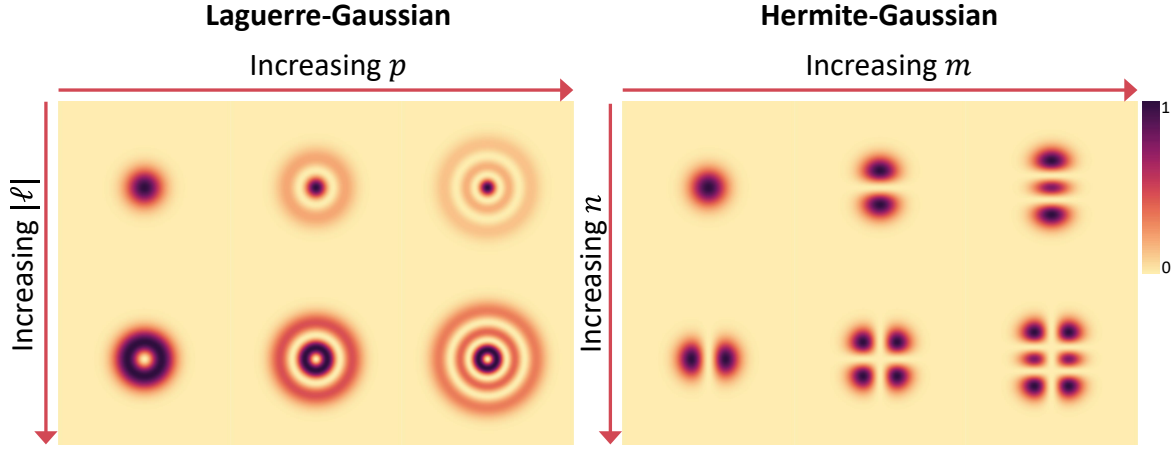
Fig. 1.1 Left, intensities of LG beams for \ell \in [0, 1] and p \in [0, 2] . Right, intensities of HG beams for n \in [0, 1] and m \in [0, 2] . For \ell = p = m = n = 0 both the HG beams and LG beams reduce to a Gaussian beam.
