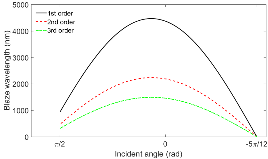
Fig. 2.2 The incident wavelength required to blaze the 1st, 2nd and 3rd order diffractions as a function of incident angle for a mirror tilt angle of \theta_B = \pi/15 and N = 1/7.6 \times 10^{-3} .
