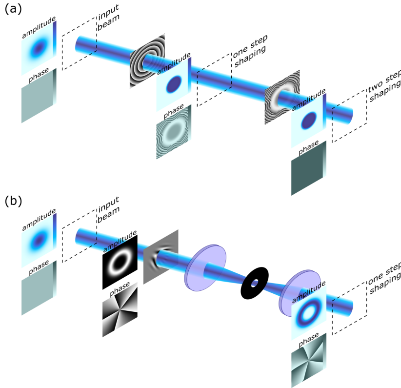
Fig. 3.1 The different approaches to creating structured light. Panel (a) shows how lossless single-step shaping can be achieved using a phase-only element, but requires the phase at the target plane to be left as a free DoF, requiring a second element for correction. Panel (b) shows how a single step in which the amplitude of the beam is also controlled can produce ideal structured light, but now the process is lossy.
