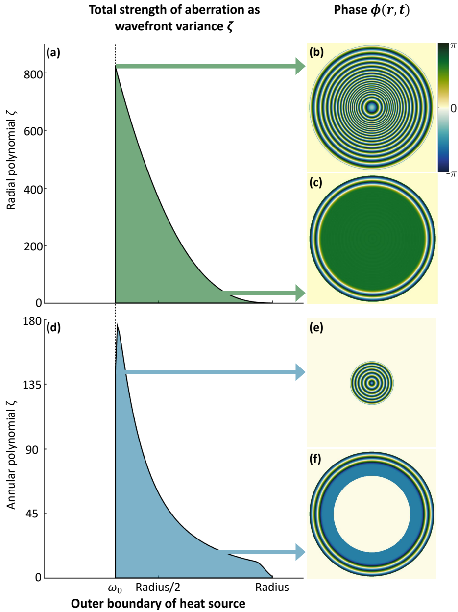
Fig. 4.14 The relationship between total aberration strength calculated as wavefront variance \zeta and the outer boundary of the heat source for the Radial (a) and Annular (d) Zernike polynomials respectively. The phase panels (b), (c), (e) and (f) show the phase aberration in each basis at the points indicated by the arrows. \omega_0 represents the minimum outer boundary for a heat source of width \omega_0 .
