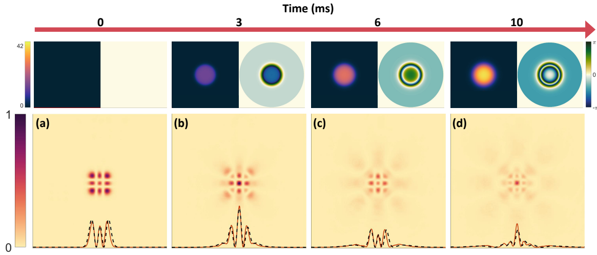
Fig. 4.10 The self action of a central heat source on an HG beam over time. The upper insets show the temperature u(r, t) of the modelled rod and the aberrating phase \phi(r, t) of the hologram. The main panels show the measured beam at four points in time, (a) at t = 0 , (b) at t = 3 , (c) at t = 6 , and (d) at t = 10 ms respectively. The line plots show the profiles of the simulated beam and the measured beams as black dashed and orange solid lines respectively.
