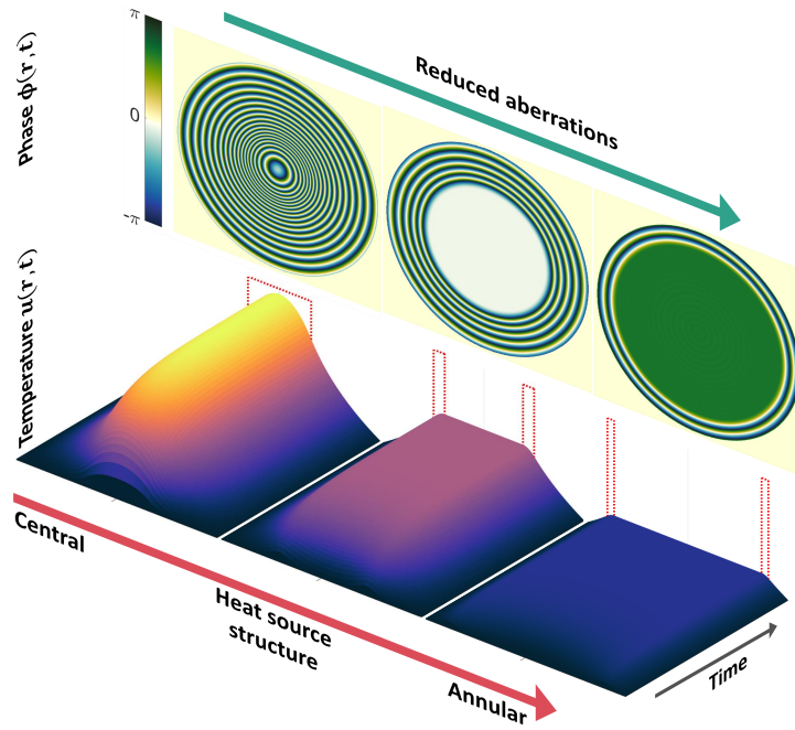
Fig. 4.5 The temperature u(r, t) and phase \phi(r, t) profiles for a rod in an annular heating regime. As the source approaches an annular ring at the radius of the rod, an area of constant phase develops in the centre of the rod, reducing aberrations.
