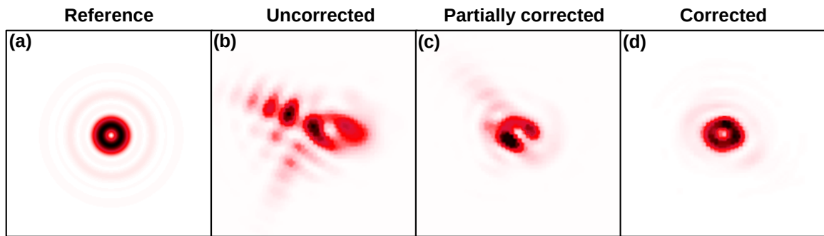
Fig. 2.13 Experimental aberration correction of the 6500 DMD. (b) The initial beam aberration is too large for the algorithm to handle, the first order astigmatism was manually corrected for. (c) The partially corrected beam after the manual aberration correction. After this, the intermediate beam can be fed through the G-S algorithm to find the remaining phase distortions. (d) The corrected beam.
