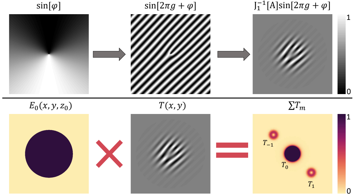
Fig. 1.3 Top, the transmission function derived by Eq. 1.29. The azimuthal phase \varphi(x, y) is combined with a diffraction grating g(x, y) yielding a characteristic ‘forked’ (i.e. bifurcating) grating. The inclusion of the J_1^{-1}[A(x, y, z_0)] component modulates the transmission function by the amplitude A(x, y) . Bottom, the effect of the transmission function on a uniform initial field E_0(x, y, z_0) . The desired LG_1^0 beam forms in the first order diffraction T_1 . The conjugate order T_{-1} creates a beam with the conjugate of the desired phase, in this case producing a LG_{-1}^0 .
