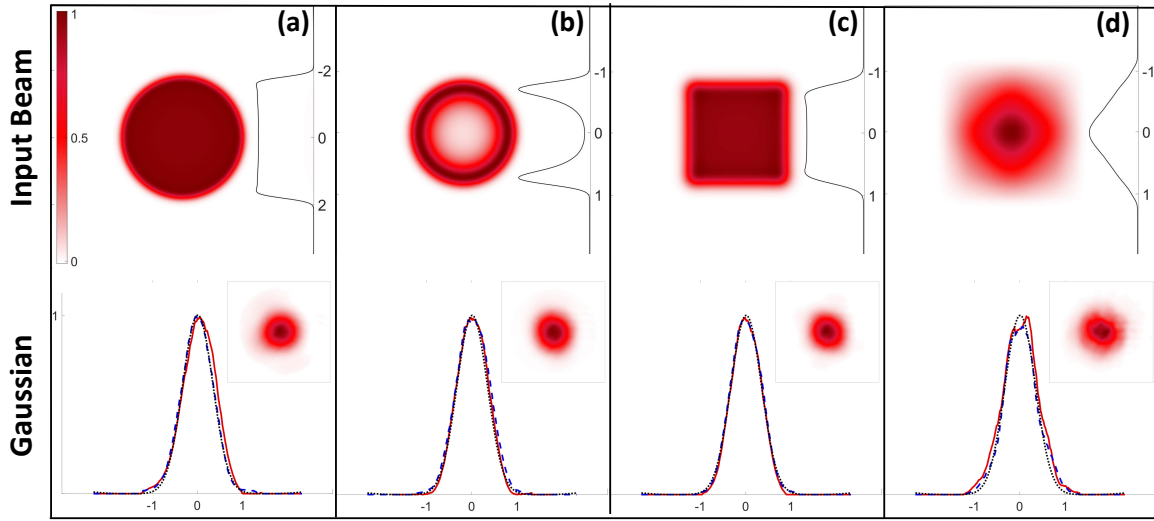
Fig. 3.8 Input beams shown as an intensity and profile, each with a flat phase, and the measured Gaussian output beam, shown for the four tested cases: (a) radial Super-Gaussian, (b) radial annulus, (c) Cartesian Super-Gaussian and (d) Cartesian linear, a beam with a linear intensity gradient. The examples cover Radial and Cartesian symmetry in high M^2 initial beams. The Gaussian beams are shown as cross-sectional profiles for x (blue dashed) and y (red solid), with the black dotted profiles as the theoretical prediction. The insets show the measured camera intensities. All profiles are plotted on an axis in millimetres.
