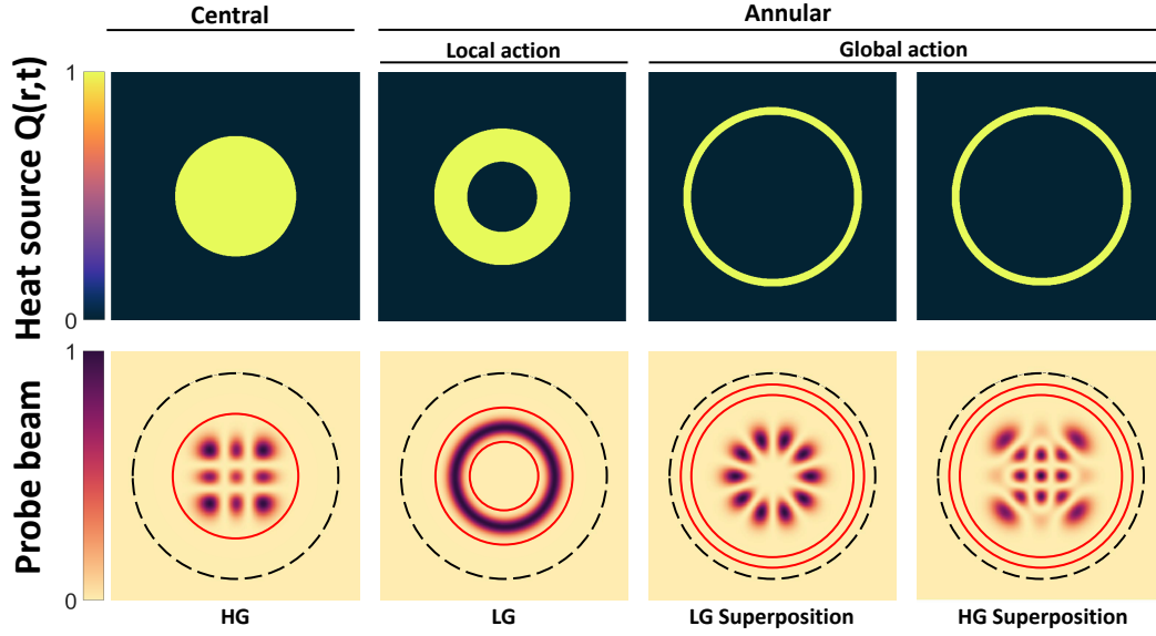
Fig. 4.1 The cases this chapter examines. The analysis makes use of an abstract heat source Q(r, t) and probe beams. The heat source is separated into two categories, central and annular. The annular case is further divided into two sub categories, the local action and the global action. The local action refers to an examination of the thermal phase-only within the annular region under heating, while the global action refers to the examination of the thermal phase for the entire optic. The red circles indicate the location of the heat source relative to the probe beam while the dotted black line indicates the circumference of the optic. The central heat source is probed with an HG beam. The local action of the annular source is probed with an LG beam. The global action of the annular source is probed with both superpositions of LG and HG beams.
