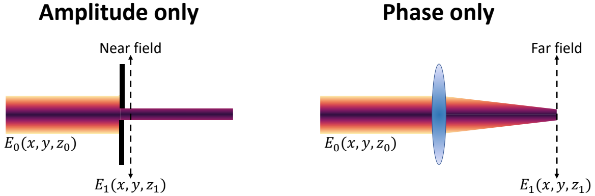
Fig. 1.2 Left, an amplitude-only transformation using an aperture which resizes a beam in the near field. Right, a phase-only transformation using a lens which resizes the beam in the far field.
