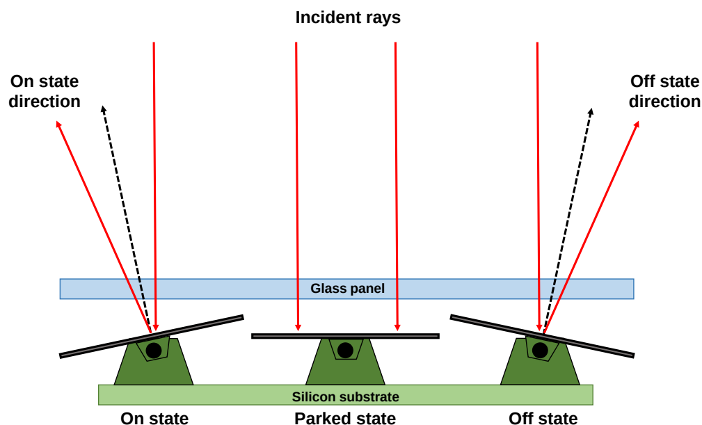
Fig. 1.6 A conceptual representation of the three possible mirror states: on; parked; and off.
