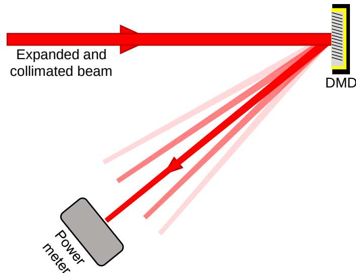
Fig. 2.6 The experimental setup used to verify the treatment of the DMD presented in Sec. 2.2.2. An expanded and collimated beam was incident onto a DMD and the power of the relevant diffraction order was measured by a power meter.
