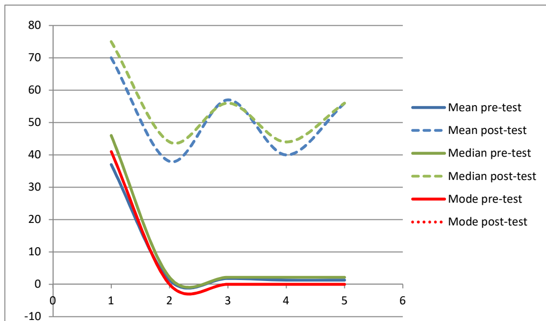
Figure 4.5 Comparison between the mean, median and mode of the pre-test and the post-test
