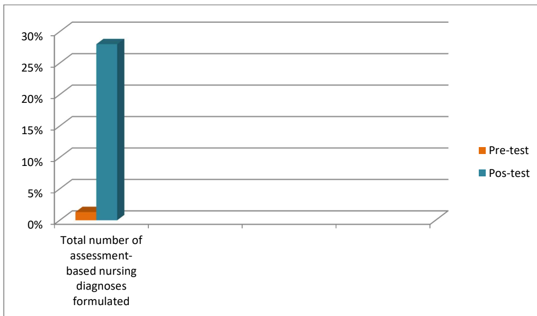
Figure 4.4 Comparison between the total numbers of assessment-based nursing diagnoses formulated by the participants in the pre-test and post-test
