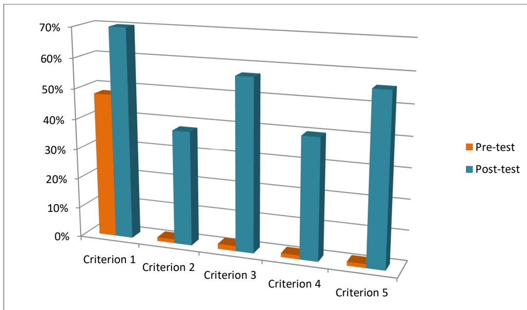
Figure 4.3 Comparison between pre-test and post-test criteria
