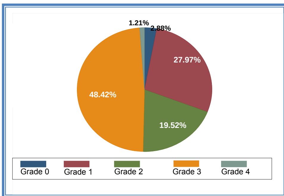
Figure 3.1: Prevalence of BV per BV Ison and Hay diagnosis grade in 1066 HIV negative women at enrolment into an HIV prevention trial in KwaZulu Natal
