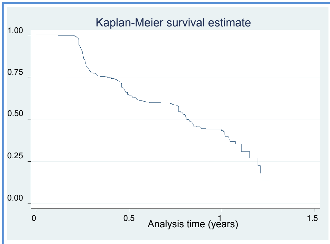
Figure 3.2: Kaplan Meier curve of time to first BV episode in women who were BV negative at enrolment into a microbicides trial in rural KwaZulu Natal.
