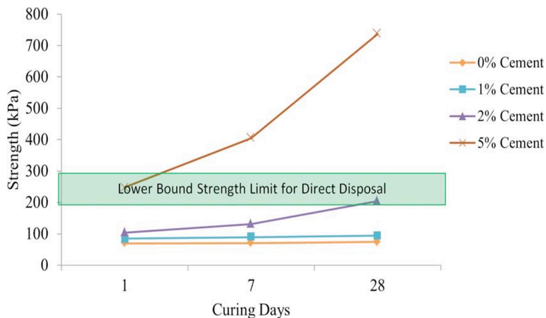
Graph 2: Compressive strength of cemented waste after one, seven and 28 days.
