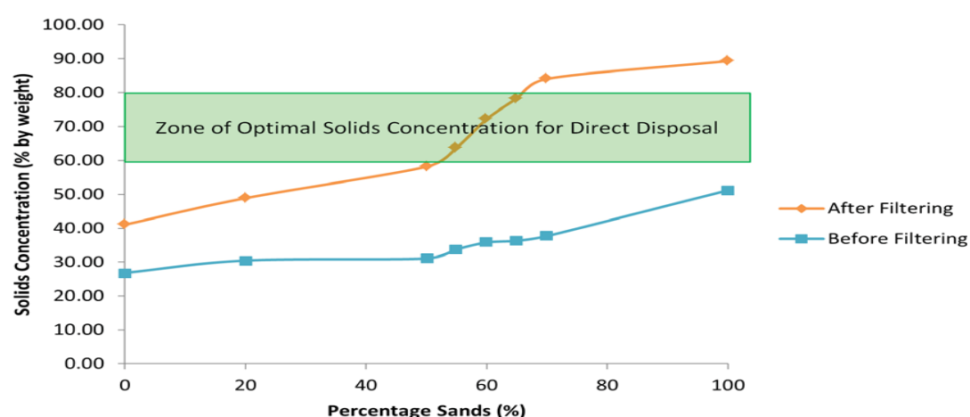
Graph 1: Effects of filtering on solids concentration of heavy mineral sand tailings
