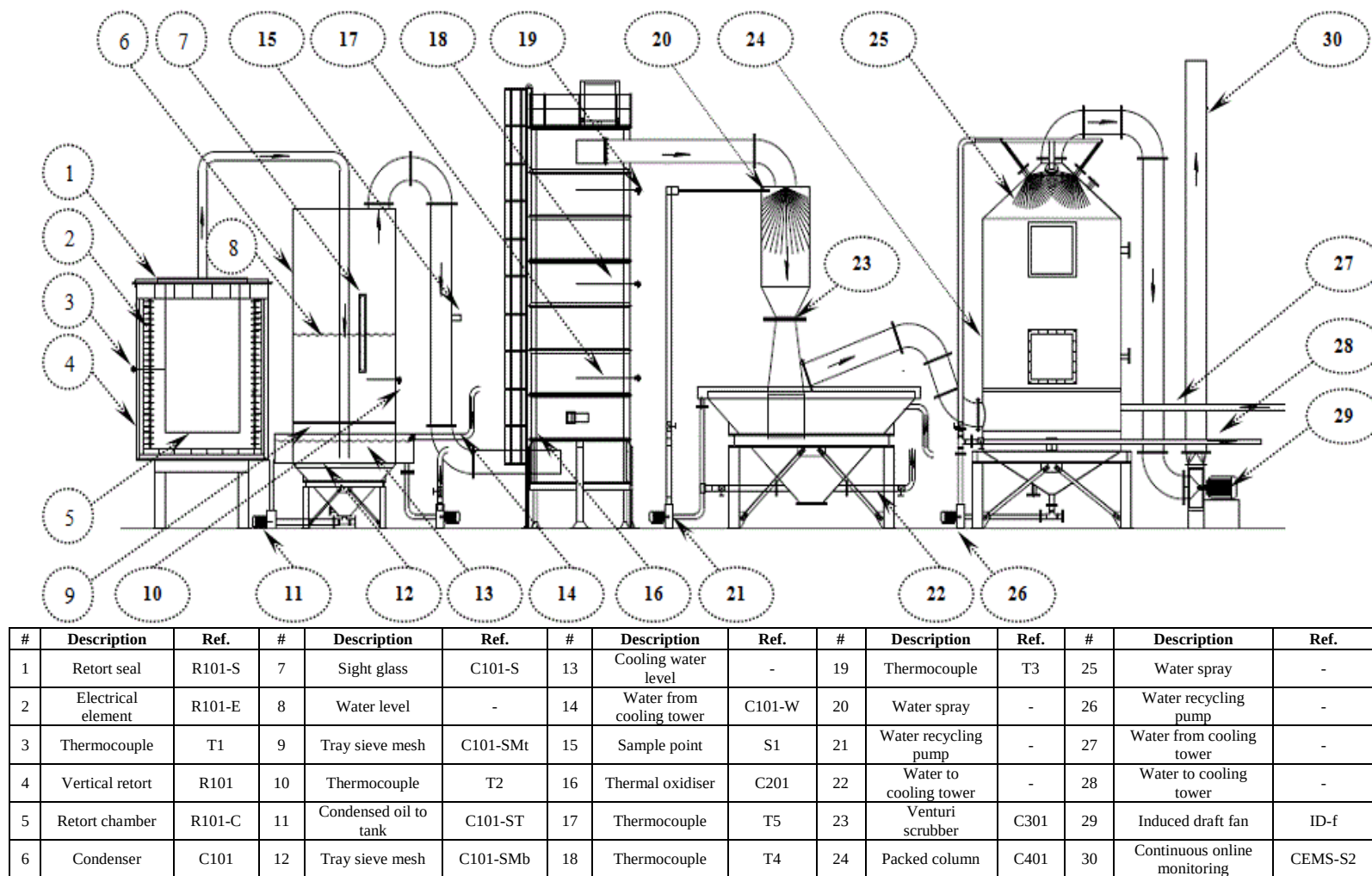
Figure A1 Experimental apparatus designed from key operational criteria ( elements, functions and critical parameters )
