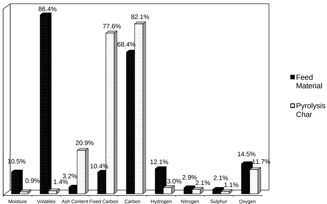
Figure 4.5 Comparison of proximate & ultimate analyses of original feed material and carbon char product
