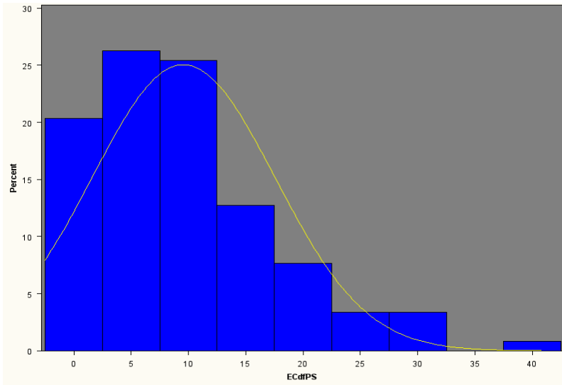
Figure 3 Ethical Climate fit difference measure distribution
