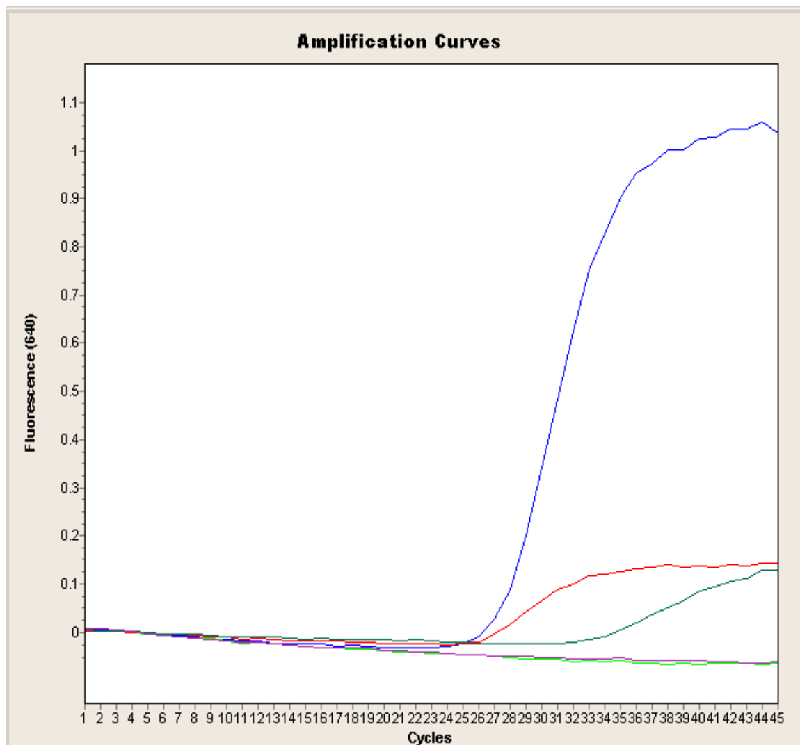
Figure 3.1 Target amplification curves for controls and representative patients
