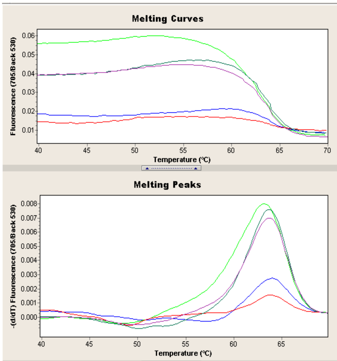
Figure 3.4 Internal Control melting curves and melting peaks
