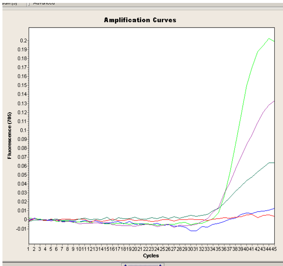
Figure 3.3 Internal Control amplification curves
