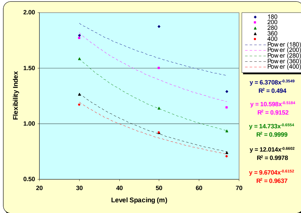
Figure 6.20: Variation of flexibility index with level spacing
