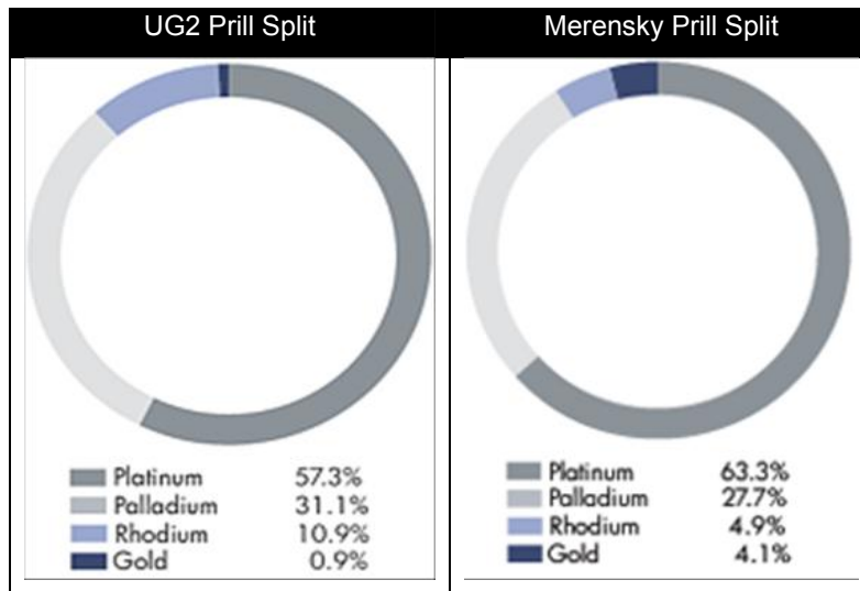
Figure 4.4: Typical average 4E prill splits for UG2 and Merensky reefs (Source: Impala Platinum, 2008; Impala Platinum, 2009)
