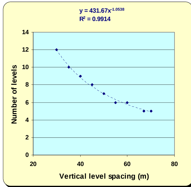
Figure 6.4: Variation of number of levels with increasing vertical level spacing
