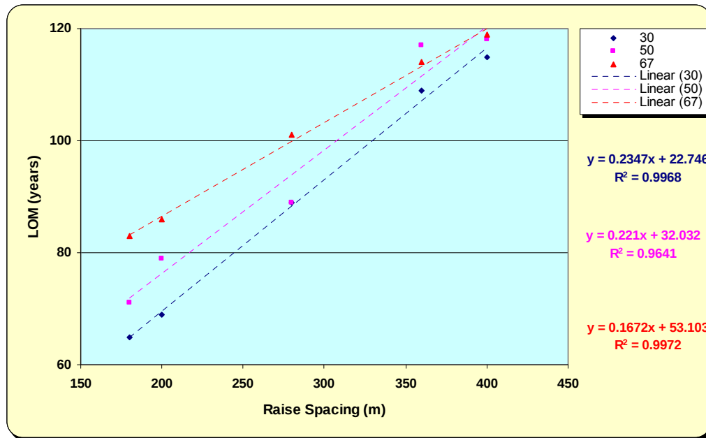
Figure 6.25: Variation of LOM with increasing raise spacing
