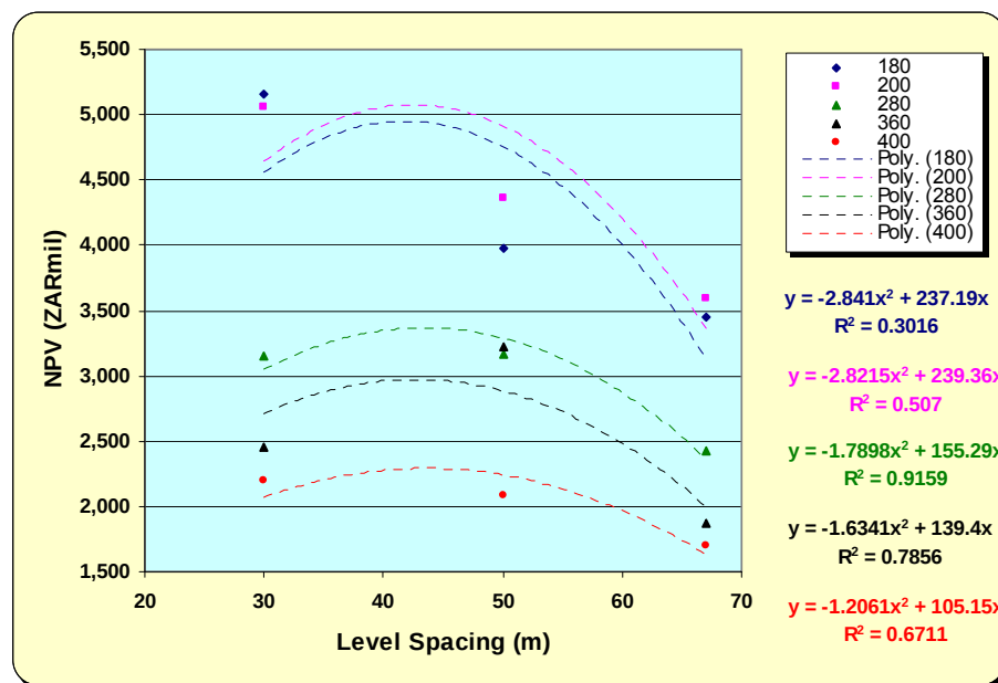
Figure 6.9: Variation of project NPV with increasing level spacing
