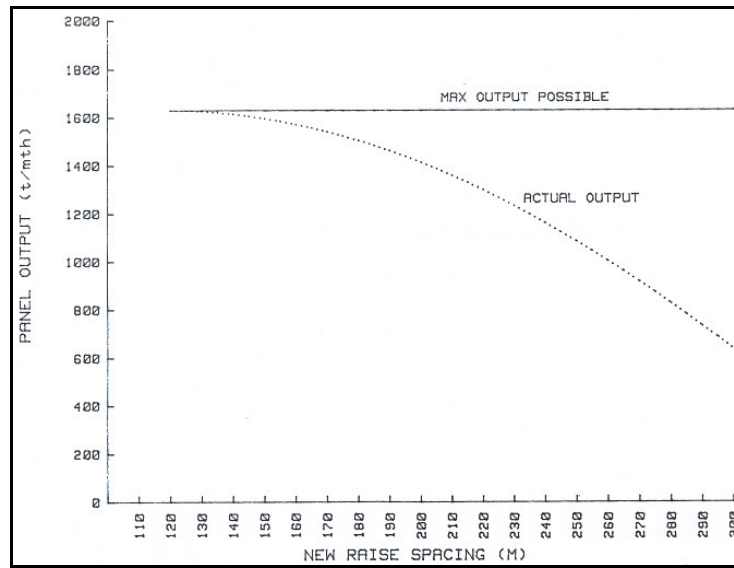
Figure 2.6: Convex quadratic relationship between panel productivity with raiseline spacing (Lawrence, 1984)
