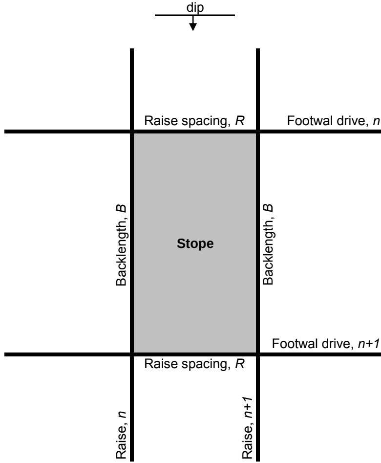
Figure 5.11: Stope blocked out by two consecutive raiselines and two consecutive levels
