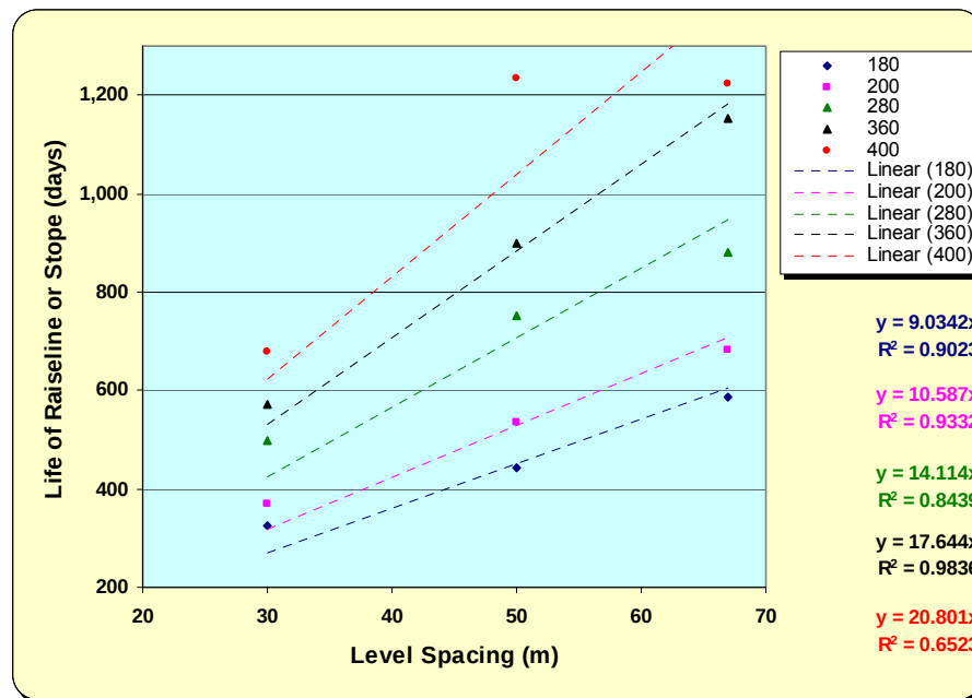
Figure 6.22: Variation of life of raiseline with increasing level spacing
