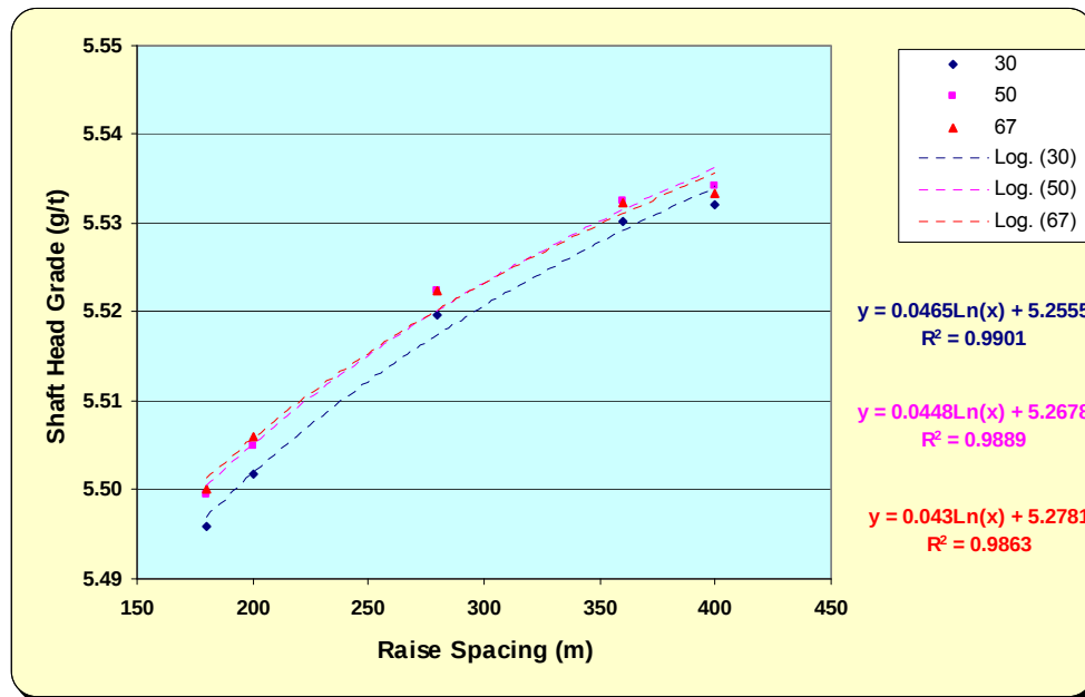
Figure 6.15: Variation of shaft head grade with increasing raise spacing
