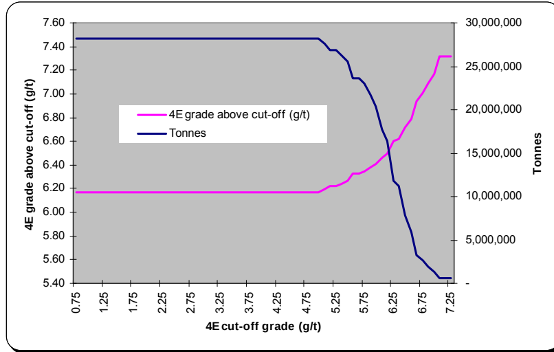
Figure 4.11: Grade-tonnage curve for OB1
