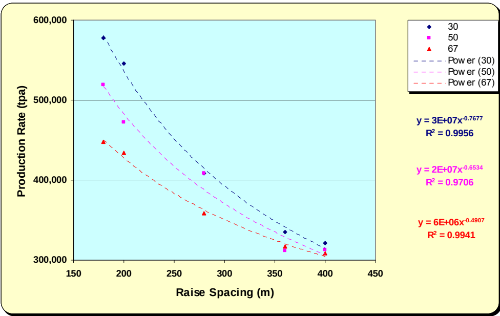
Figure 6.19: Variation of production rate with increasing raise spacing
