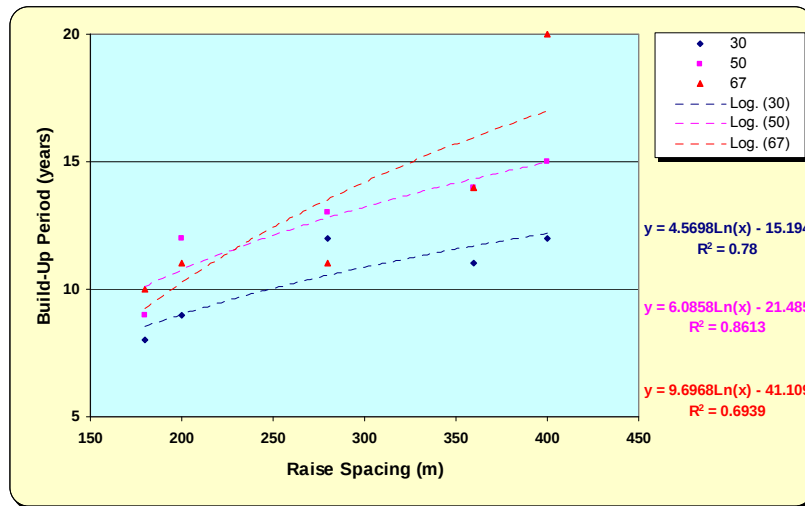
Figure 6.27: Variation of build-up period with increasing raise spacing
