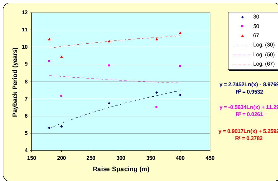
Figure 6.12: Variation of payback period with increasing raise spacing
