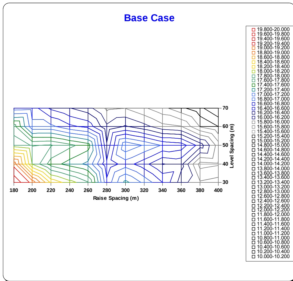
Figure 7.1: A 3-D Excel surface contour plot of the AHP priority score for the base case
