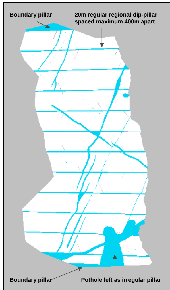
Figure 5.10: A Mine2-4D® illustration of the 67_400 layout showing stoping areas (in white), regular pillars and geological structures left as irregular pillars (in blue).
