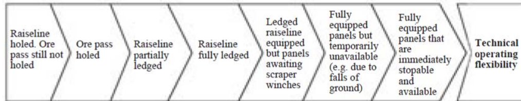
Figure 3.1: Sequence of typical mining phases in the build-up to technical operating flexibility
