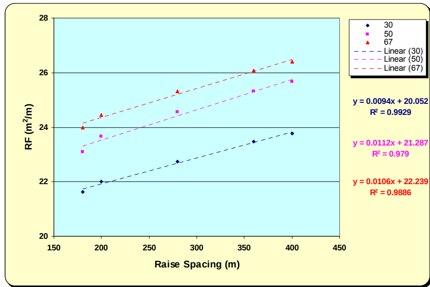
Figure 6.14: Variation of RF with increasing raise spacing
