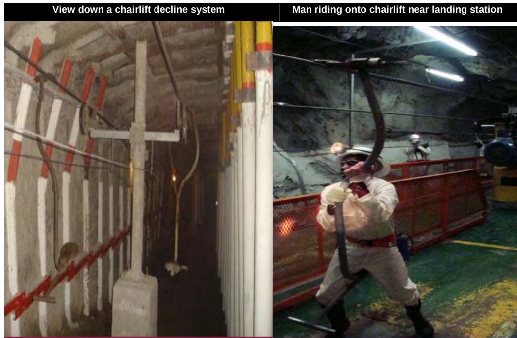
Figure 5.3: Photos taken underground illustrating a chairlift decline
