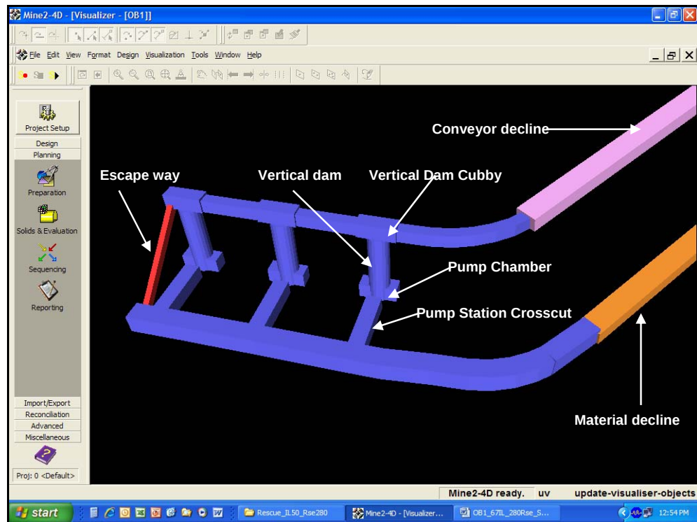
Figure 5.6: Mine2-4D® illustration of water reticulation infrastructure at bottom of OB1
