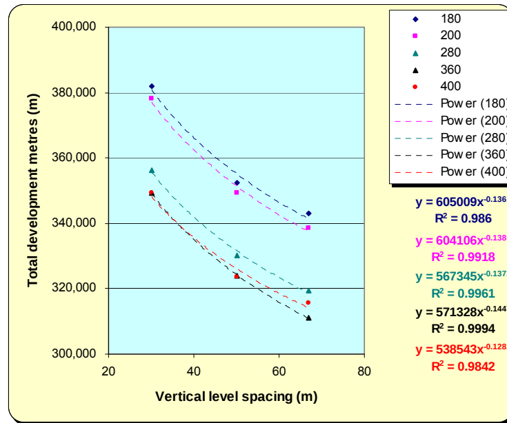
Figure 6.3: Variation of total development metres with level spacing
