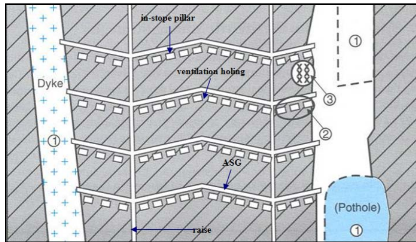
Figure 1.22: Longitudinal plan of a typical conventional breast layout (Adapted from Jager and Ryder, 1999)
