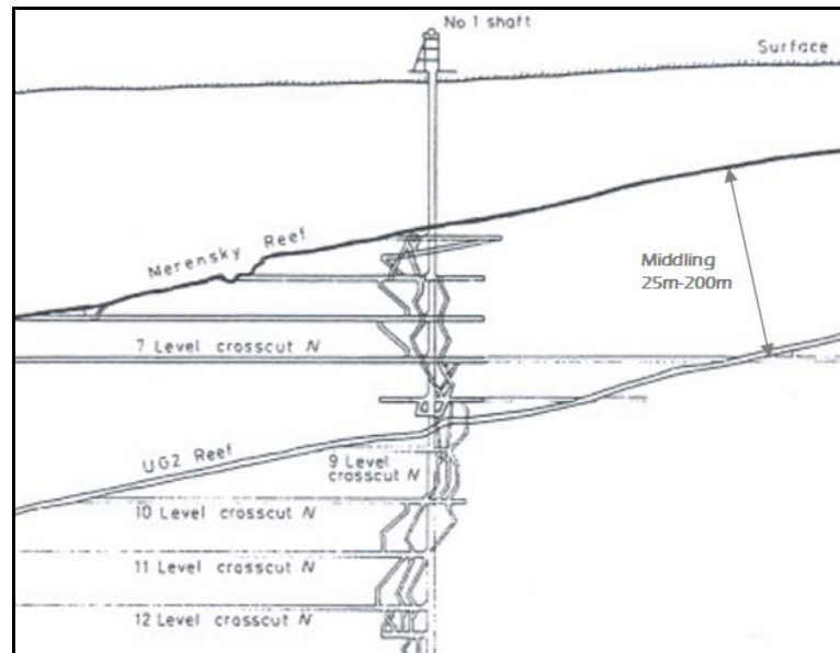
Figure 1.9: Typical section across a Bushveld Complex mine showing the Merensky overlying the UG2 reef (Adapted from Buchanan, 1987)
