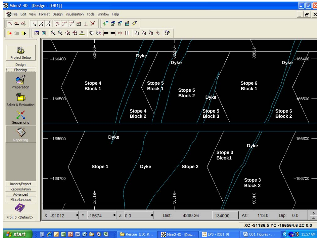
Figure 6.5: A Mine2-4D® illustration of OB1 stopes divided into blocks by dykes
