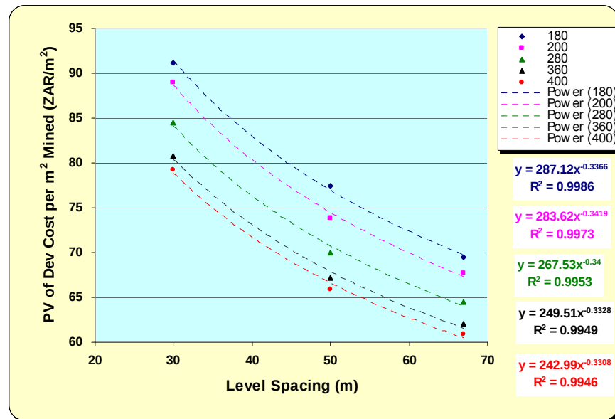
Figure 6.7: Variation of PV of development cost per centare mined in relation to level spacing
