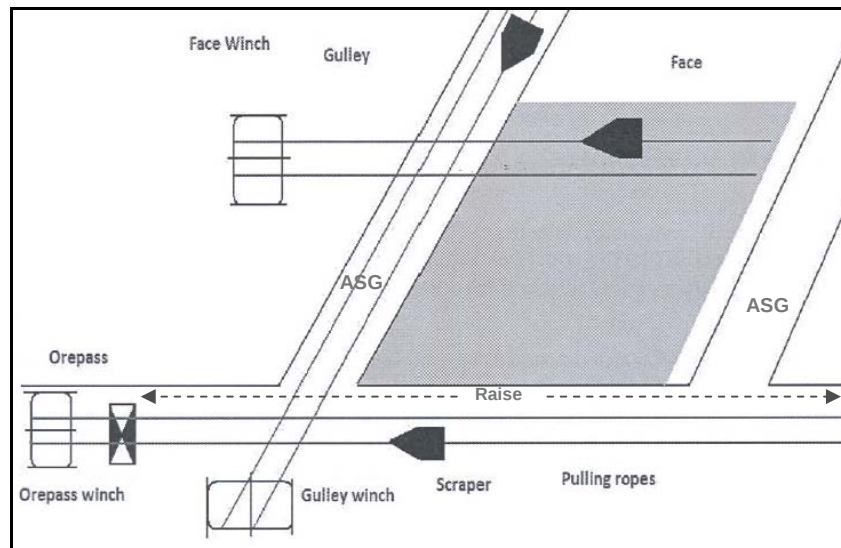
Figure 1.17: Typical scraper winch arrangement in a conventional mining stope panel layout (Courtesy of Anglo Platinum MTS)
