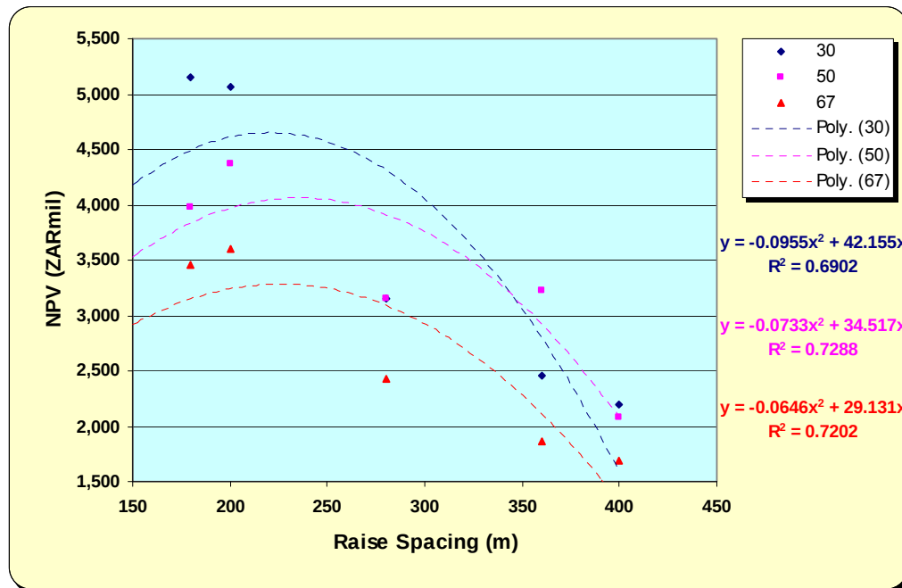
Figure 6.10: Variation of project NPV with increasing raise spacing
