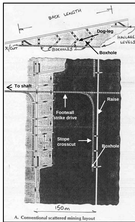
Figure 1.20: A typical crosscut access conventional mining layout (Fleming, 2002)
