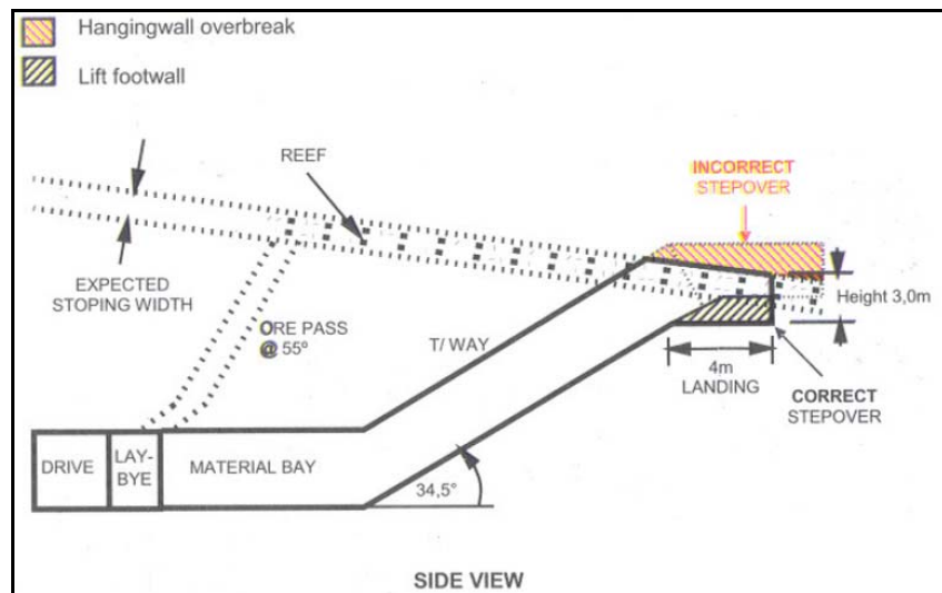
Figure 1.24: Side view across a laybye access raise connection (Impala Platinum, 2007a)
