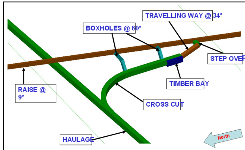
Figure 1.21: A 3-D perspective of a crosscut access layout at a raise connection in Mine 2-4D®
