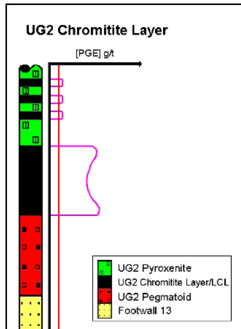
Figure 5.13: Typical PGE value distribution over reef thickness in UG2 reef (Impala Platinum Mining Projects, 2003)
