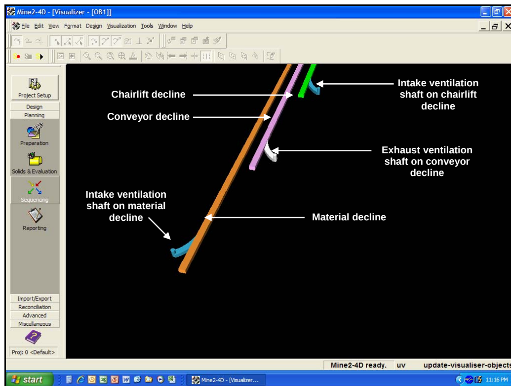
Figure 5.7: Mine2-4D illustration of intake and exhaust shaft splits on declines near surface
