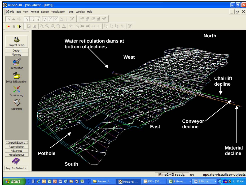
Figure 5.2: Relative positions of the three-cluster decline system for OB1 in Mine2-4D®
