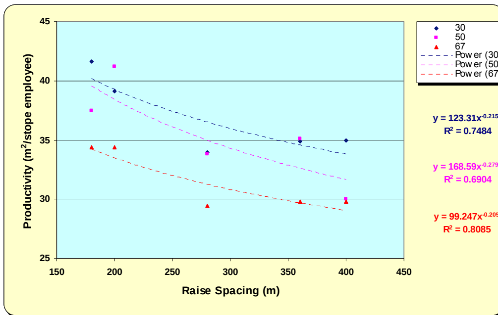
Figure 6.17: Variation of productivity with increasing raise spacing
