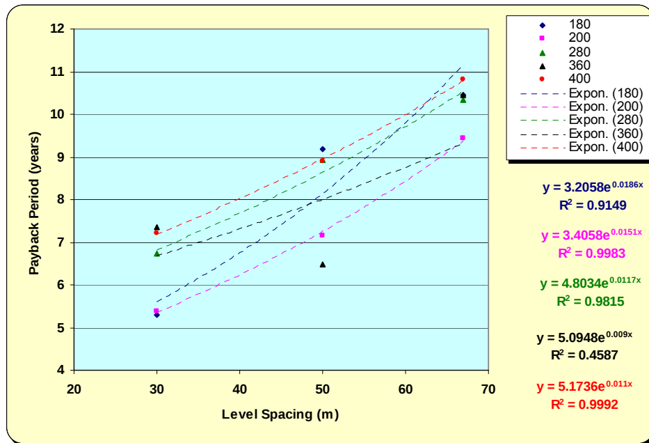
Figure 6.11: Variation of payback period with level spacing
