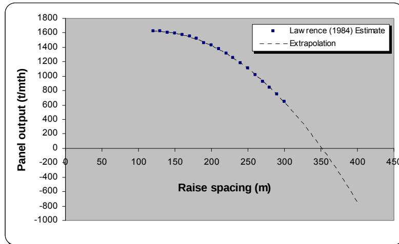
Figure 2.7: Extrapolation of the Lawrence (1984) model at longer raiseline spacing
