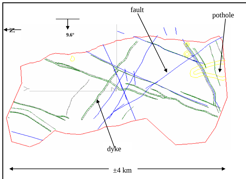
Figure 4.1: A Mine 2-4D® representation of OB1 structural geology
