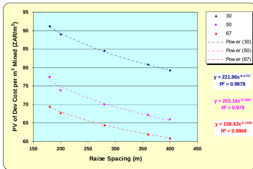
Figure 6.8: Variation of PV of development cost per centare mined in relation to raise spacing
