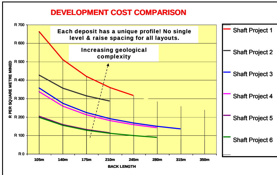
Figure 2.10: Half-Level Model output for different shafts (Adapted from Anglo Platinum MTS, 2005)
