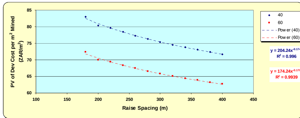
Figure 6.28: Cross-interpolation of PV values to estimate PV values for layouts that were not designed
