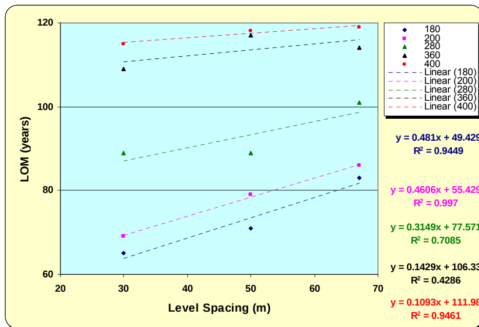
Figure 6.24: Variation of LOM with increasing level spacing
