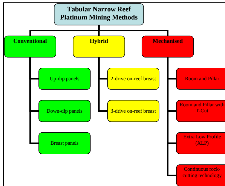
Figure 1.13: Topology of South African platinum underground mining methods
