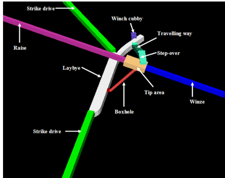
Figure 1.25: A 3-D perspective of a laybye access raise connection in Mine2-4D®
