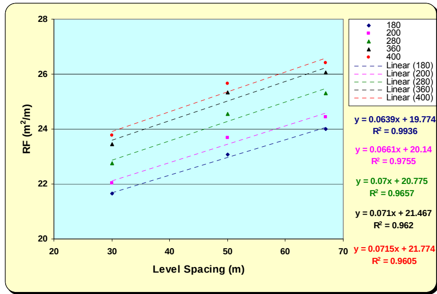
Figure 6.13: Variation of RF with level spacing
