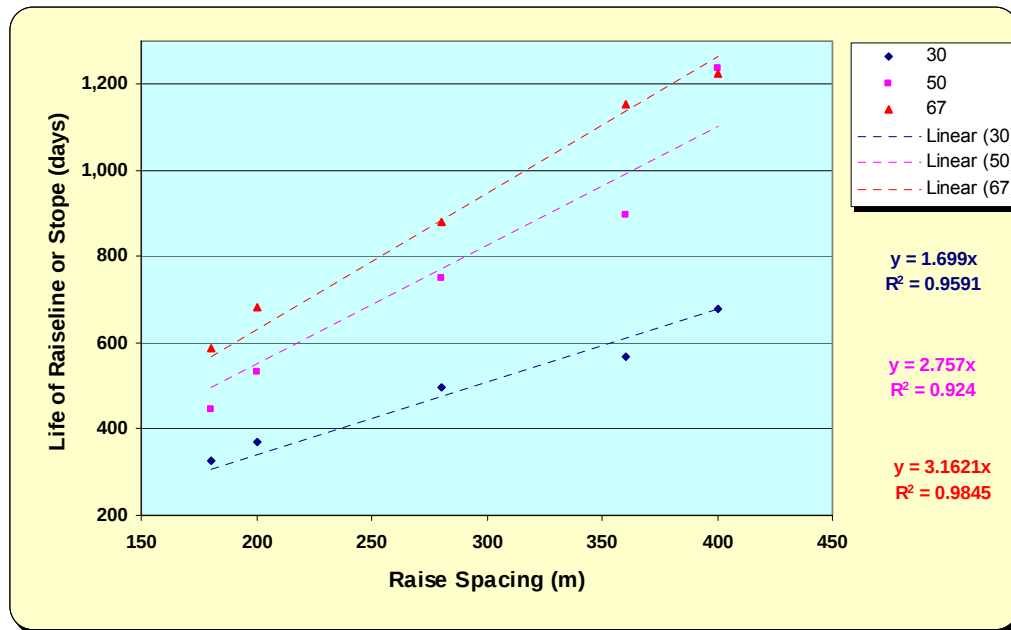
Figure 6.23: Variation of life of raiseline with increasing raise spacing
