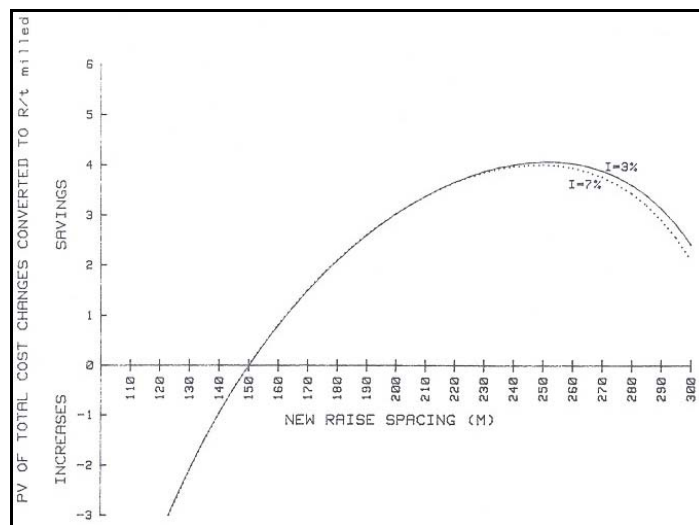
Figure 2.8: Variation of PV of cost savings with increasing raise spacing (Lawrence, 1984)
