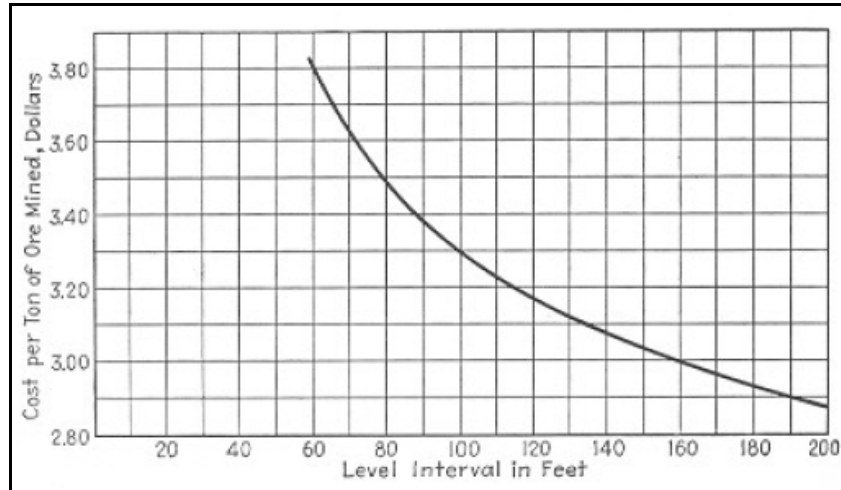
Figure 2.1: Variation of cost per tonne ore mined with increasing level interval or spacing (Lewis, 1941)
