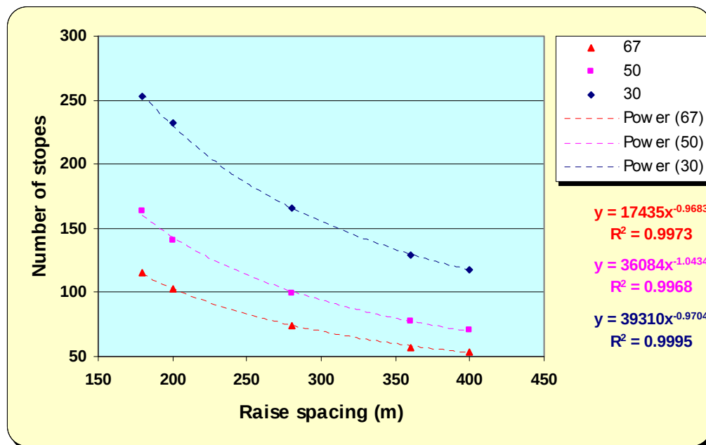
Figure 6.6: Variation of number of stopes with increasing raise spacing
