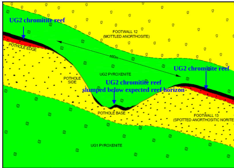
Figure 1.12: Section across a typical UG2 pothole (Adapted from Impala Platinum Mining Projects, 2003)
