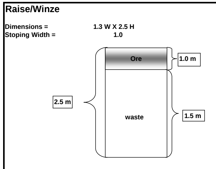
Figure 5.12: Cross-sectional area of a raise or winze showing the ore and waste portions
