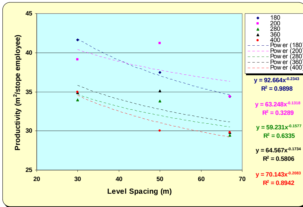
Figure 6.16: Variation of productivity with increasing level spacing
