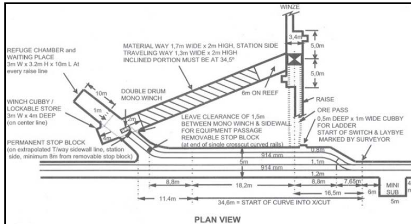
Figure 1.23: Plan view of a laybye access layout at a raise connection (Impala Platinum, 2007a)
