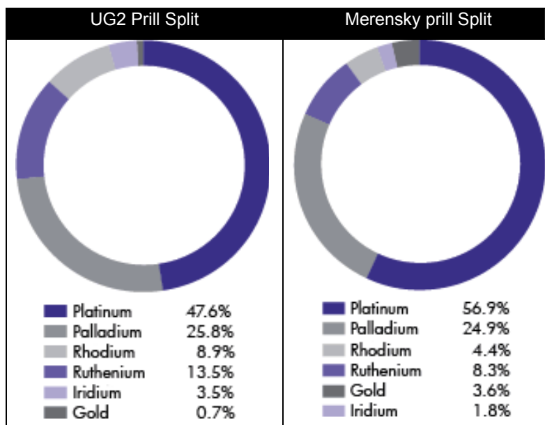
Figure 4.5: Typical average 4E prill splits for UG2 and Merensky reefs (Source: Impala Platinum, 2008; Impala Platinum, 2009)
