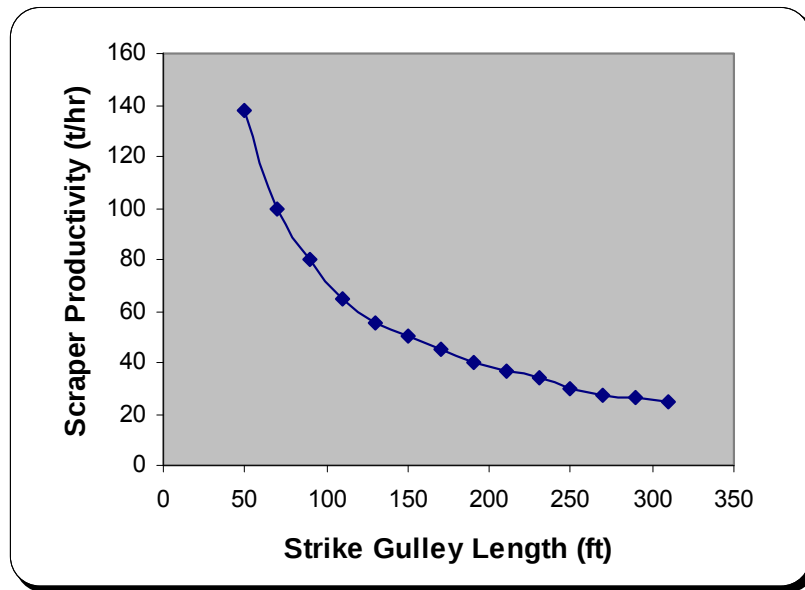
Figure 2.2: Variation of scraper winch productivity with increasing strike gulley length on a panel (Adapted from Brassell, 1964)
