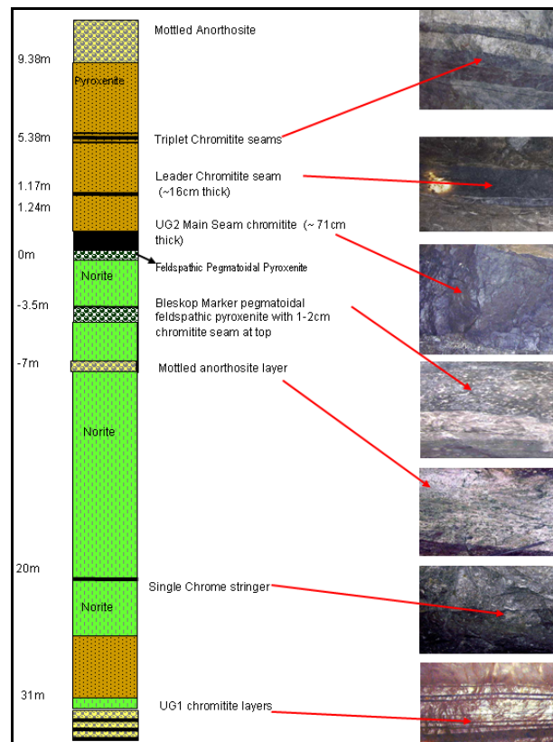
Figure 1.11: Typical UG2 stratigraphy showing the actual rock type appearance (Source: Anglo Platinum, Boschfontein Shaft, Geology Department, 2004)
