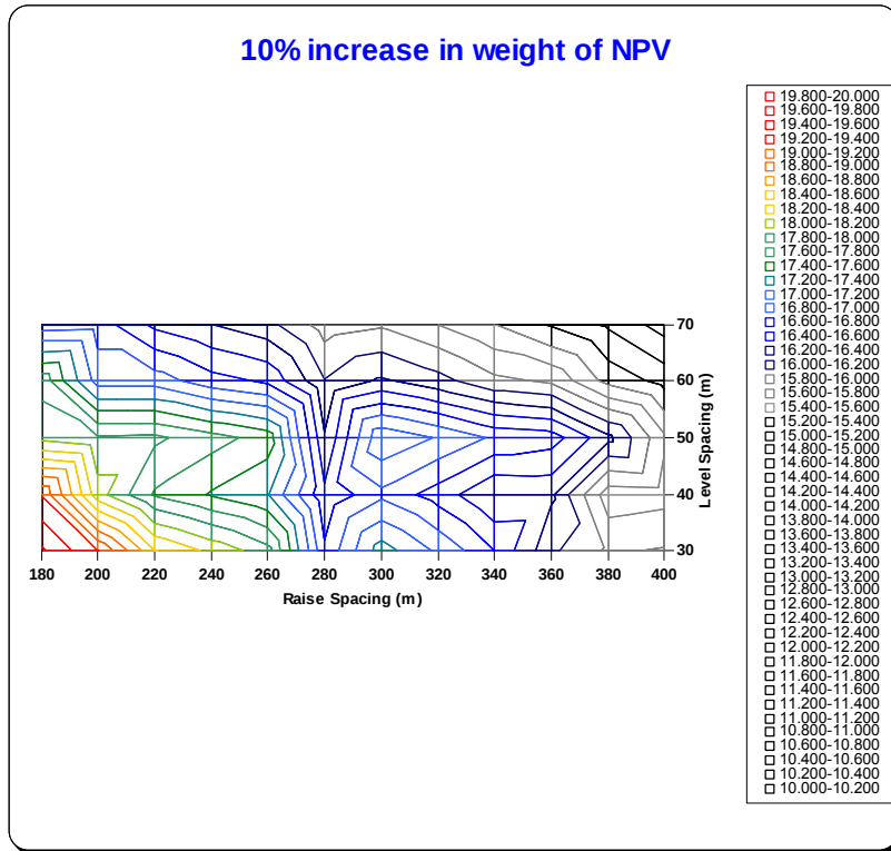
Figure 7.3: A 3-D Excel surface plot of the AHP priority score when importance of NPV increases by 10%
