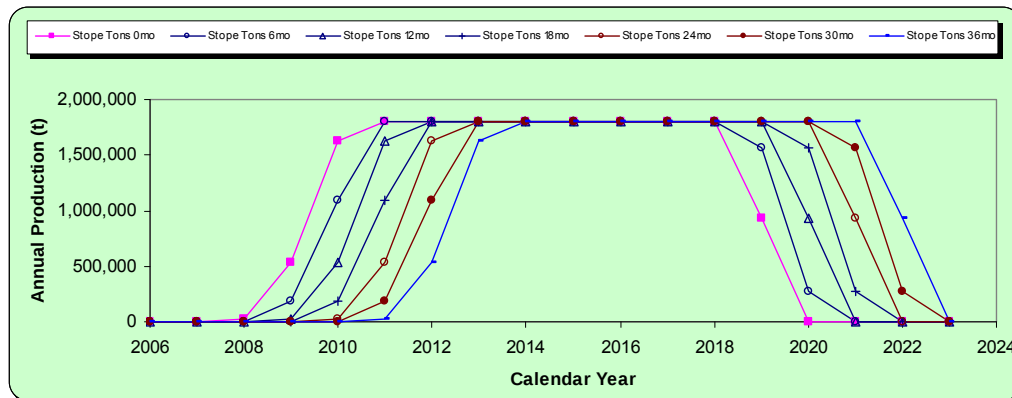
Figure 3.2: OB1 production profiles at variable ore availability
