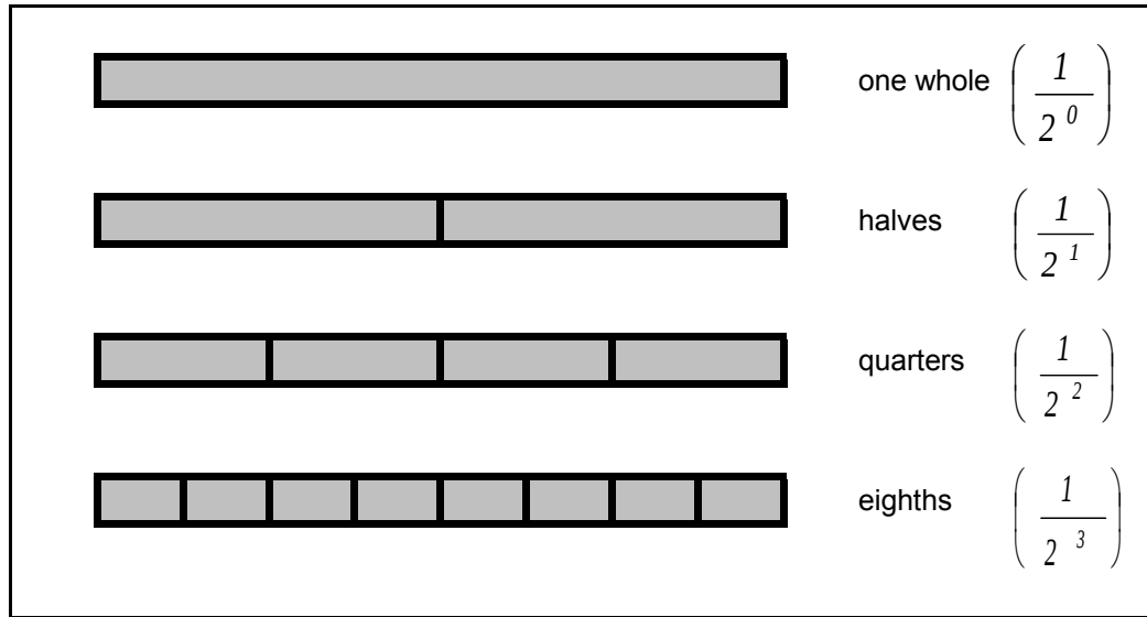
Figure 2.11: Analogy of line and strike distance being repeatedly into equal parts
