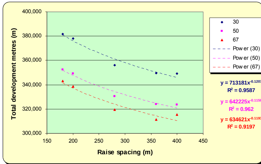
Figure 6.2: Variation of total development metres with raise spacing
