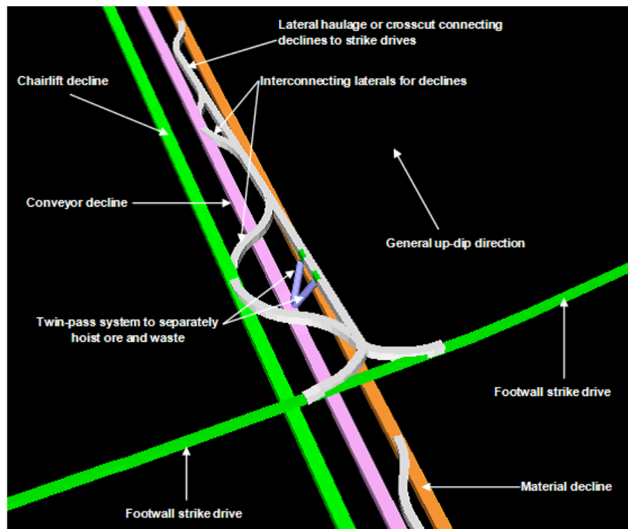
Figure 5.9: 3-D illustration of off-reef development breaking away from declines
