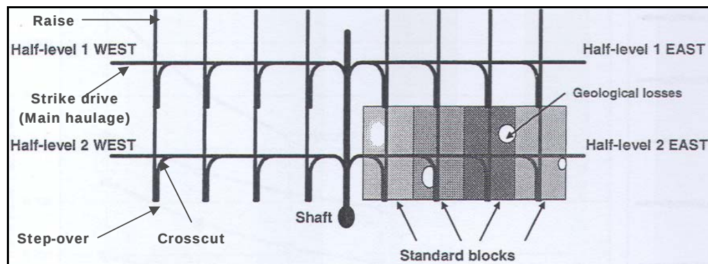
Figure 1.16: A schematic illustration of crosscut access conventional mining in plan view (Adapted from Smith and Vermeulen, 2006)
