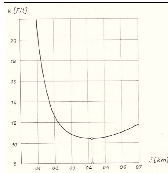
Figure 2.5: Variation of specific cost function, K , with crosscut panel length, S (Zambó, 1968)
