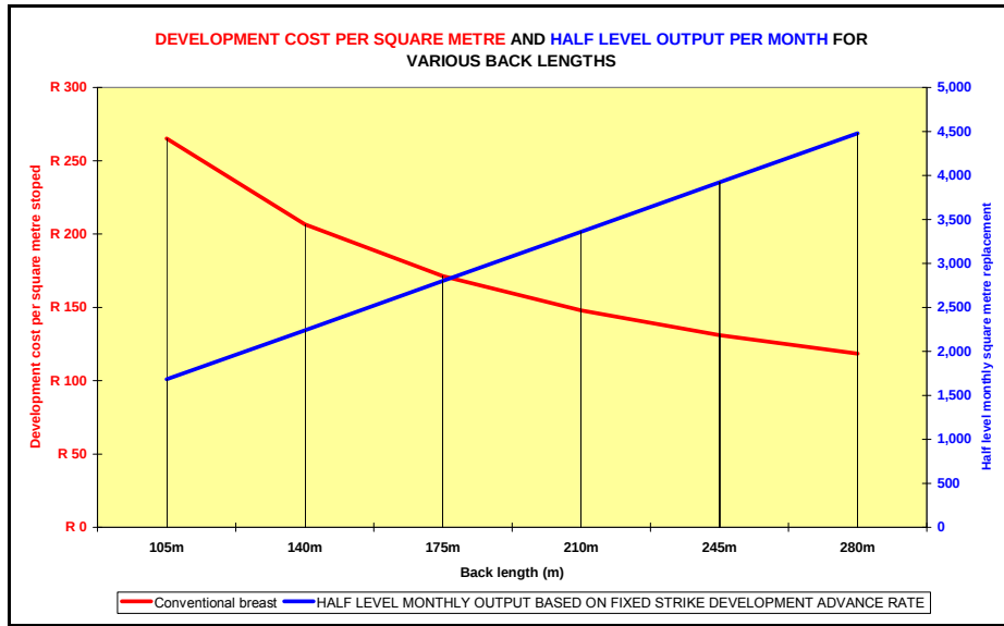
Figure 2.9: Typical Half-Level Model Output (Anglo Platinum MTS, 2005)
