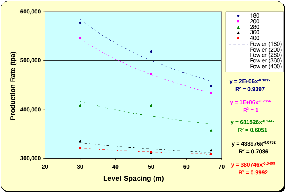
Figure 6.18: Variation of production rate with increasing level spacing
