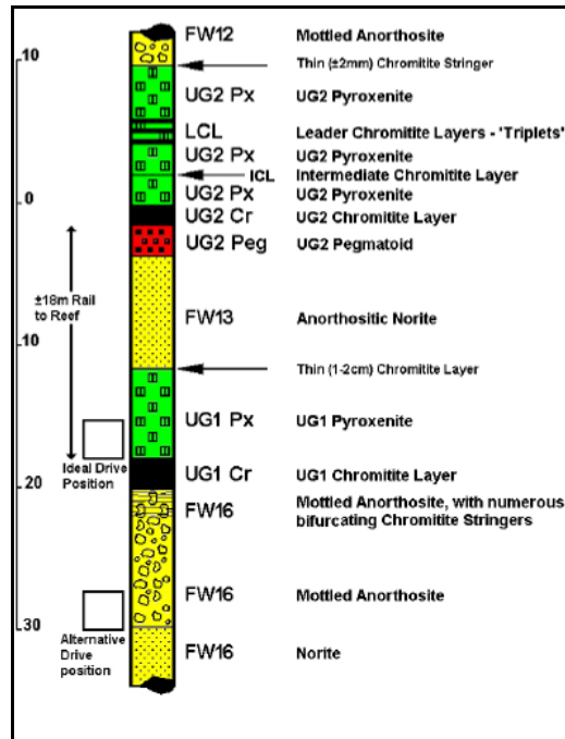
Figure 1.10: General UG2 stratigraphy showing optimal location of footwall development (Source: Impala Platinum Mining Projects, 2003)
