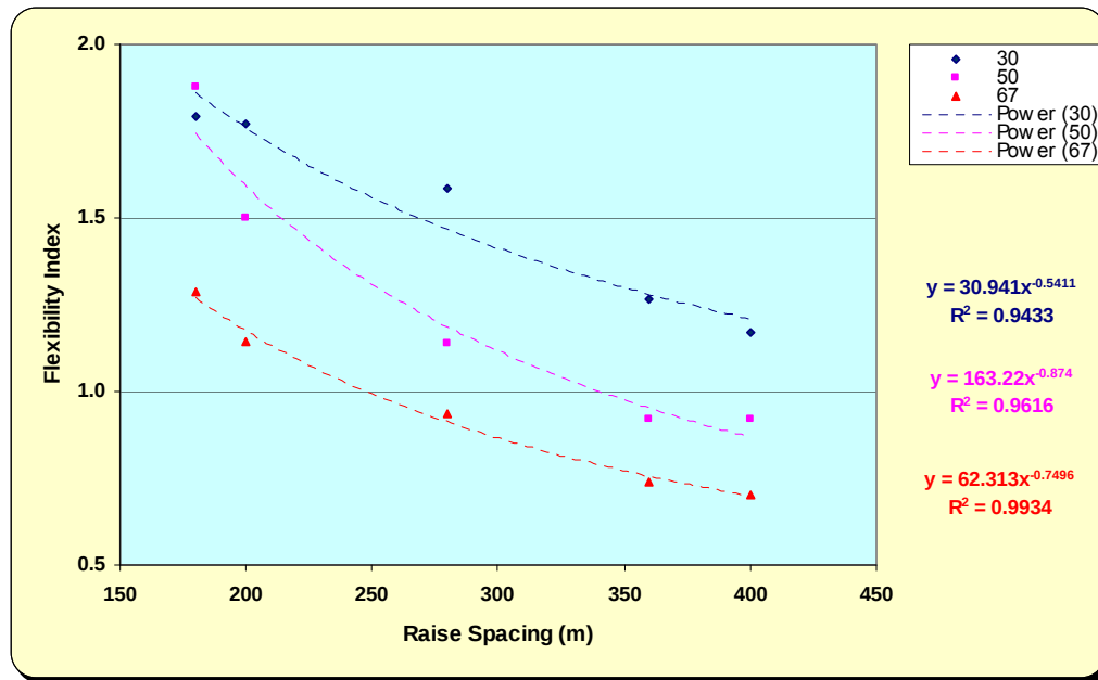
Figure 6.21: Variation of flexibility index with raise spacing
