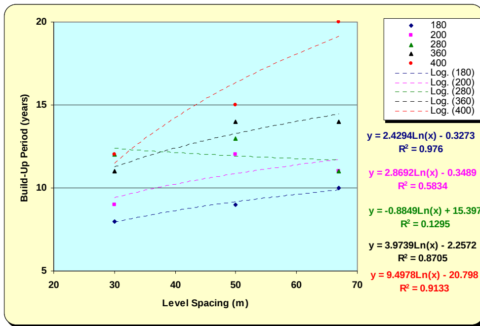
Figure 6.26: Variation of build-up period with level spacing
