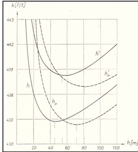
Figure 2.4: Variation of the specific cost function, K , with level interval, h (Zambó, 1968)
