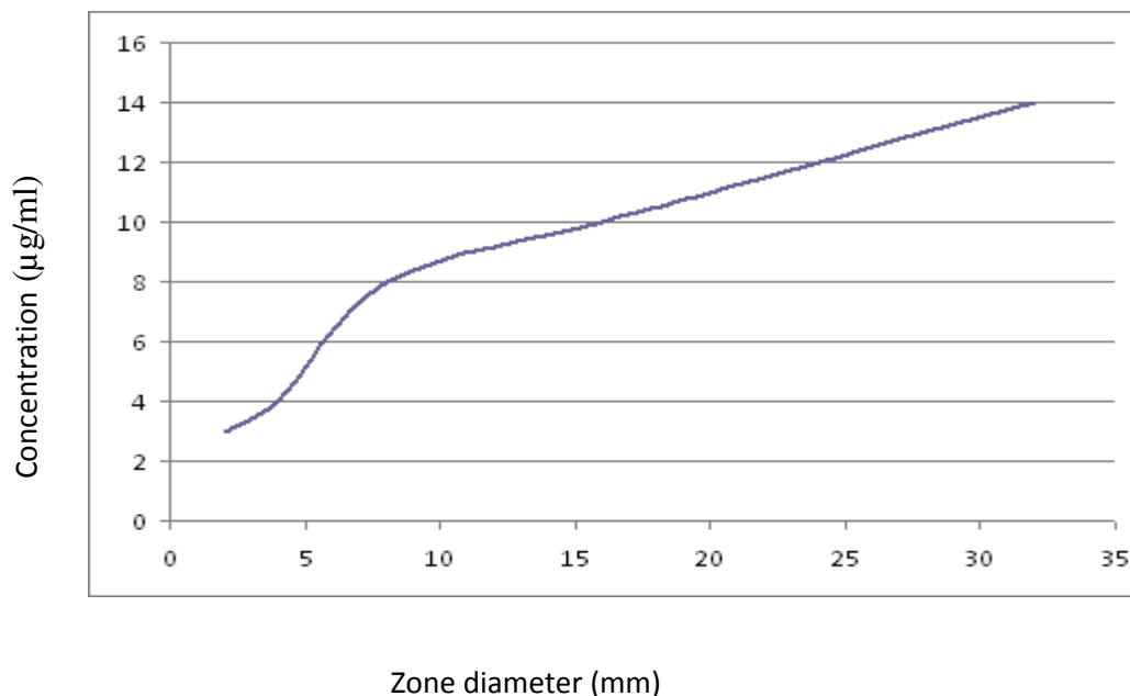
Fig. 20: Calibration curve for chloramphenicol concentration
