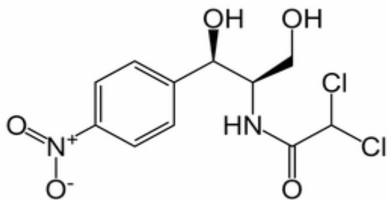
Fig. 2: Structure of chloramphenicol
