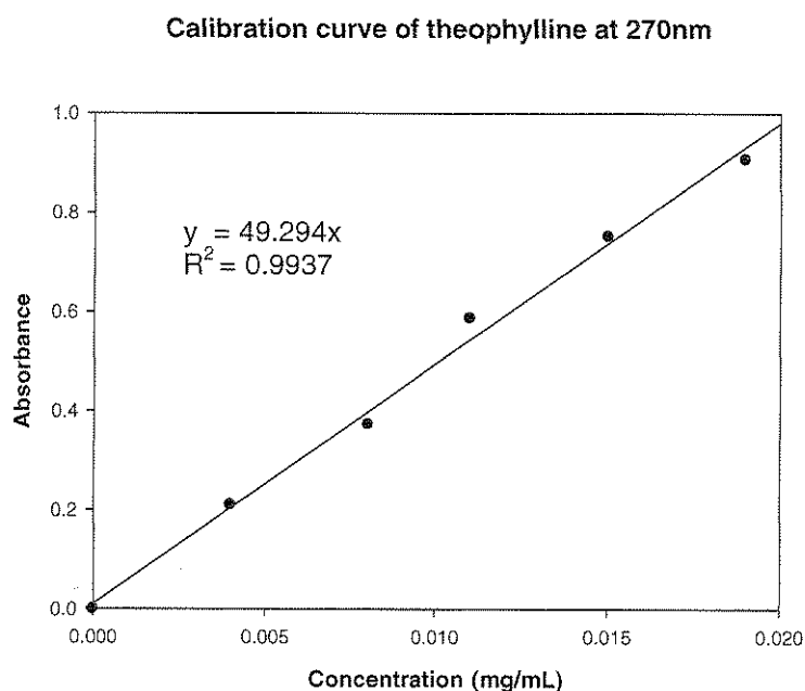
Figure 2.2. Calibration curve of theophylline in phosphate buffer of pH 6.8 (simulated intestinal fluid) ( N = 3 ; in all cases SD < 0.02 ).
