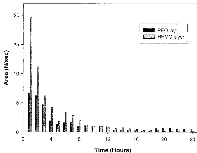
Figure 2.15. Gel strength transitions measured on both axial planes of the tablet configuration (PEO layer and HPMC layer), (N=3; in all cases SD<0.5).
