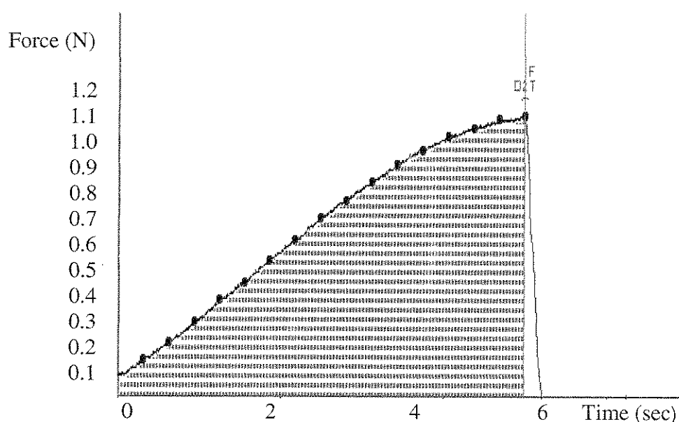
Figure 2.4. Typical textural profile for the determination of gel strength transitions (N=3).
