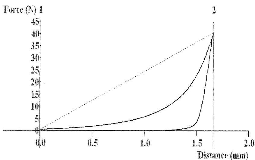
Figure 2.3. Typical textural profile for the determination of matrix hardness (N=3).
