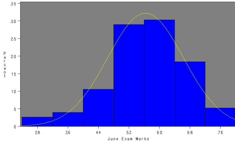
Fig 5.3 Assumption of Normality for Fisher's Z transformation
