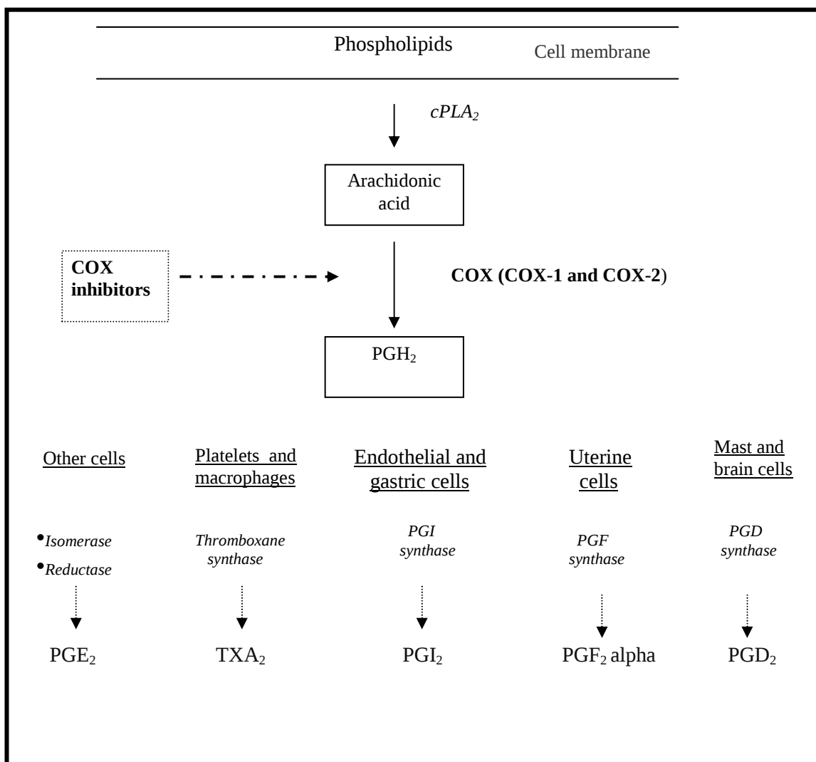
Figure 3. The arachidonic acid cascade showing the cyclooxygenase (COX) pathway, the biosynthesis of the cyclic endoperoxide, \text{PGH}_2 , and the final prostanoids: \text{PGE}_2 , \text{PGF}_2 \text{ alpha} , \text{PGD}_2 , \text{PGI}_2 and \text{TXA}_2 . The cell-specific enzymes (synthases) which result in the formation of the prostanoids in their specific cells are shown in italics. Diagram adapted from Funk (2001).
