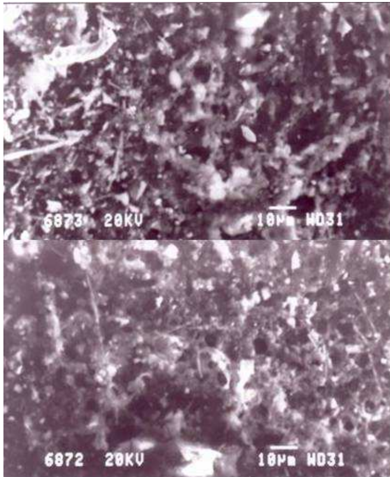
Figure 17: Typical SEM micrograph of galena-rich phase morphologies after microbial attack showing much precipitate cover with no distinct microbial induced pitting. [Magnification = 850]
