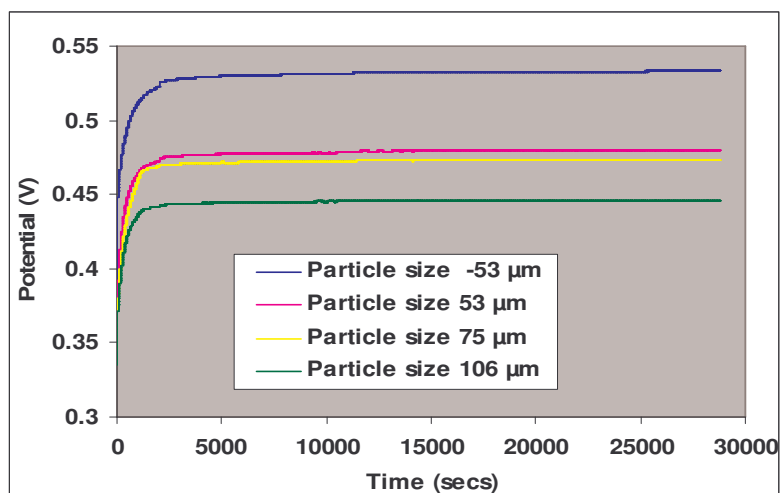
Figure 12: Open-circuit potentials of the four particle size fractions exposed to microbial attack for 18 days
