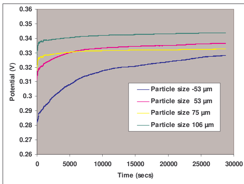
Figure 10: Open-circuit potentials of the four particle size fractions exposed to microbial attack for 6 days
