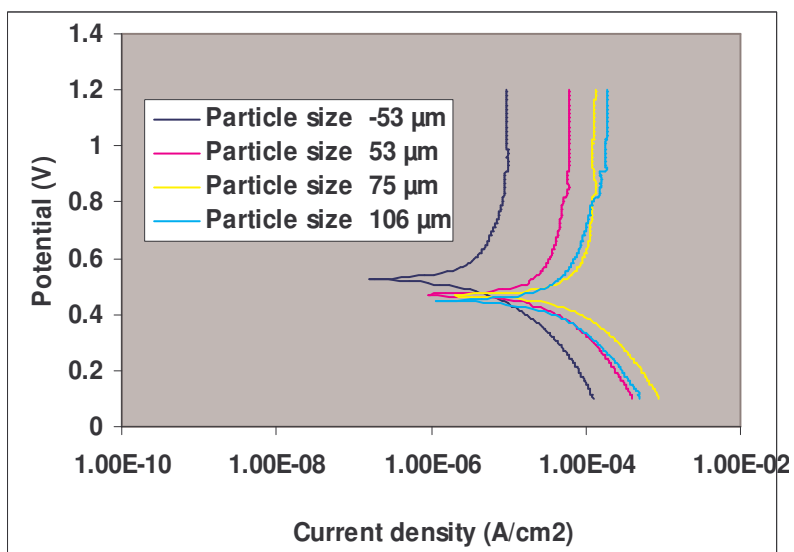
Figure 9: Polarization curves of the four particle size fractions exposed to microbial attack for 18 days
