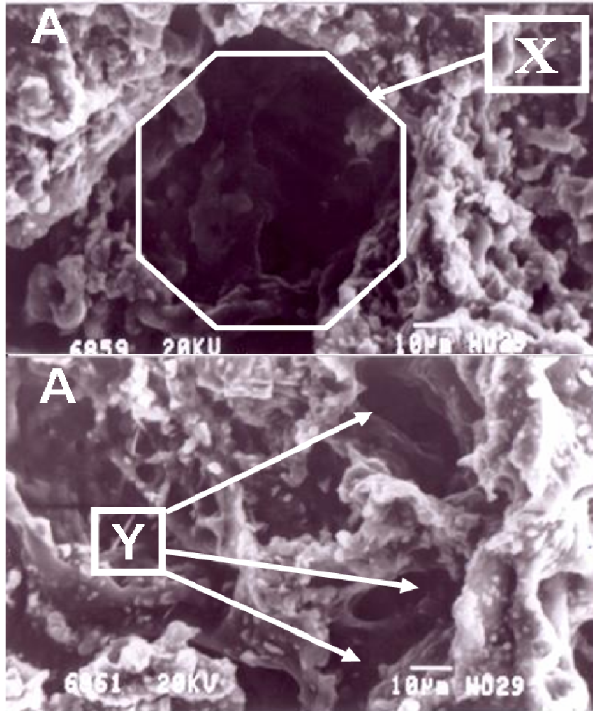
Figure 16: Typical SEM micrograph of sphalerite-rich phase morphologies after microbial attack deep hollow dissolution pit (X) and dissolution channels of elongated elliptical pits (Y). [Magnification = 850]
