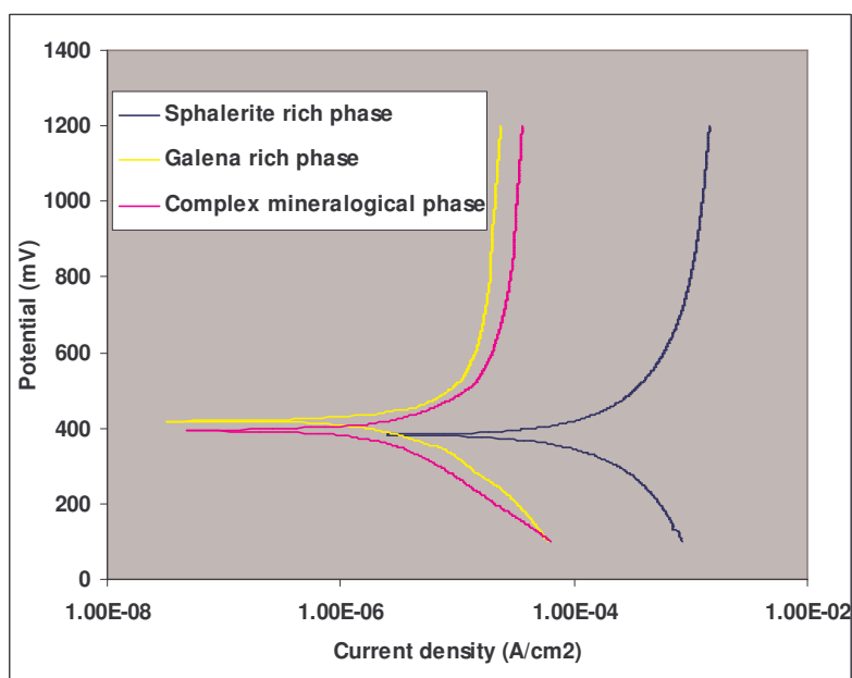
Figure 15: Polarization curves of the three different mineral-rich phases exposed to microbial attack for 18 days
