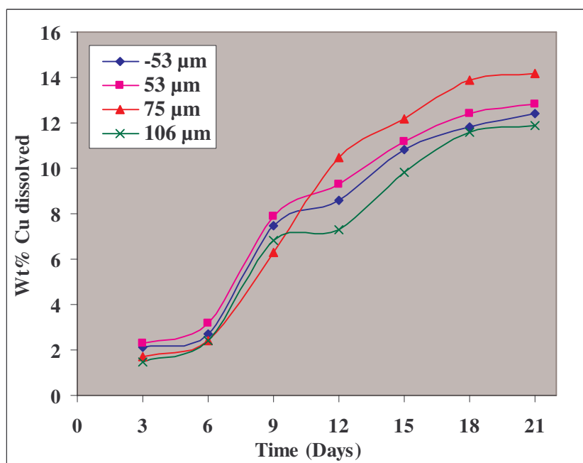
Figure 3: Effects of particle size on copper dissolution. [Stirring speed of 150 rpm, pH of 2.0, 10% wt/vol pulp density, and 6% vol/vol volume of inoculum addition]
