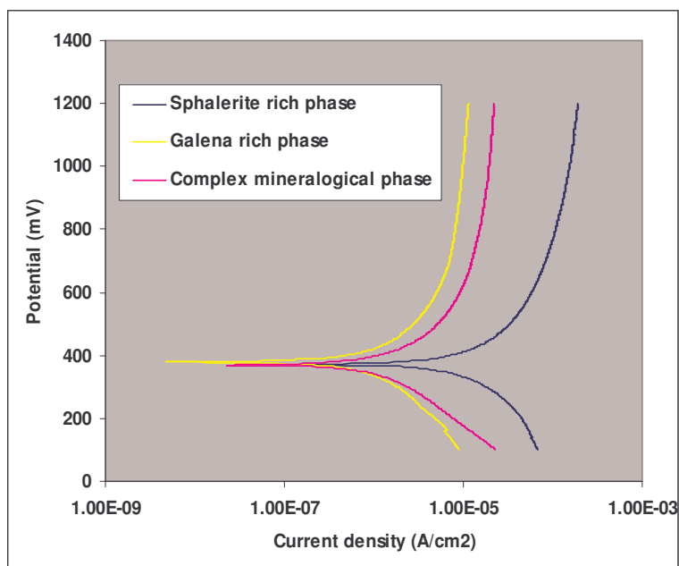
Figure 14: Polarization curves of the three different mineral-rich phases exposed to microbial attack for 12 days
