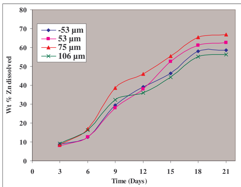
Figure 2: Effects of particle size on zinc dissolution. [Stirring speed of 150 rpm, pH of 2.0, 10% wt/vol pulp density, and 6% vol/vol volume of inoculum addition]
