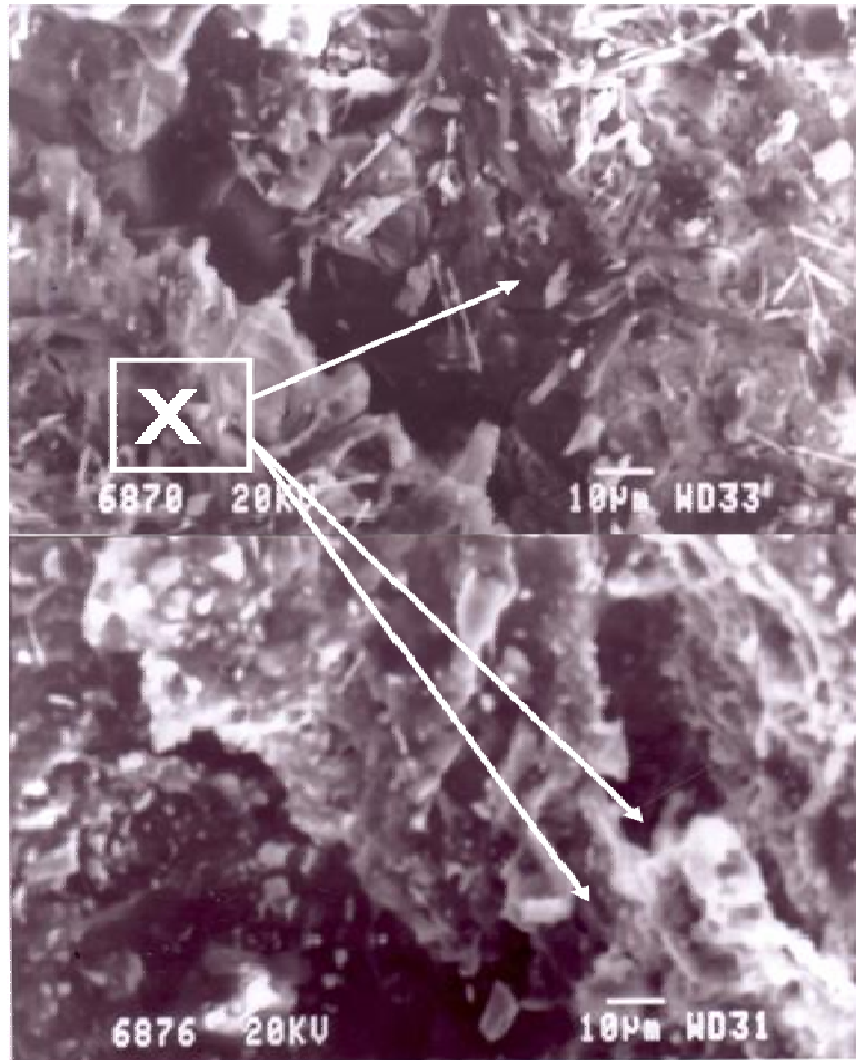
Figure 18: Typical SEM micrograph of the complex mineralogical phase morphologies after microbial attack showing no regular microbial attack and dissolution pits (X). [Magnification = 850]
