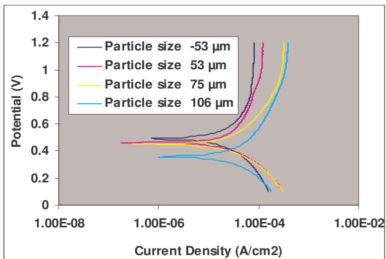
Figure 8: Polarization curves of the four particle size fractions exposed to microbial attack for 12 days
