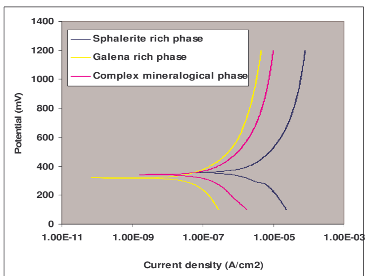
Figure 13: Polarization curves of the three different mineral-rich phases exposed to microbial attack for 6 days
