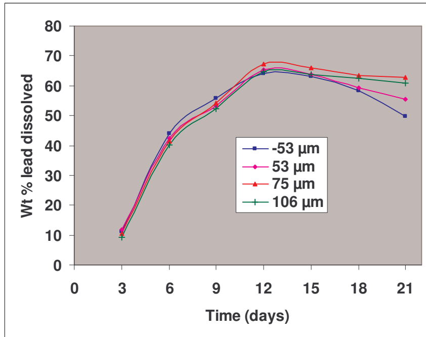
Figure 4: Effects of particle size on lead dissolution. [Stirring speed of 150 rpm, pH of 2.0, 10% wt/vol pulp density, and 6% vol/vol volume of inoculum addition]
