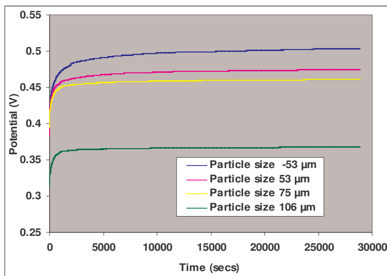
Figure 11: Open-circuit potentials of the four particle size fractions exposed to microbial attack for 12 days
