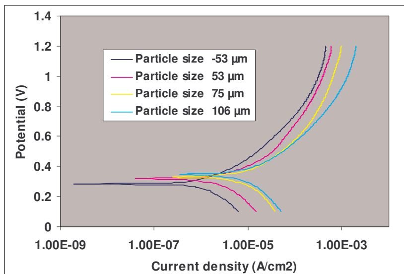
Figure 7: Polarization curves of the four particle size fractions exposed to microbial attack for 6 days
