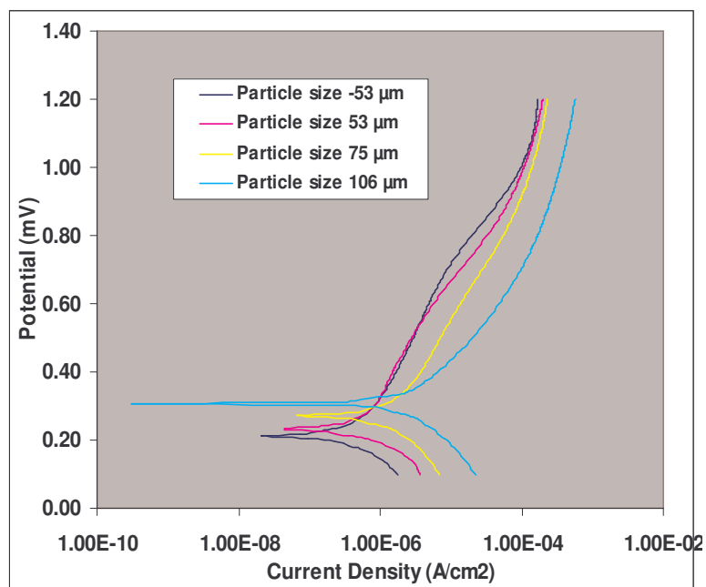
Figure 6: Polarization curves of fresh electrodes from the four particle size fractions before bioleaching
