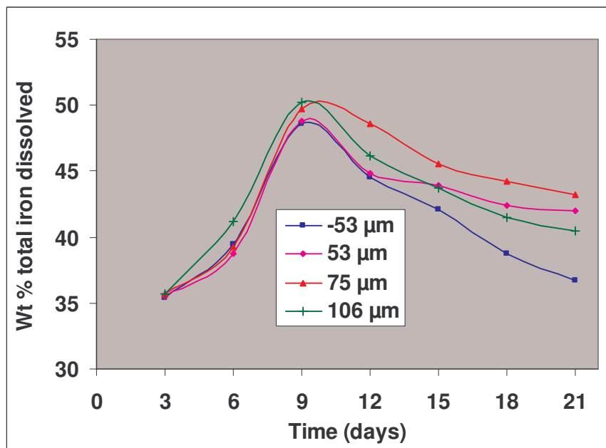
Figure 5: Effects of particle size on iron dissolution. [Stirring speed of 150 rpm, pH of 2.0, 10% wt/vol pulp density, and 6% vol/vol volume of inoculum addition]
