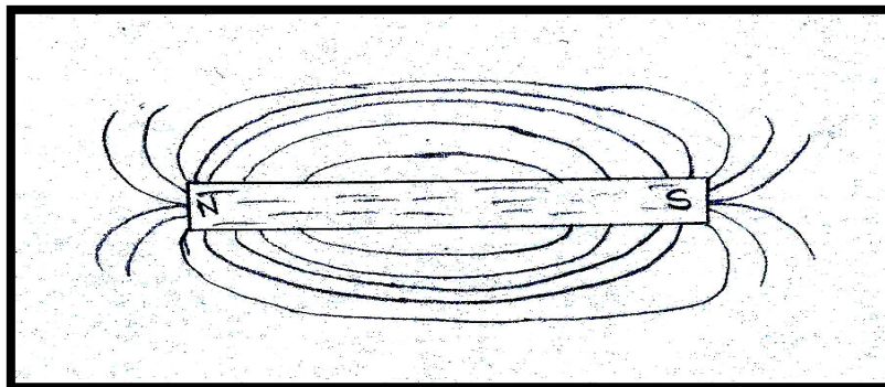
Diagram 8.1: Magnetic field lines around a magnet
