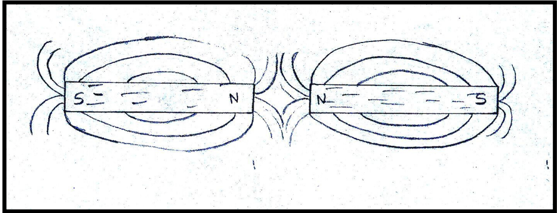
Diagram 8.3: Magnetic field lines between like poles-A2
