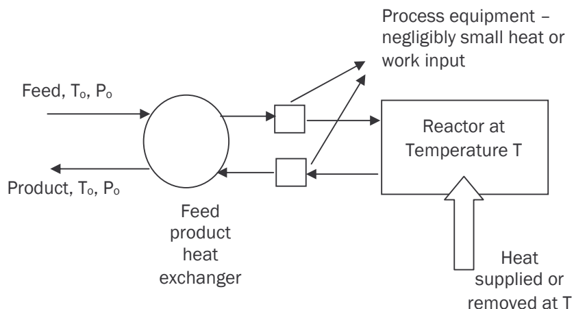
Figure 5.2: Schematic representation of a simple chemical process
