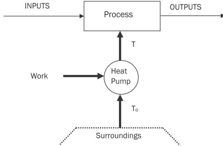
Figure 5.4: Representing the process as a heat pump
