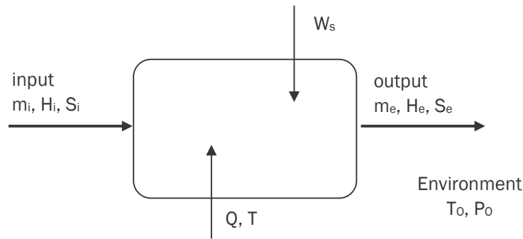
Figure 3.3: General flow process at steady state
