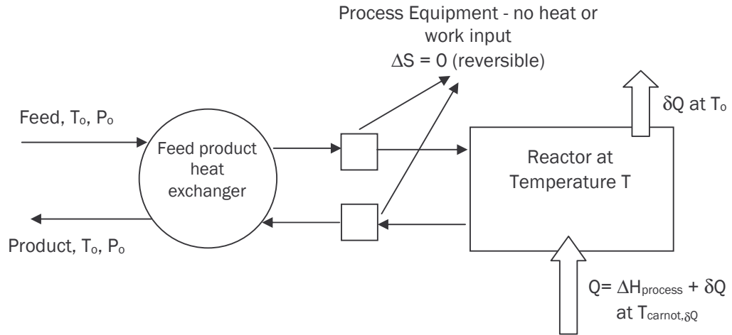
Figure 5.6: Schematic representation of a process where additional heat \delta Q is added
