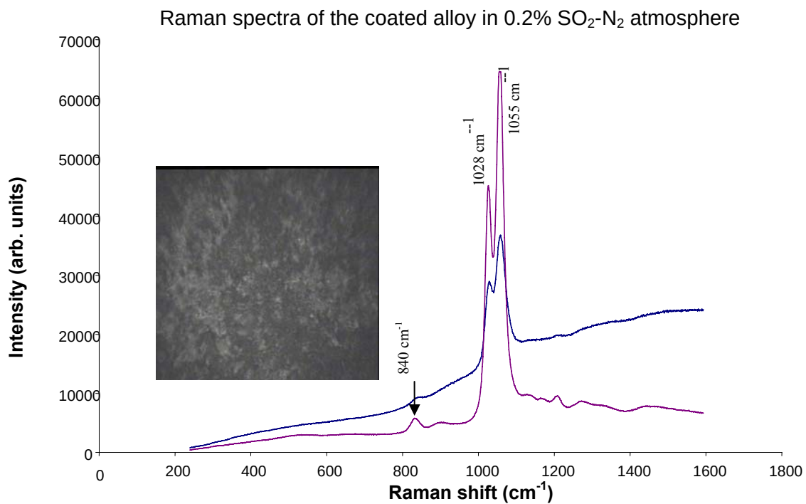
Figure 5.63 Raman spectra collected on the external surface of the coated alloy after sulphidation at 900°C for a period of 60 hours
