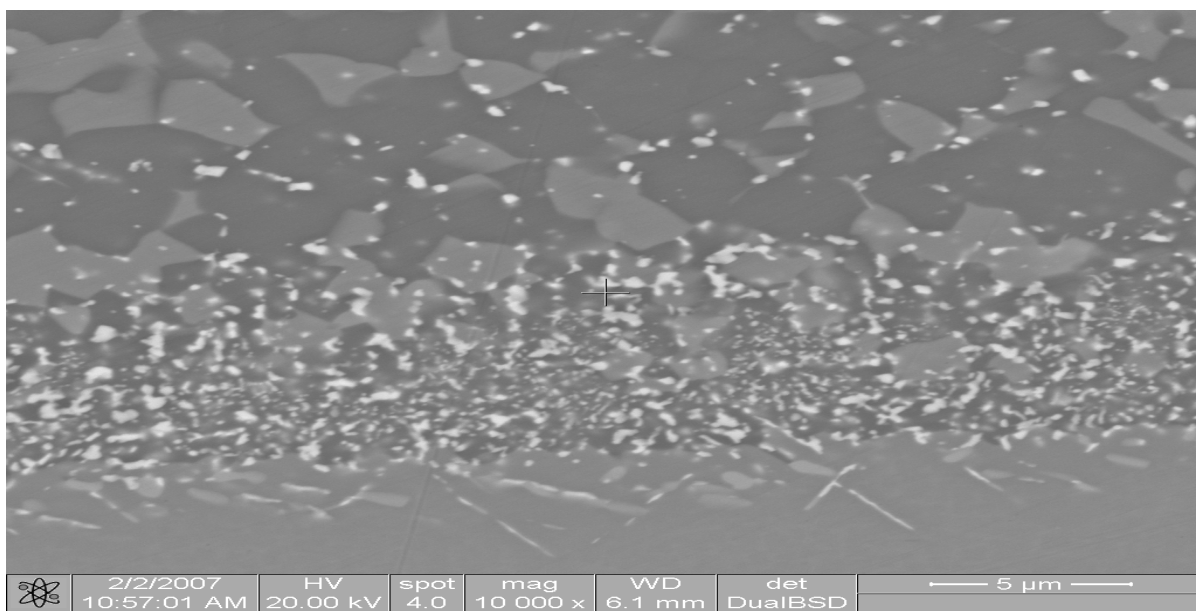
Figure 5.51 Inter-diffusion zone at high magnification of the coated Ni-based superalloy after 60 hours in a 0.2% SO 2 -N 2 atmosphere
