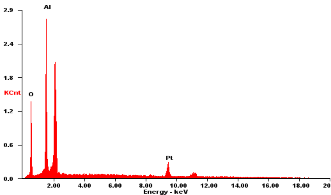
Figure 5.43 EDS analysis performed on the dark area in the corroded section on alloy RS3
