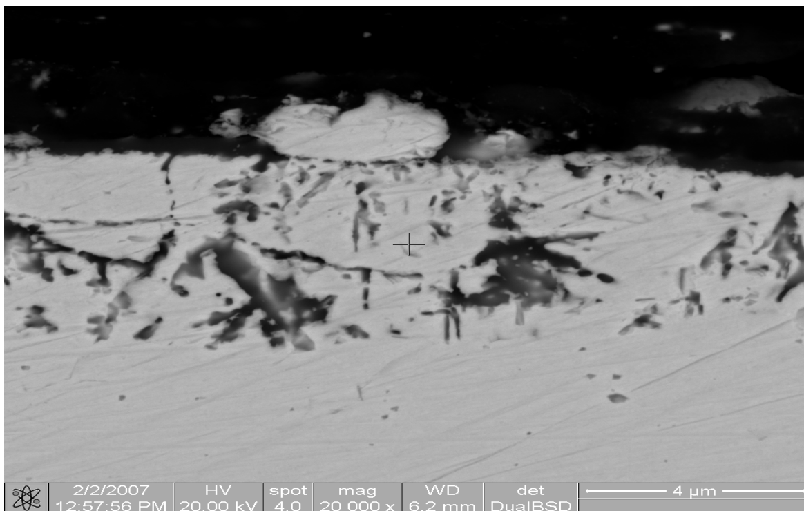
Figure 5.42 Secondary image of cross section of alloy RS3 after sulphidation test
