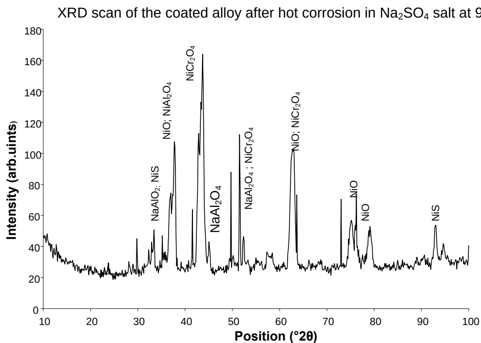
Figure 5.29 X-ray diffraction patterns on the surface of the coated Ni-based superalloys after hot corrosion
