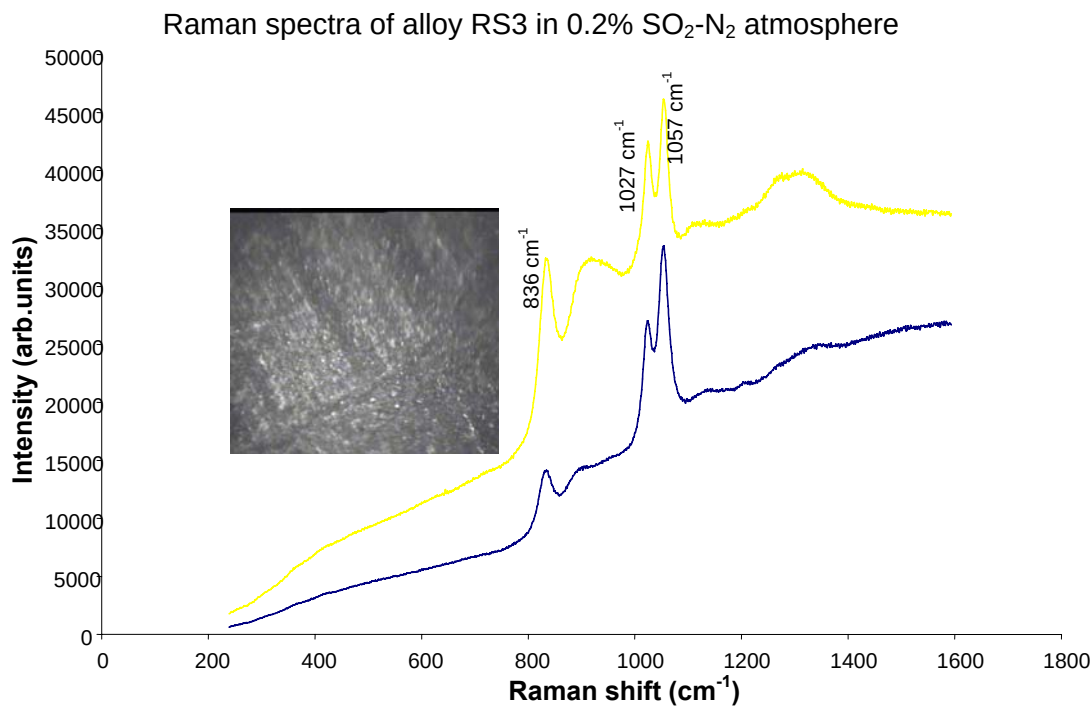
Figure 5.66 Raman spectra collected on the external surface of alloy RS3 after sulphidation at 900°C for a period of 60 hours
