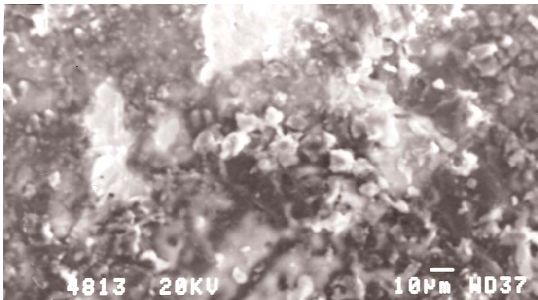
Figure 5.11 Secondary electron image of the corrosion morphology of alloy P420 after hot corrosion at 950°C for 792 hours
