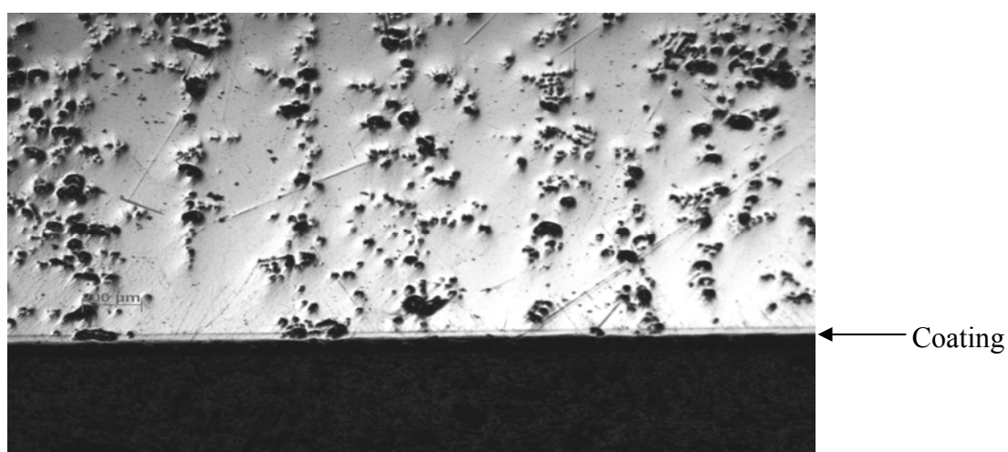
Figure 4.1 Cross section of a coated Ni-based superalloy in as polished condition showing a thin coating applied on the surface of the alloy
