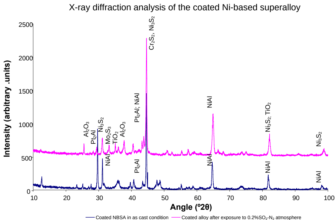
Figure 5.55 XRD spectrum performed on the coated Ni-based superalloy before and after corrosion in controlled atmosphere constituting of 0.2% \text{SO}_2\text{-N}_2 at 900^{\circ}\text{C} for a period of 60 hours
