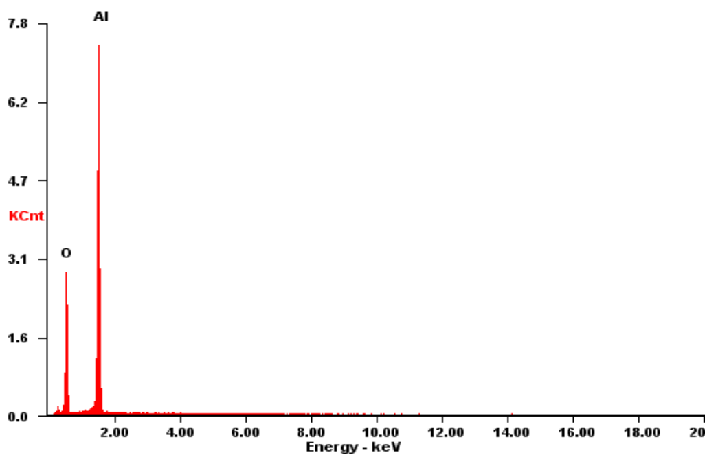
Figure 5.50 EDS analysis performed on the external scale of the coated alloy after sulphidation test
