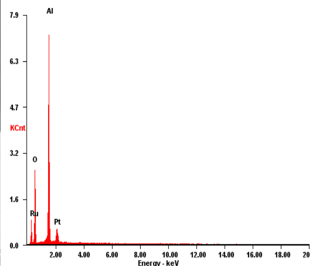
Figure 5.41 EDS analysis performed on the external scale of alloy RS2
