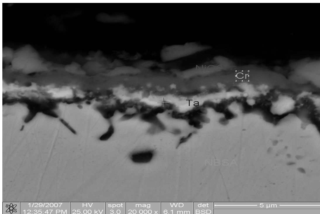
Figure 5.54 Secondary image of the cross section of the uncoated Ni-based superalloy after sulphidation test
