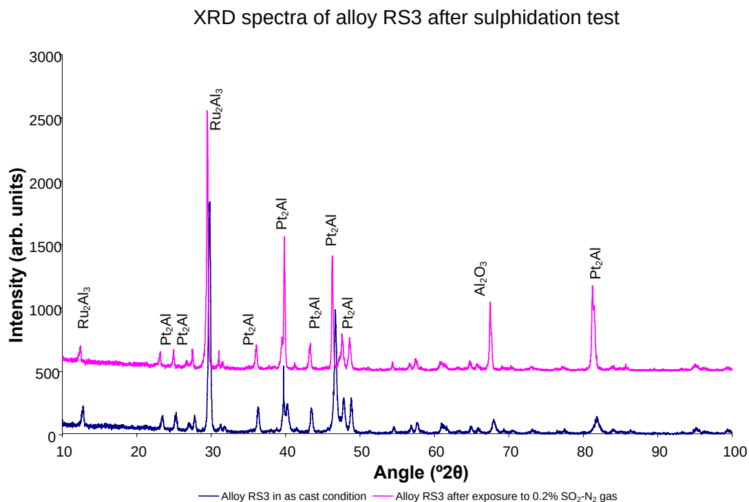
Figure 5.59 XRD spectrum performed on the external surface of alloy RS3 [Pt-Al-Cr-Ru] before and after exposure to a 0.2% \text{SO}_2\text{-N}_2 atmosphere at 900°C for a period of 60 hours
