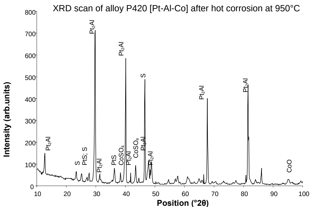
Figure 5.27 X-ray diffraction patterns on alloy P420 after corrosion at 950°C
