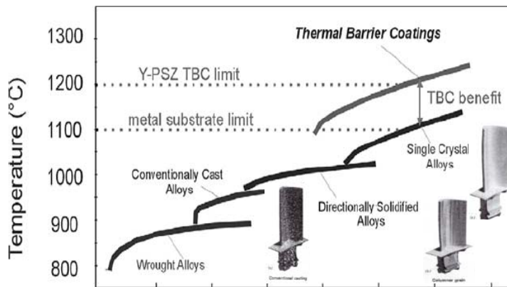
Figure 2.4 Processing techniques developed to increase working temperatures in gas turbines [Schultz et al. , 2003]
