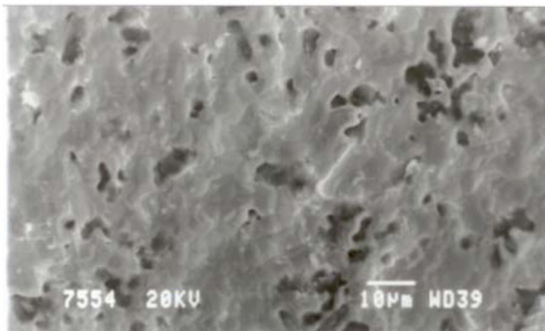
Figure 5.16 Secondary electron image of the corrosion morphology of alloy RS3 after hot corrosion in molten Na 2 SO 4 salt at 950°C for duration of 540 hours
