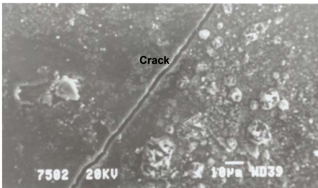
Figure 5.6 Secondary electron image of the corrosion morphology of the uncoated CMSX-4 after hot corrosion at 950°C with a crack running across the surface of the alloy
