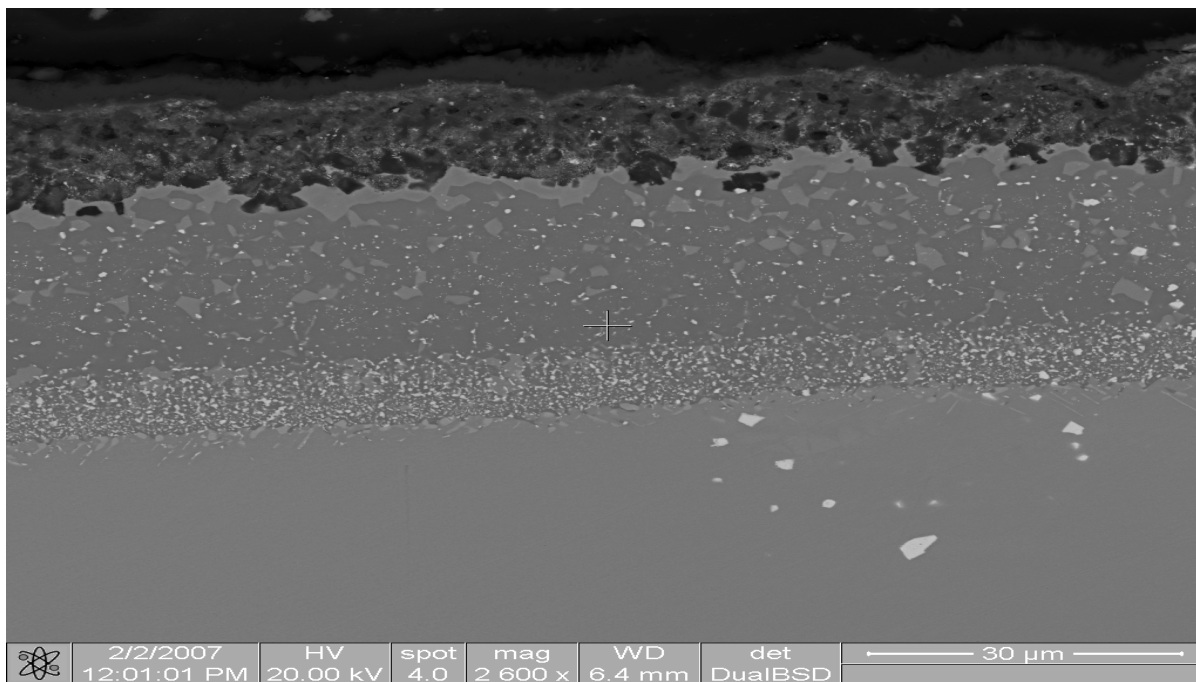
Figure 5.49 Cross section showing the different phases formed when the alloy was exposed to 0.2% \text{SO}_2\text{-N}_2 atmosphere
