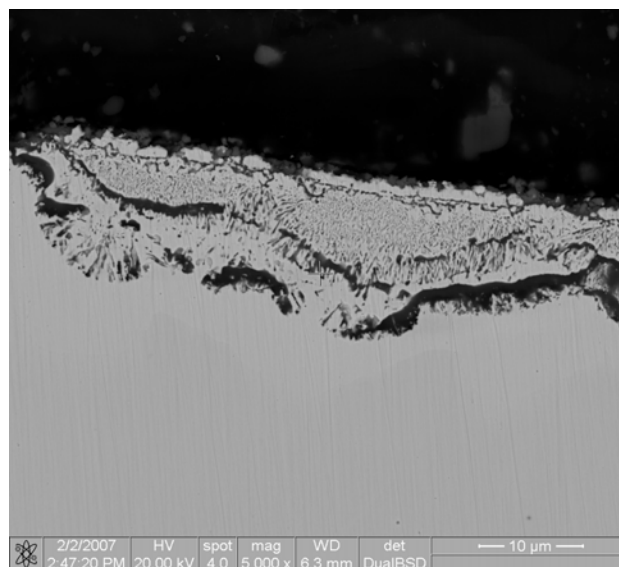
Figure 5.47 Transverse section of alloy P421 across the corroded area of alloy P421 after the sulphidation test
