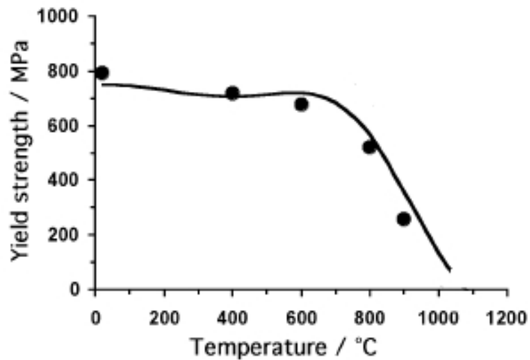
Figure 2.3 Yield strength versus temperature indicates capabilities of the \gamma' -phase with increasing temperature [Bhadesia, 2003]
