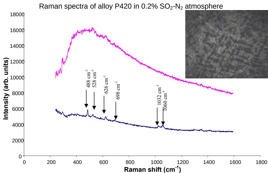
Figure 5.67 Raman spectra collected on the external surface of alloy P420 after sulphidation at 900°C for a period of 60 hours
