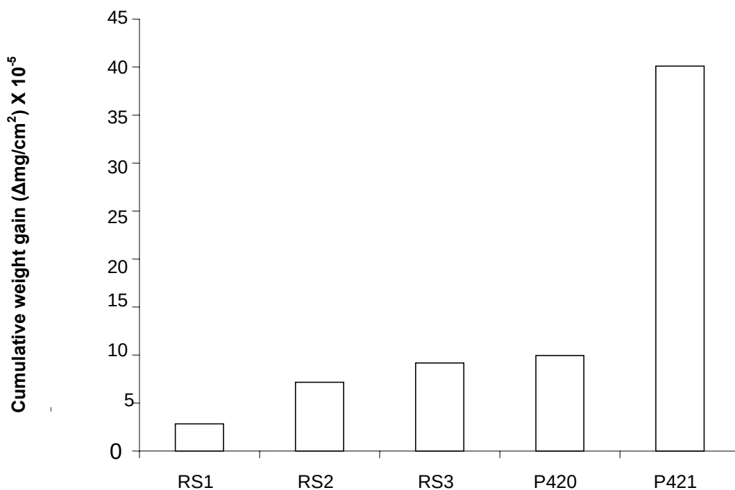
Figure 5.4 Cumulative weight gains of Pt-based superalloys after 792 hours in molten salt
