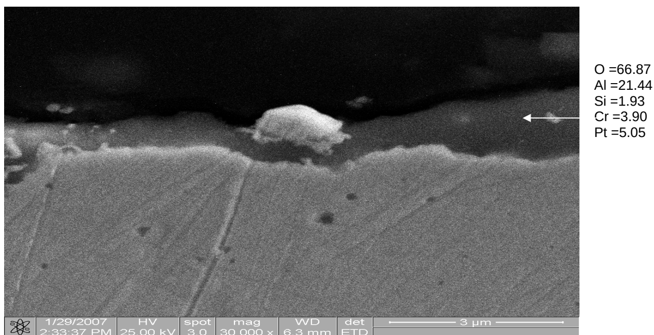
Figure 5.37 SEM image showing the external oxide layer that formed on the surface of alloy RS1
