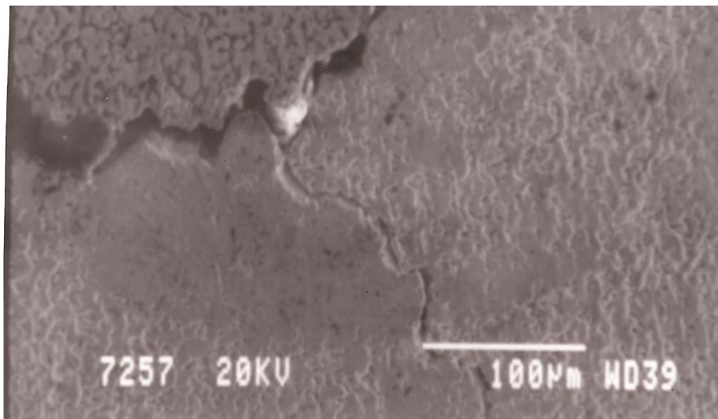
Figure 5.10 Secondary electron image of the surface morphology on alloy P420 after exposure to molten \text{Na}_2\text{SO}_4 salt for a period of 540 hours
