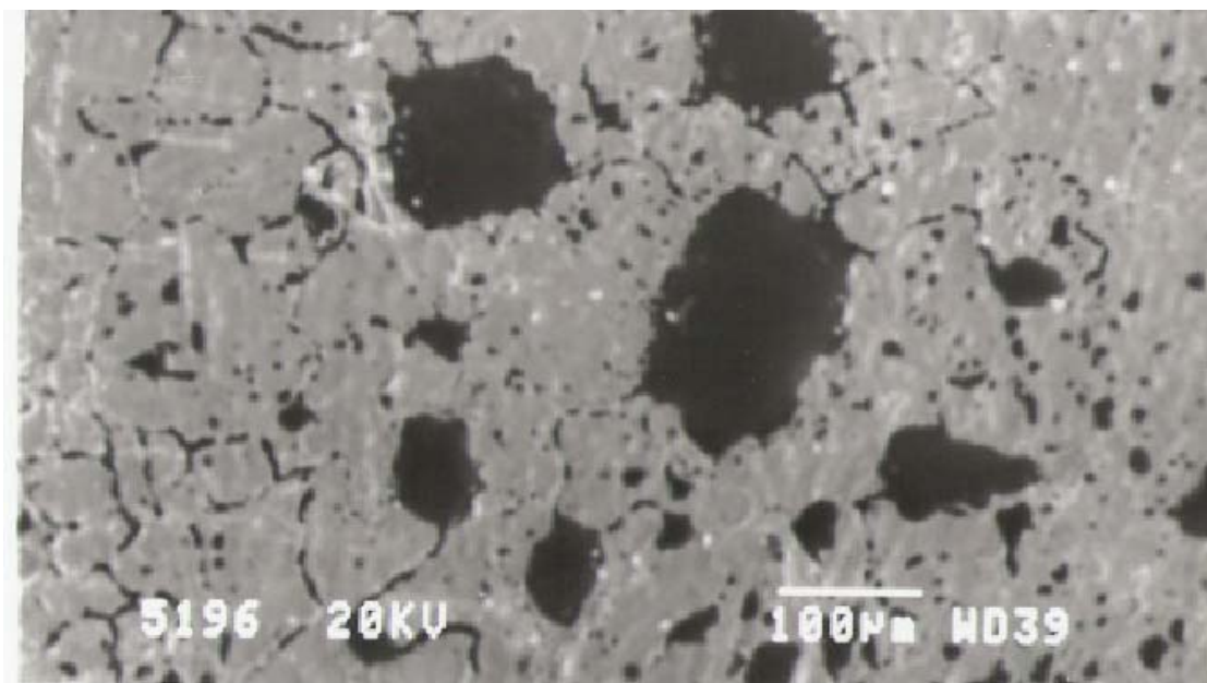
Figure 5.17 Secondary electron image of corrosion morphology of alloy RS3 after hot corrosion in molten Na 2 SO 4 salt at 950°C for duration of 792 hours
