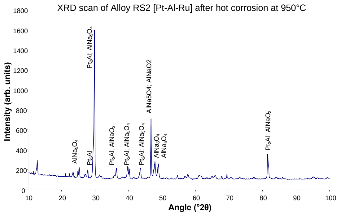
Figure 5.25 X-ray diffraction patterns on the scale of alloy RS2 after hot corrosion
