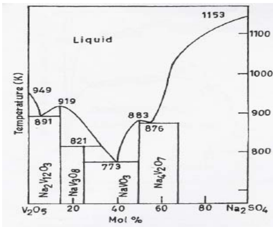
Figure 2.6 Equilibrium phase diagram for Na 2 SO 4 -V 2 O 5 [Gitanjaly et al. , 2002]
