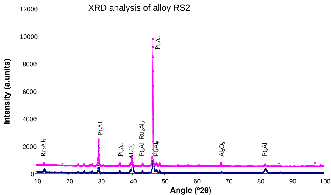
Figure 5.58 XRD spectrum performed on the external surface of alloy RS2 [Pt-Al-Ru] before and after exposure to 0.2% \text{SO}_2\text{-N}_2 atmosphere at 900°C for a period of 60 hours
