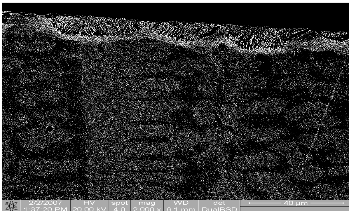
Figure 5.45 Secondary electron image of alloy P420 with the dendritic structure below the corroded area
