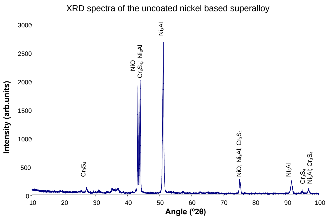
Figure 5.56 XRD pattern on the uncoated Ni-based superalloy after exposure to 0.2% \text{SO}_2 - \text{N}_2 atmosphere
