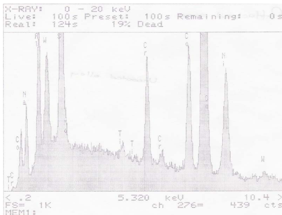
Figure 5.7 EDS analysis performed on the surface of the uncoated alloy that was exposed to molten salt at 950°C for a period of 792 hours
