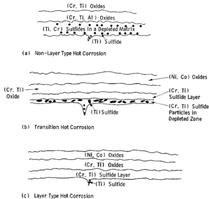
Fig. 8. Schematic characterization of corrosion products found at areas typical of the three different hot corrosion regions.
