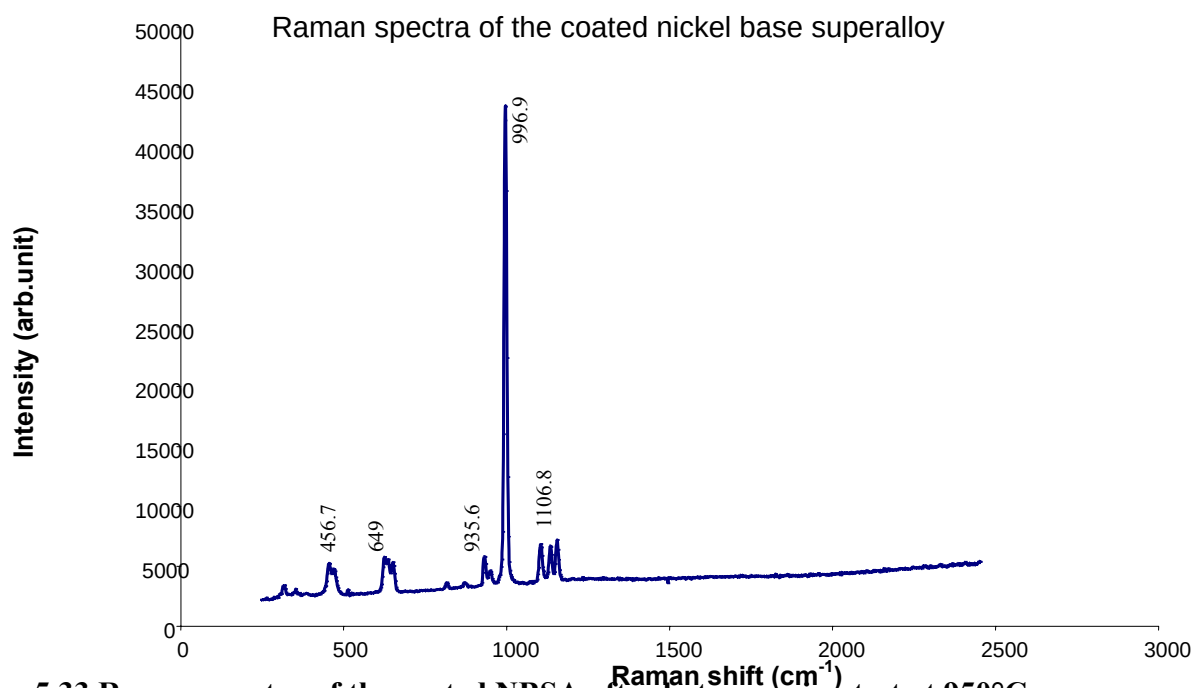
Figure 5.33 Raman spectra of the coated NBSA after hot corrosion test at 950°C
