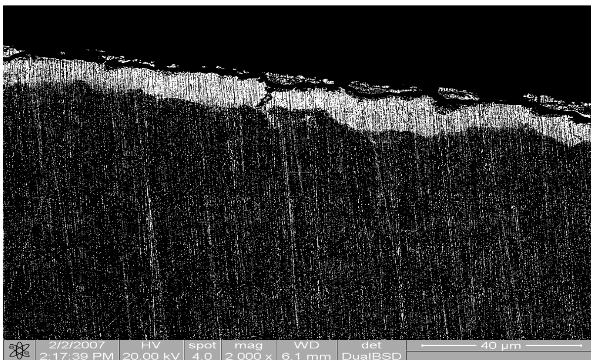
Figure 5.48 Transverse section of alloy P421 showing the Al depleted area after exposing the alloy to a 0.2% SO 2 -N 2 environment
