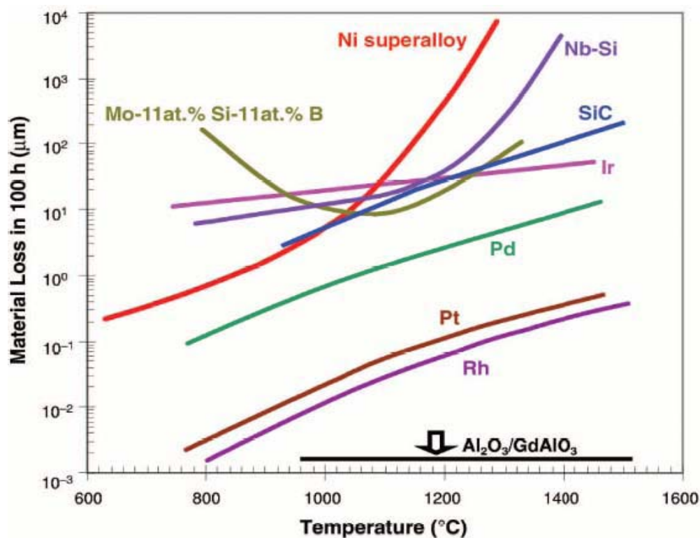
Figure 3.5 Oxidation resistant material used for high temperature applications [Cornish et al. , 2003]
