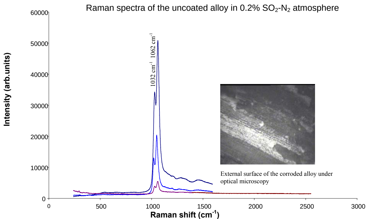
Figure 5.62 Raman spectra collected on the external surface of the uncoated alloy after sulphidation at 900°C for a period of 60 hours
