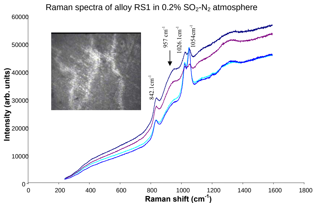
Figure 5.64 Raman spectra collected on the external surface of alloy RS1 after sulphidation at 900°C for a period of 60 hours
