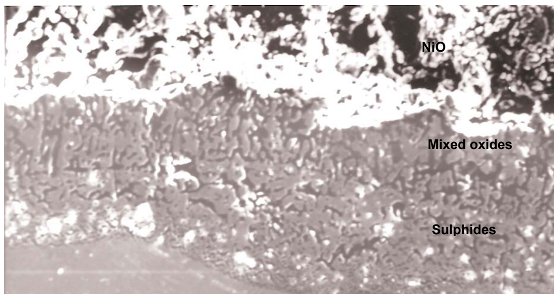
Figure 5.19 Cross sectional morphology of the uncoated alloy after hot corrosion attack in molten \text{Na}_2\text{SO}_4 salt
