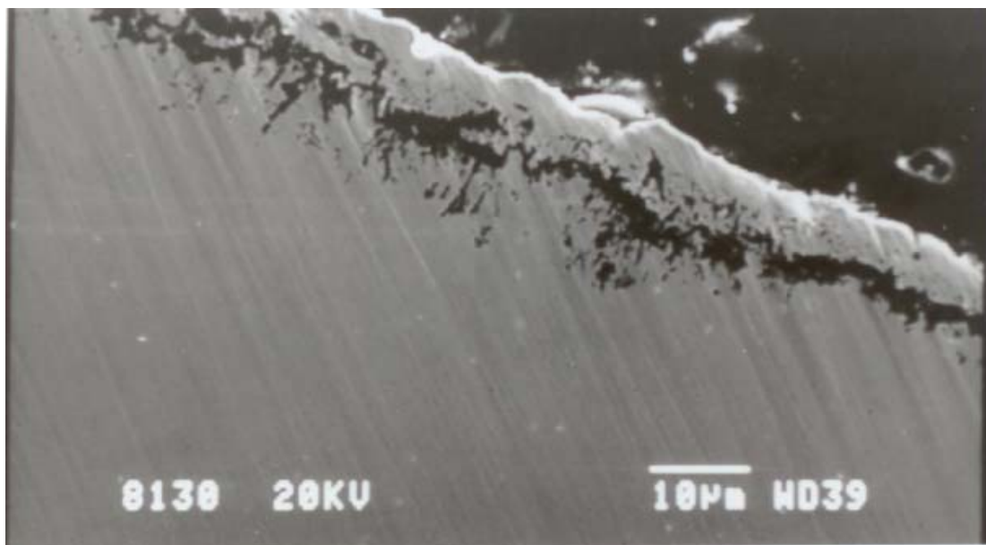
Figure 5.22 Secondary electron micrograph of the cross section of alloy RS2 after hot corrosion test at 950°C
