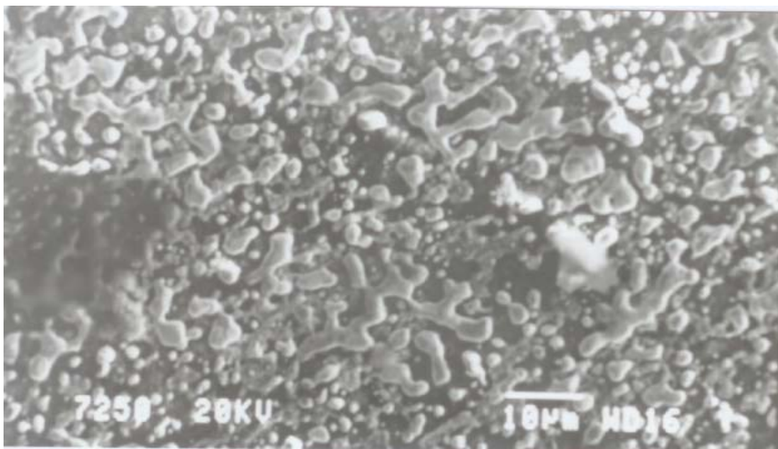
Figure 5.8 Secondary electron image of alloy P421 with non-protective oxide scale after hot corrosion at 950°C after 540 hours
