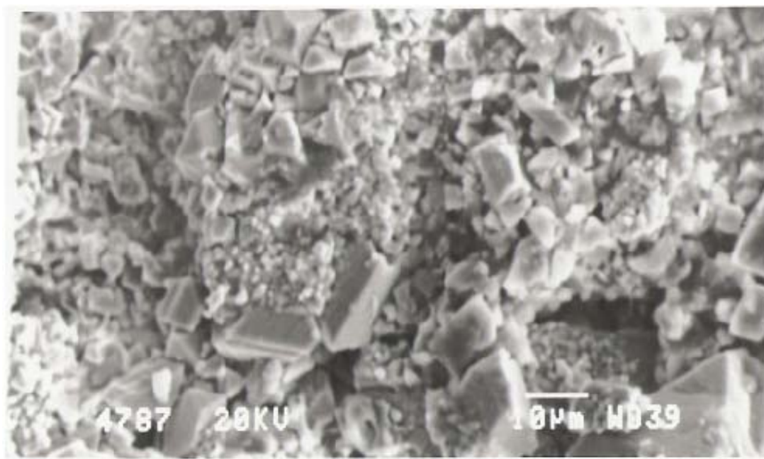
Figure 5.9 Secondary electron image of crystal structured corrosion morphology on alloy P421 after undergoing hot corrosion at 950°C for 792 hours
