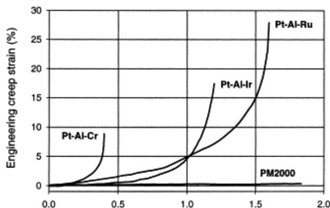
Figure 3.4 Stress rupture strength of an ODS alloy (PM2000) and ternary Pt-based superalloys at 1300 °C and 30 MPa [Süss et al. , 2002]
