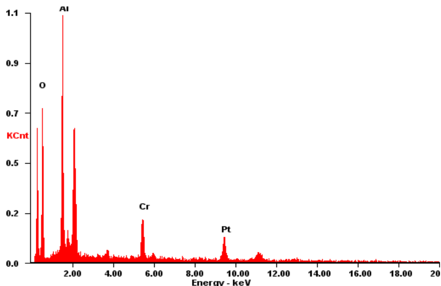
Figure 5.38 EDS analysis performed on the external scale that formed on the surface of alloy RS1 after the sulphidation test in 0.2% SO 2 -N 2 environment
