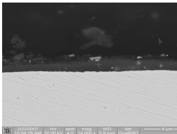
Figure 5.40 Cross section of alloy RS2 at 14000 X magnification with an \text{Al}_2\text{O}_3 scale forming on the surface of the alloy
