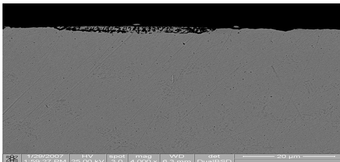
Figure 5.35 SEM image showing cross section of alloy RS1 after the sulphidation test in 0.2\%\text{SO}_2\text{-N}_2 gas at 900^\circ\text{C}
