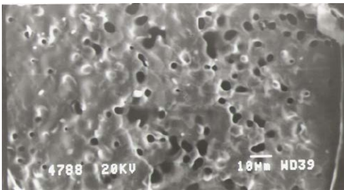
Figure 5.15 Secondary electron image of the corrosion morphology that resulted on the surface of alloy RS2 after at 950°C for 792 hours
