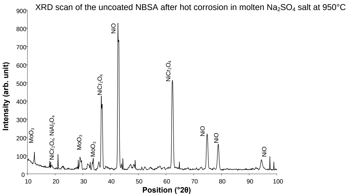
Figure 5.30 X-ray diffraction patterns on the surface of uncoated Ni-based superalloy after hot corrosion
