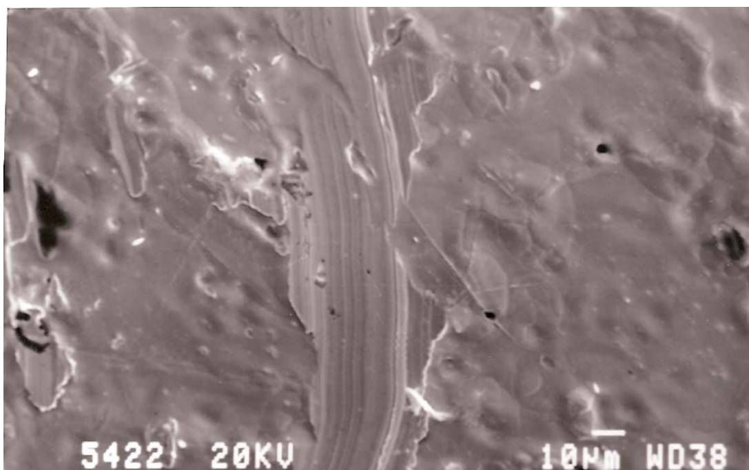
Figure 5.13 Secondary electron images of a porous oxide scale on the surface of alloy RS1 after hot corrosion in molten salt for 792 hours
