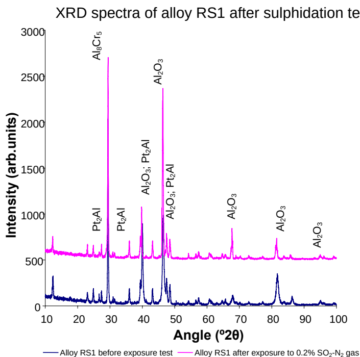
Figure 5.57 XRD spectra performed on the external surface of alloy RS1 before and after exposure to 0.2% \text{SO}_2\text{-N}_2 atmosphere at 900°C for a period of 60 hours
