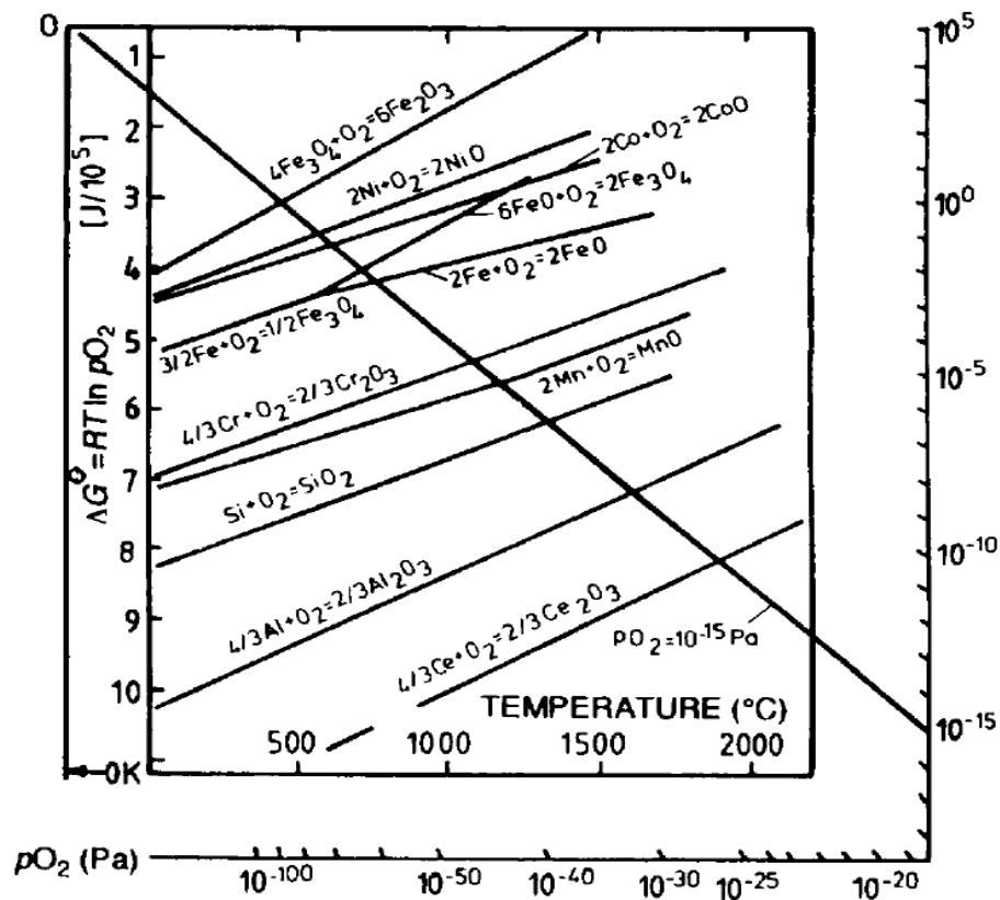
Figure 2.5 Ellingham diagram of oxides plotted against partial pressures [Gaskell, 1981]
