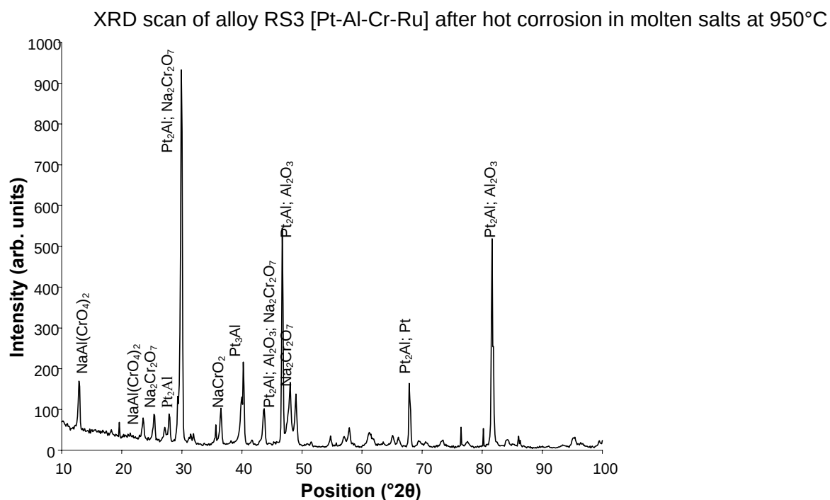
Figure 5.26 X-ray diffraction patterns on the surface of alloy RS3 after hot corrosion
