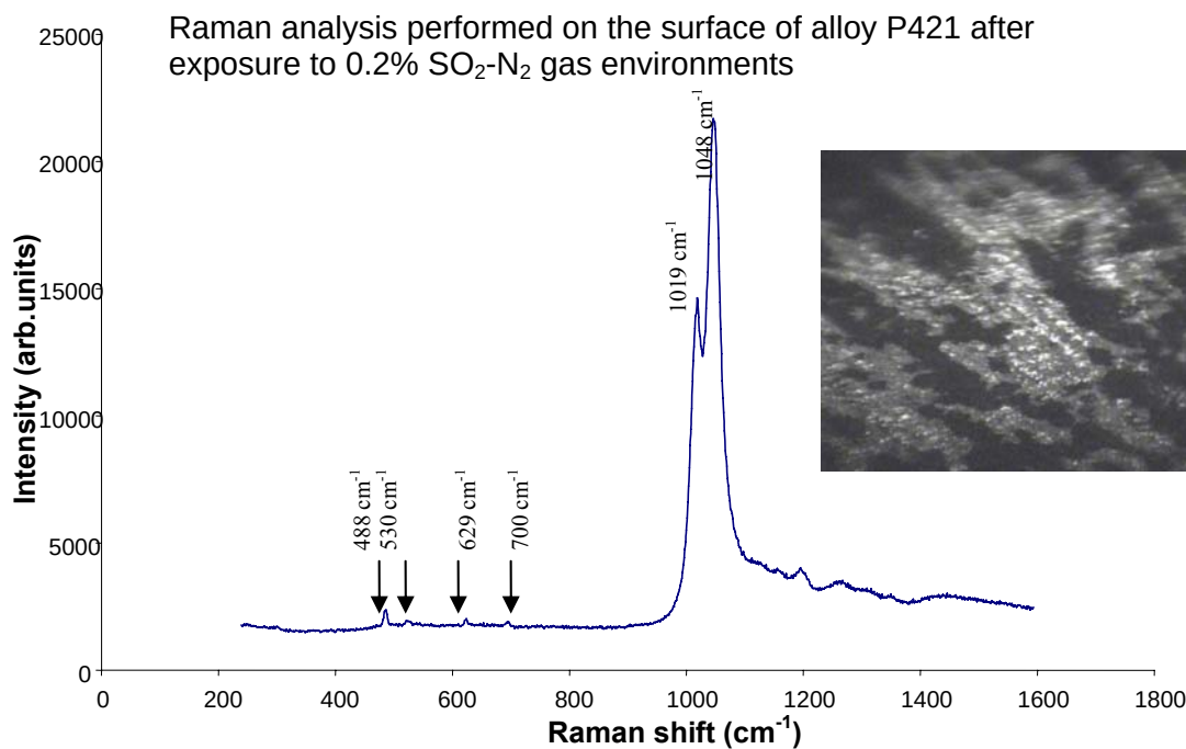
Figure 5.68 Raman spectra collected on the external surface of alloy P421 after sulphidation at 900°C for a period of 60 hours
