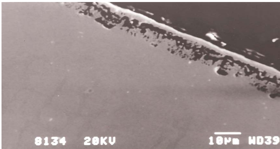
Figure 5.23 Secondary electron micrograph of the cross section of alloy RS3 after hot corrosion test at 950°C
