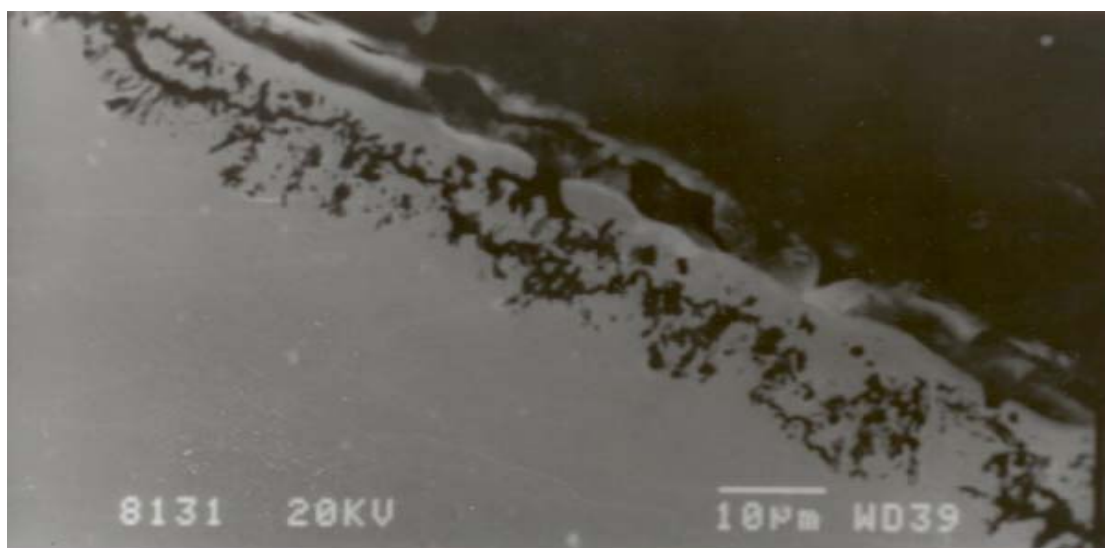
Figure 6.1 Cross section of alloy RS3 showing fluxing of the external scale when the alloys were immersed in molten \text{Na}_2\text{SO}_4 salt
