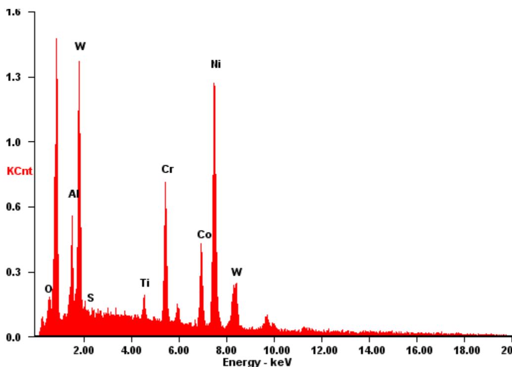
Figure 6.3 EDS spot analysis performed on the needles formed
