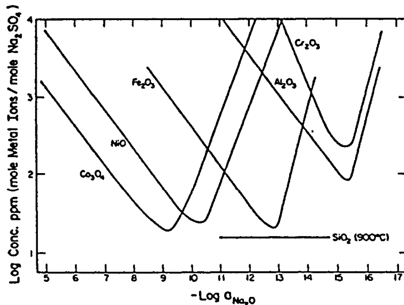
Figure 2.9 Calculated solubilities of metal oxides at 1200 K in molten \text{Na}_2\text{SO}_4 salt [Rapp, 2002]
