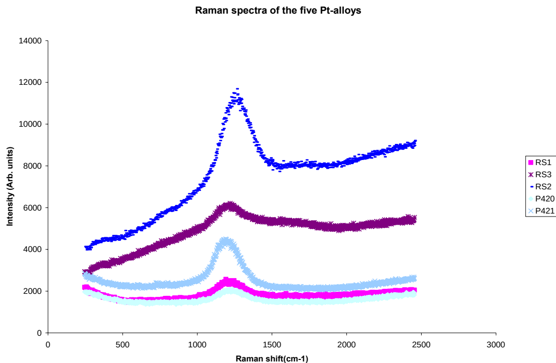
Figure 5.31 Raman spectra obtained from the five Pt-based superalloys after hot corrosion investigations at 950 °C
