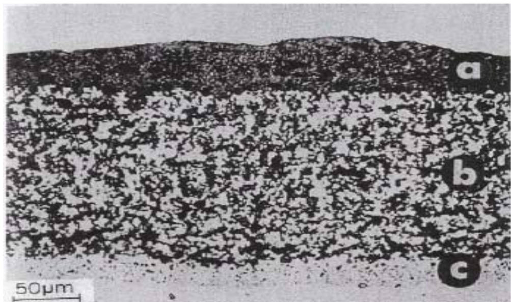
Figure 2.7 Typical microstructure of type I hot corrosion [Stringer, 1987]
