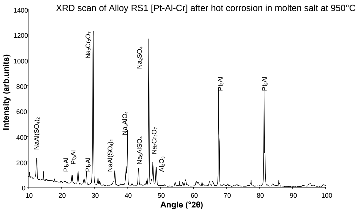
Figure 5.24 X-ray diffraction patterns on the scale of alloy RS1 after hot corrosion
