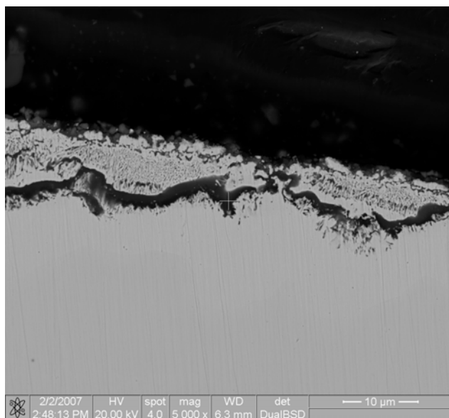
Figure 5.46 Transverse section of corroded alloy P421 after the sulphidation test at 900°C
