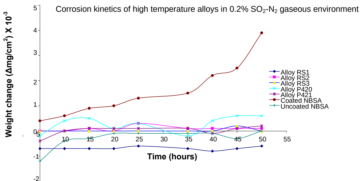
Figure 5.34 Corrosion kinetics of the seven investigated alloys after sulphidation in a 0.2% SO 2 -N 2 gaseous environment
