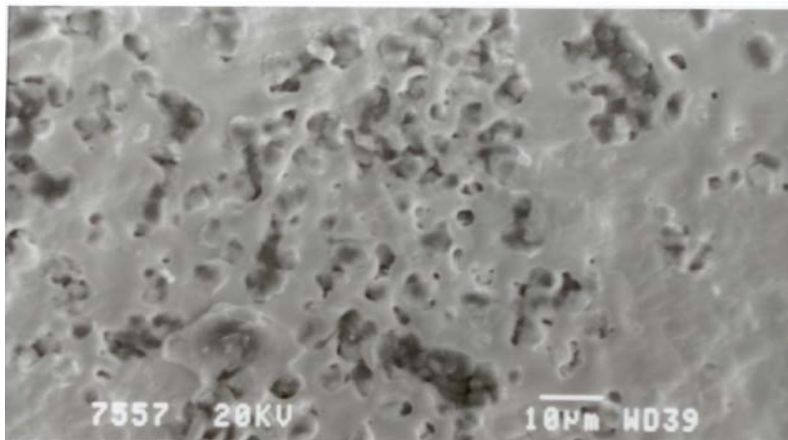
Figure 5.14 Secondary electron image of the corrosion morphology that resulted on the surface of alloy RS2 after at 950°C for 540 hours
