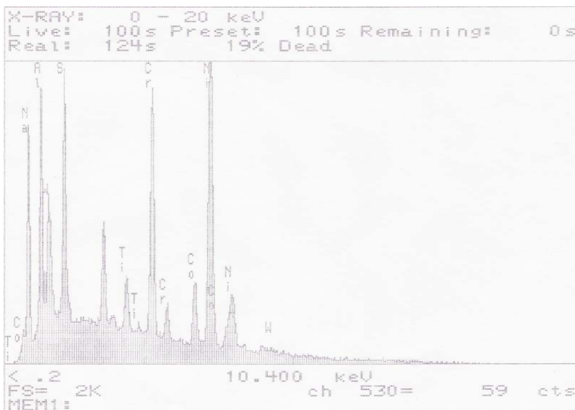
Figure 5.20 SEM scan obtained after performing cross sectional analysis on the surface of the uncoated alloy
