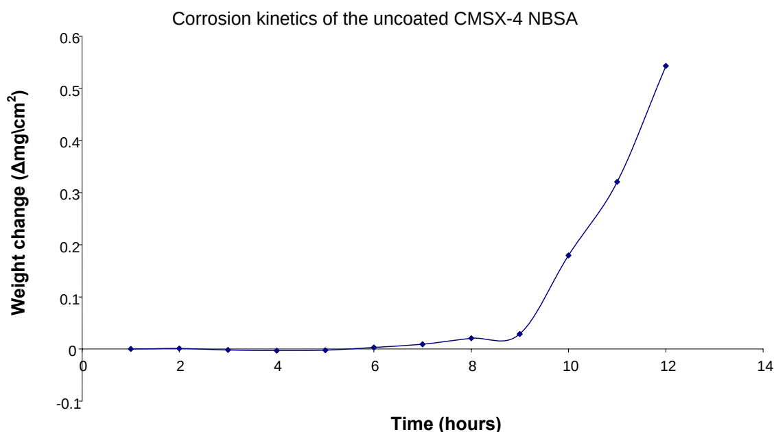
Figure 5.1 Corrosion kinetics of uncoated Ni-based superalloy (CMSX-4) after exposure to molten \text{Na}_2\text{SO}_4 salt at 950^\circ\text{C}
