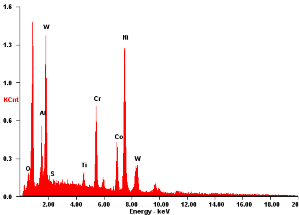
Figure 5.52 EDS analysis performed on the needle-like phases that formed between the substrate and the coating
