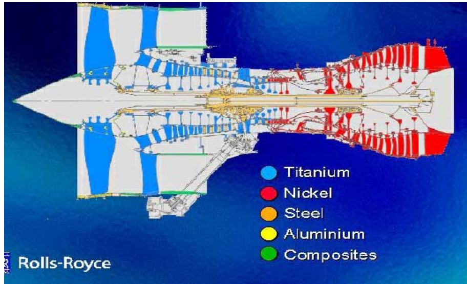
Figure 2.1 Different materials used in the aerospace industry [Bhadesia, 2003]
