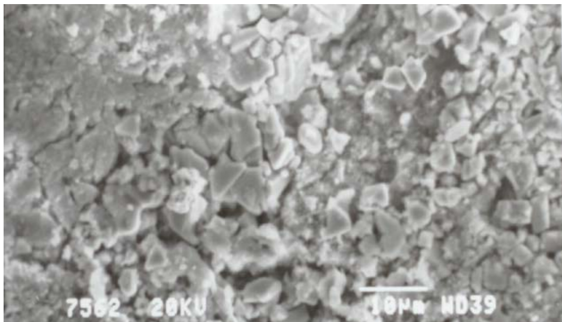
Figure 5.5 Secondary electron micrograph showing corrosion morphology of the coated NBSA that resulted after hot corrosion in molten Na 2 SO 4 salt at 950°C
