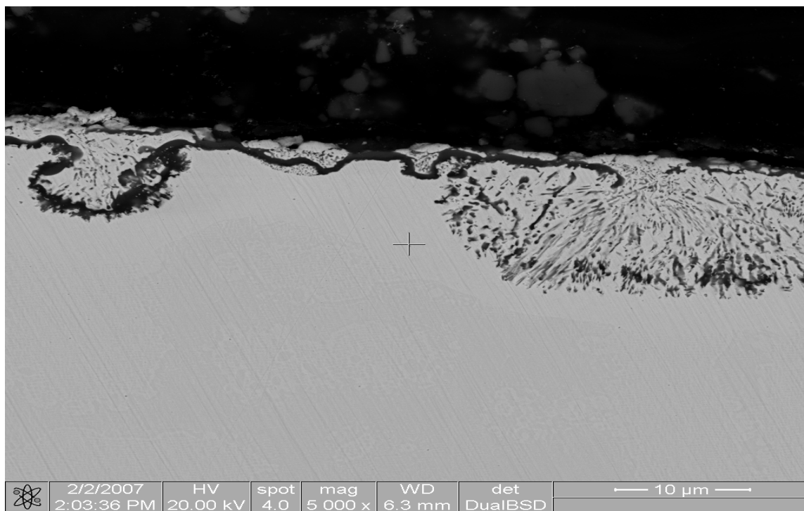
Figure 5.44 Secondary image of alloy P420 after sulphidation test in 0.2% SO 2 -N 2 environment
