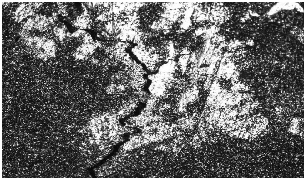
Figure 6.2 Spallation around the cracks on the surface of alloy P420 that was subjected to molten salts at 950°C for a period of 540 hours
