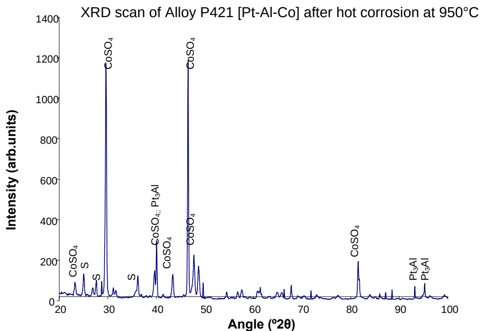
Figure 5.28 X-ray diffraction patterns on the surface of alloy P421 after hot corrosion
