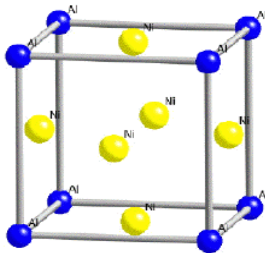
Figure 2.2 A fcc crystal structure of the \gamma' precipitate [Bhadesia, 2003]
