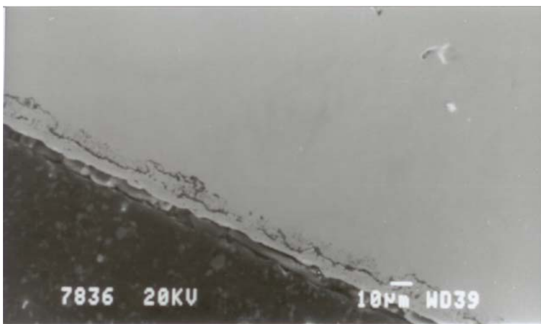
Figure 5.21 Secondary electron micrograph of the cross section of alloy RS1 after hot corrosion test at 950°C
