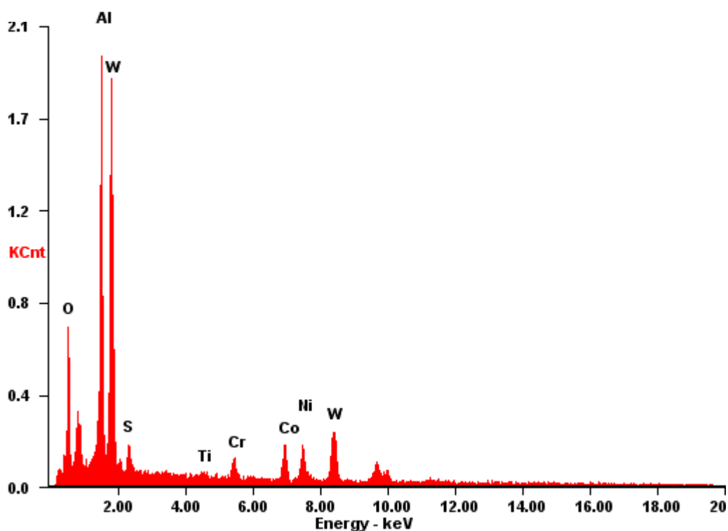
Figure 5.53 EDS analysis performed on the coated alloy in the area below the \text{Al}_2\text{O}_3 scale
