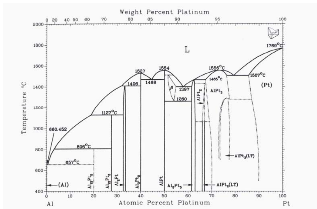
Figure 3.1 Binary phase diagram of Pt-Al system [Massalski et al. , 1986]
