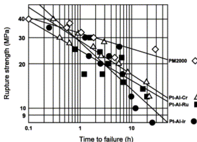
Figure 3.3 Stress rupture strength of an ODS alloy (PM2000) and ternary Pt-based superalloys at 1300 °C in air [Süss et al. , 2002]
