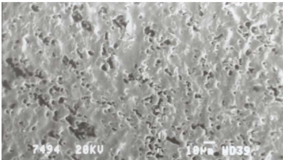
Figure 5.12 Secondary electron images showing a porous oxide scale on the surface of alloy RS1 after hot corrosion in molten salt for 540 hours
