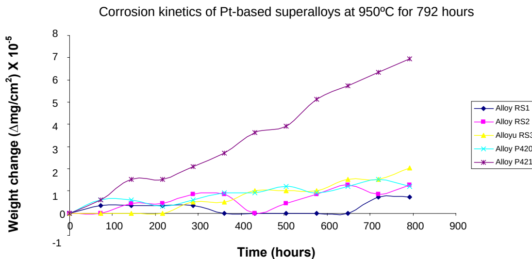
Figure 5.3 Corrosion kinetics of Pt-based superalloys in molten salts at 950°C for duration of 792 hours
