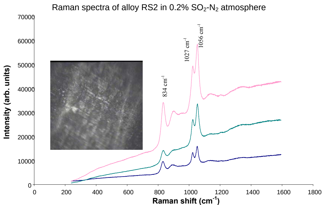
Figure 5.65 Raman spectra collected on the external surface of alloy RS2 after sulphidation at 900°C for a period of 60 hours
