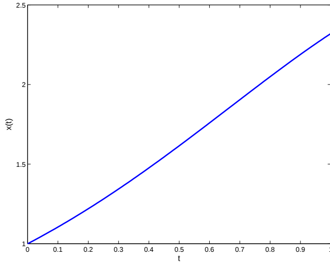
Figure 1.1: Graph of the exact solution to Problem ODE1
