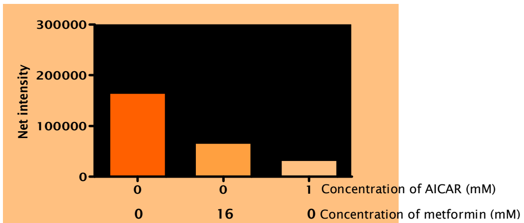
Figure 3.9: (A) Comparison of the cytoplasmic level of NF- \kappa B in metformin and AICAR treated cultures and control cells. Data is expressed as mean \pm SD from 3 experiments. (B) Comparison of the nuclear level of NF- \kappa B in metformin and AICAR treated cells and control cells. Data is expressed as mean \pm SD from 5 experiments; * p < 0.05 versus controls.
