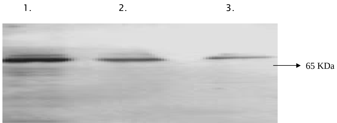
Figure 3.8: (A) Western blotting of the cytoplasmic extracts of U1 cells with anti-NF- \kappa B antibody: control cells, lane 1, metformin treated cells, lane 2; AICAR treated cells, lane 3. This is representative of 3 Western blots. 4 \mu g of protein were loaded in each well (B) Western blotting of the nuclear extracts of U1 cells with anti-NF- \kappa B antibody: control cells, lane 1, metformin treated cells, lane 2, and AICAR treated cells, lane 3. This blot is representative of 5 Western blots. 4 \mu g of protein were loaded in each well.
