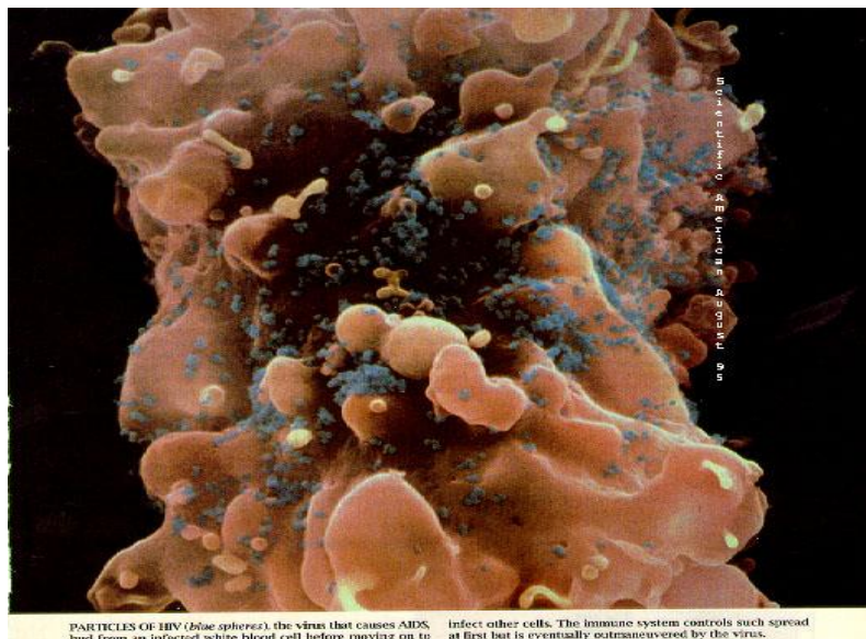
Figure 1.8: A photograph of HIV, in blue, budding from a T-cell [65].
