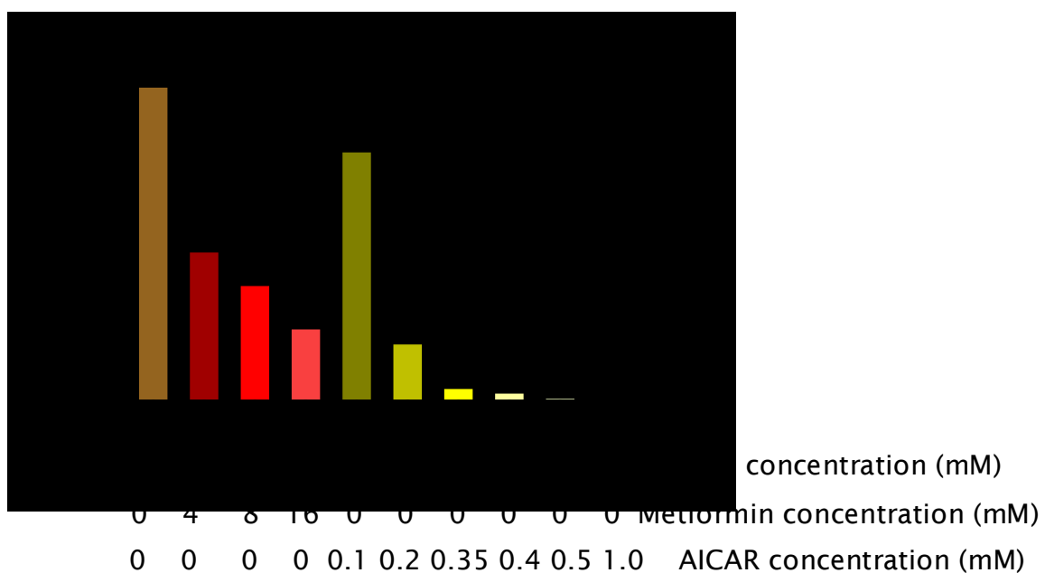
Figure 3.5. Determination of metformin and AICAR concentrations that had the strongest inhibition of HIV-1 replication in U1 cells.
