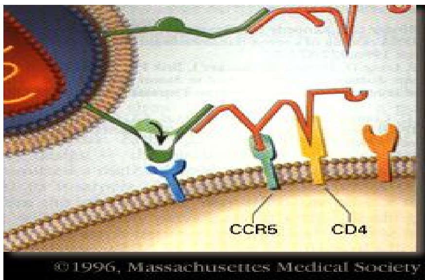
Figure 1.6: (A) and (B) Show the interaction of HIV-1 gp120 and gp41 with the host cell receptor CD4 and co-receptor CCR5 [62].
