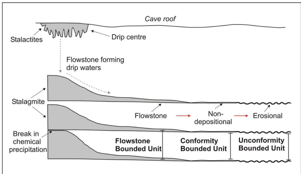
Figure 3.3. Schematic diagram showing a classic Flowstone Bounded Unit and its correlative conformity and unconformity bounded units, depending on the boundary conditions of the unit.
