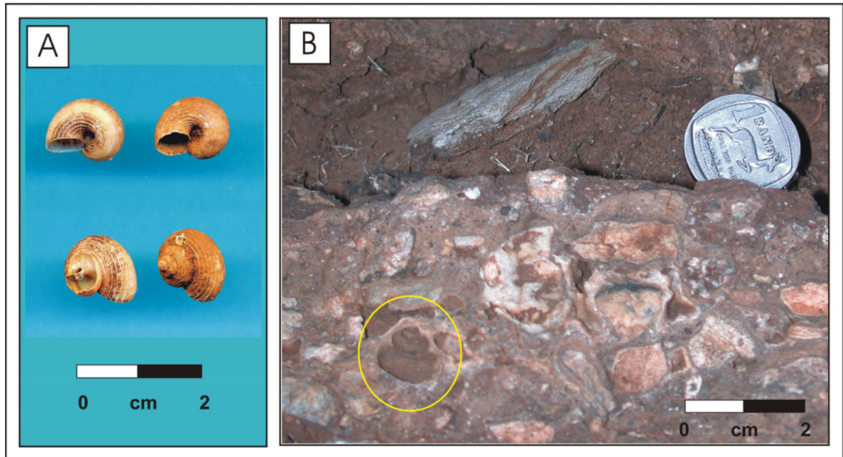
Figure 3.8. Specimens of the snail Trophidophora insularis , A: Isolated specimens recovered from decalcified sediments, B: Snail impression in breccia FBU LK from the Eastern Face 1.
