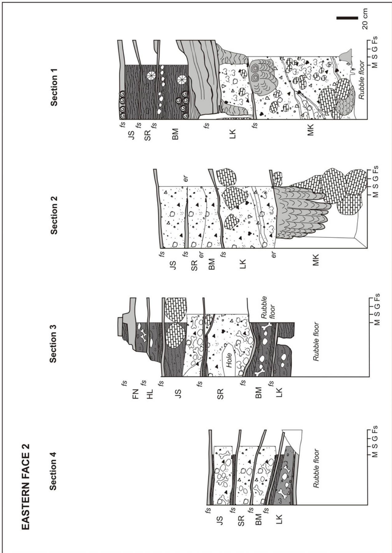
Figure 3.23. Stratigraphic sections for the Eastern Face 2.
