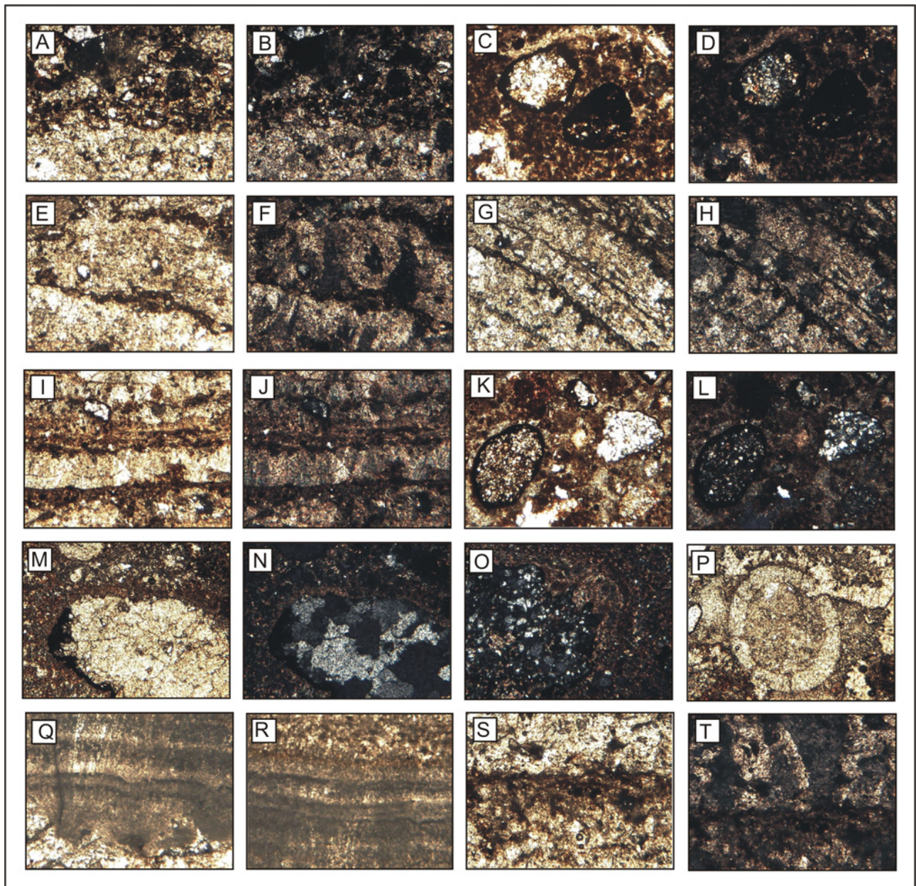
Figure 3.4. Photomicrographs of thin section from the basal units of the Western Face 1, in plane polarised (pp) and crossed polarised (xp) light. Scale on all pictures is 1.6mm across the base of the image. A: Flowstone sediment interface from SR (pp), B: Flowstone sediment interface from SR (xp). C Sediment from SR showing polycrystalline quartz grains (pp), D: Sediment from SR showing polycrystalline quartz grains (xp). E: SR lower flowstone, showing detrital contamination (pp), F: SR lower flowstone, showing detrital contamination (xp). G: SR lower flowstone, showing detrital contamination (pp), H: SR lower flowstone, showing detrital contamination (xp). I: BM flowstone (pp), J: BM flowstone (xp). K: BM sediment showing polycrystalline quartz grains (pp), L: BM sediment showing polycrystalline quartz grains (xp). M: LK sediment showing polycrystalline quartz grain (pp), N: LK sediment showing polycrystalline quartz grain (xp). O: LK sediment showing polycrystalline quartz grain (xp). P: Fossil bone from LK (pp). Q and R: FBI 2 upper flowstone, showing bladed aragonite crystals and detrital contamination (pp). S: FBI 2 upper flowstone with detrital contamination (pp), T: FBI 2 upper flowstone with detrital contamination, calcite crystals seen better under crossed polars (xp).
