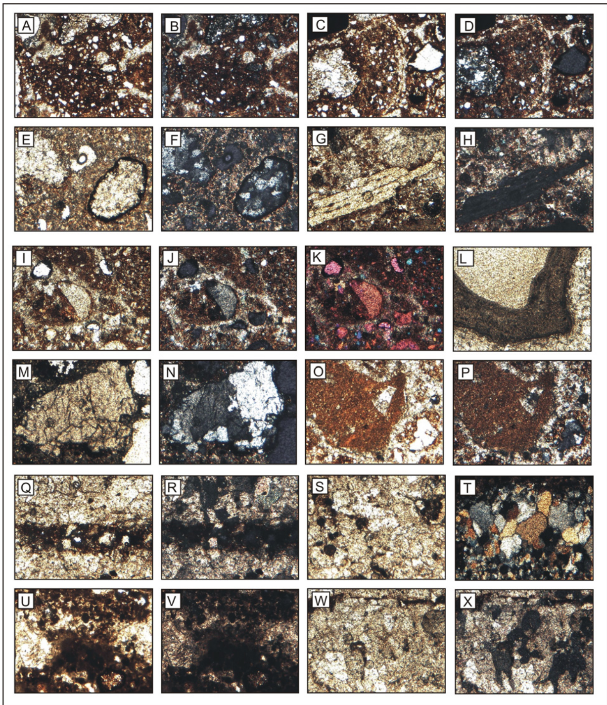
Figure 3.5. Photomicrographs of thin section from the upper units of the Western Face 1. Scale on all pictures is 1.6mm across the base of the image. A and C: Sediment from FN showing pedo-relic particles (pp), B and D: Sediment from FN showing pedo-relic particles (xp). E: Sediments from HL showing polycrystalline quartz grains (pp), F: Sediments from HL showing polycrystalline quartz grains (xp). G: Bone fragment from HL (pp), H: Bone fragment from HL (xp). I: HL sediments (pp), J: HL sediments (xp), K (xp, gypsum plate). L: Bone from HL (pp). M: polycrystalline quartz grain from HL (pp), N: polycrystalline quartz grain from HL (xp). O: Pedo-relic particle from HL (pp), P: Pedo-relic particle from HL (xp). Q: JS top flowstone with layer of detritus (pp), R: JS top flowstone with layer of detritus (xp). S: Sediment from JS showing polycrystalline quartz grain (pp), T: Sediment from JS showing polycrystalline quartz grain (xp). U: JS lower flowstone, with significant detrital contamination (pp), V: JS lower flowstone, with significant detrital contamination (xp). W: JS lower flowstone with slightly less detritus (pp), X: JS lower flowstone with slightly less detritus (xp).
