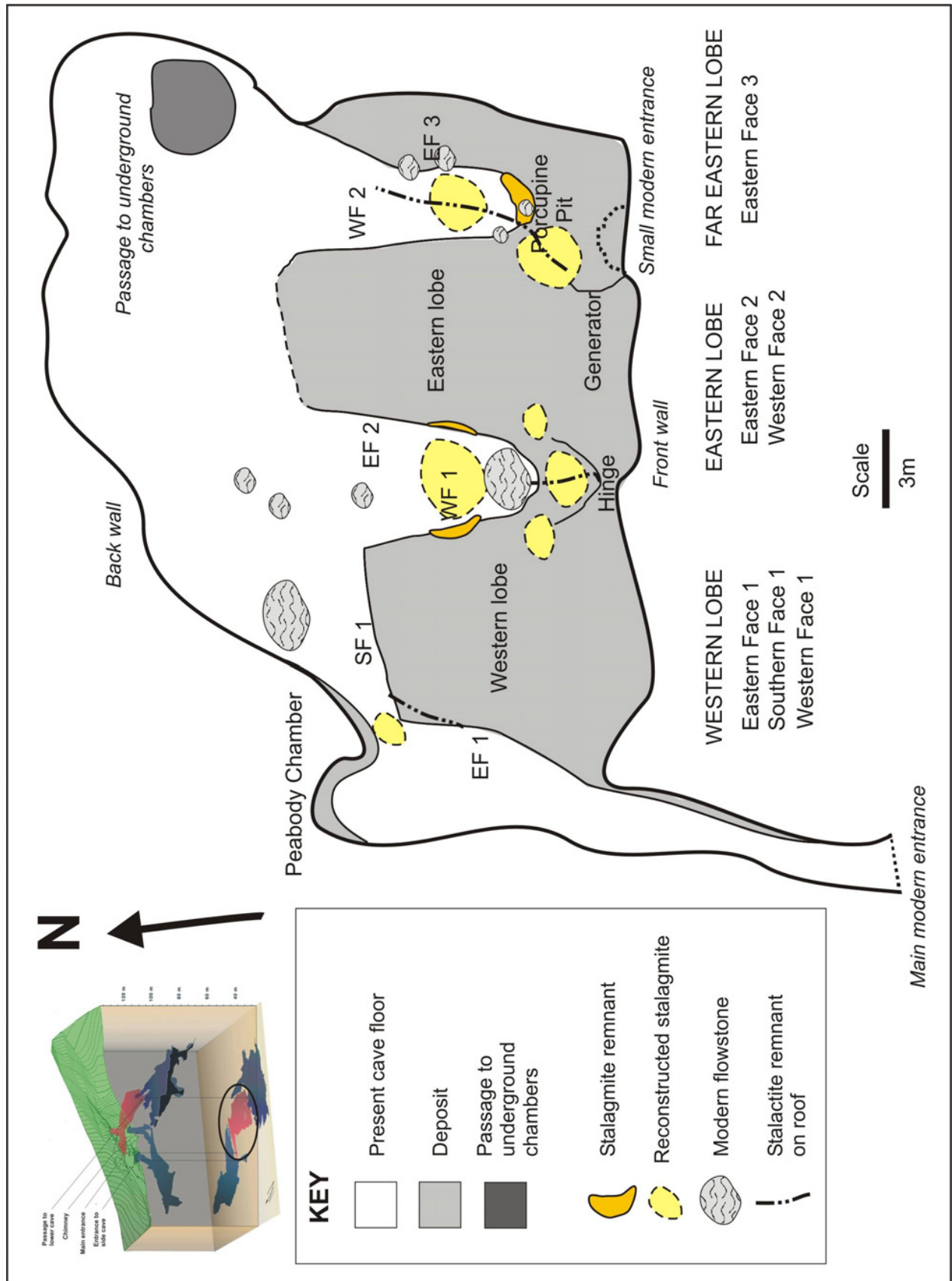
Figure 3.2. Schematic diagram of Gladysvale Cave in plan view showing drip centre reconstruction.
