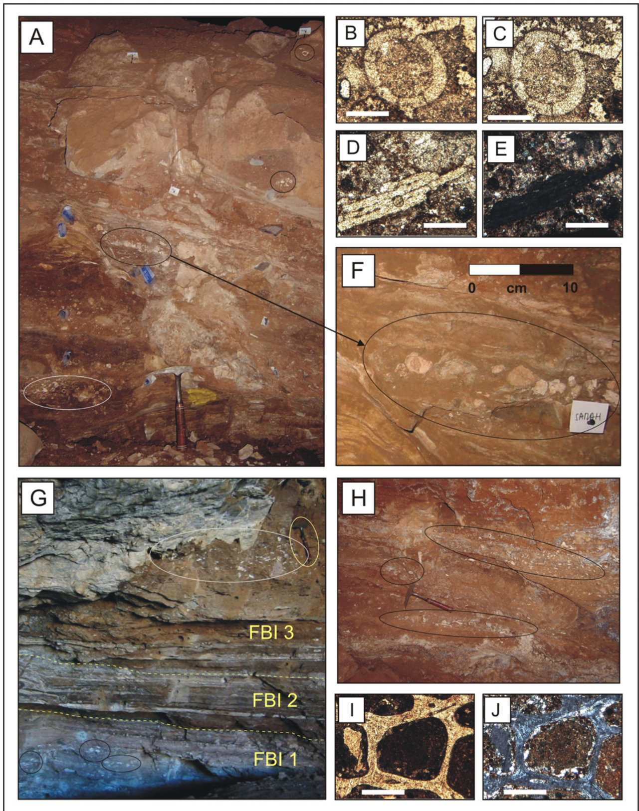
Figure 3.7. Fossil bone and coprolite occurrence in the younger internal deposits at Gladysvale Cave. A: Fossil bone occurrences in the Western Face 1 (30cm geopick for scale); B – E: photomicrographs of bone from the Western Face 1 (scale bar 0.5mm, B & D plane polarised light, C & E crossed polars); F: an enlargement of the accumulation of hyena coprolites in unit SR; G: Bone occurrence in the Peabody Chamber, including those in FBI 1 (30cm geopick for scale, circled in yellow); H: Dense bone accumulations in the Peabody Extension section; I & J: photomicrographs of spongy bone from the Peabody Chamber (scale bar 0.05mm, I plane polarised light, J crossed polars).
