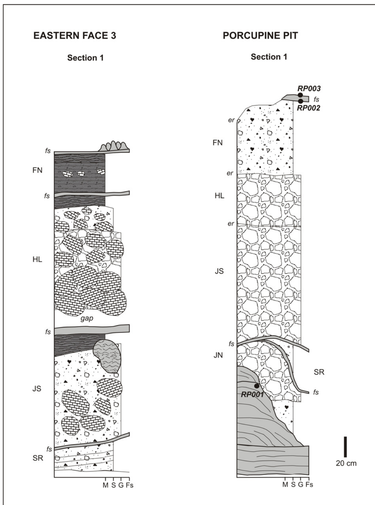
Figure 3.26. Stratigraphic columns for the Eastern Face 3 (left) and the Porcupine Pit (right).
