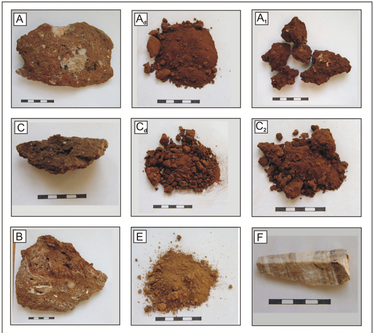
Figure 3.10. Photographs of samples of Gladysvale sedimentary facies: Letter inserts refer to facies name: Photograph A: Facies A. A_d is the decalcified version of Facies A. Photograph A_1 : variation A_1 of facies A (note darker colour). Photograph C: Facies C (note dark brown colour and lack of clasts). C_d is the decalcified version of Facies C. C_2 is one of the variations of Facies C. Photograph B: Facies B (note reddish brown colour, presence of fossil bone and thin pervasive flowstones). Photograph E: Facies E, yellowish brown version of Facies E (note powdery texture, decalcified nature and lack of clasts). Photograph F: Facies F, flowstone, this sample is from the basal stalagmite in the Porcupine Pit and is a good example of the layered nature of the Gladysvale flowstones. Scale bar in cm.
