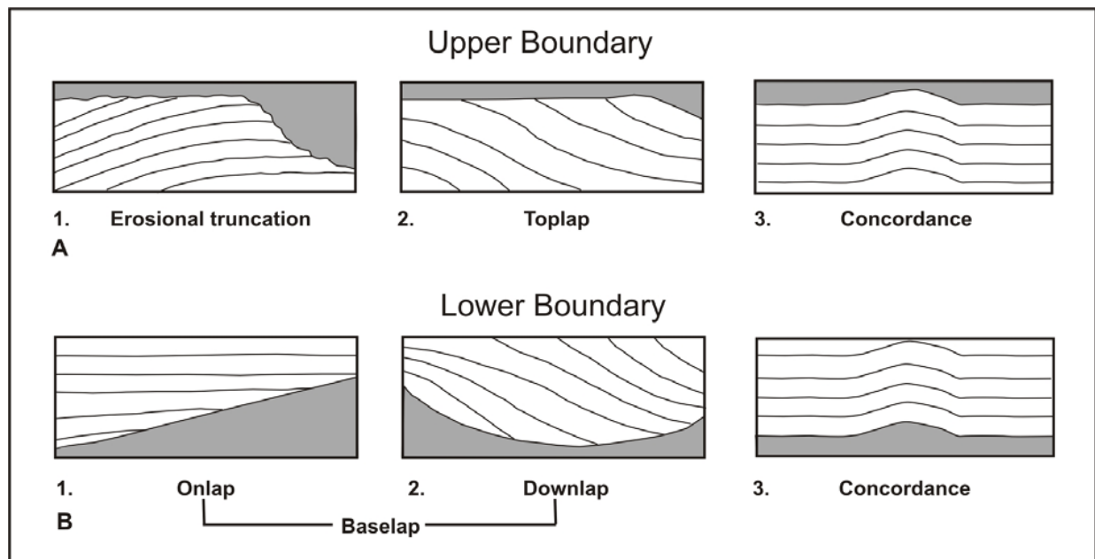
Figure 3.11. Sequence stratigraphic terminologies as used in this study. Relationships of strata to the upper boundary (A) and lower boundary (B) of a depositional sequence (Mitchum et al. , 1977).
