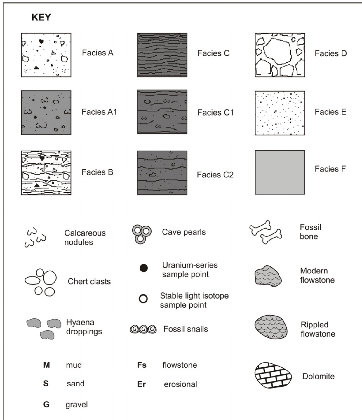
Figure 3.12. Key for facies and sedimentary structures recorded in the Gladysvale stratigraphic columns.
