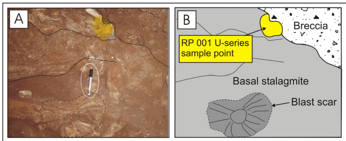
Figure 3.1. Photograph (A) and line drawing (B) showing blast scar and RP001 U-series sample point (yellow) in the Porcupine Pit (12 cm pen for scale, circled in white).
