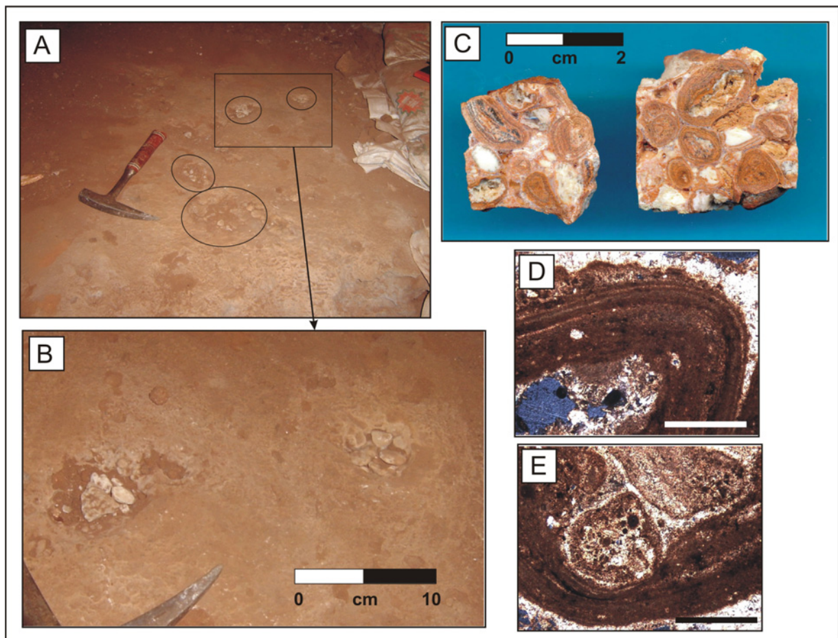
Figure 3.9. Cave pearls at Gladysvale Cave: A: Modern flowstone growing in the Hinge area, showing pits with cave pearls (30 cm geopick for scale); B: enlargement of cave pearls from Figure A; C: Cave pearl 'conglomerate'; D & E: photomicrographs of cave pearls, showing multi-layered coatings and single grain nuclei (D) and multi-grain, micropeds nuclei (E) (0.5mm scale bar, crossed polars).
