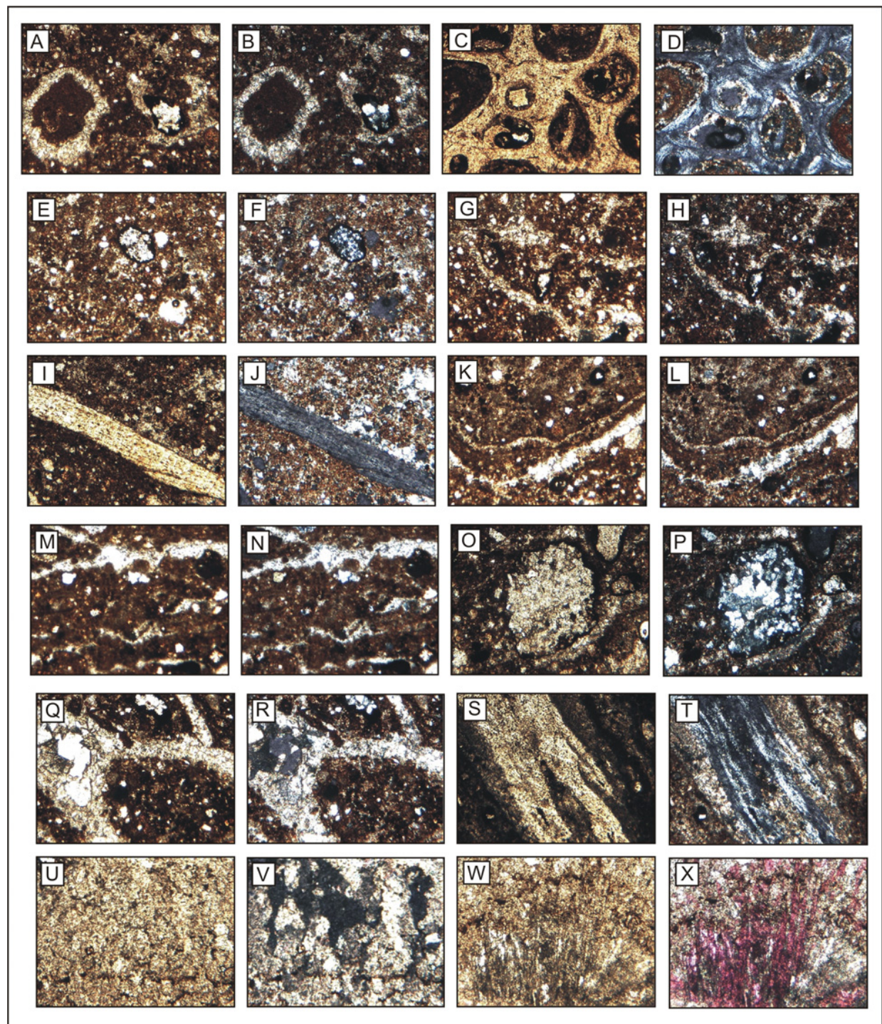
Figure 3.6. Photomicrographs of thin section from the Peabody Chamber. Scale on all pictures is 1.6mm across the base of the image. A: Sediment from FN showing calcite rims around grains (pp), B: Sediment from FN showing calcite rims around grains (xp). C: Spongy bone from HL (pp), D: Spongy bone from HL (xp). E: Sediment from HL showing polycrystalline quartz grain (pp), F: Sediment from HL showing polycrystalline quartz grain (xp). G: Sediment from JS showing calcite rims on grains (pp), H: Sediment from JS showing calcite rims on grains (xp). I: Bone from JS (pp), J: Bone from JS (xp). K: Pedo-relic with calcite rim from SR (pp), L: Pedo-relic with calcite rim from SR (xp). M: Calcite rich sediment from BM (pp), N: Calcite rich sediment from BM (xp). O: LK sediment showing polycrystalline quartz grain (xp), P: LK sediment showing polycrystalline quartz grain (xp). Q: pedo-relic and polycrystalline quartz grain with calcite rims from LK (pp), R: pedo-relic and polycrystalline quartz grain with calcite rims from LK (xp). S: Bone from LK (pp), T: Bone from LK (xp). U: FBI 2 top flowstone (pp), V: FBI 2 top flowstone (xp). W: FBI 2 top flowstone showing bladed aragonite crystals (pp), X: FBI 2 top flowstone showing bladed aragonite crystals (pp with gypsum plate).
