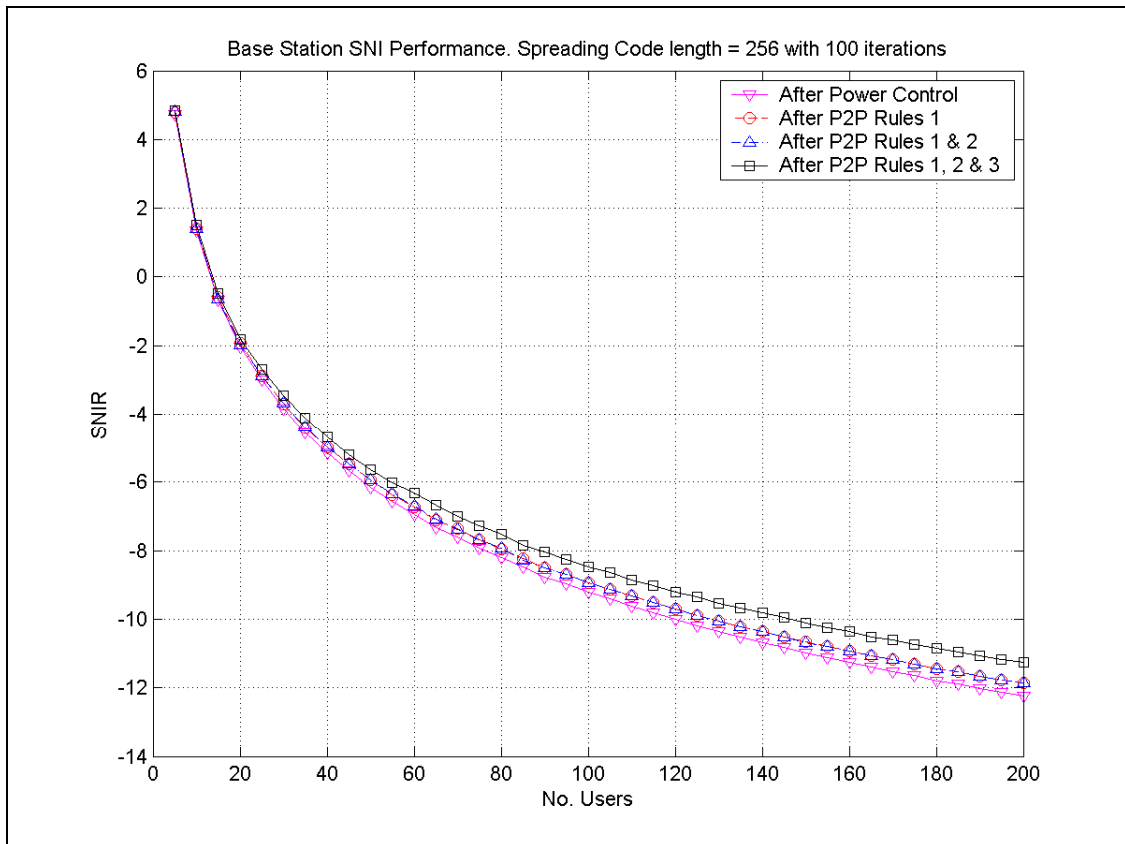
Figure 7.6: SNI Performance at the Base Station
