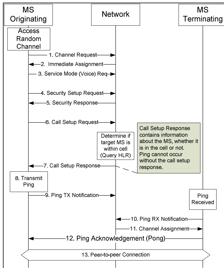
Figure 4.5: Call setup procedure
