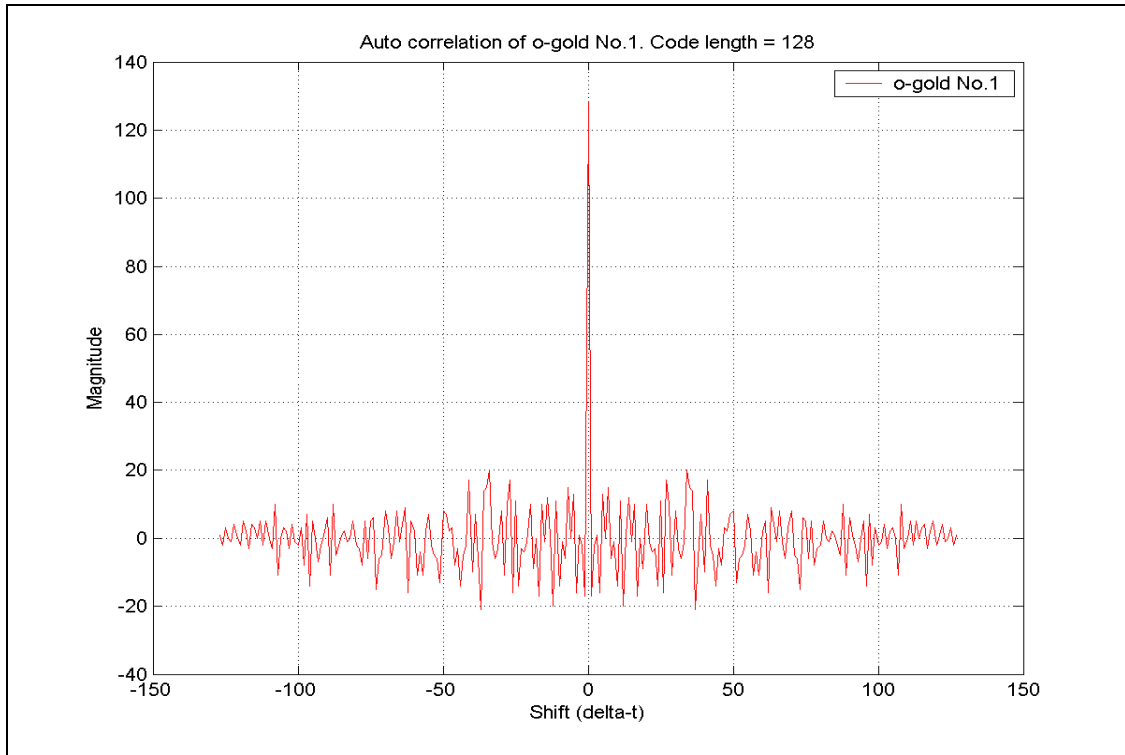
Figure 5.3: Auto-correlation result of an orthogonal Gold code sequence
