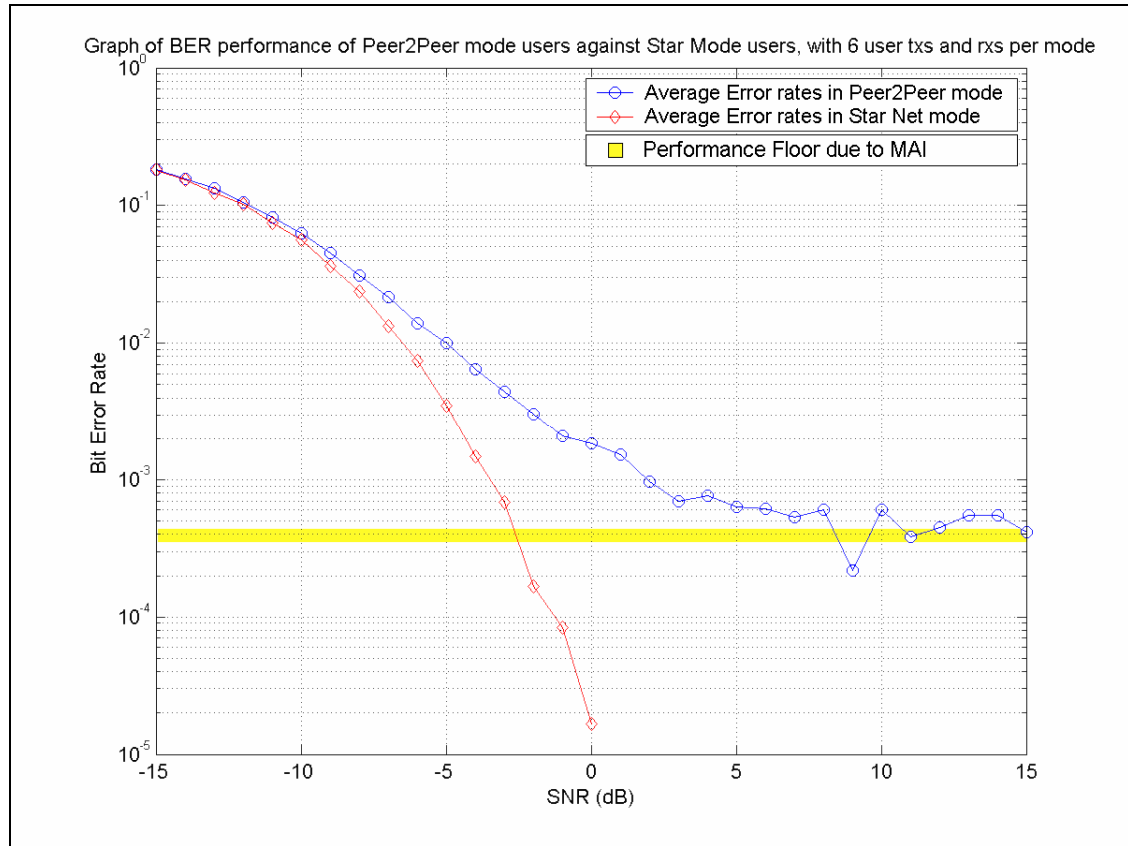
Figure 5.7: BER performance of 6 CDD users against 6 standard users with code length 128
