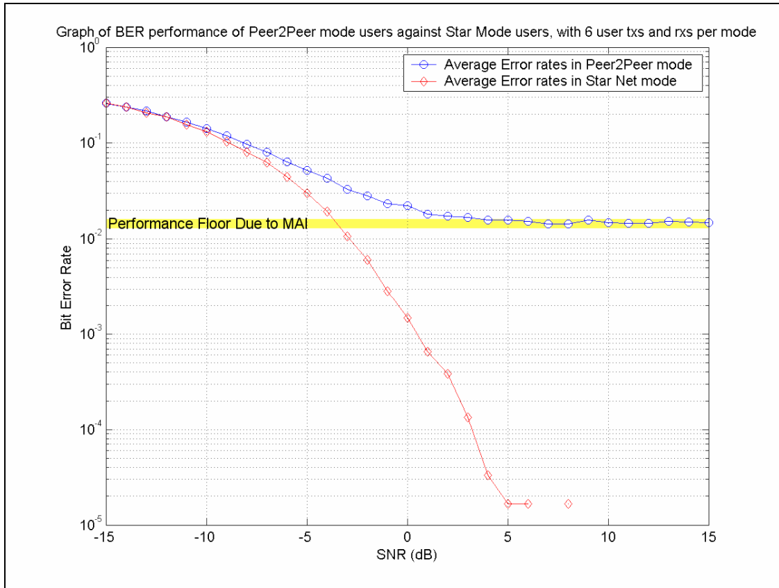
Figure 5.6: BER performance of 6 CDD users against 6 standard users with code length 64
