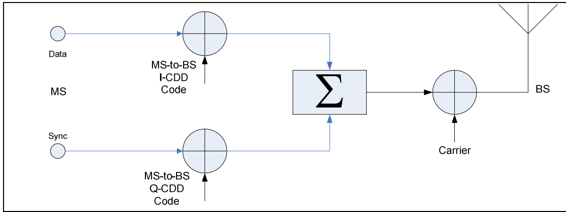
Figure 2.8: Coding For CDD [17]
