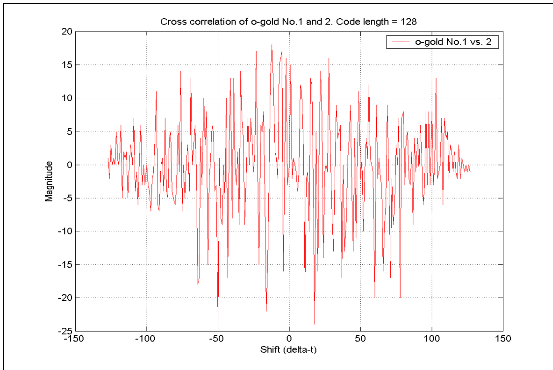
Figure 5.2: Cross-correlation result of two orthogonal Gold code sequences
