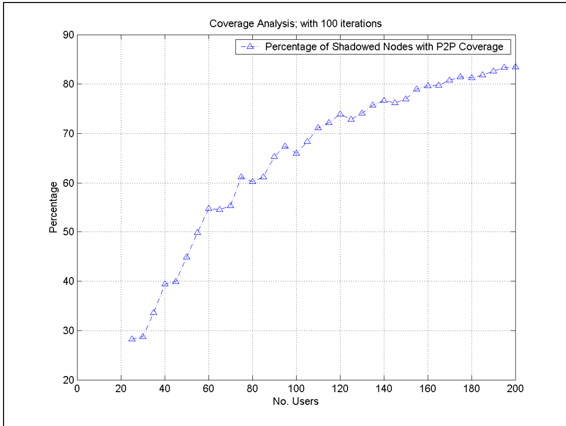
Figure 7.5: Ratio of Shadowed Nodes with Peer-to-peer Coverage to Shadowed Nodes for 2 Slots
