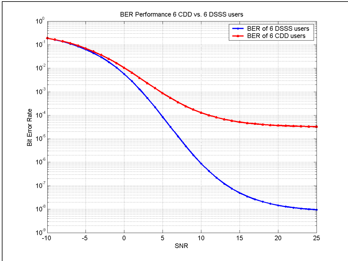
Figure 7.1: Theoretical Performance of 6 CDD users vs. 6 DSSS users
