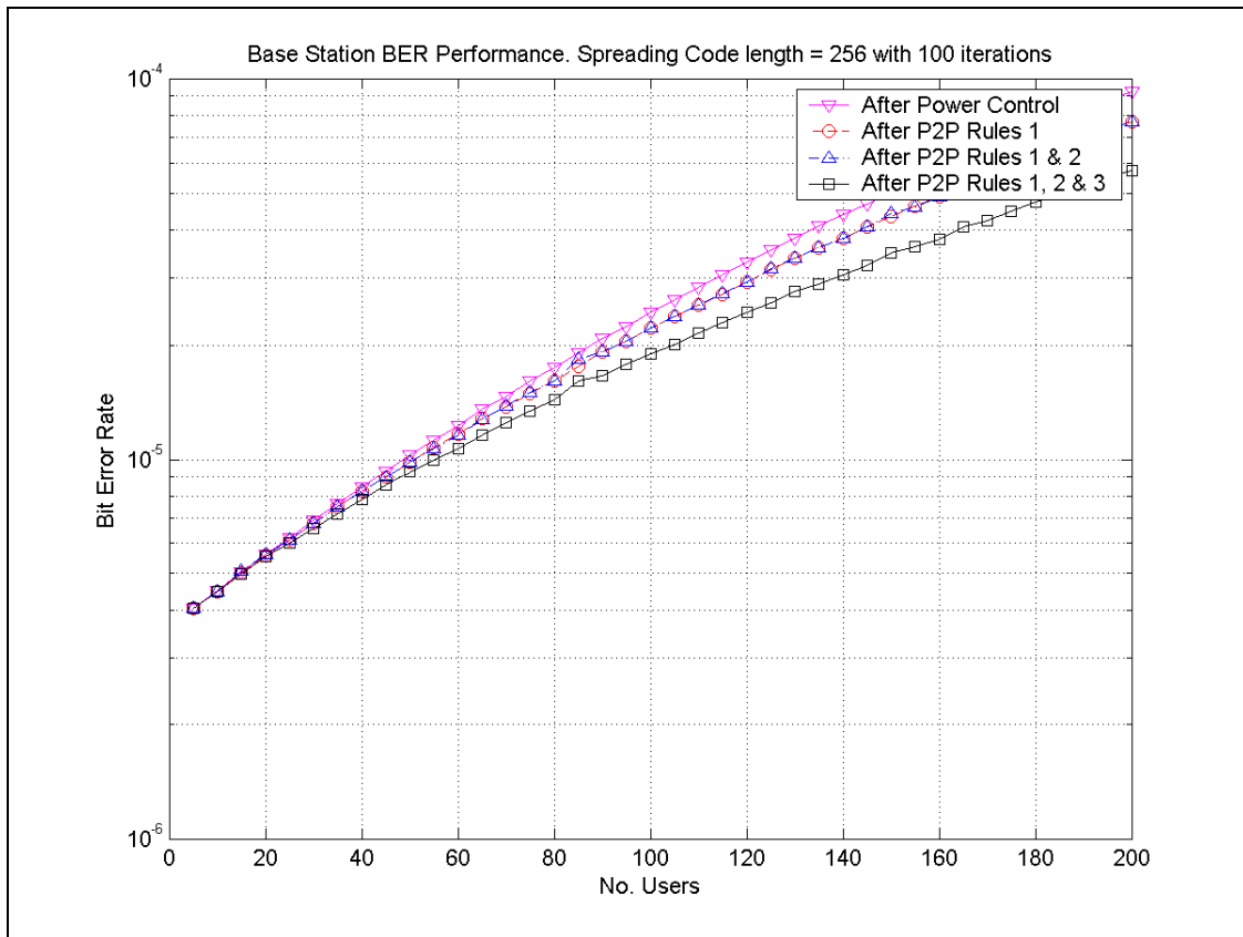
Figure 7.8: Base Station BER Performance
