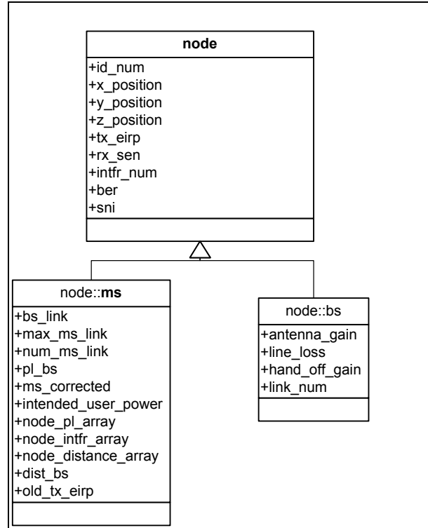
Figure 6.1: Node Class Diagram
