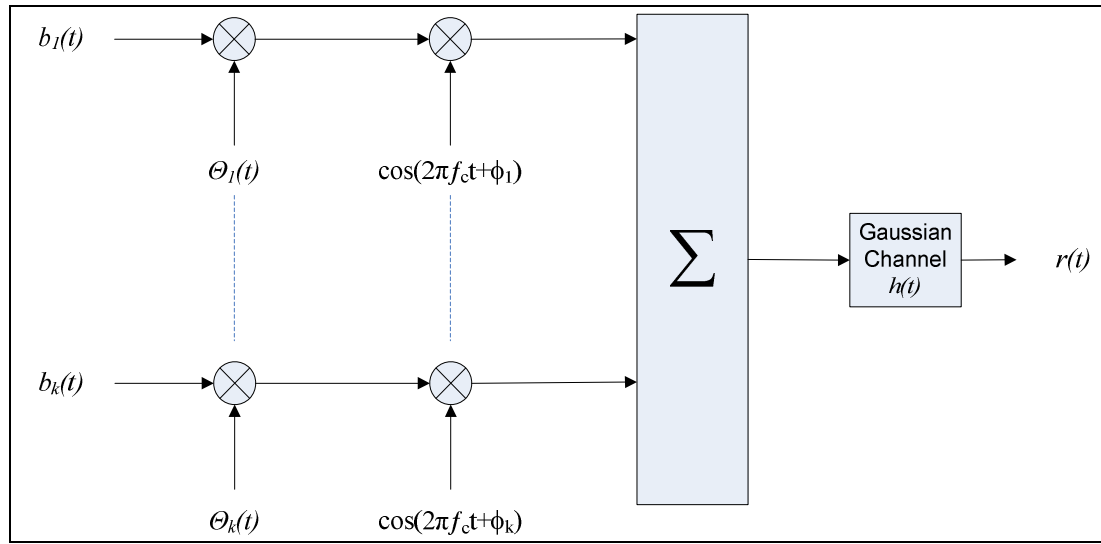
Figure 2.5: Schematic diagram of a DSSS system with k users
