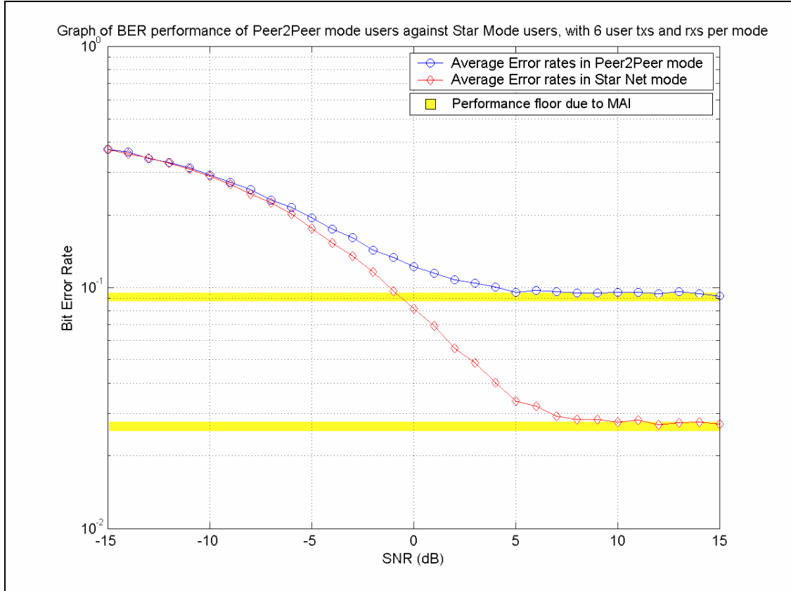
Figure 9.1: BER performance of 6 CDD users against 6 standard users with code length 16
