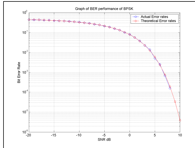
Figure 9.2: Plot of BPSK performance against theoretical error rates
