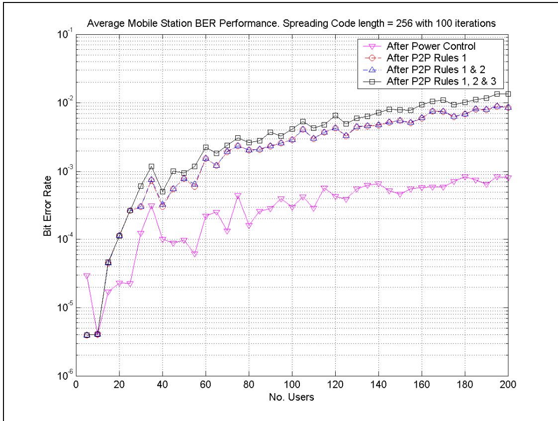
Figure 7.9: MS BER Performance
