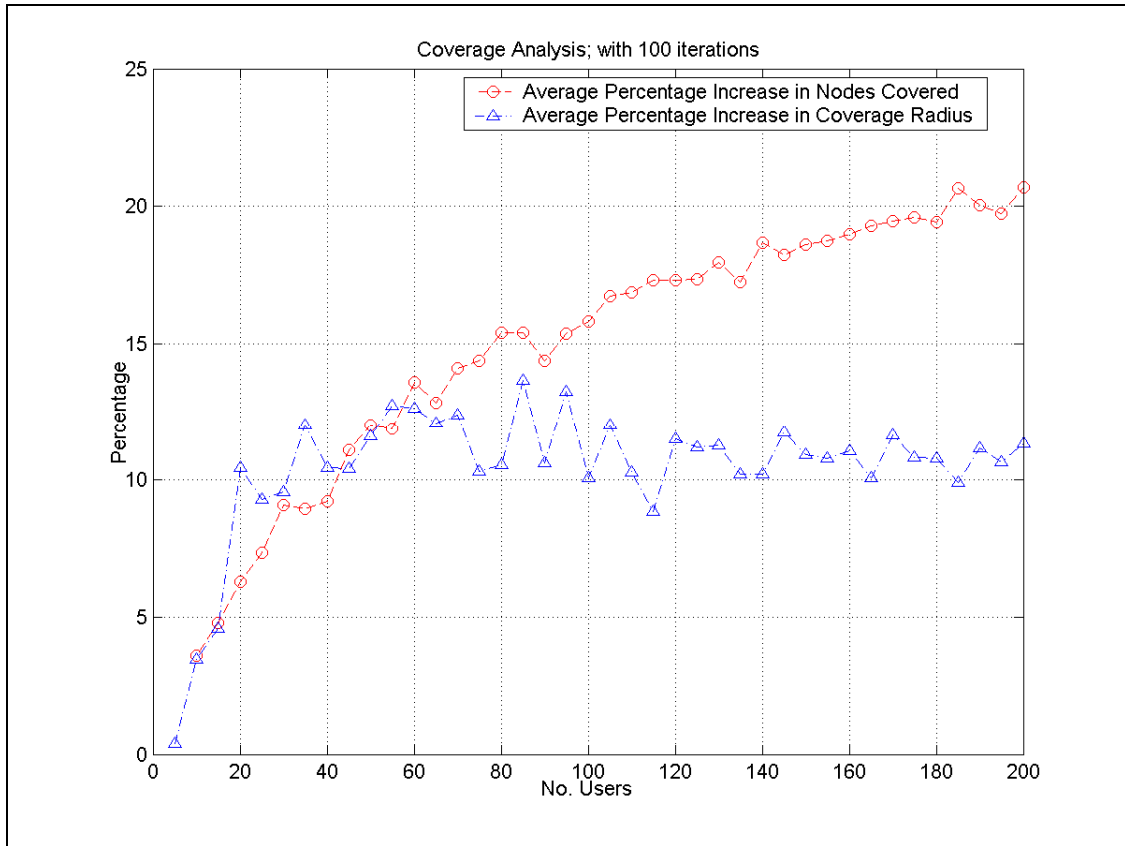
Figure 7.2: Percentage of the Coverage Increase of the Overall Node Population for 1 Slot
