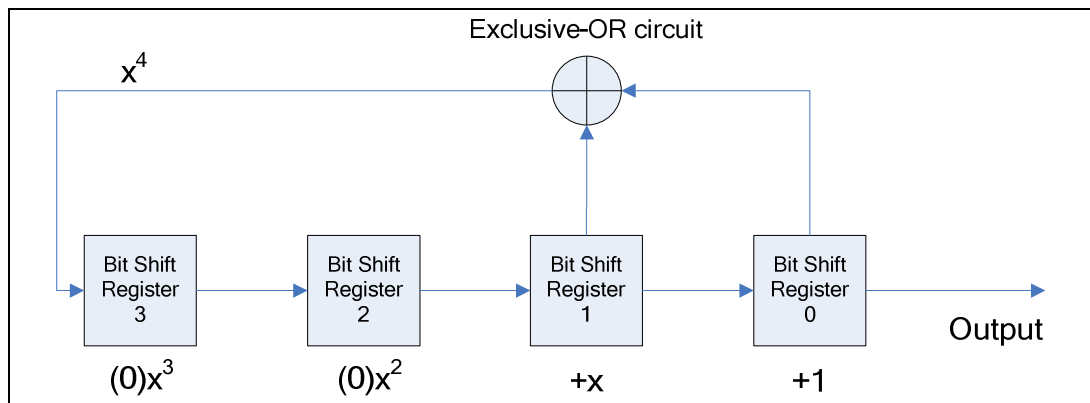
Figure 2.6: Linear Feedback Shift Register Circuit of 4 bits ( x^4+x+1 )
