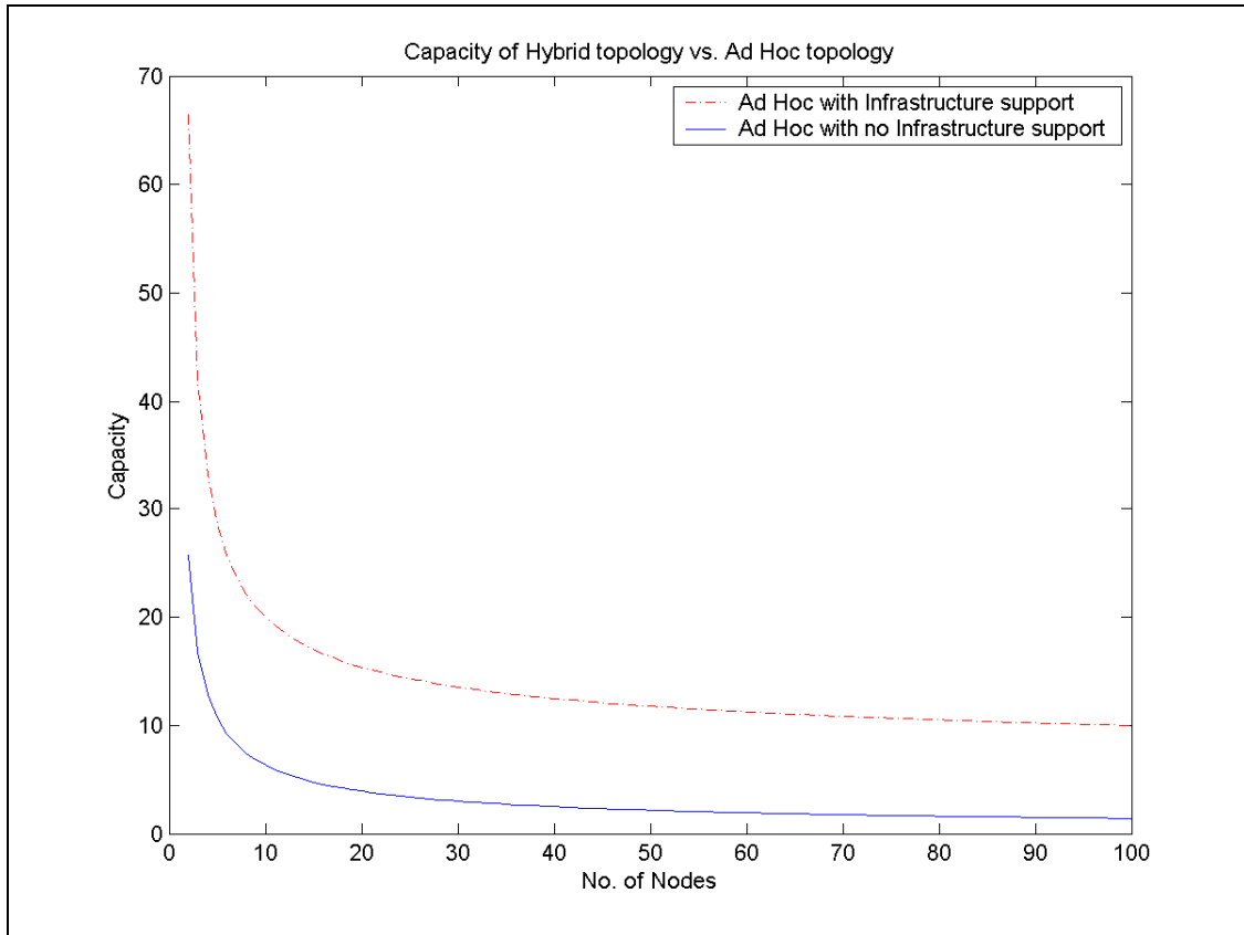
Figure 3.2: Comparison of the Capacity of a Hybrid Topology vs. Ad-hoc Topology with constant band width per node [28]
