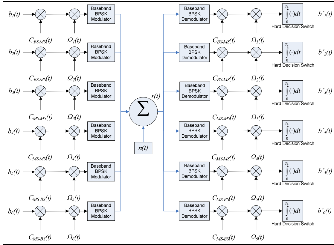
Figure 5.4: Representation of Simulation Environment 1
