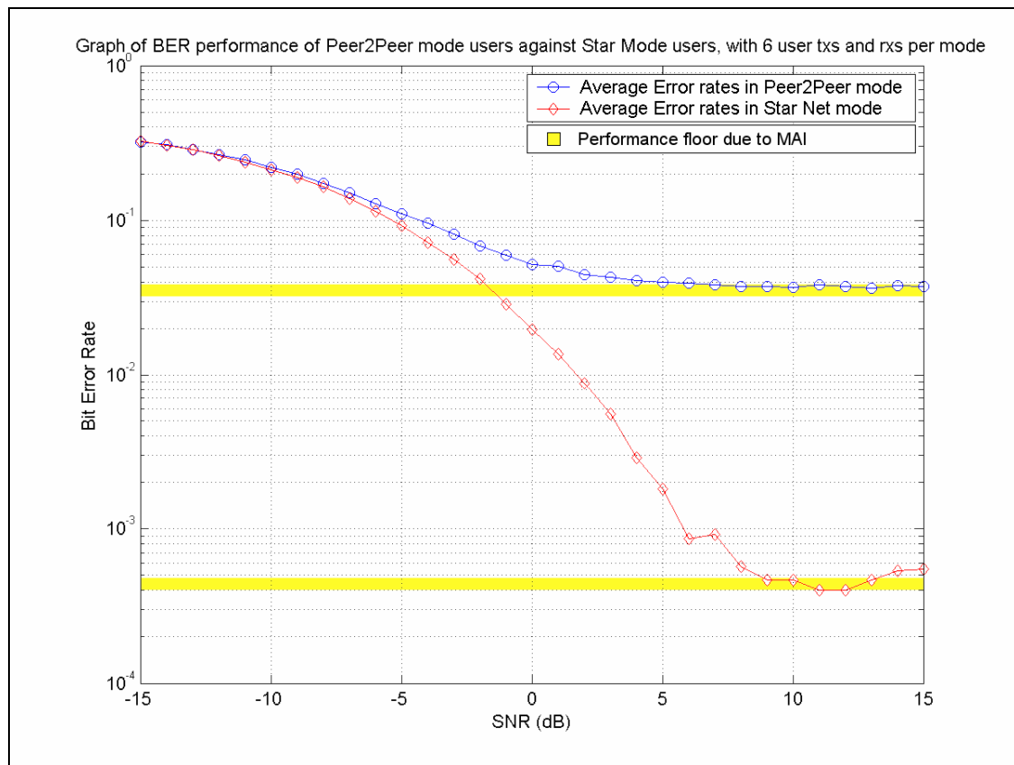
Figure 5.5: BER performance of 6 CDD users against 6 standard users with code length 32
