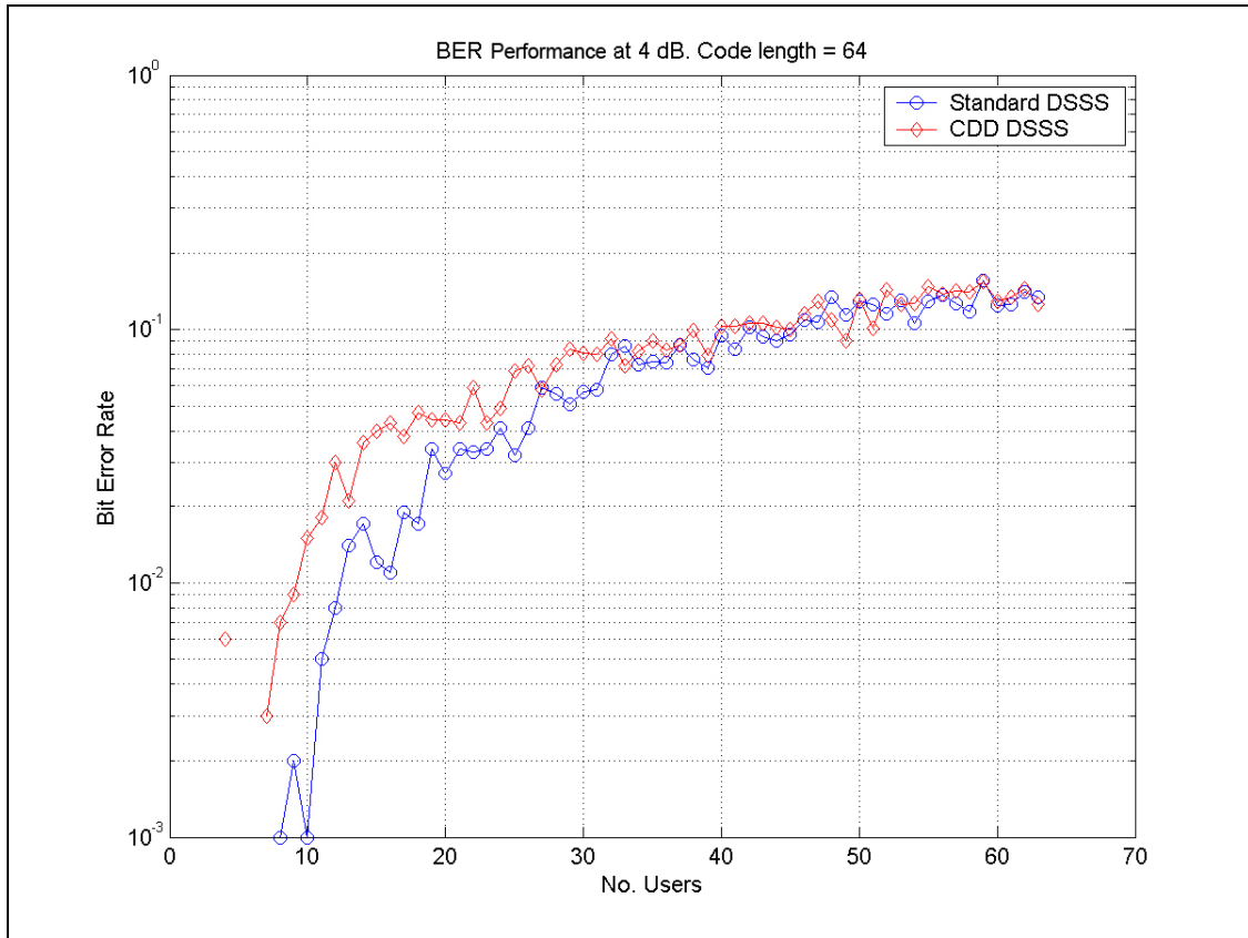
Figure 5.8: Channel Loading Performance of CDD vs. DSSS
