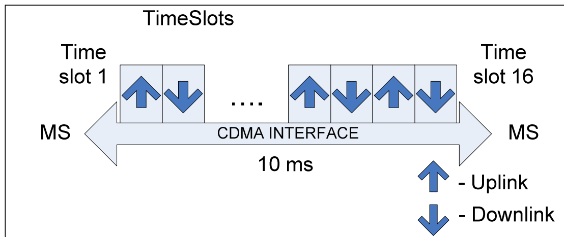
Figure 4.3: Graphical Representation of TDD
