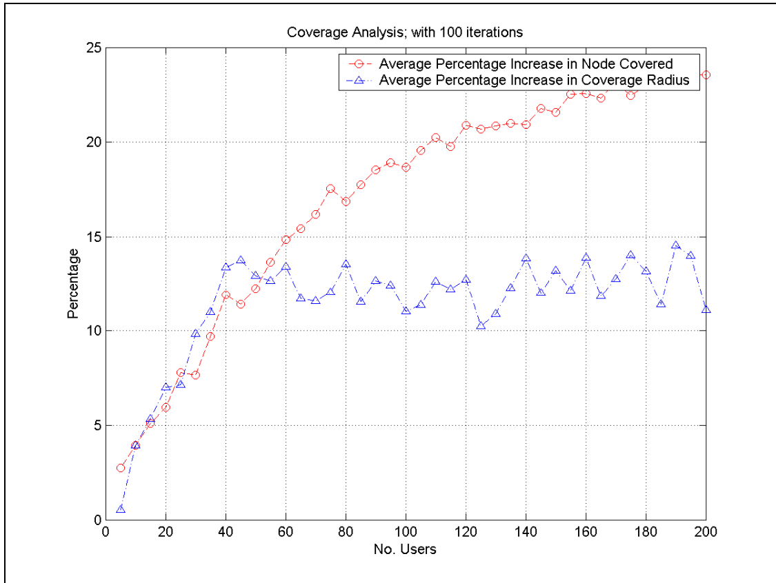
Figure 7.3: Percentage of the Coverage Increase of the Overall Node Population for 2 Slots
