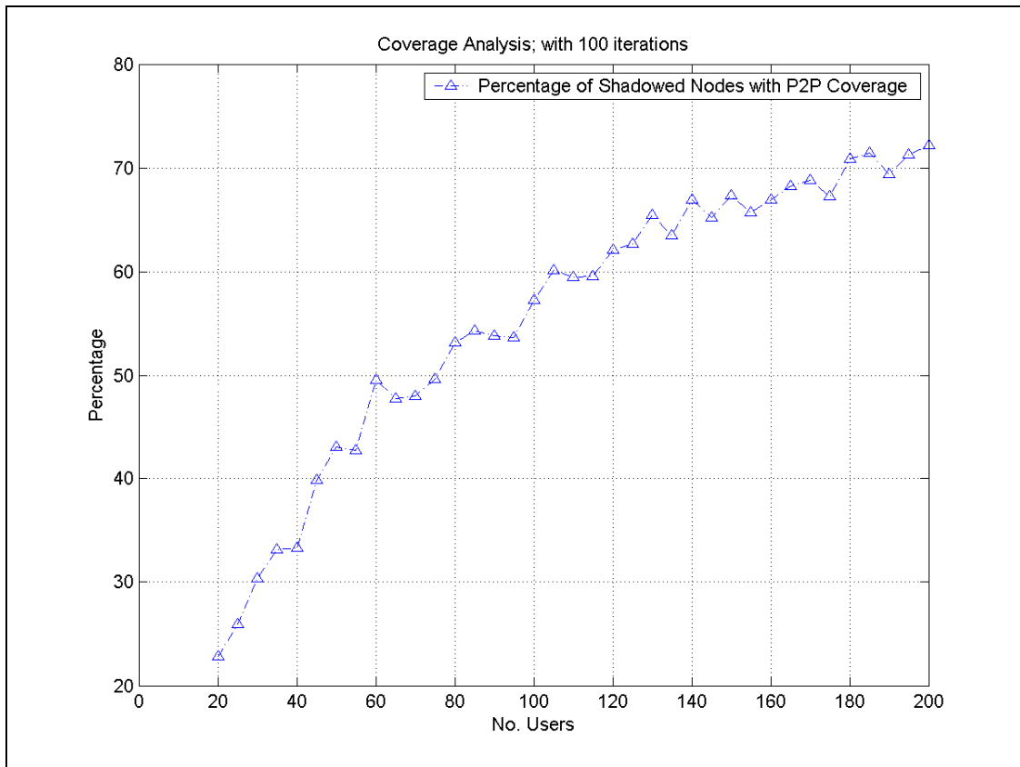
Figure 7.4: Ratio of Shadowed Nodes with Peer-to-peer Coverage to Shadowed Nodes for 1 Slot
