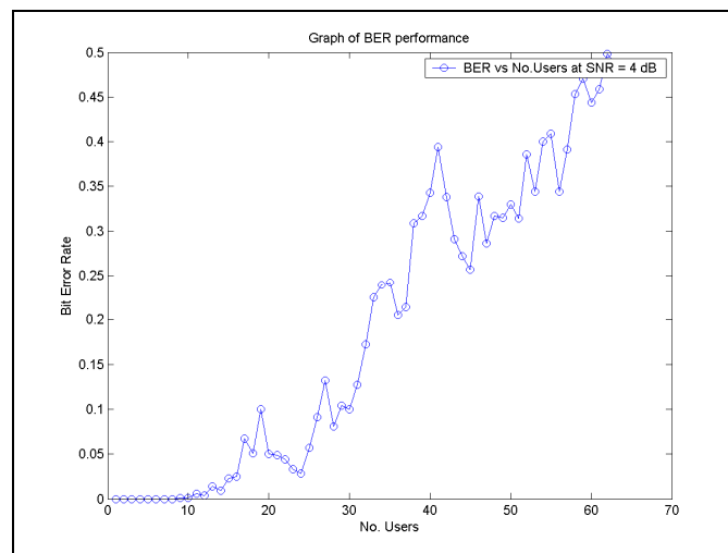
Figure 9.3: DSSS Channel loading test results
