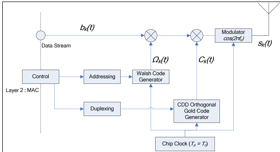
Figure 4.1: MS Transmitter Structure
