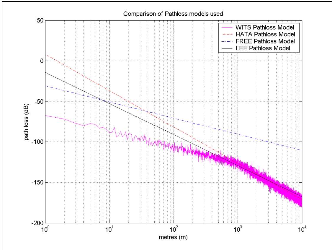
Figure 6.2: Path Loss Model Comparison
