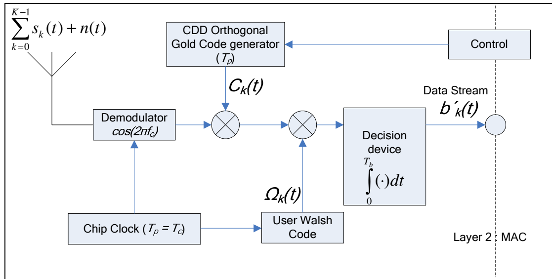
Figure 4.2: MS Receive Structure
