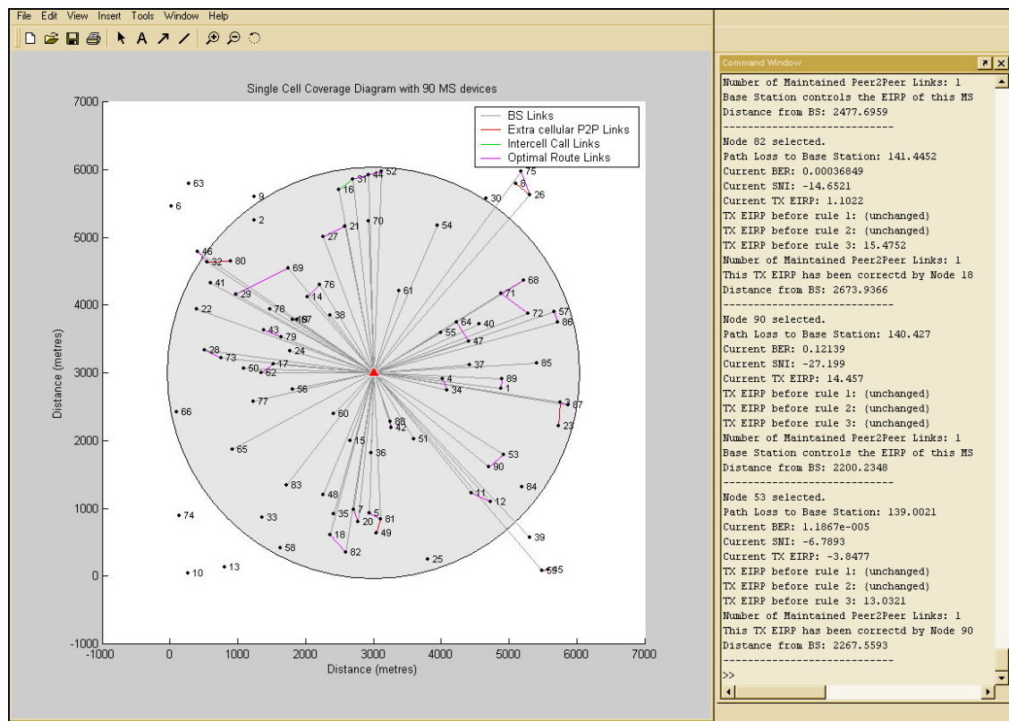
Figure 6.4: Graphical Representation of Simulation Environment
