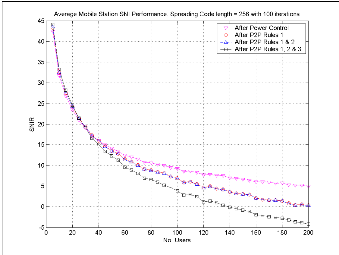
Figure 7.7: Average Mobile SNI Performance for a Single Slot Strategy
