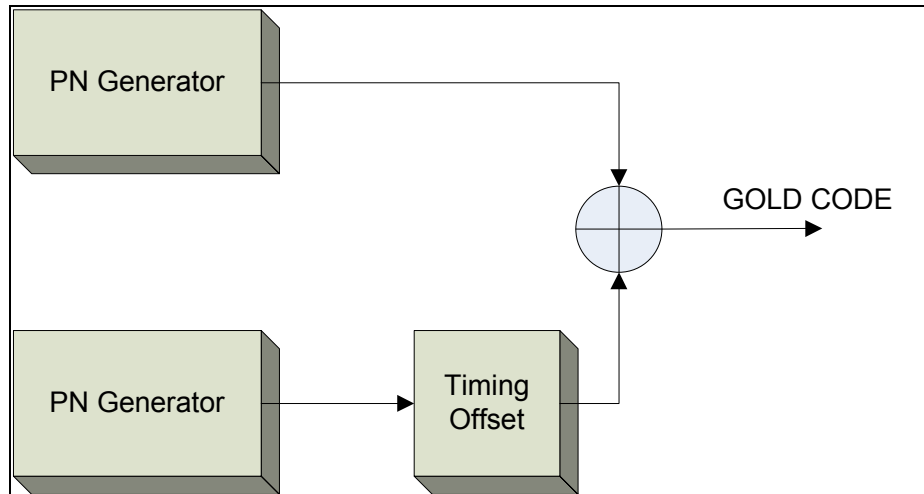
Figure 2.7: Gold Code Sequence Generation
