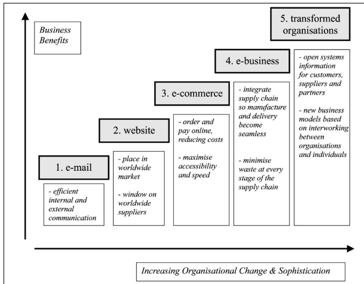
Figure 2: E-Adoption Model
