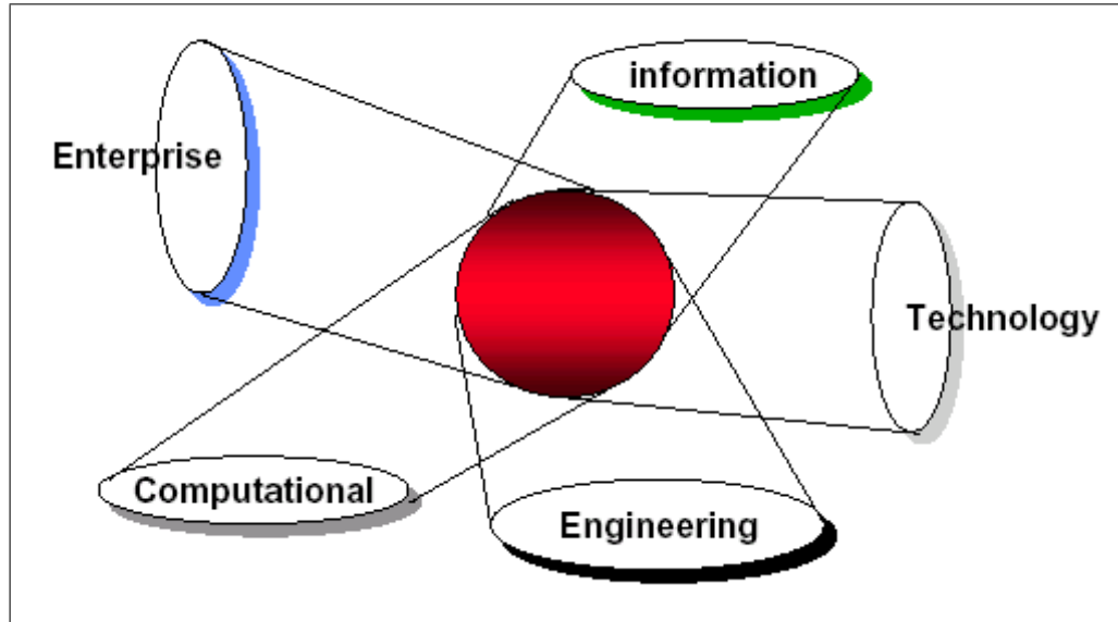
Figure 2.4: RM-ODP Viewpoints [2]
