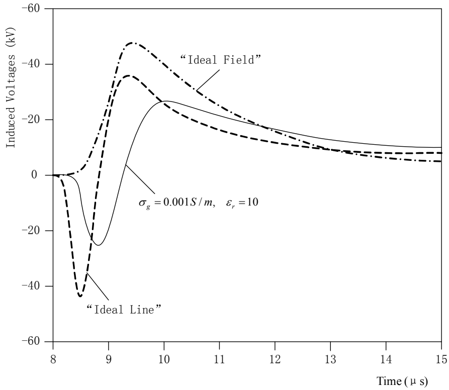
Fig 5.11 Calculated voltages on a 5-km matched overhead line induced by a typical subsequent return stroke. ( \sigma_g = 0.001 \text{ S/m} , \epsilon_r = 10 ).
