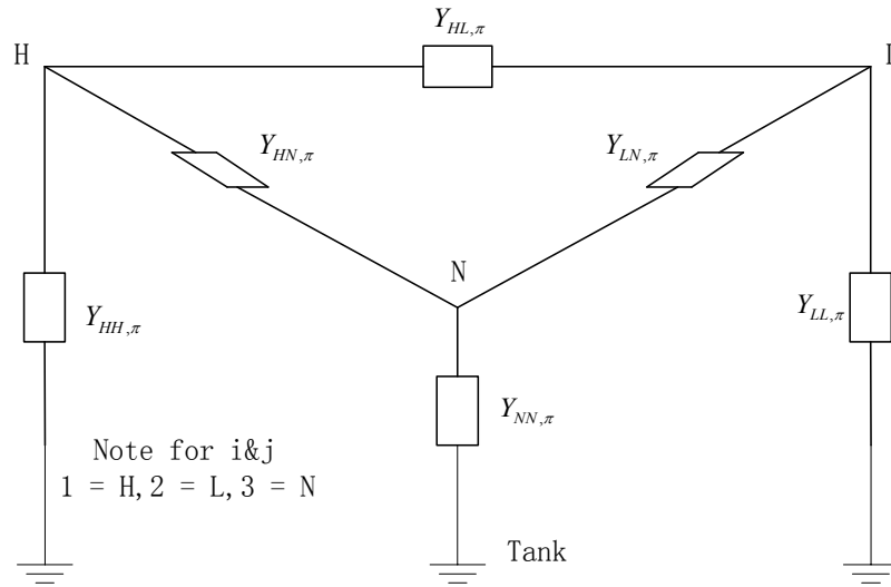
Fig 5.1 Single-line diagram of the multi-terminal \pi -equivalent
