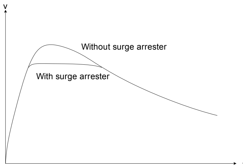
Fig 5.12 The surge characteristic of a ZnO surge arrester
