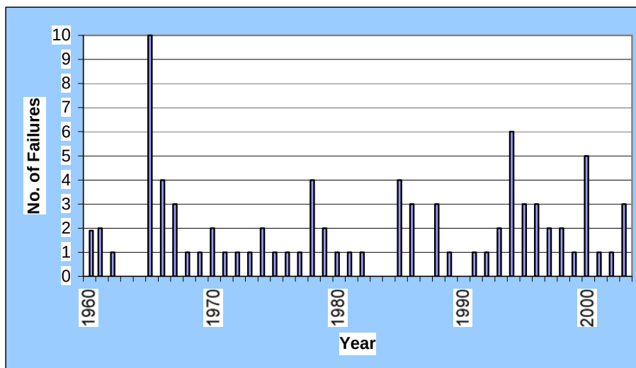
Figure 2.2.1: Number of recorded tailings facility failures since 1960 (Antenna 2004)
