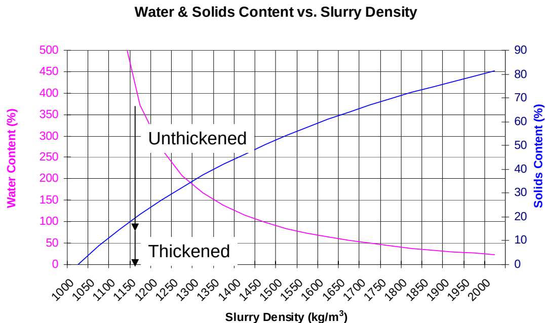
Figure 3.3.7: Water & solids content versus slurry density (specific gravity of 2,7t/m 3 )
