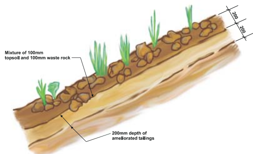
Daggafontein Closure : Optimised surface stabilisation Option 5 : Topsoil, armouring and amelioration
