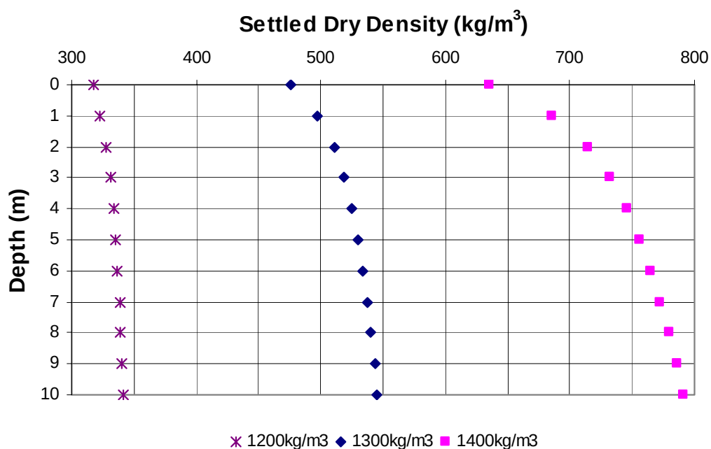
Figure 3.3.8: Slurry dry density versus depth
