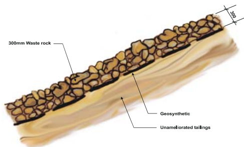
Daggafontein Closure : Surface stabilisation Option 4 : Waste rock cladding
