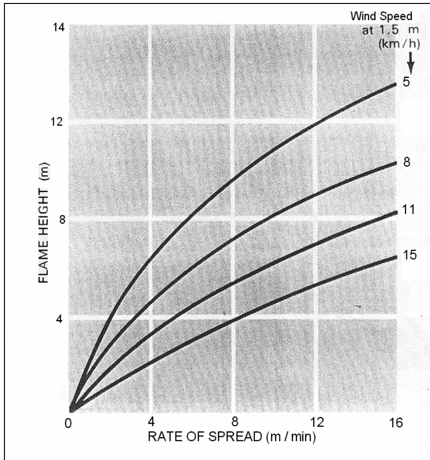
Figure 2.2: The relationship between flame height and rate of spread in dry sclerophyll eucalypt forest 10-15 m high and carrying 20 t/ha of available fuel at various wind speeds (after Luke and McArthur, 1978).
