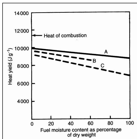
Figure 2.1: The relationship between heat of combustion, moisture content and heat yield in wildland fuel complexes (after Byram, 1959; Bond and Van Wilgen, 1996). Lines A, B, and C show estimates of heat yield for complete combustion, small fires and large fires, respectively.
