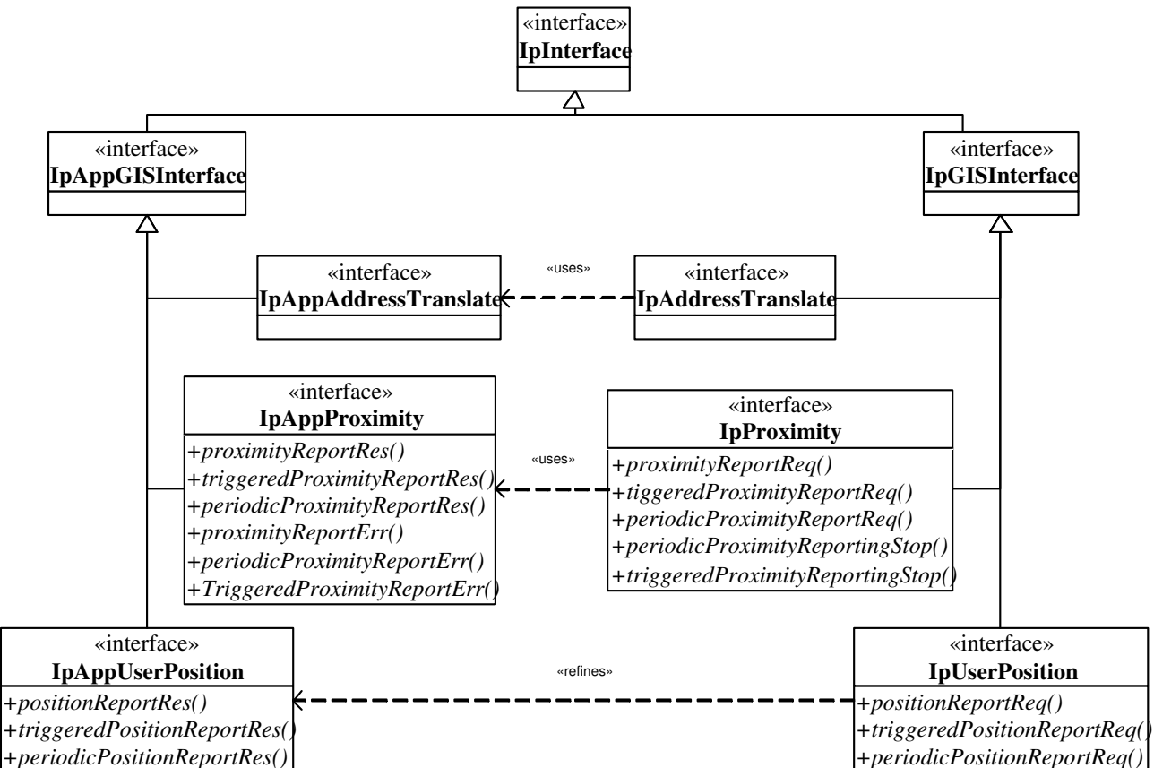
Figure 5.2: Class Diagram
