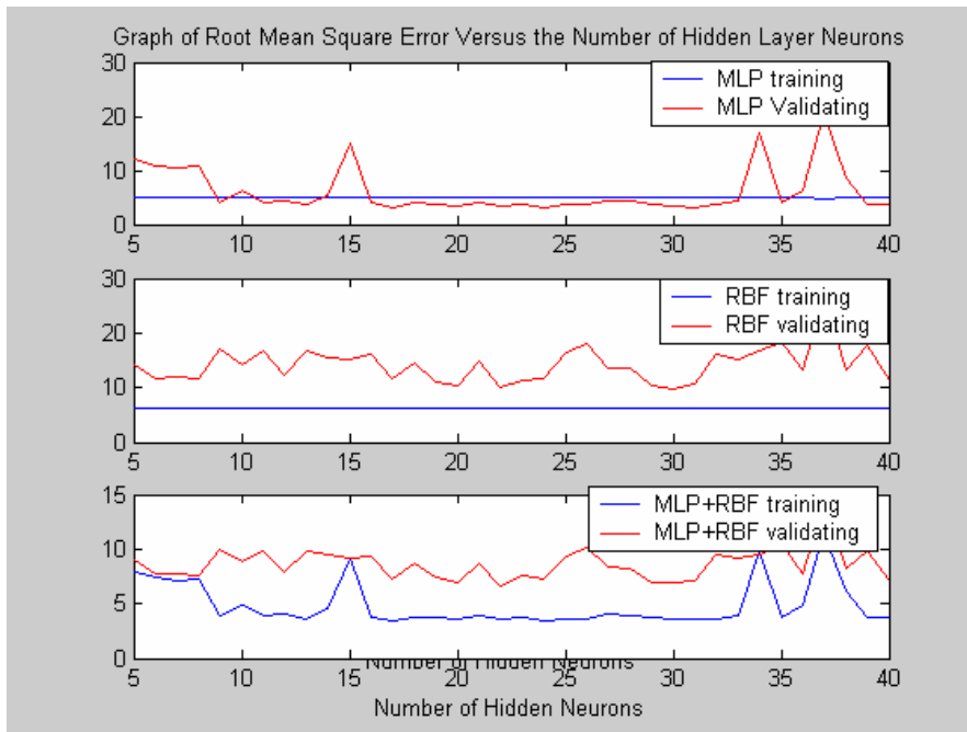
Figure 5: Relationship between RMS error hidden layer neurons for the different architecture types
