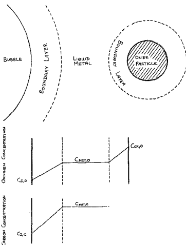
Figure 4.2: Schematic representation of a bubble, an oxide particle and the associated boundary layers and concentration gradients in the Rising Bubble Reaction Zone.
