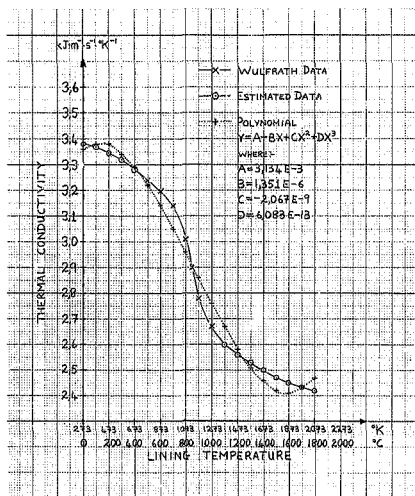
Figure 7.4: Temperature dependence of the thermal conductivity of dolomite bricks
