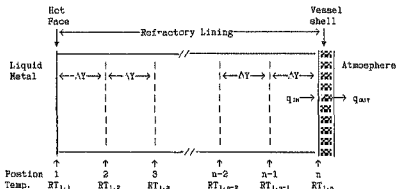
Figure 7.2: Schematic subdivision of vessel lining into incremental distance elements for unsteady state heat flow calculations. Lining temperatures at the start of a process time step and heat fluxes in and out of the vessel shell are shown
