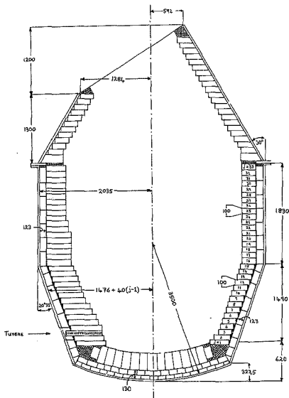
Figure 5.1: Vertical cross section through vessel shell and lining
