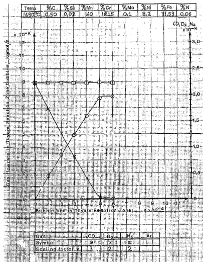
Figure 2.4: Typical Tuyere Reaction Model data in respect of gas flowrates resulting from a 1:1 O 2 /N 2 blowing ratio and an initial 15mm diameter bubble
