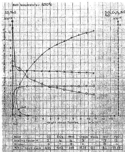
Figure 4.6: Typical Rising Bubble Reaction Model data output in respect of oxide flow rates resulting from a 1:1 \text{O}_2:\text{N}_2 blowing ratio and an initial 15mm diameter bubble at the tuyeres.
