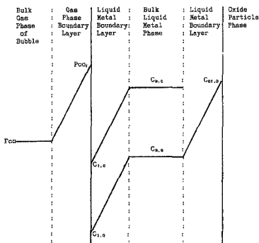
Figure A1: Schematic representation of concentration gradients in the boundary layers at the metal/gas interface of a bubble and the metal/oxide interface of an oxide particle
