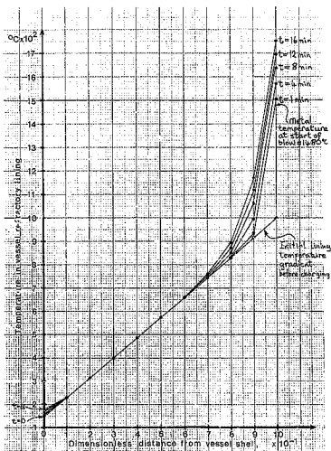
Figure 7.5: Calculated temperature profile development in a new refractory lining.
