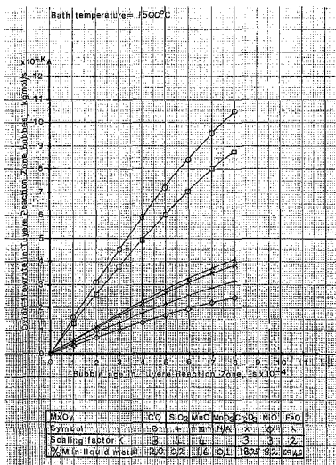
Figure 2.3: Typical Tuyere Reaction Model data in respect of oxide flow rates resulting from a 3:1 O 2 :N 2 blowing ratio and an initial 15mm diameter bubble
