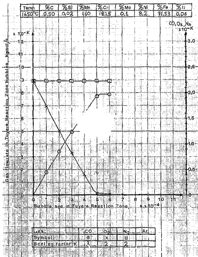
Figure 2.4: Typical Tuyere Reaction Model data in respect of flowrates resulting from a 0.1% blowing ratio and an initial 15mm diameter bubble
