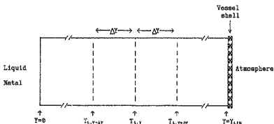
Figure 7.1: Finite element model of temperature distribution and heat flow through the refractory lining
