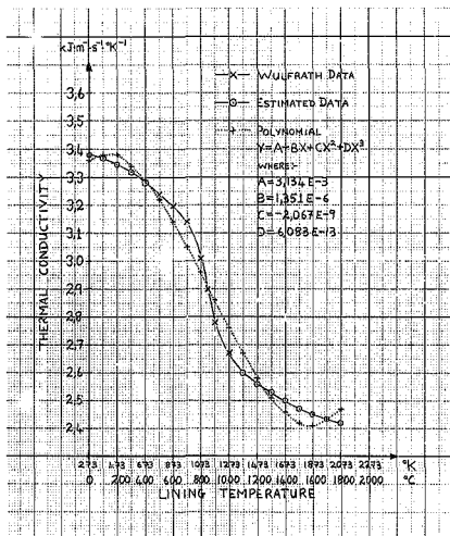
Figure 7.4: Temperature dependence of the thermal conductivity of dolomite bricks
