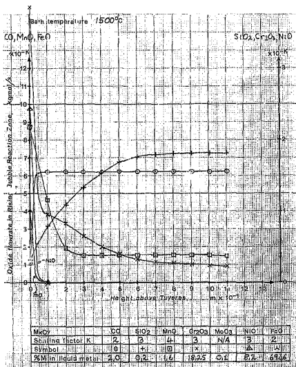
Figure 4.4: Typical Rising Bubble Reaction Model data output in respect of oxide flowrates resulting from a 3:1 O 2 /N 2 blowing ratio and an initial 15mm diameter bubble at the tuyere.
