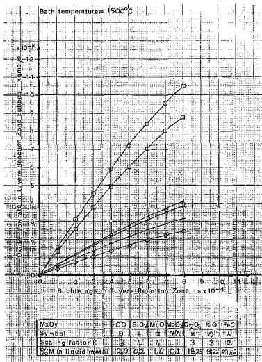
Figure 2.3: Typical Tuyere Reaction Model data in respect of oxide flowrates resulting from a 3:1 O 2 :N 2 blowing ratio and an initial 15mm diameter bubble
