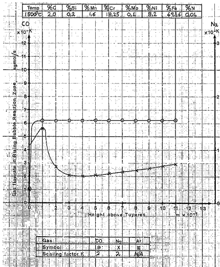
Figure 4.3: Typical Rising Bubble Reaction Model data output in respect of gas flowrates resulting from a 3:1 O 2 /N 2 blowing ratio and an initial 15mm diameter bubble at the tuyeres.
