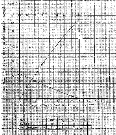
Figure 2.2: Typical Tuyere Reaction Model data in respect of gas flowrates resulting from a 3:1 O 2 :N 2 blowing ratio and an initial 15mm diameter bubble
