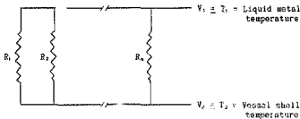
Figure 6.2: Resistance analogue of heat flow through refractory lining
