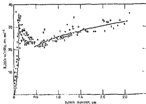
Figure 3.3. Rising velocity of single bubbles in water
