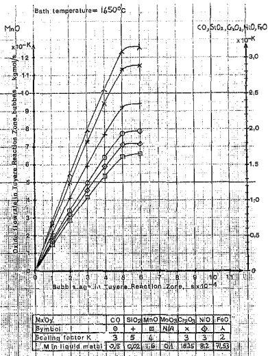
Figure 2.5: Typical Tuyere Reaction Model data in respect of oxide flow rates resulting from a 1:1 O 2 :N 2 blowing ratio and an initial 15mm diameter bubble
