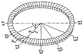
Figure 6.3: The n 'th brick course of the vessel lining
