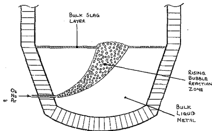
Figure 4.1: Schematic representation of the Rising Bubble Reaction Zone.
