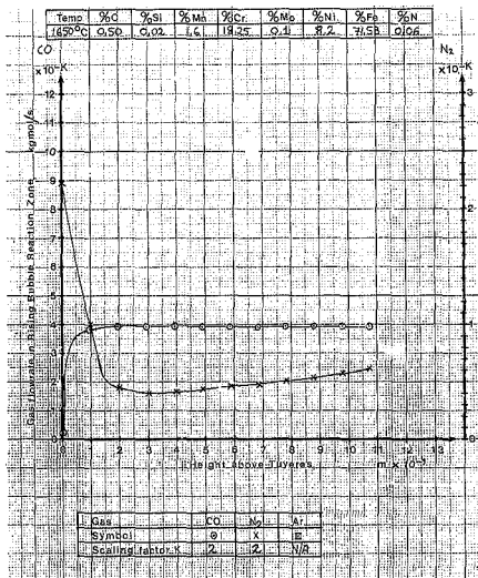
Figure 4.5: Typical Rising Bubble Reaction Model data output in respect of gas flowrates resulting from a 1:1 O 2 :N 2 blowing ratio and an initial 15mm diameter bubble at the tuyeres.
