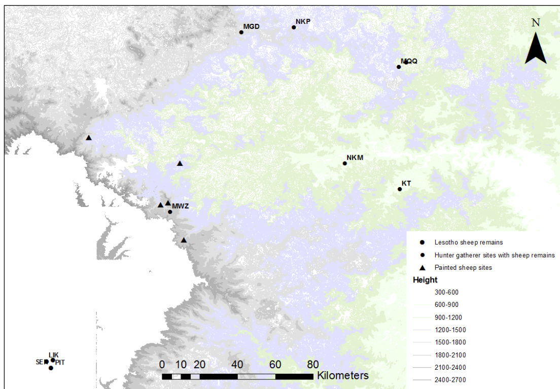
Figure 2.2: The spatial and temporal distribution of hunter-gatherer sites containing sheep remains in Lesotho and the Thukela Basin, KwaZulu-Natal. Full site names can be found in Appendix A (pg 222 & 223).
