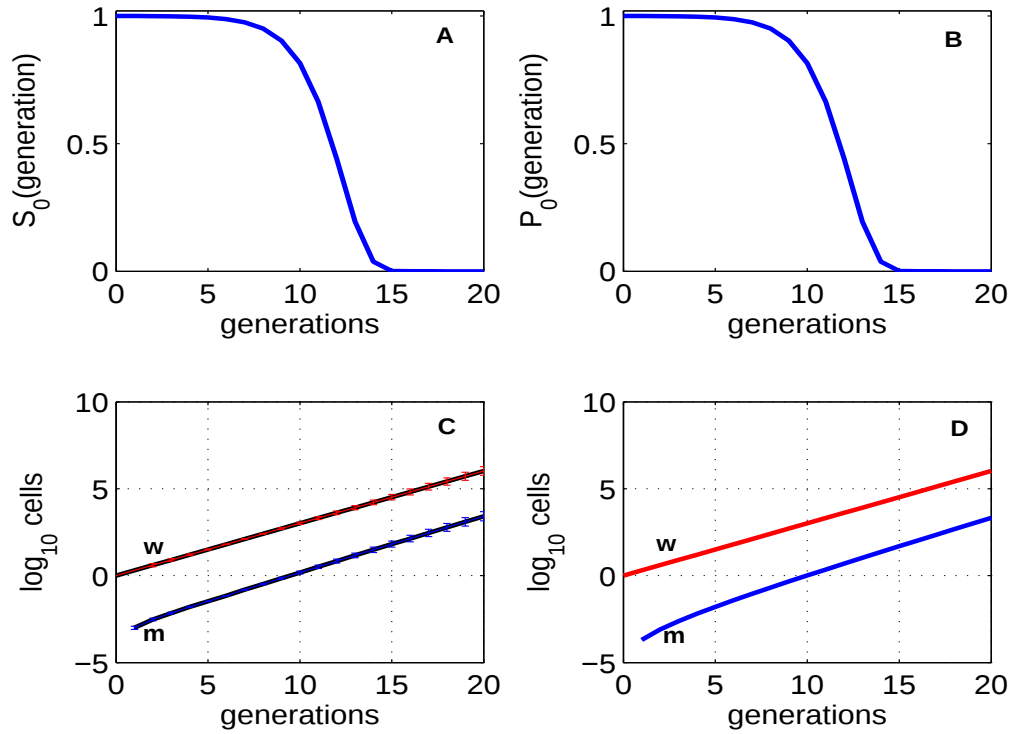
Figure 2.7: The probability that the mutant has never occurred (A) and (B) the probability that the mutant is not currently present in the population. (C) Average cell counts (wild-type (w) and mutant (m)) of 1000 runs of the branching process, started by a single wild-type infected cell (with 95% confidence intervals) and (D) the expected cell counts given by the formulas for R_0 = 2 , mutation rate \eta = 10^{-4} . The simulations and the formulas give the same result.
