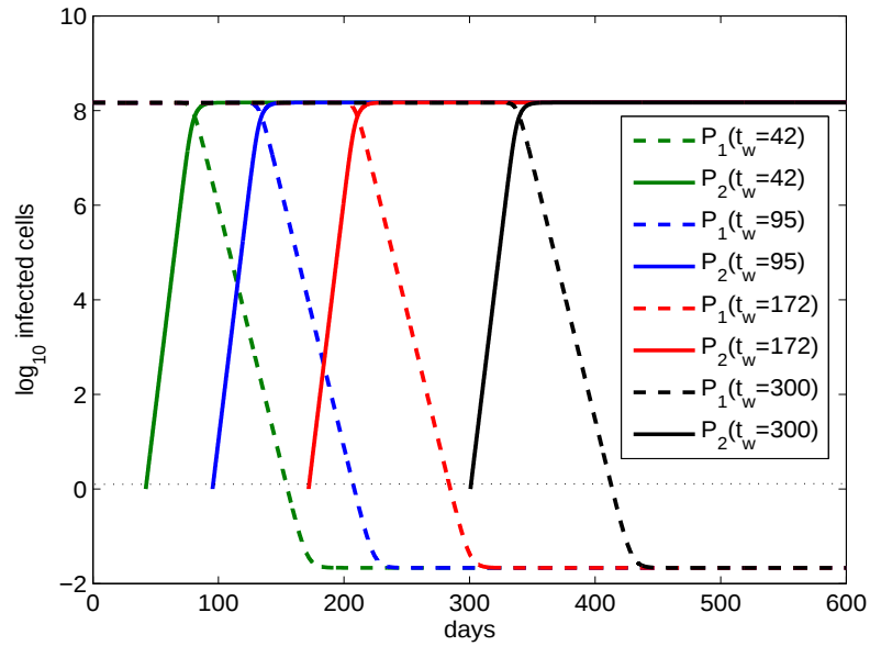
Figure 2.3: Growth of mutant strain including pseudo sampled waiting times. The times ( < t_w > ) chosen are 42, 95, 172 and 300 which are chosen so that there are spaced inversely proportional to the probability density. The other parameter values are as in figure 2.1 and k_2 = 1.5k_1 .
