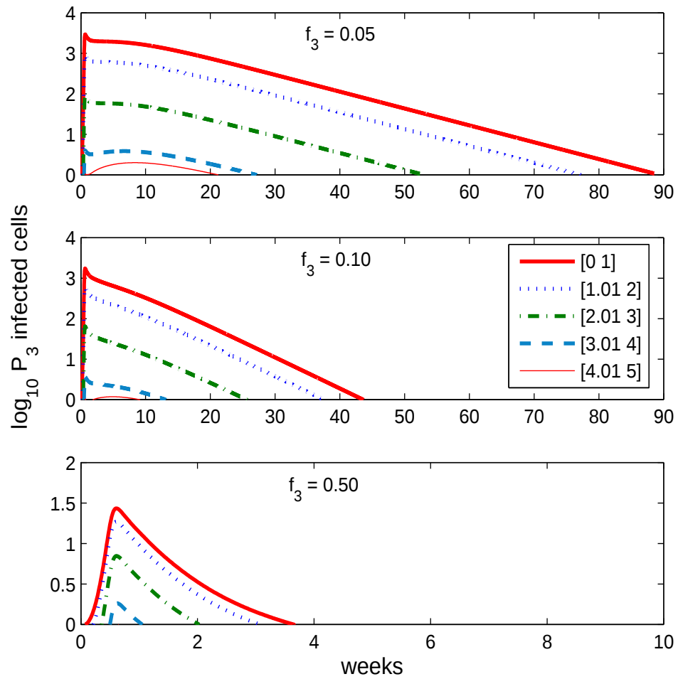
Figure 5.4: Dynamics of the rare mutant with 5%, 10% and 50% fitness cost relative to the wild-type strain that gets produced at the centre of the intervals [0, 1] , [1, 2] , [2, 3] , [3, 4] and [4, 5] . The other parameter values are as in figure 5.2.
