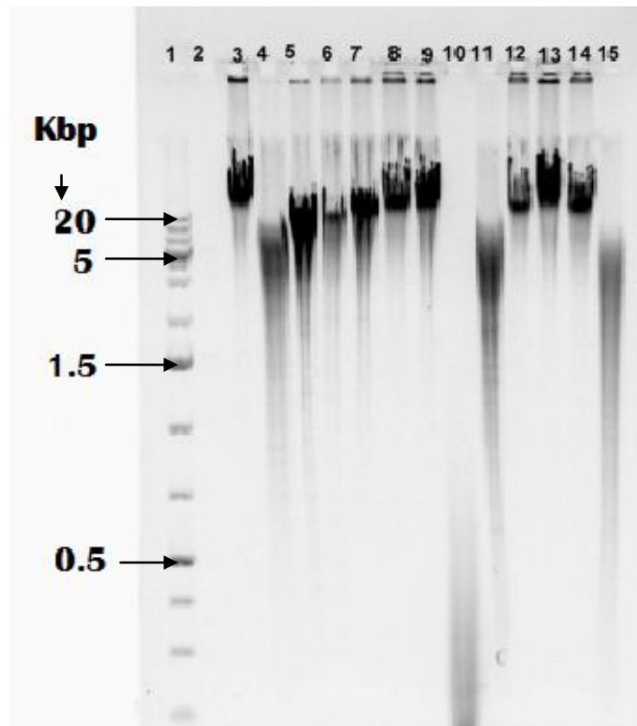
Figure 6: Determination of the restriction enzyme to be used for library construction; electrophoresed on a 0.4% agarose gel. M. smegmatis 43756Km1 after digestion with X MA II ( Lane 4 ), Bam HI ( 5 ), Bgl II ( 6 ), Hind III ( 7 ), Sau 3A ( 8 ), Nhe I ( 9 ), Nsi I ( 10 ), Pst I ( 11 ), Sfu I ( 12 ), Xba I ( 13 ), Xho II ( 14 ), Xmi I ( 15 ). Lane 1 – molecular weight marker, Lane 3 – undigested DNA.
