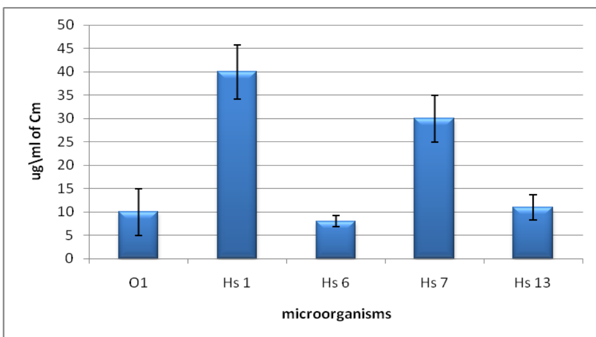
Figure 11: Determination of chloramphenicol MICs of Rhodococcus strains.
