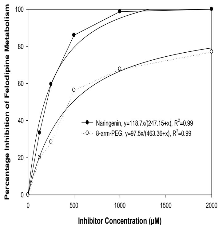
Figure 5.8: The influence of naringenin and 8-arm-PEG on intestinal tissue metabolism of felodipine (N=3; S.D.<0.01 in all cases).
