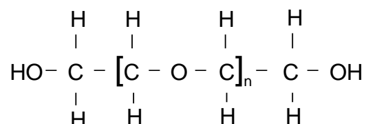
Figure 5.1: The molecular structure of poly(ethylene glycol).
