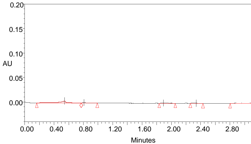
Figure 5.10: A typical UPLC chromatogram obtained from felodipine-free pig plasma.
