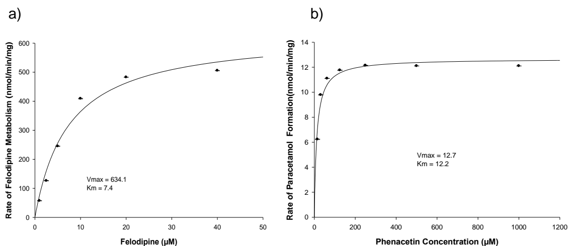
Figure 3.9: Michaelis-Menten Plot depicting the enzyme kinetic parameters of a) CYP3A4-catalyzed felodipine metabolism and b) CYP1A2-catalyzed phenacetin o-deethylation generated by Enzyme Kinetic Software (SigmaPlot: Enzyme Kinetic Module) (N=3; S.D.<0.005 in all cases).
