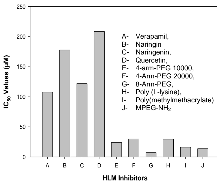
Figure 4.5: Comparison of the potencies of the investigated MPCIs.
