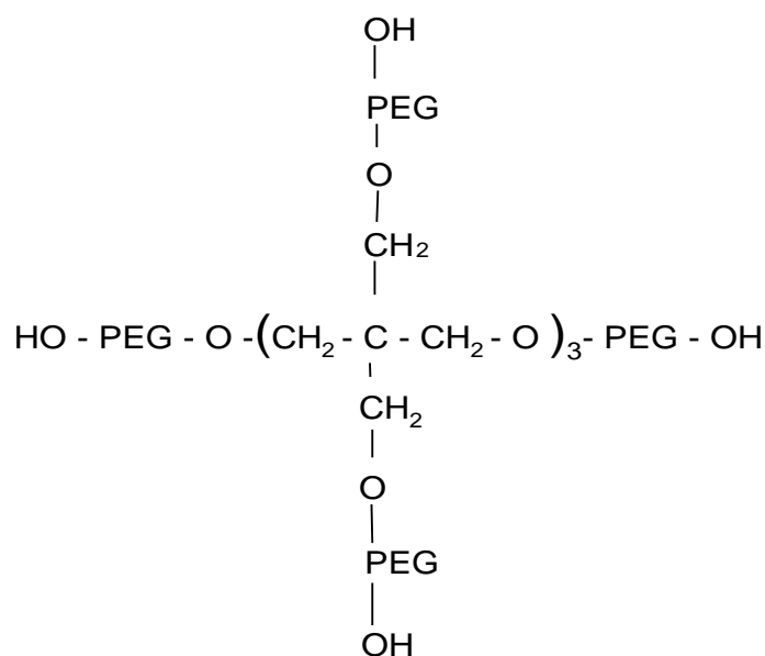
Figure 5.2: The molecular structure of 8-arm-PEG.
