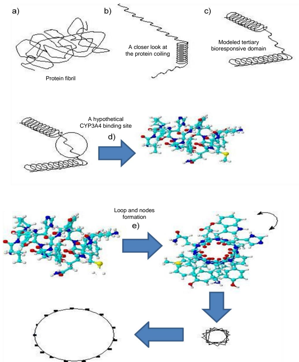
Figure 4.3: Computational models showing the molecular structure of the bio-reactive sites of CYP3A4, with a) protein fibril; b) a closer look at protein coiling; c) tertiary structural and bioresponsive domain for biomimetic activity; and d) the arrow represents hypothetical binding site on the 3-dimensional protein structure (e) with loop and nodes formation.
