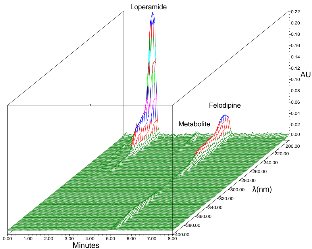
Figure 3.3: UPLC chromatograms showing the retention time of felodipine (5.037 minutes), the appearance of its metabolite (3.542 minutes) and the internal standard (1.434 minutes).
