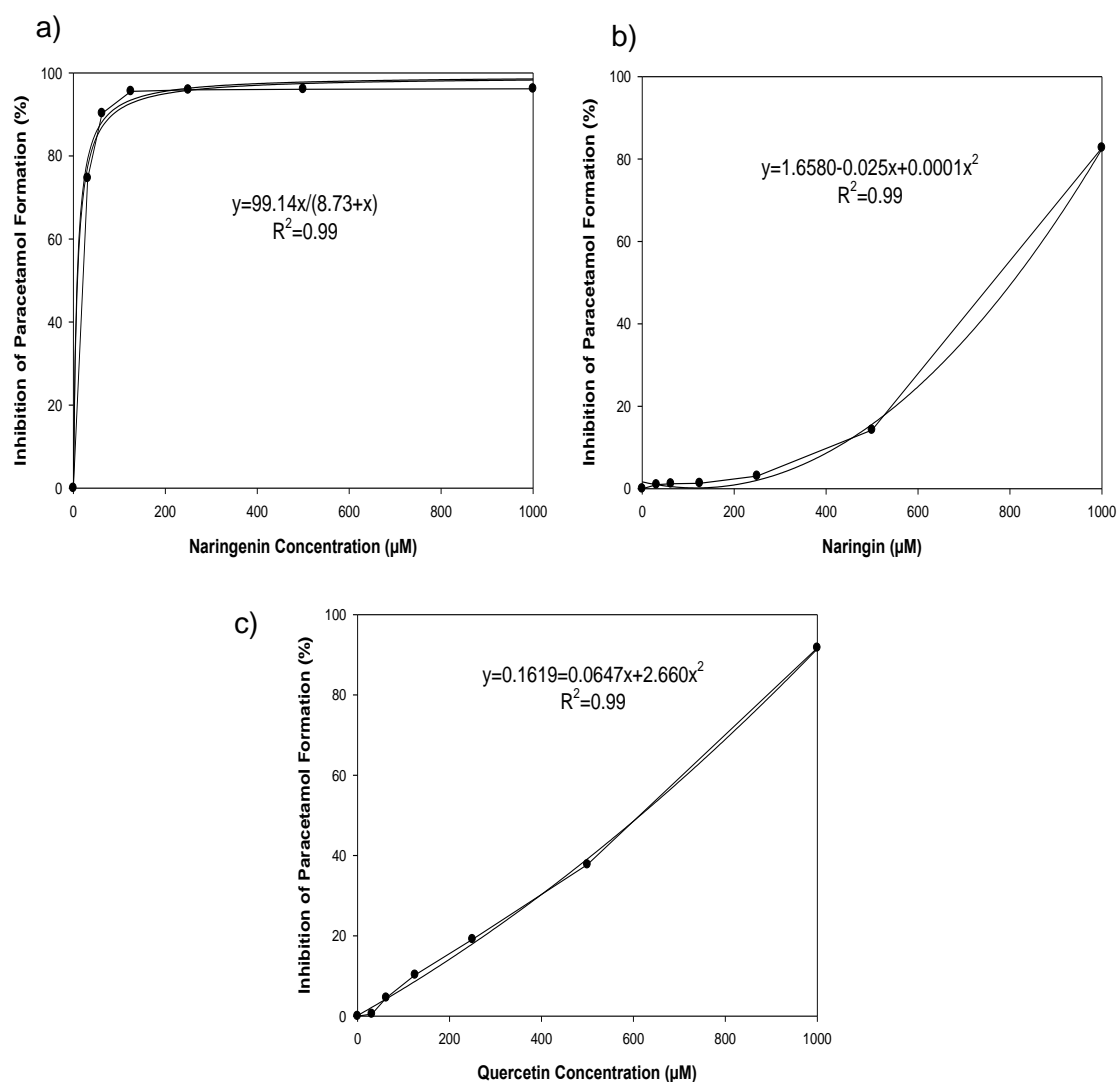
Figure 3:13: The effects of varying concentrations of a) naringenin, b) naringin and c) quercetin, on phenacetin metabolism by HLM (N=3; S.D.<0.005 in all cases).
