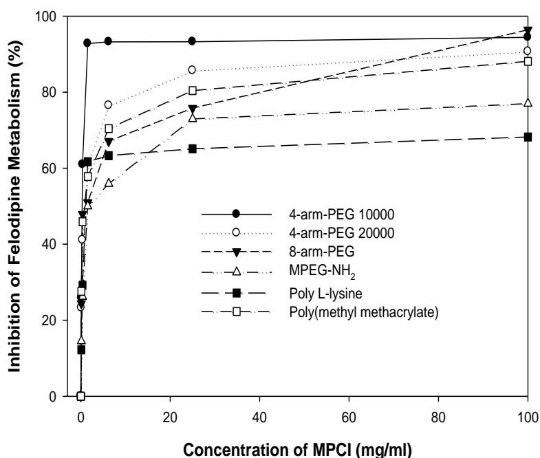
Figure 4.4: The inhibitory effects of the Modeled Pre-systemic Cytochrome P450 3A4 Inhibitors on the CYP3A4-catalyzed felodipine metabolism (N=3; S.D.<0.005 in all cases).
