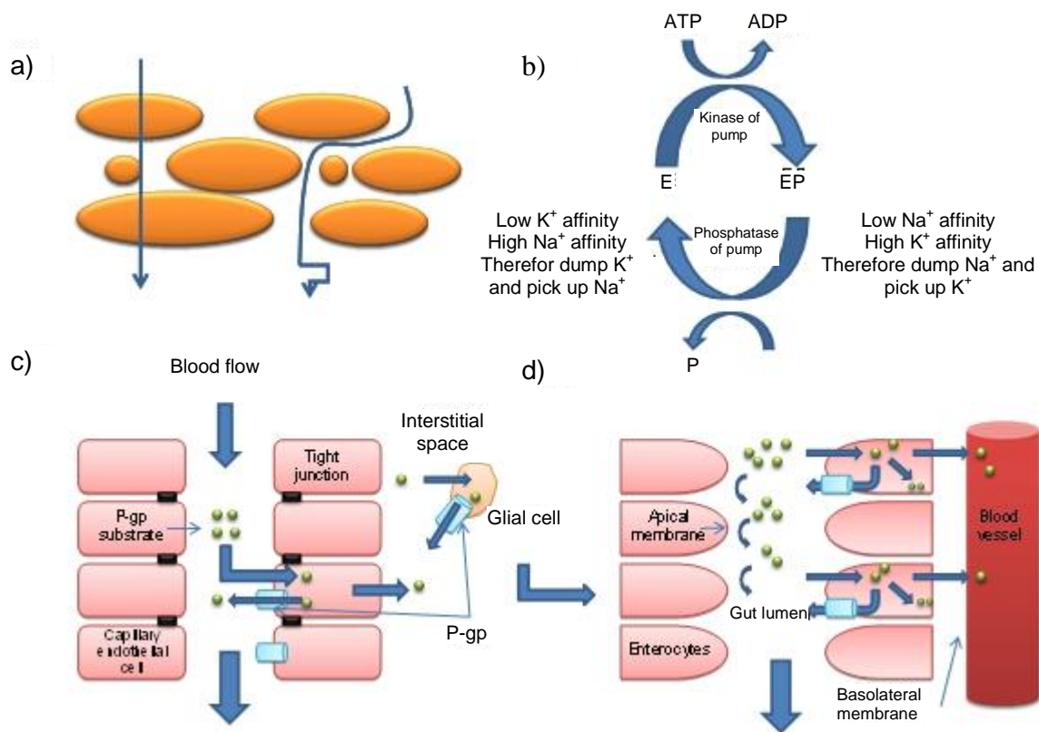
Figure 2.3: A schematic depicting the a) transcellular and paracellular transport routes b) active transport c) passive transport and d) facilitated transport of compounds across the GIT lumen (Adapted from: Matheny et al., 2009).
