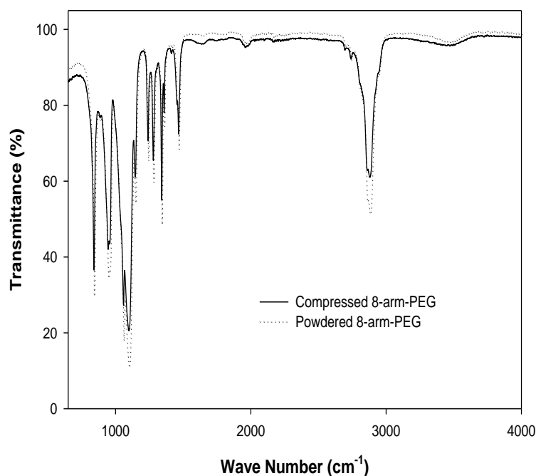
Figure 5.6: FTIR spectra of powdered and compressed 8-arm-PEG generated.
