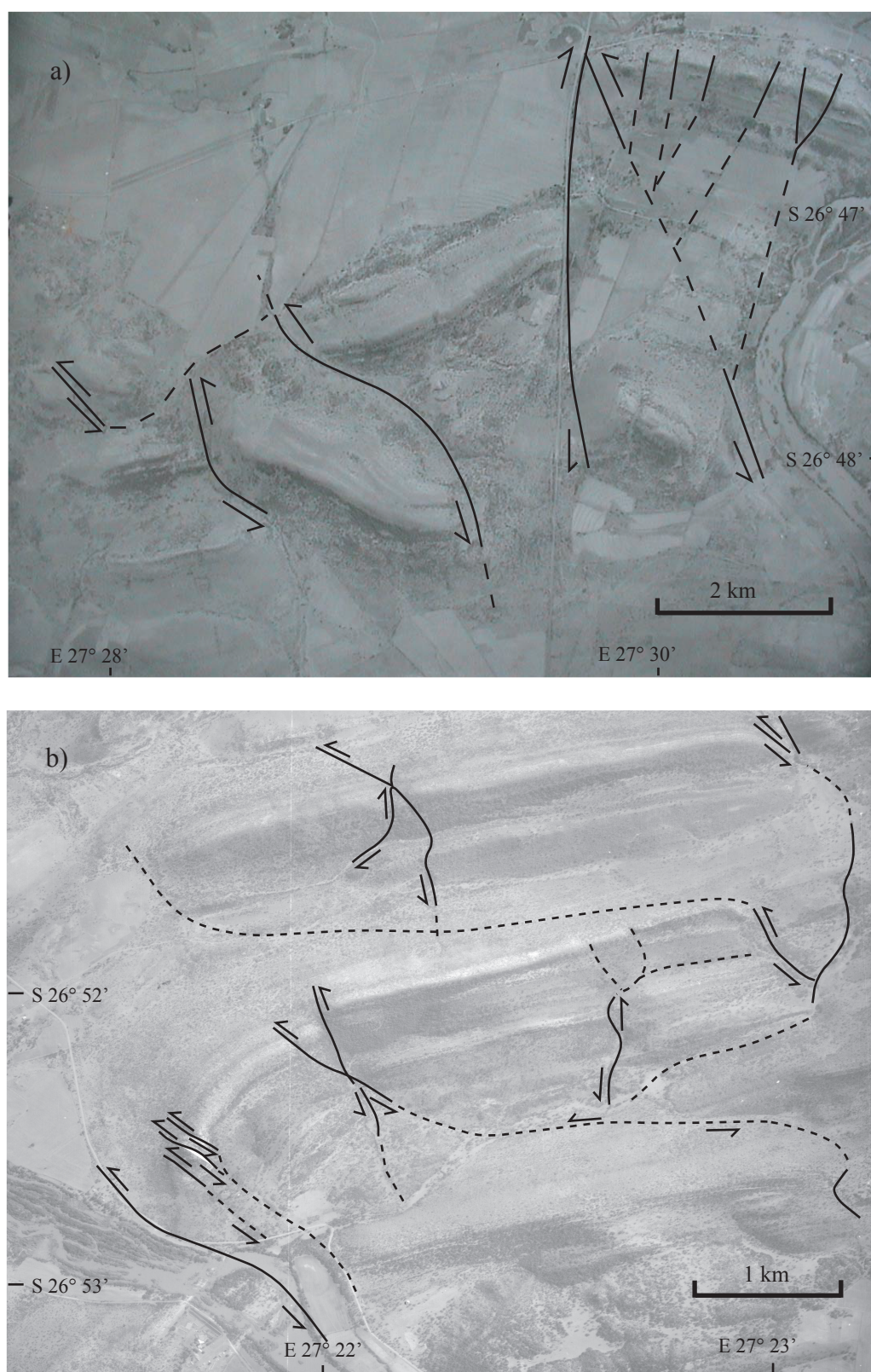
Fig. 2.20: (a) Large-scale faults with radial and tangential strike orientations and displacements of hundreds of metres indicated by displaced West Rand Group quartzites. Fault traces confirmed by surface mapping are shown with solid lines, inferred faults are shown with dashed lines. See text for further detail. (b) Example of a homoclinal, asymmetric fold (fold E) in the northern part of the collar (see Fig. 2.16), which is associated with large-scale, radial faults. These faults are shown by solid lines where their existence was confirmed by surface mapping.
