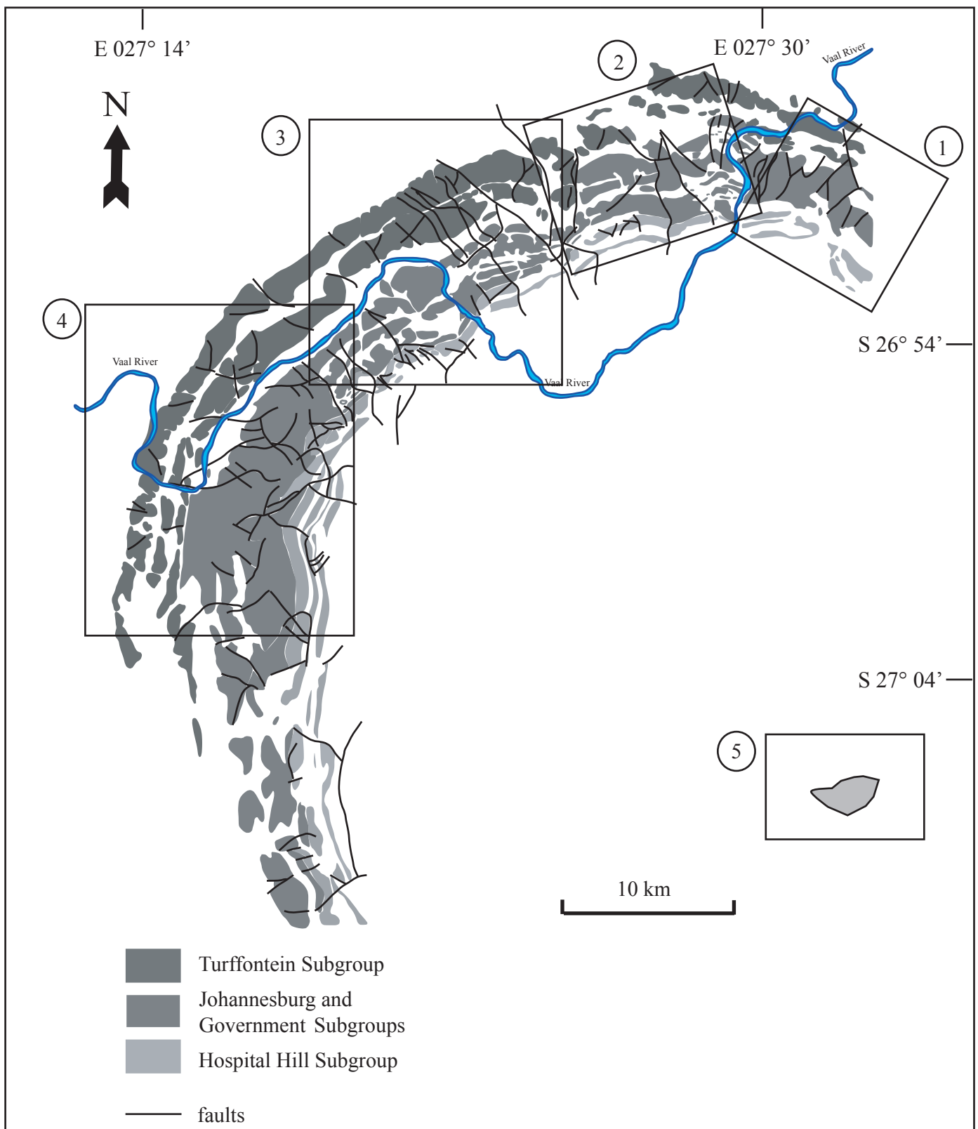
Fig. 1.21: Schematic map of the exposed collar strata in the Vredefort Dome showing the main lithologies and major faults. The numbered insets (1 to 5) cover the studied areas and are presented in detail with locations in Appendix No. 2 (based on the map by Bisschoff 2000).
