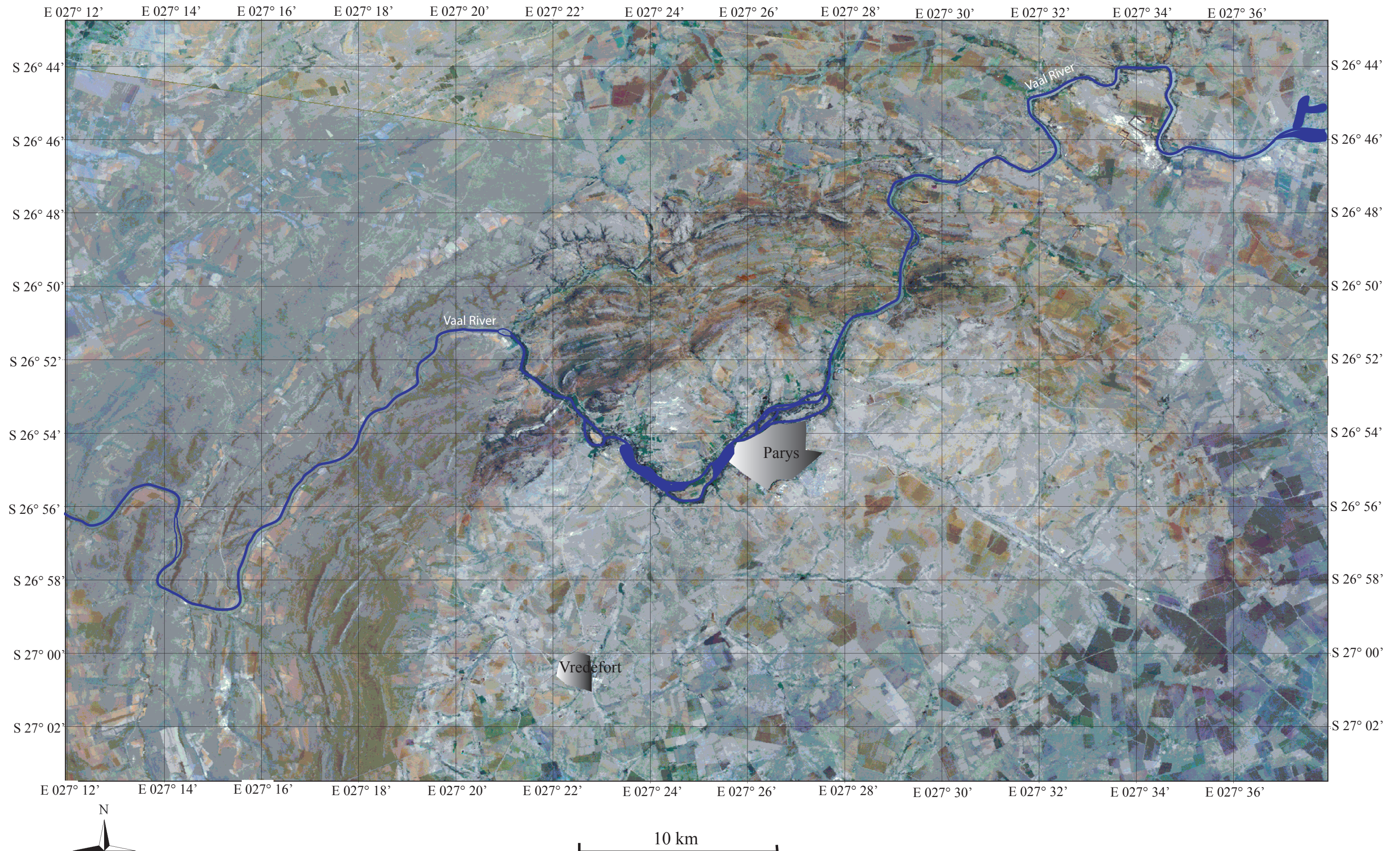
Fig. 1.20: Landsat image with a TM 321 true colour combination of the Vredefort Dome showing the northern parts of the collar and the core. This Landsat image was used additionally to the detailed surface mapping to support and complement the dataset of large-scale structures in the collar rocks of the Vredefort Dome (courtesy of DeBeers Mining Corporation, Johannesburg). For details and flight information see Appendix No. 1a.
