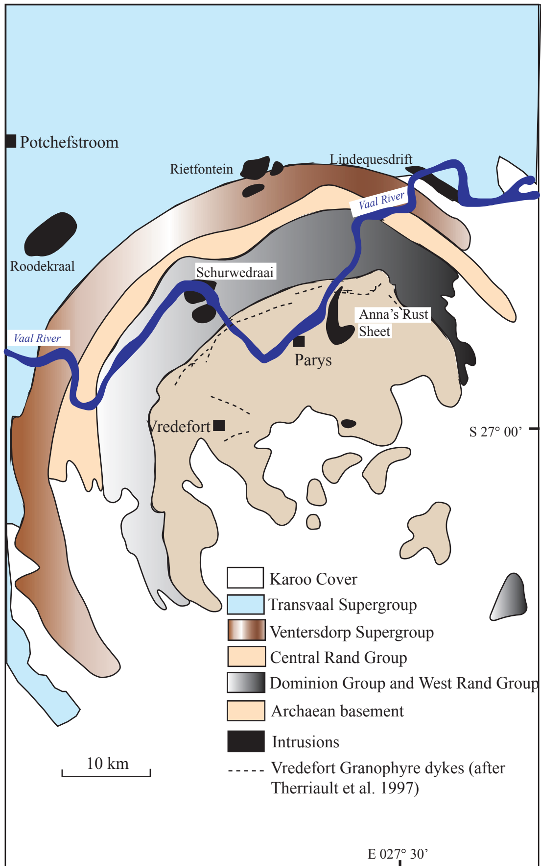
Fig. 1.11: Schematic map of the Vredefort Dome showing the intrusive complexes in the area and the distribution and exposure of the Vredefort Granophyre (modified after Gibson and Reimold 2001).
